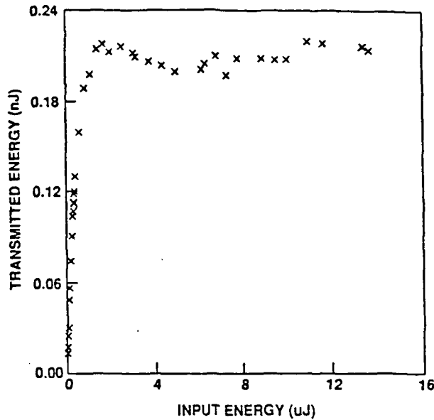
Figure 10. Input / output response of a CAP solution optical limiter for 30 ps 532 nm pulses. Solution cell pathlength was 1 cm. Beam waist radius was 20 \mu\text{m} . Solution concentration was 7.9 \times 10^{-4} M corresponding to 34% transmission at 532 nm for 1 cm.
