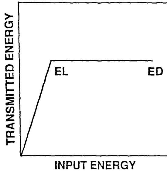
Figure 1. Input-output response of an ideal optical limiter. EL is the threshold limiting energy, ED is the damage threshold and the dynamic range is defined as DR = ED/EL .
