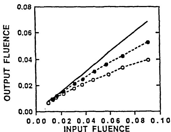
Figure 5. Nanosecond nonlinear transmission of CAP (filled circles) and SiNc (open circles) solutions. Solid line corresponds to linear response with T = 0.75 . Fluence is in J/cm^2 .
