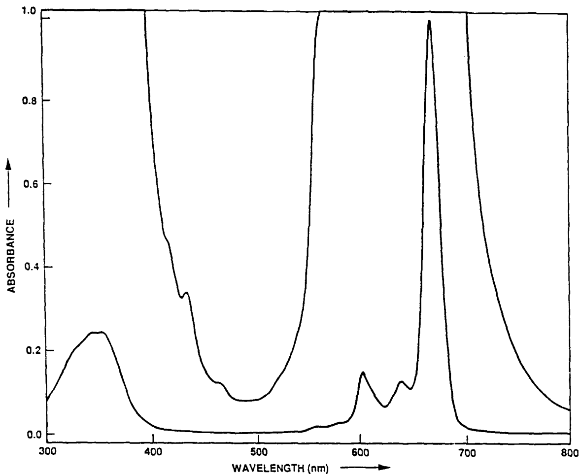
Figure 3. Absorption spectrum of chloroaluminumphthalocyanine in ethanol solution. The lower trace is for a concentration of 4 \times 10^{-6} M and the upper trace is for 3.2 \times 10^{-4} M. The pathlength is 1 cm.
