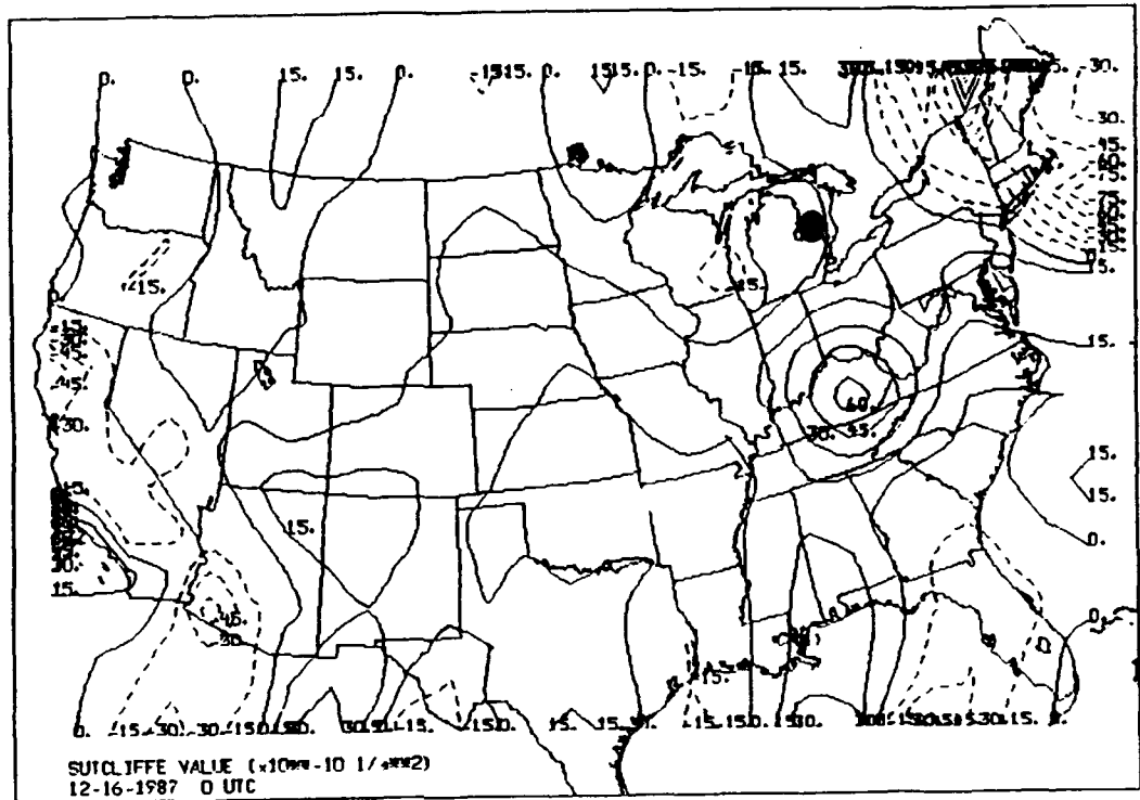
Figure 4-10. Sutcliffe Equation Analysis Model total values for 00 UTC 16 Dec 87 ( 10^{-10} \text{ s}^{-2} ). Dot is surface storm center. Solid lines are positive values and dashed lines are negative values.
