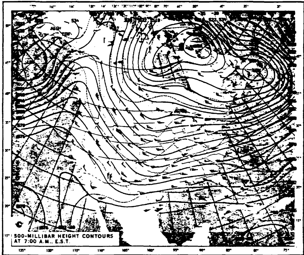
Figure 4-12c. 12 UTC 13 Feb 91 500mb Analysis. Solid lines depict geopotential height (decameters); dashed lines depict isotherms (C) (NOAA, 1991).
