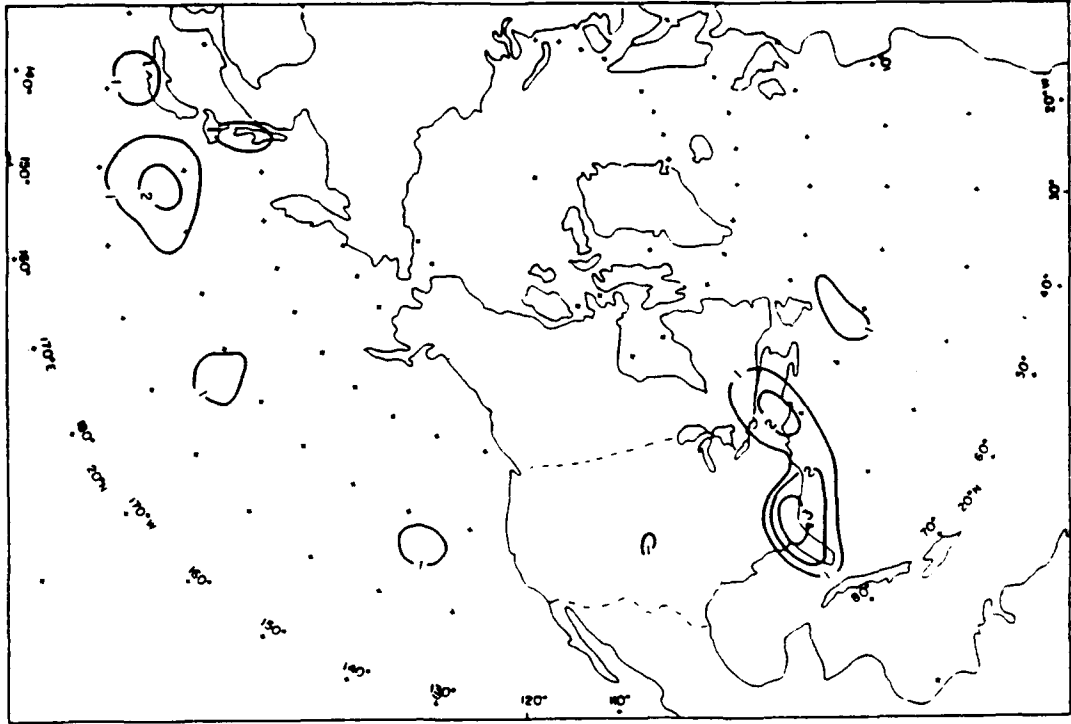
Figure 2-3. Geographic distribution of explosive cyclones (after Roebber, 1984).
