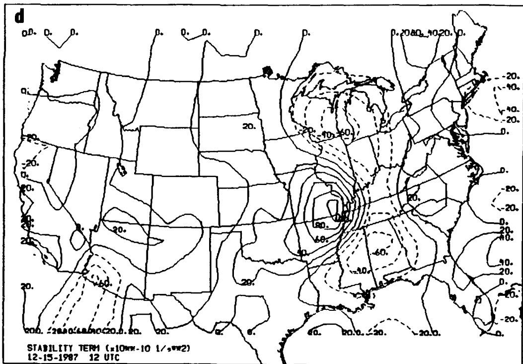
Figure 4-9. c) Thickness Advection Term values for 12 UTC 15 Dec 87 ( 10^{-10} \text{ s}^{-2} ). Solid lines are positive values and dashed lines are negative values. d) Stability Term values for 12 UTC 15 Dec 87 ( 10^{-10} \text{ s}^{-2} ). Solid lines are positive values and dashed lines are negative values.
