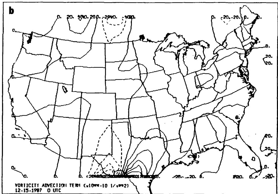
Figure 4-8. a) Sutcliffe Equation Analysis Model total values for 00 UTC 15 Dec 87 ( 10^{-10} \text{ s}^{-2} ). Dot is surface storm center. Solid lines are positive values and dashed lines are negative values. b) Vorticity Advection Term values for 00 UTC 15 Dec 87 ( 10^{-10} \text{ s}^{-2} ). Solid lines are positive values and dashed lines are negative values.
