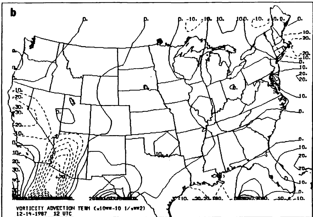
Figure 4-7. a) Sutcliffe Equation Analysis Model total values for 12 UTC 14 Dec 87 ( 10^{-10} \text{ s}^{-2} ). Dot is surface storm center. Solid lines are positive values and dashed lines are negative values. b) Vorticity Advection Term values for 12 UTC 14 Dec 87 ( 10^{-10} \text{ s}^{-2} ). Solid lines are positive values and dashed lines are negative values.
