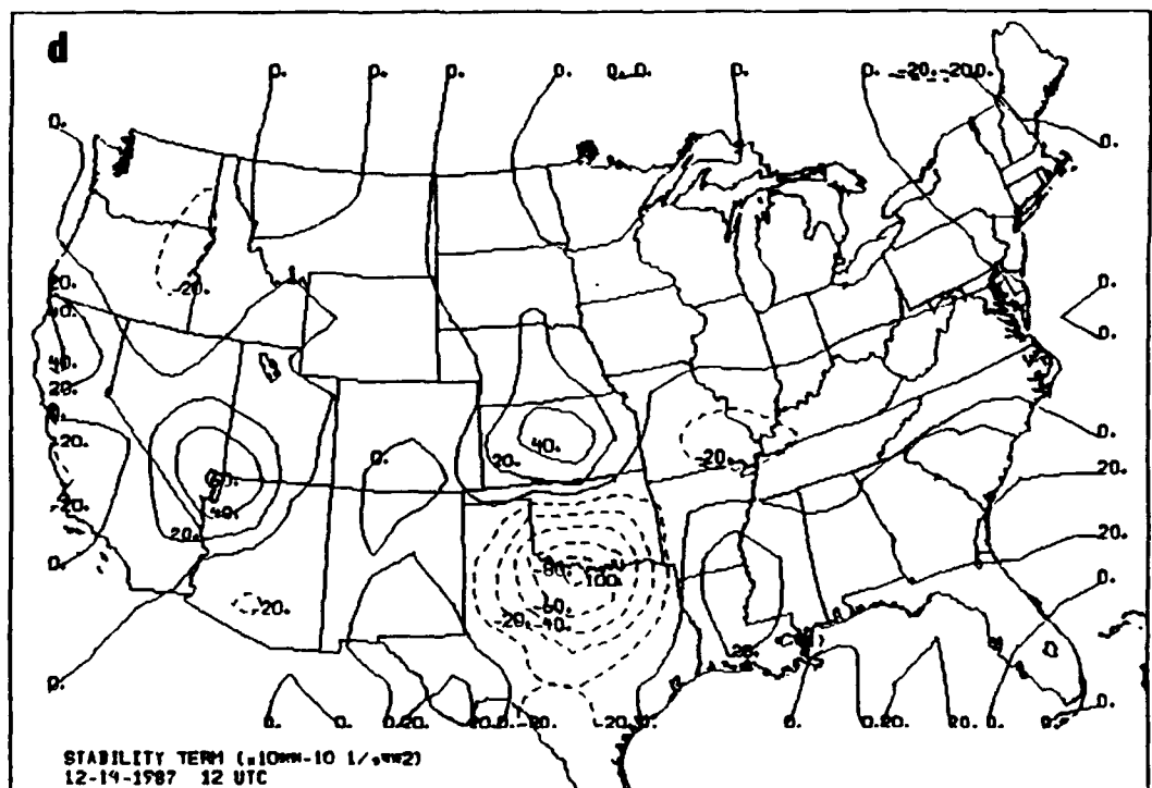
Figure 4-7. c) Thickness Advection Term values for 12 UTC 14 Dec 87 ( 10^{-10} \text{ s}^{-2} ). Solid lines are positive values and dashed lines are negative values. d) Stability Term values for 12 UTC 14 Dec 87 ( 10^{-10} \text{ s}^{-2} ). Solid lines are positive values and dashed lines are negative values.
