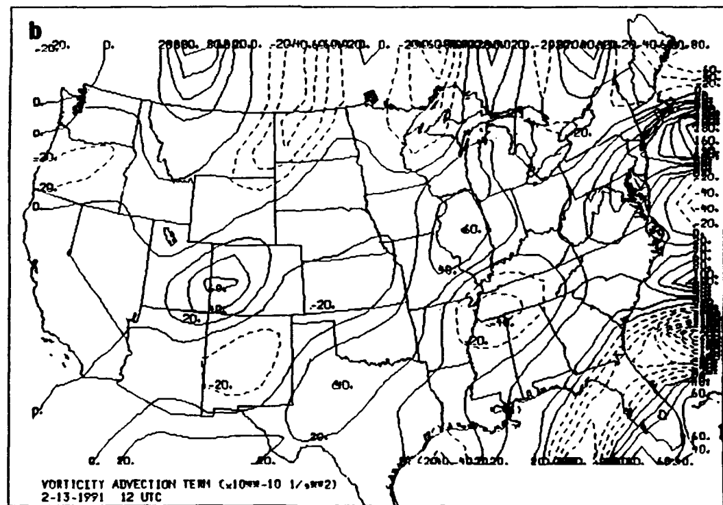
Figure 4-15. a) Sutcliffe Equation Analysis Model total values for 12 UTC 13 Feb 91 ( 10^{-10} \text{ s}^{-2} ). Dot is surface storm center. Solid lines are positive values and dashed lines are negative values. b) Vorticity Advection Term values for 12 UTC 13 Feb 91 ( 10^{-10} \text{ s}^{-2} ). Solid lines are positive values and dashed lines are negative values.
