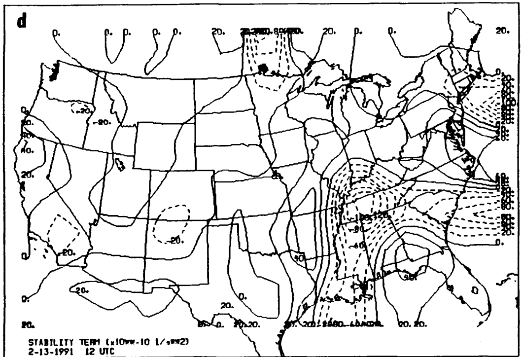
Figure 4-15. c) Thickness Advection Term values for 12 UTC 13 Feb 91 ( 10^{-10} \text{ s}^{-2} ). Solid lines are positive values and dashed lines are negative values. d) Stability Term values for 12 UTC 13 Feb 91 ( 10^{-10} \text{ s}^{-2} ). Solid lines are positive values and dashed lines are negative values.
