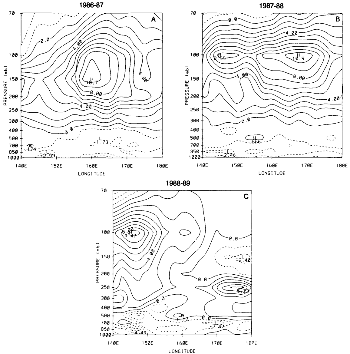
Figure 5.25: Pressure-longitude diagrams of divergence during the maximum convection phase of the MJO averaged between the equator and 10.0^{\circ}\text{S} using the ECMWF data set for a.) 1986-87, b.) 1987-88 and c.) 1988-89. Solid lines indicate divergence and dashed lines indicate convergence. The units are \times 10^{-6} \text{ s}^{-1} and the contour interval is 1.0 \times 10^{-6} \text{ s}^{-1} .
