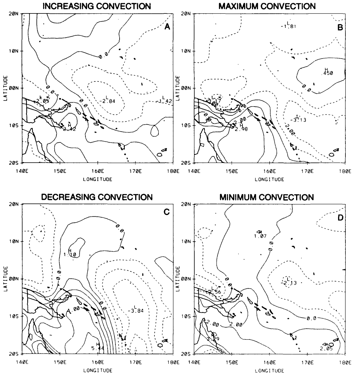
Figure 5.17: 1986-87 latitude-longitude diagrams of ECMWF composited meridional wind ( \text{m s}^{-1} ) at 850 mb for the a.) increasing, b.) maximum, c.) decreasing and d.) minimum convection phases of the MJO. Solid contours represent southerly winds and dashed represent northerlies. The contour interval is 1.0 \text{ m s}^{-1} .
