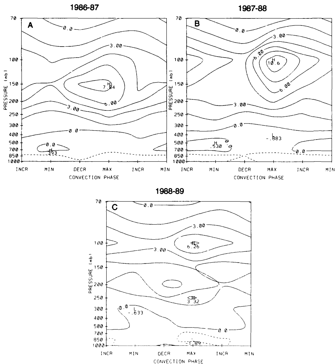
Figure 5.23: Pressure-phase diagrams of divergence at 5.0^{\circ}\text{S} averaged between 140^{\circ}\text{E} and 180^{\circ} using the ECMWF data set for a.) 1986-87, b.) 1987-88 and c.) 1988-89. Solid lines indicate divergence and dashed lines indicate convergence. The units are \times 10^{-6} \text{ s}^{-1} and the contour interval is 1.5 \times 10^{-6} \text{ s}^{-1} .
