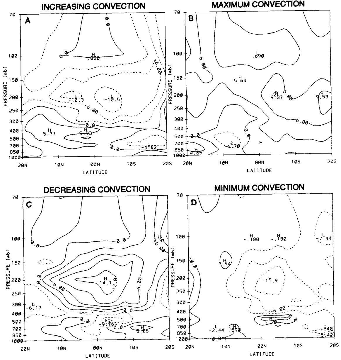
Figure 5.37: Pressure-latitude diagram of relative humidity anomalies (%) averaged from 140°E to 180° for the a.) increasing, b.) maximum, c.) decreasing and d.) minimum convection phase of the MJO. The solid lines are moist anomalies and the dashed are dry. The contour interval is 3.0%.
