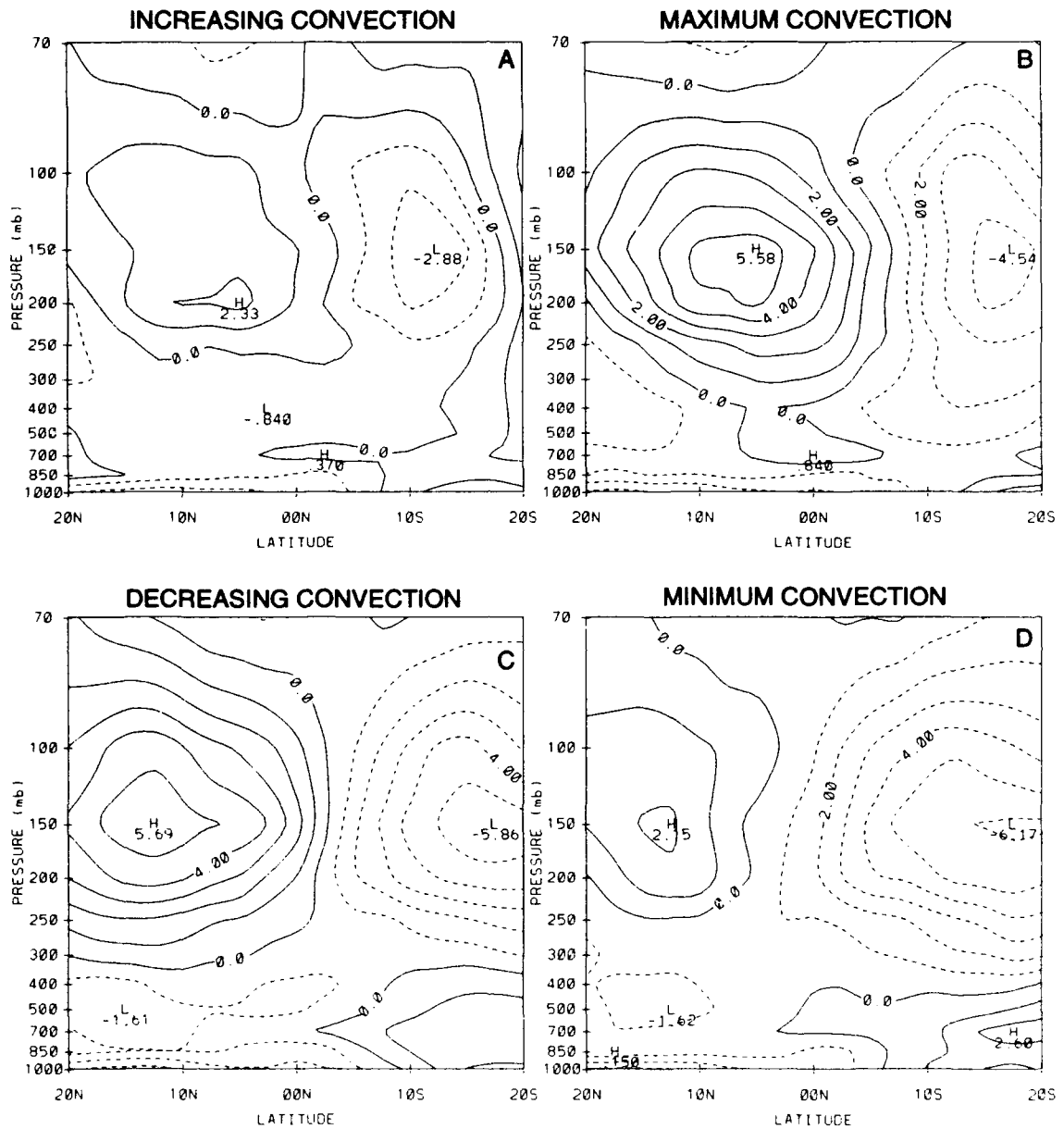
Figure 5.20: 1986-87 pressure-latitude diagrams of ECMWF composited meridional wind ( \text{m s}^{-1} ) averaged from 140^{\circ}\text{E} to 180^{\circ} for the a.) increasing, b.) maximum, c.) decreasing and d.) minimum convection phases of the MJO. Solid contours represent southerly winds and dashed represent northerlies. The contour interval is 1.0 \text{ m s}^{-1} .
