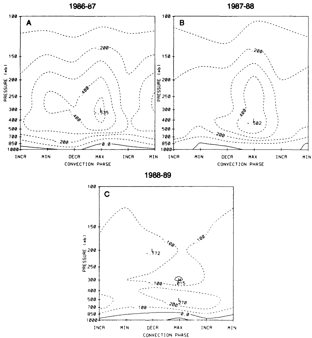
Figure 5.26: Pressure-phase diagrams of ECMWF composited vertical motion ( \mu\text{b s}^{-1} ) averaged from 140^{\circ}\text{E} to 180^{\circ} at 5.0^{\circ}\text{N} for a.) 1986-87, b.) 1987-88 and c.) 1988-89. Solid contours represent downward motion and dashed represent upward motion. The contour interval is 0.1 \mu\text{b s}^{-1} .
