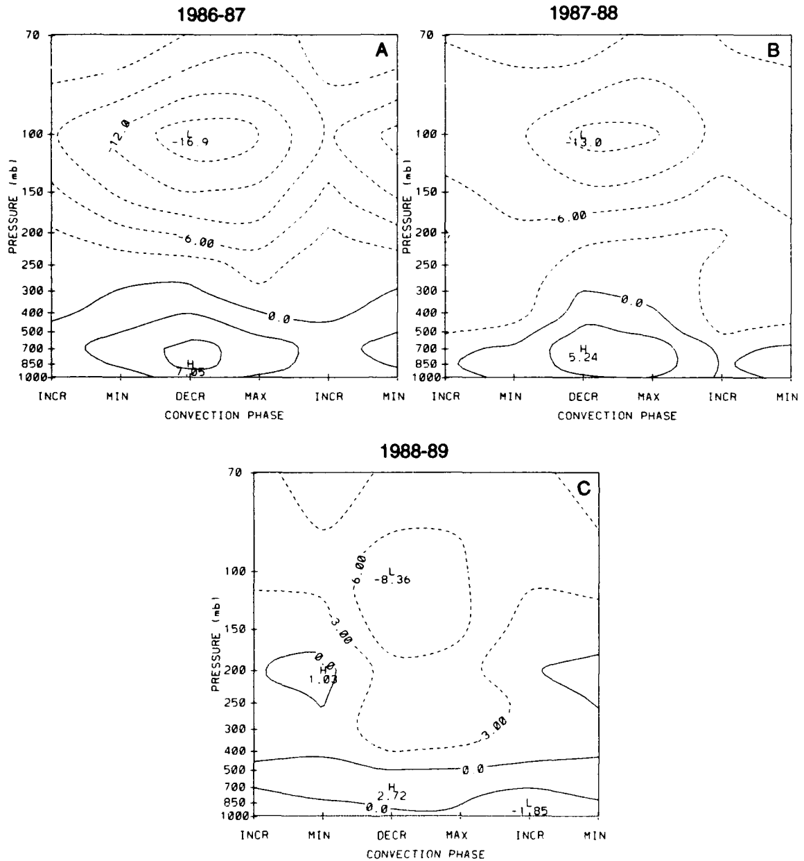
Figure 5.1: Pressure-phase diagrams of ECMWF composited zonal wind ( \text{m s}^{-1} ) averaged from 140^{\circ}\text{E} to 180^{\circ} at 5.0^{\circ}\text{S} for a.) 1986-87, b.) 1987-88 and c.) 1988-89. Solid contours represent westerly winds and dashed represent easterlies. The contour interval is 3.0 \text{ m s}^{-1}
