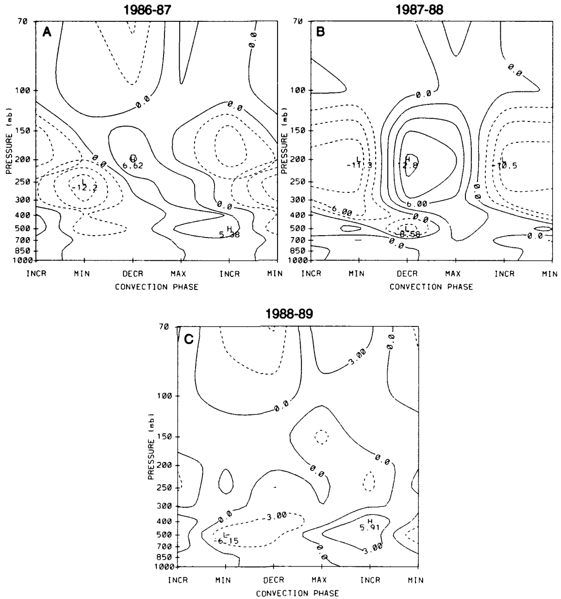
Figure 5.36: Pressure-phase diagram of relative humidity anomalies (%) at 5.0°S averaged from 140°E to 180° for a.) 1986-87, b.) 1987-88 and c.) 1988-89. The solid lines are moist anomalies and the dashed are dry. The contour interval is 3.0%.
