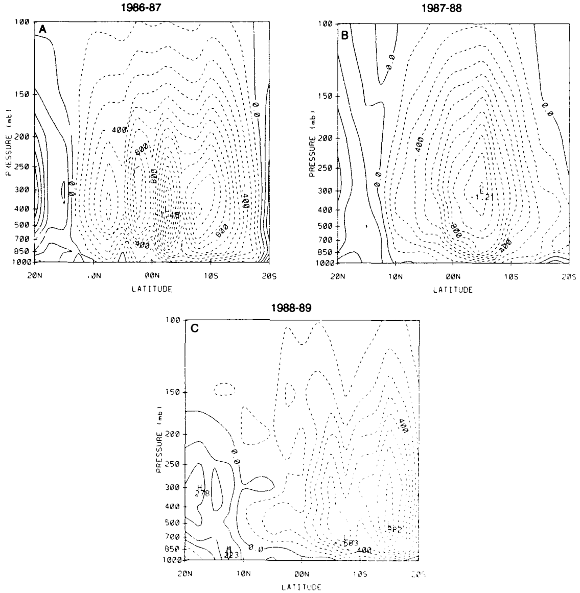
Figure 5.29: Pressure versus latitude diagrams of ECMWF composited vertical motion ( \mu\text{b s}^{-1} ) averaged from 140^\circ\text{E} to 180^\circ for the maximum convective phase for a.) 1986-87. b.) 1987-88 and c.) 1988-89. Solid lines represent downward motion and dashed lines represent upward motion. Contour interval 0.1 \mu\text{b s}^{-1} .
