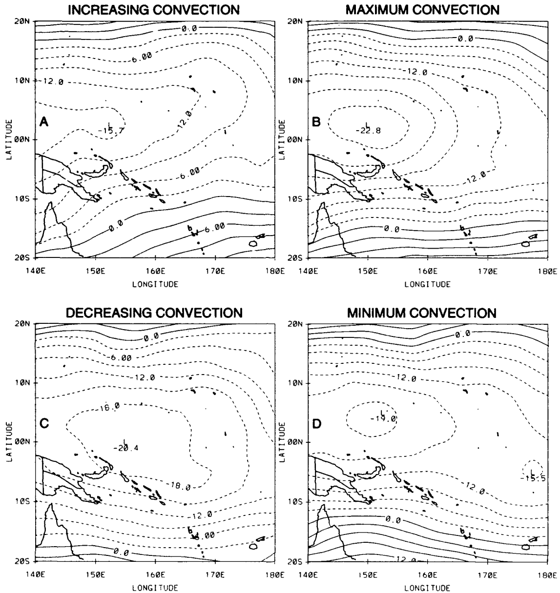
Figure 5.6: 1986-87 latitude-longitude diagrams of ECMWF composited zonal wind ( \text{m s}^{-1} ) at 100 mb for the a.) increasing, b.) maximum, c.) decreasing and d.) minimum convection phases of the MJO. Solid contours represent westerly winds and dashed represent easterlies. The contour interval is 3.0 \text{ m s}^{-1} .
