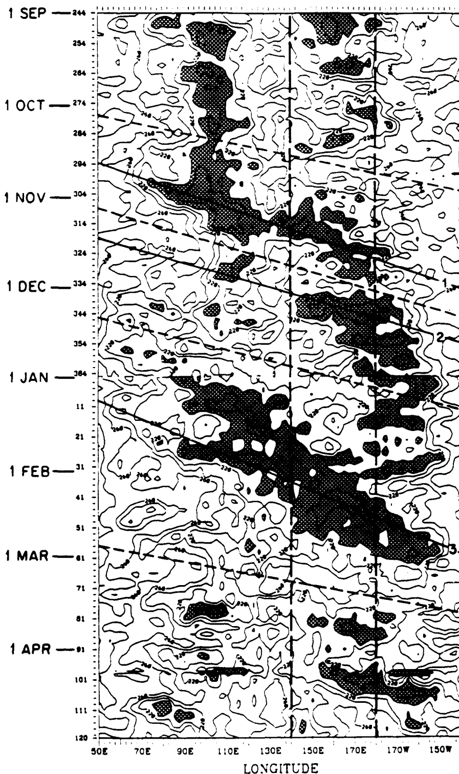
Figure 3.3: Hovmöller of OLR from September 1986 through April 1987 in units of W m^{-2} . Regions of OLR \leq 200 W m^{-2} are cross-hatched and the contour interval is 20 W m^{-2} . The dashed vertical line indicates the zonal boundaries of the domain. The horizontal dashed (solid) lines indicate the axes of maximum (minimum) OLR which correspond to the axes of minimum (maximum) convective activity.
