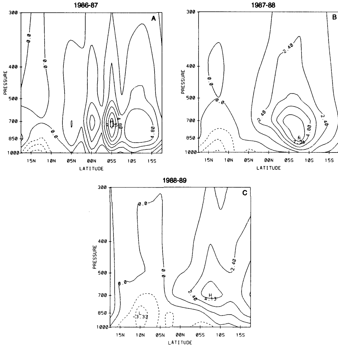
Figure 6.8: Pressure-latitude diagram of Q_2 in ^{\circ}\text{K day}^{-1} for the maximum convection phase of the MJO averaged between 140^{\circ}\text{E} and 180^{\circ} using the ECMWF data set for A.) 1986-87, b.) 1987-88 and c.) 1988-89. Solid lines indicate an apparent moisture sink and dashed lines indicate an apparent moisture source. The contour interval is 1.2^{\circ}\text{K day}^{-1} .
