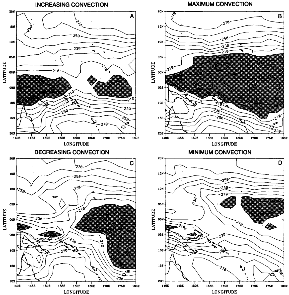
Figure 4.2: Composited OLR based on the MJO phase at 160^\circ\text{E} for 1986-87 for the a.) increasing, b.) maximum, c.) decreasing and d.) minimum convection phases. Units are \text{W m}^{-2} and the contour interval is 10 \text{ W m}^{-2} . Values \leq 200 \text{ W m}^{-2} are cross-hatched.
