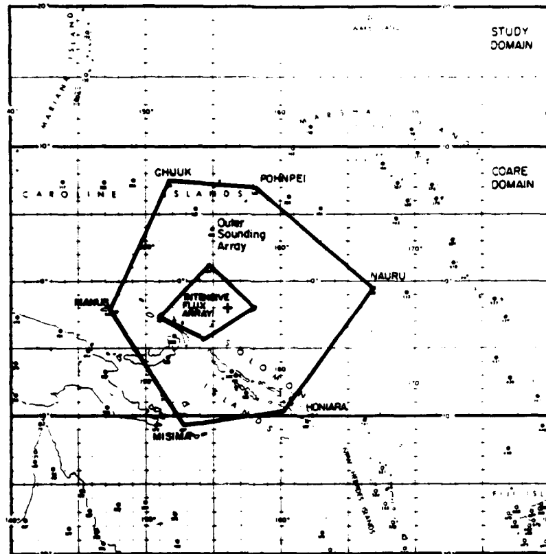
Figure 3.2: Map of the western Pacific Ocean showing the domain of this study and the domain of the 1992-93 TOGA/COARE experiment (from the TOGA/COARE Operations Plan 1992). The outer region represents the domain of this study. The rectangular box indicates the COARE large-scale domain. The larger trapezoid is the outer sounding array (OSA) and the interior region is the intensive flux array (IFA).
