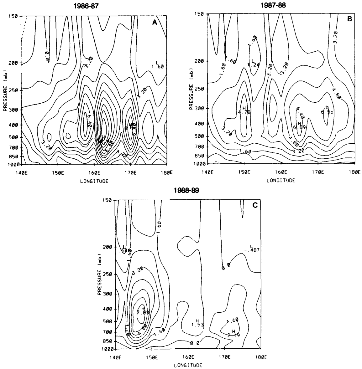
Figure 6.9: Pressure- longitude diagram of Q_1 in ^{\circ}\text{K day}^{-1} for the maximum convection phase of the MJO averaged between the equator and 10.0^{\circ}\text{S} using the ECMWF data set for a.) 1986-87, b.) 1987-88 and c.) 1988-89. Solid lines indicate an apparent heat source and dashed lines indicate an apparent heat sink. The contour interval is 0.8^{\circ}\text{K day}^{-1} .
