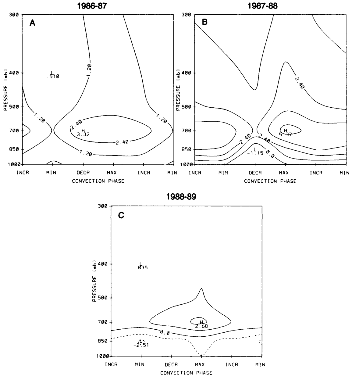
Figure 6.2: Pressure-convective phase of Q_2 averaged from 140^\circ\text{E} to 180^\circ at 2.5^\circ\text{S} for a.) 1986-87, b.) 1987-88 and c.) 1988-89 in units of ^\circ\text{K day}^{-1} . The solid lines indicate the apparent moisture sink and the dashed lines indicate the apparent moisture source. The contour interval is 1.2^\circ\text{K day}^{-1} .
