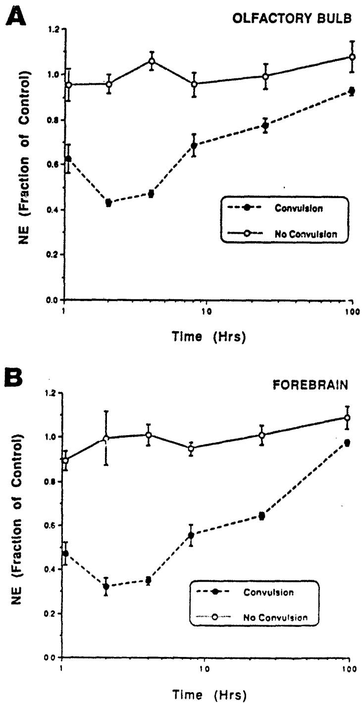
Figure 7. Differences in Norepinephrine (NE) Levels in Convulsing and Nonconvulsing Animals after a Single 78 \mu\text{g}/\text{kg} soman injection. A) olfactory bulb. B) forebrain. Time axis is logarithmic.
