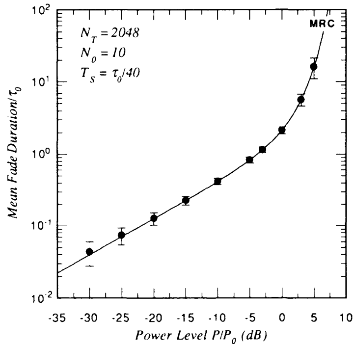
Figure 21b. Mean fade duration of 200\tau_0 realizations.
