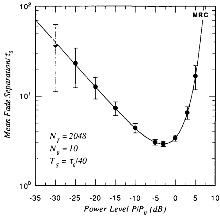
Figure 22b. Mean fade separation of 200\tau_0 realizations.
