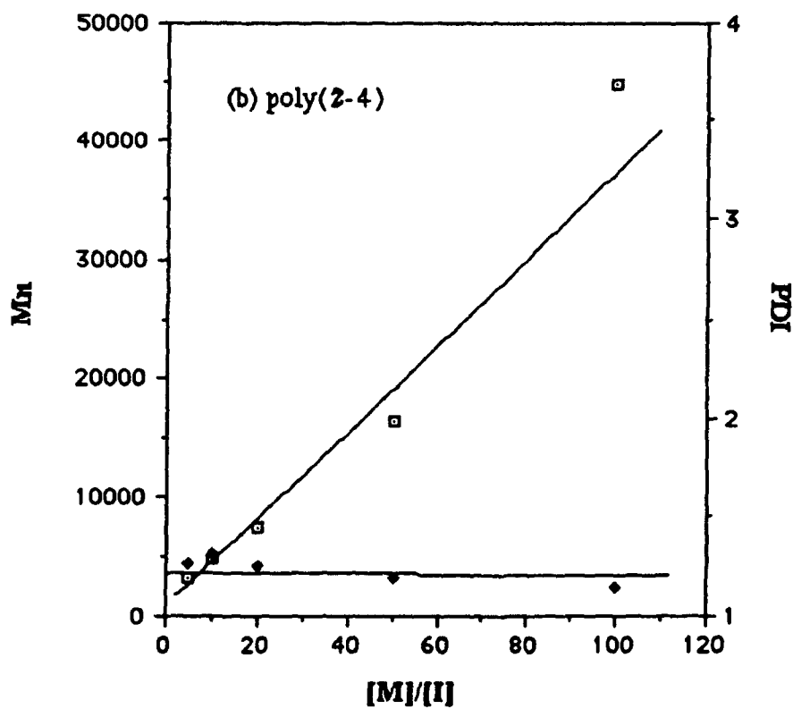
Figure 1. Plots of number average molecular weight ( M_n ) and the polydispersity ( PDI = M_w/M_n ) of (a) poly(1-5), and (b) poly(2-4) versus the molar ratio of monomer to initiator ( [M]/[I] ).
