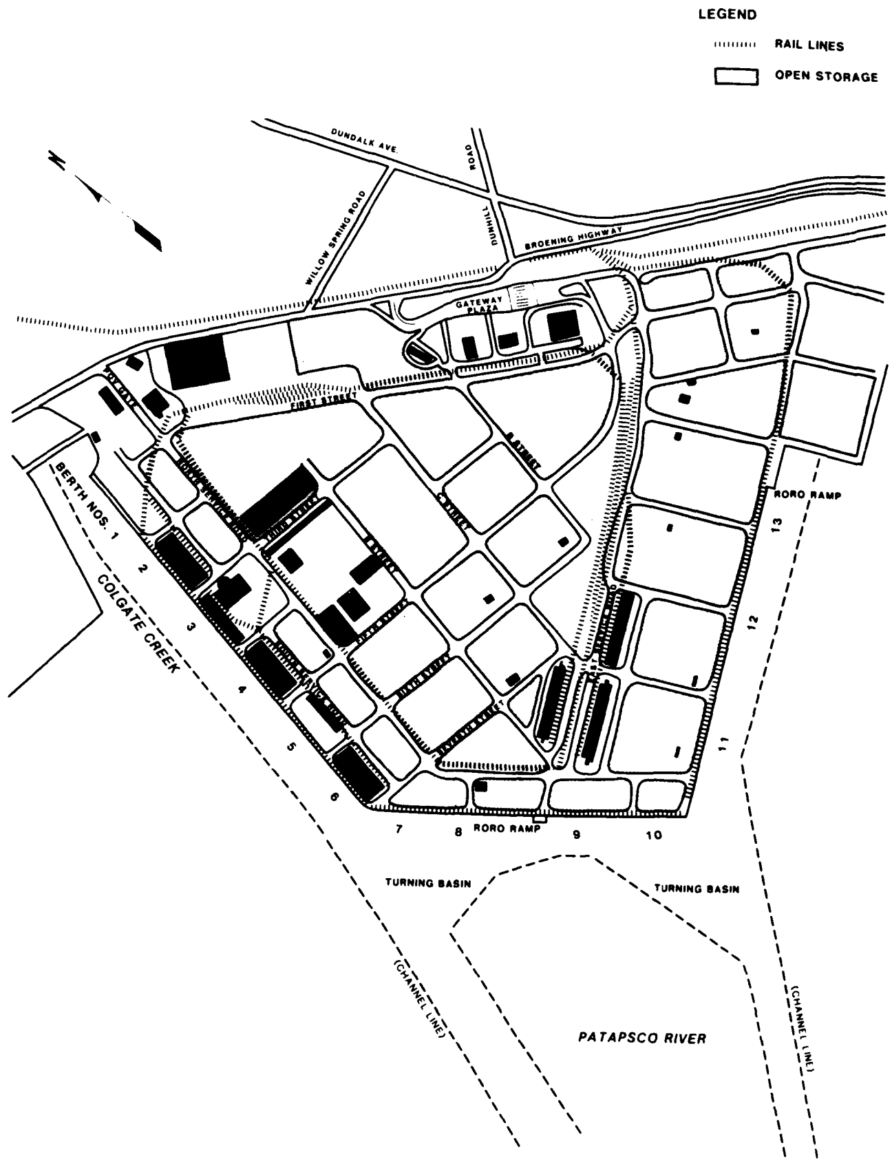
Figure II-BAL-6. Plan of Dundalk Marine Terminal.
