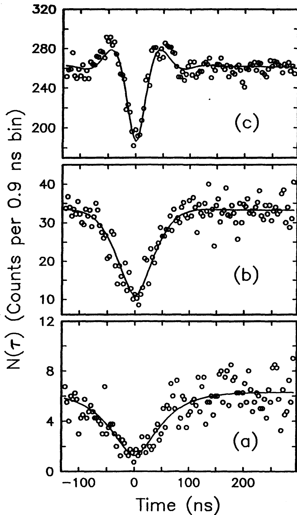
FIG. 2. N(\tau) for a single pentacene molecule ( \lambda_{exc} \approx 593.4 \text{ nm} ). The antibunching is clearly seen for t \rightarrow 0 . Rabi-frequencies \Omega : (a) 11.2 MHz; (b) 26.2 MHz; (c) 68.9 MHz. For example, case (b) involved 3.6 \times 10^3 start-stop events over a time period of 1 hr. The solid lines are fits to the data with \Omega = (a) 1-10 MHz, (b) 25.5 MHz, and (c) 71.3 MHz.
