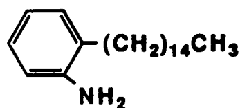
2-pentadecyl aniline
