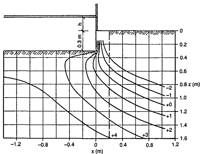
Figure 94. Isotherms for a long building. (10 m wide; clay soil; outside temperature = -9.0^{\circ}\text{C} ; U-value of floor slab = 0.582\text{ W/m}^2\text{K} ; heat flow through foundation wall = 1.19\text{ W/mK} ; crawl space ventilation rate = 1\text{ m}^3/\text{m}^2\text{h} ; crawl space temperature = 3.2^{\circ}\text{C} .) (From Adamson 1972.)
