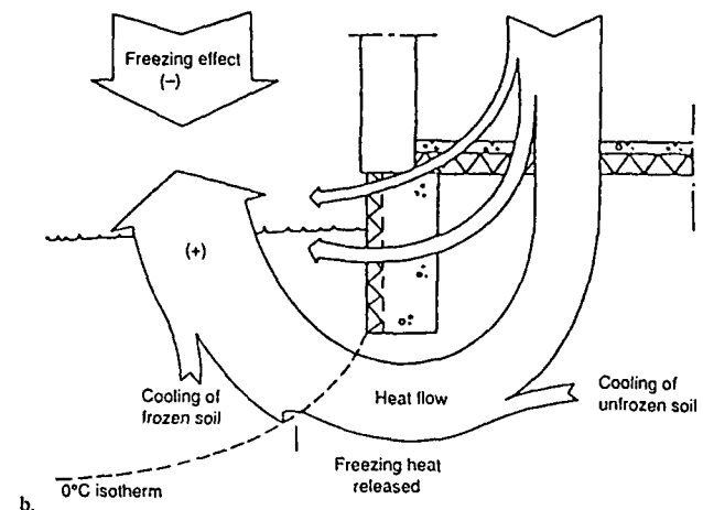
Figure 16. Frost protection principle in Finland using a 0^{\circ}\text{C} isotherm limitation. (From VTT 1987.)
