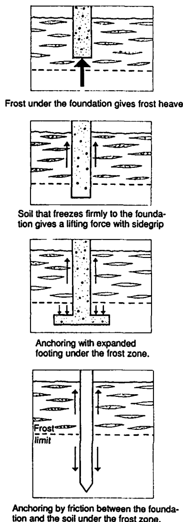
Figure 145. Frost heave and sidegrip. (From Torgersen 1976b.)
