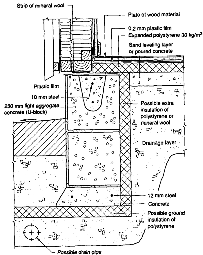
Figure 84. Light floor with foundation wall of light aggregate concrete. (From NBI 1986.)
