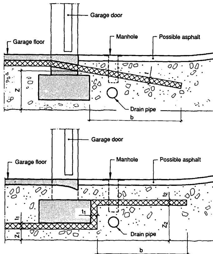
Figure 141. Frost protection of a garage entrance drive. (From NBI 1978.)
