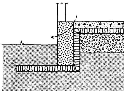
Figure 158. Foundation placed on ground insulation. (From Thue 1972.)
