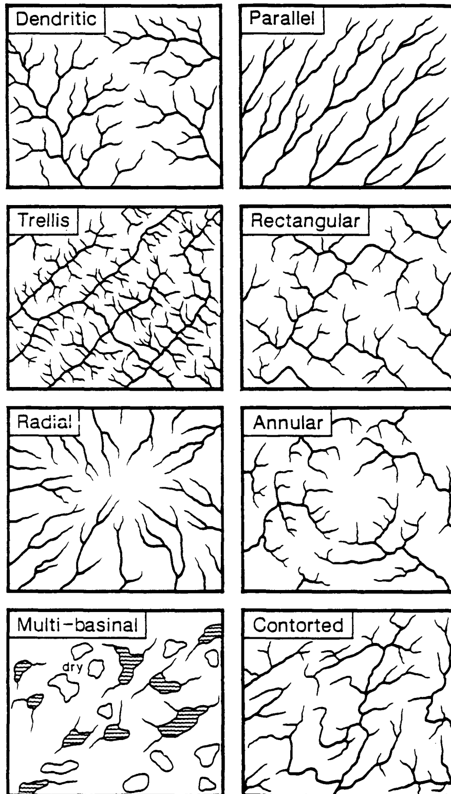
Figure 1. Basic Drainage Patterns (Adapted from Howard, 1967)
