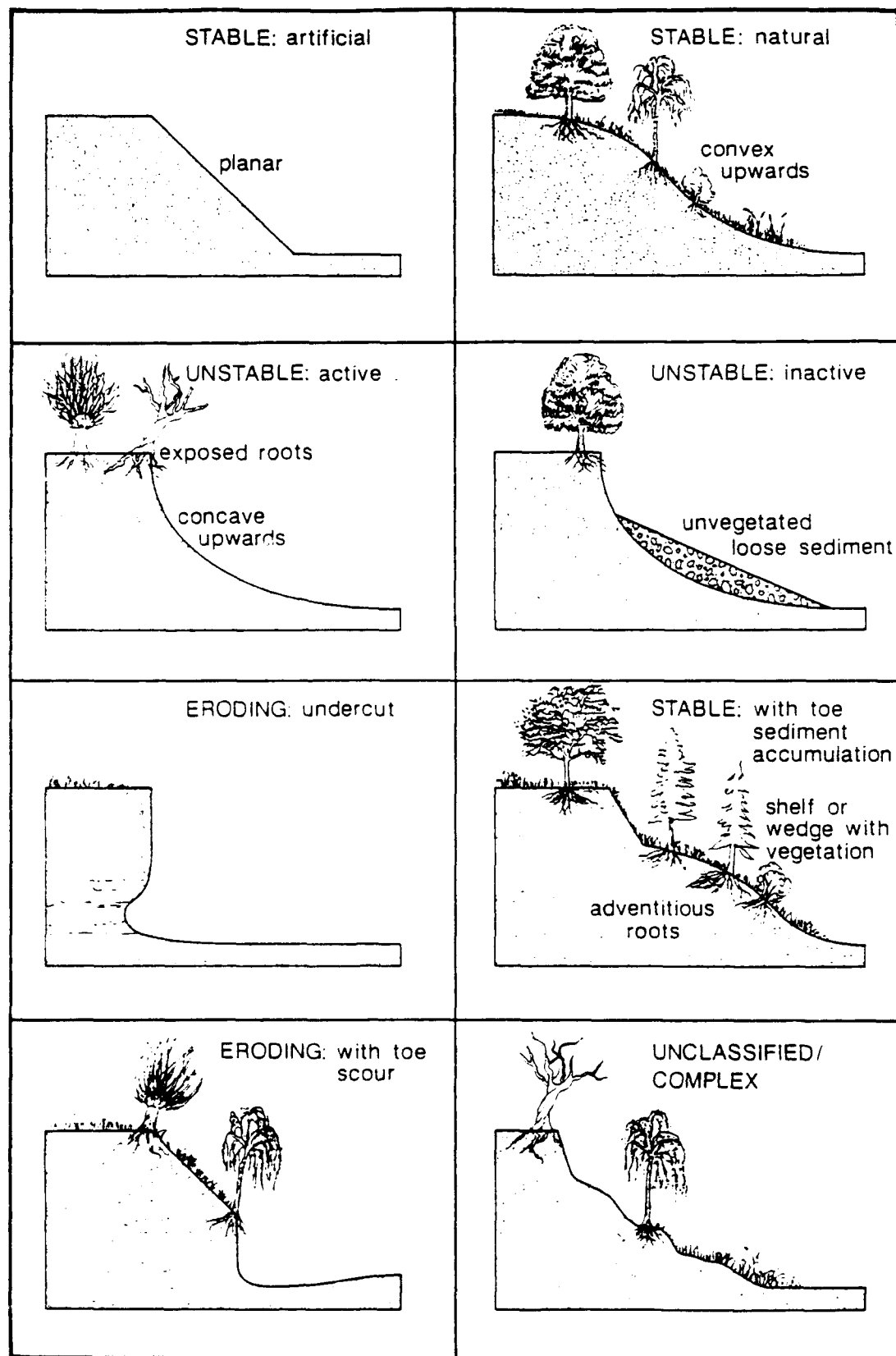
Figure 20. Typical bank profiles
