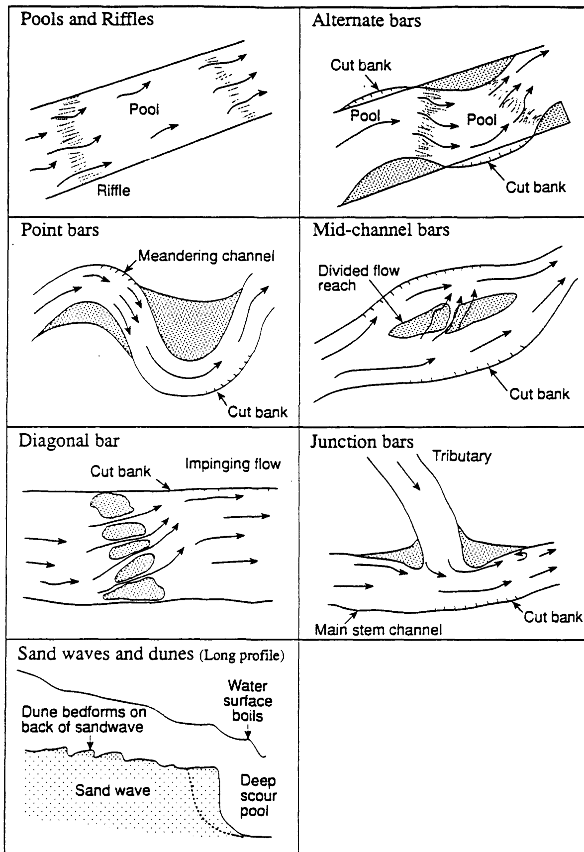
Figure 15. Bar type classification
