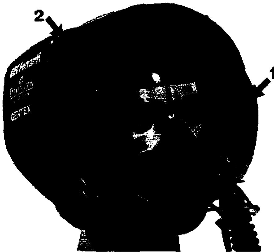
Figure 1. In a helmet under development by a GEC/Ferranti-led team, symbols from two projectors (Arrow 1) will show head-up display information as well as night vision enhancement from built-in image intensifiers (Arrow 2), projected onto the pilot's visor. (Source: Aviation Week , 11 November 1991, p. 78)
