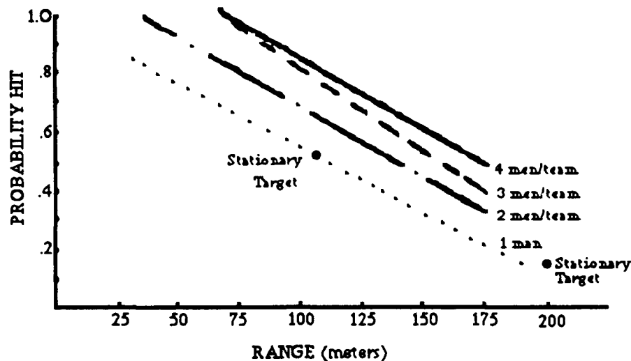
Figure III-13. LAW vs. Moving Tank
