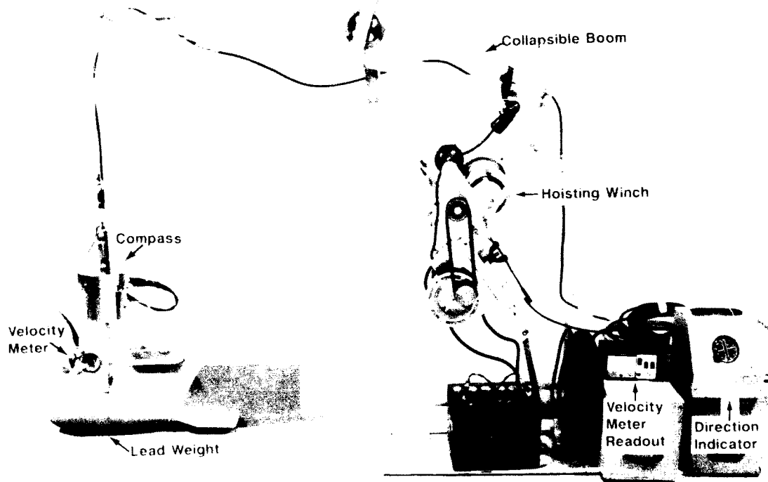
Figure 5. Components of the field instrument assembly
