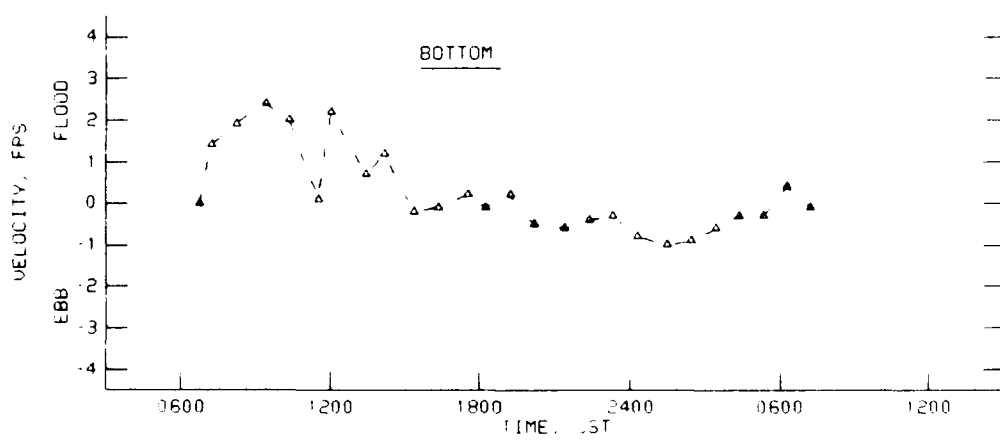
VELOCITIES AT R6.0A 25-26 MAY 1990
