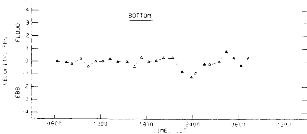
VELOCITIES AT R4.0A 25-26 MAY 1990
