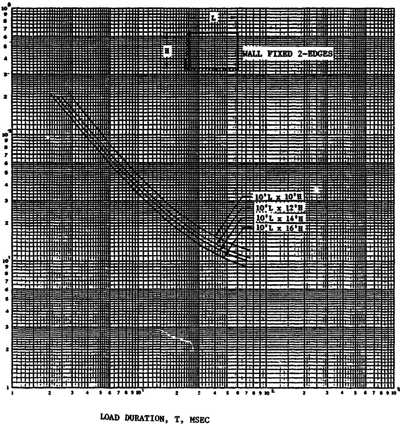
FIGURE 3-5 ALLOWABLE PEAK SHOCK PRESSURE VS LOAD DURATION
