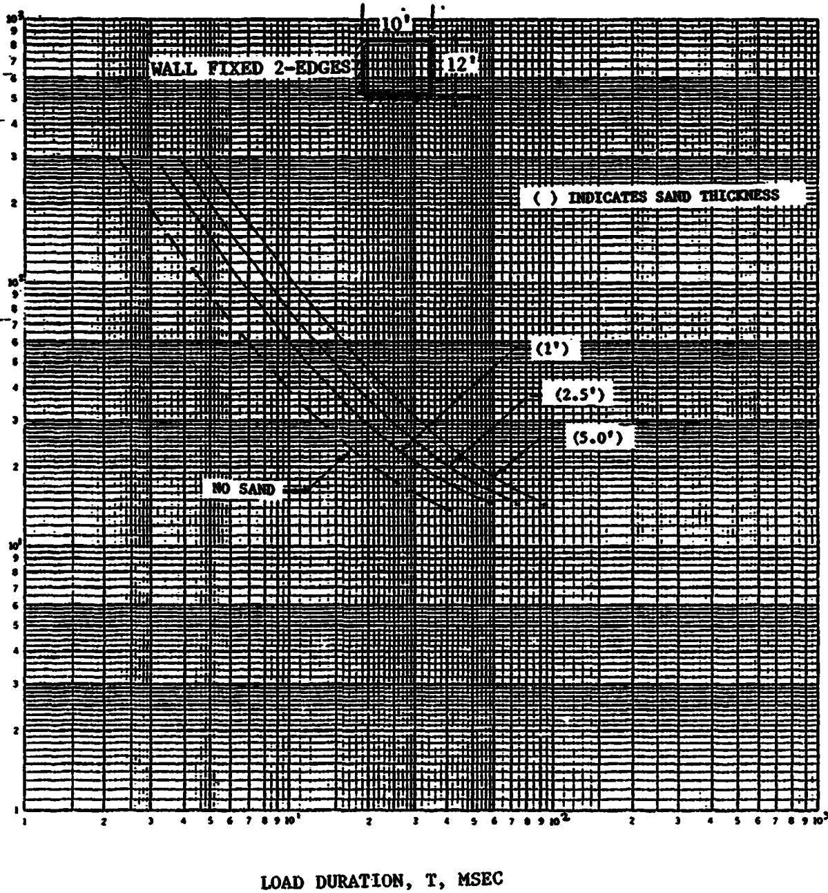
FIGURE 3-20 ALLOWABLE PEAK SHOCK PRESSURE VS LOAD DURATION
