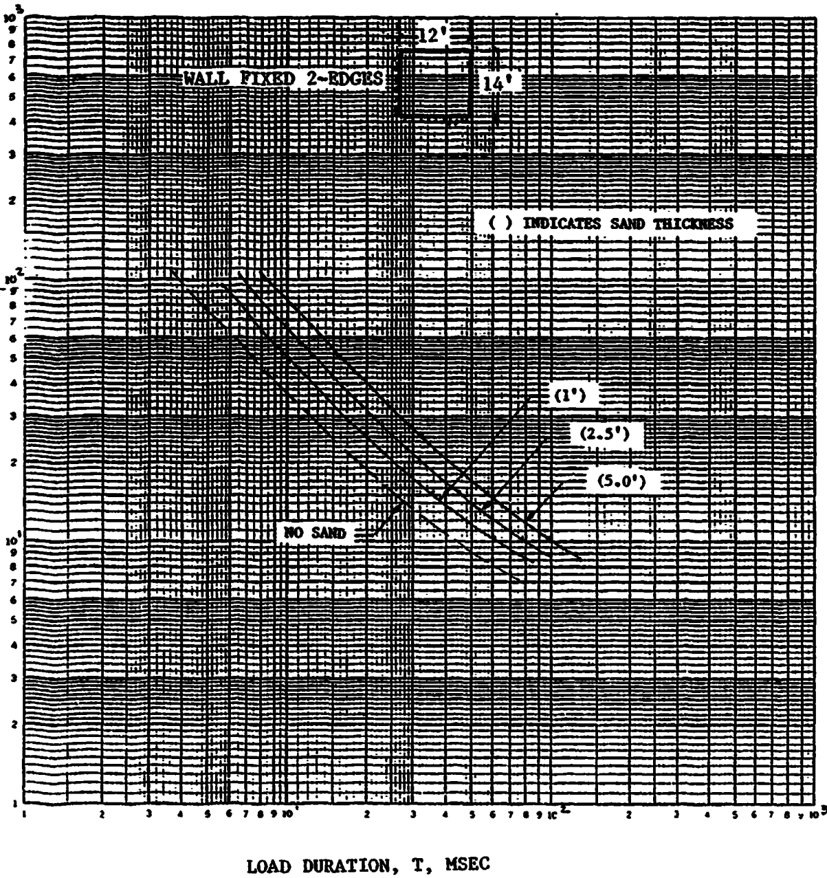
FIGURE 3-25 ALLOWABLE PEAK SHOCK PRESSURE VS LOAD DURATION
