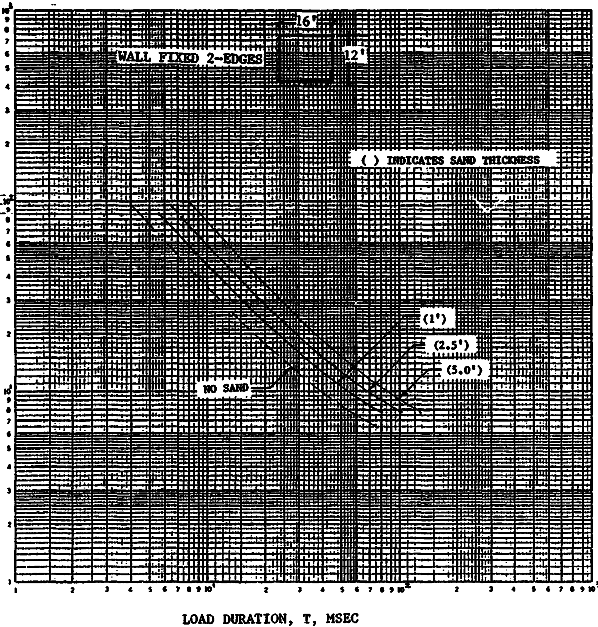
FIGURE 3-32 ALLOWABLE PEAK SHOCK PRESSURE VS LOAD DURATION
