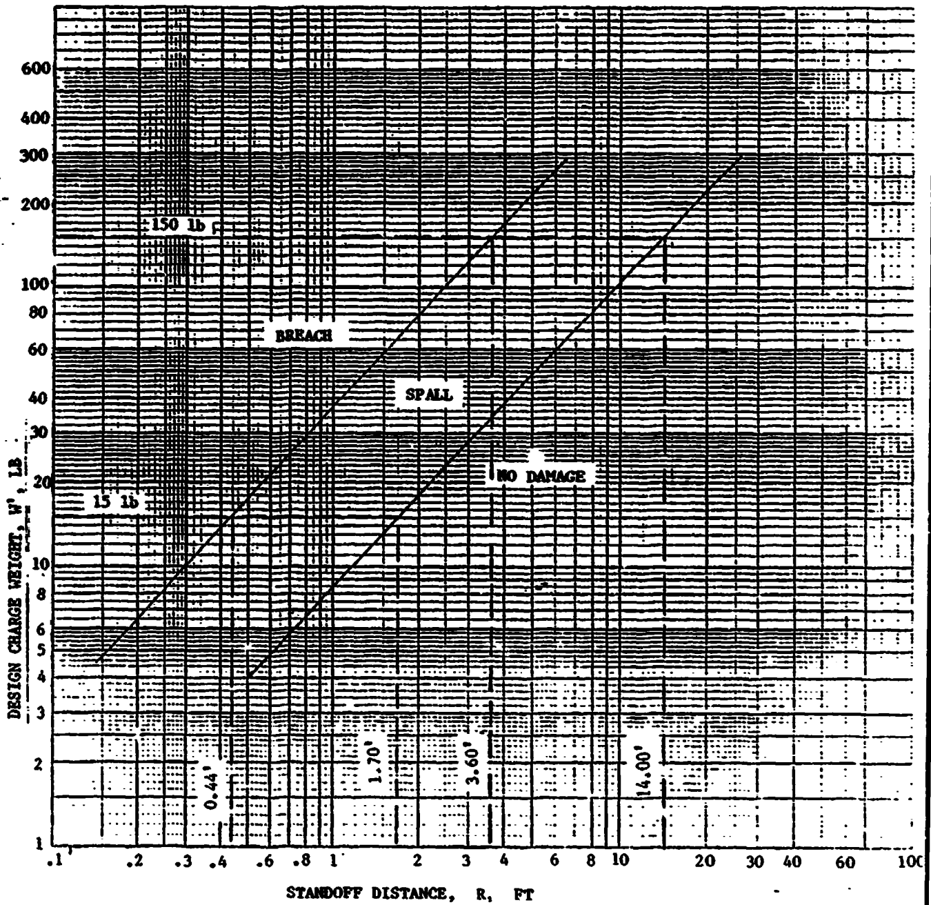
FIGURE 3-40 DESIGN CHARGE WEIGHT VERSUS STANDOFF DISTANCE (BARE CHARGE)
