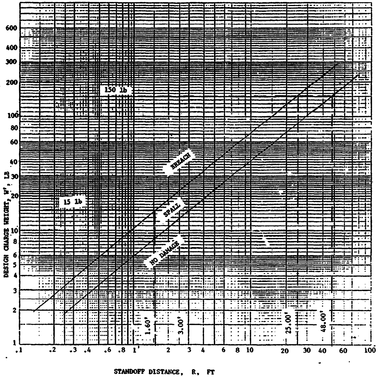
FIGURE 3-41 DESIGN CHARGE WEIGHT VERSUS STANDOFF DISTANCE (CASED CHARGES)
