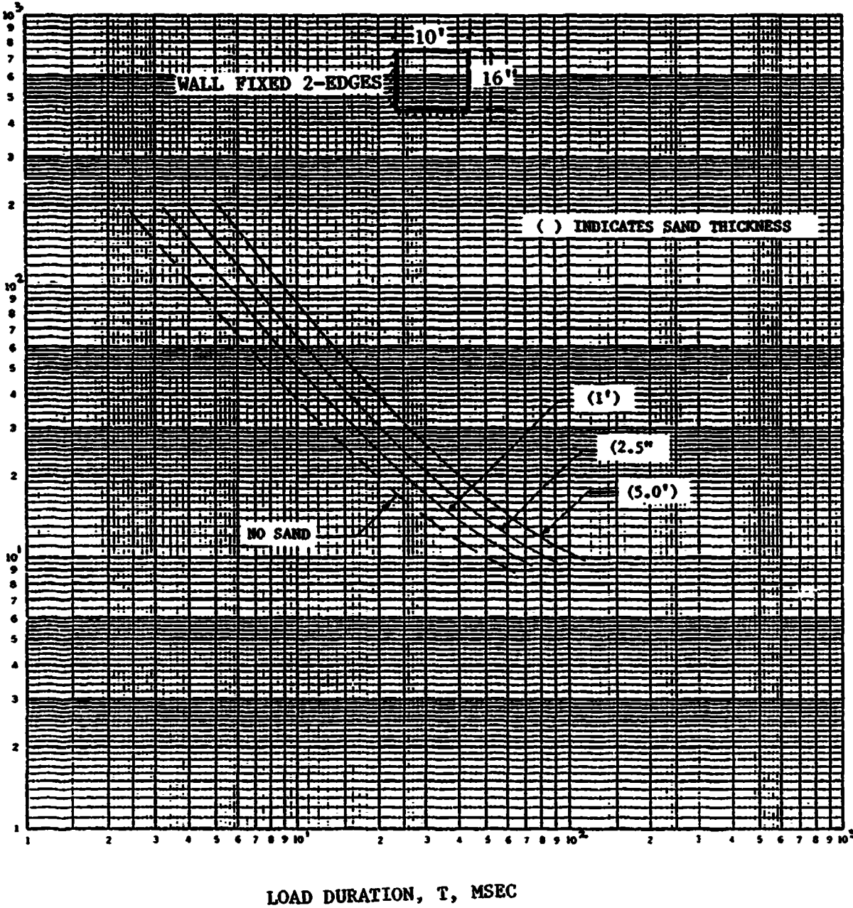
FIGURE 3-22 ALLOWABLE PEAK SHOCK PRESSURE VS LOAD DURATION
