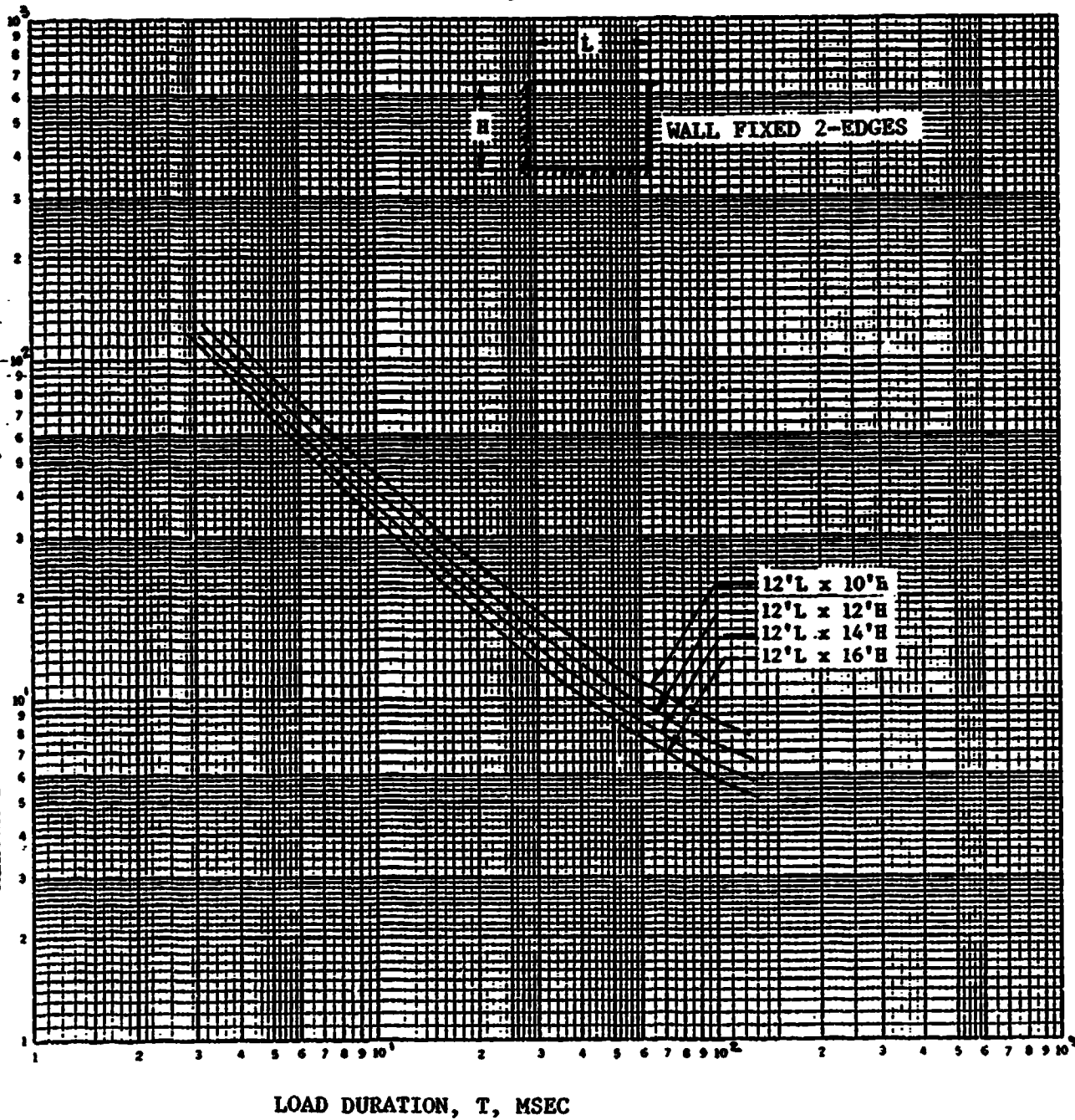
FIGURE 3-6 ALLOWABLE PEAK SHOCK PRESSURE VS LOAD DURATION
