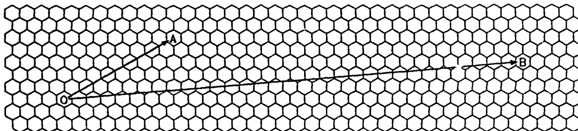
Figure 1. Two-dimensional graphite lattice structure. Line segments OA and OB represent two lattice translation vectors for the hexagonal lattice.
