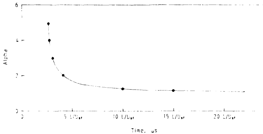
Figure 7: Smooth line joining the theoretical points which show the relationship between \alpha , (U_s - u_p) and the time to attenuate a shock wave in a medium following flyer plate impact.
