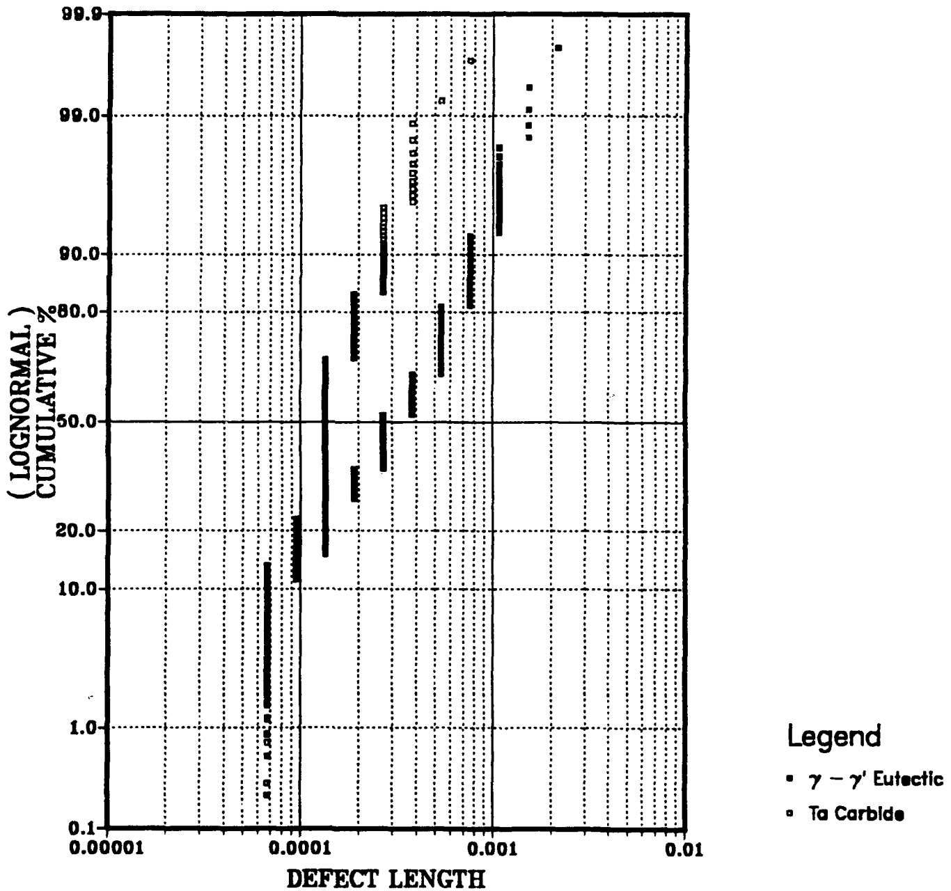
Figure 4: PWA 1484 + HIP \gamma - \gamma' Eutectic vs. Tantalum Carbide Distributions
