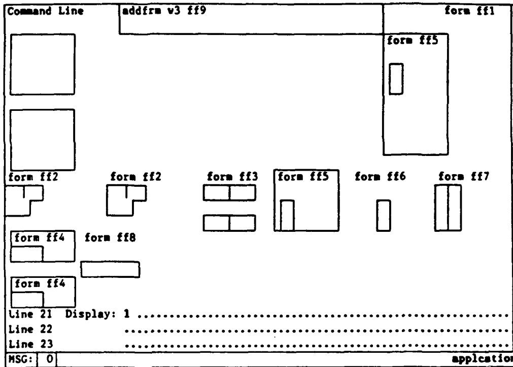
Figure 5-13a Add Form ff9
