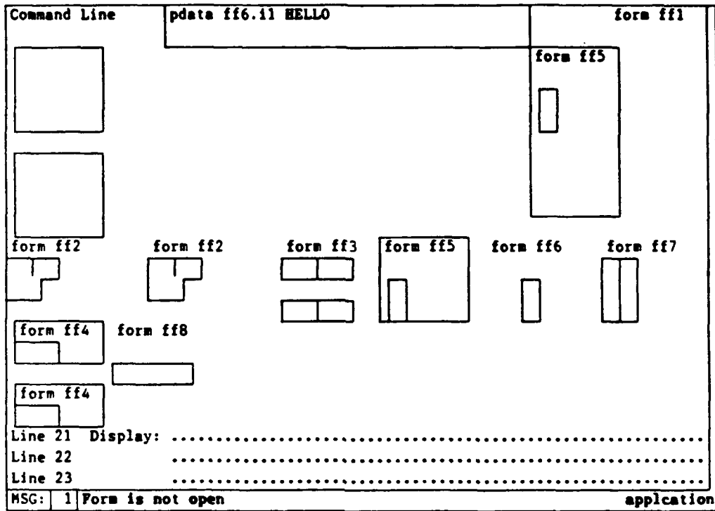
Figure 5-16a Test PDATA
