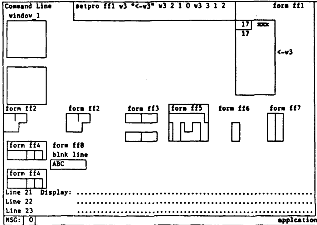
Figure 5-77f Case 3 Result
