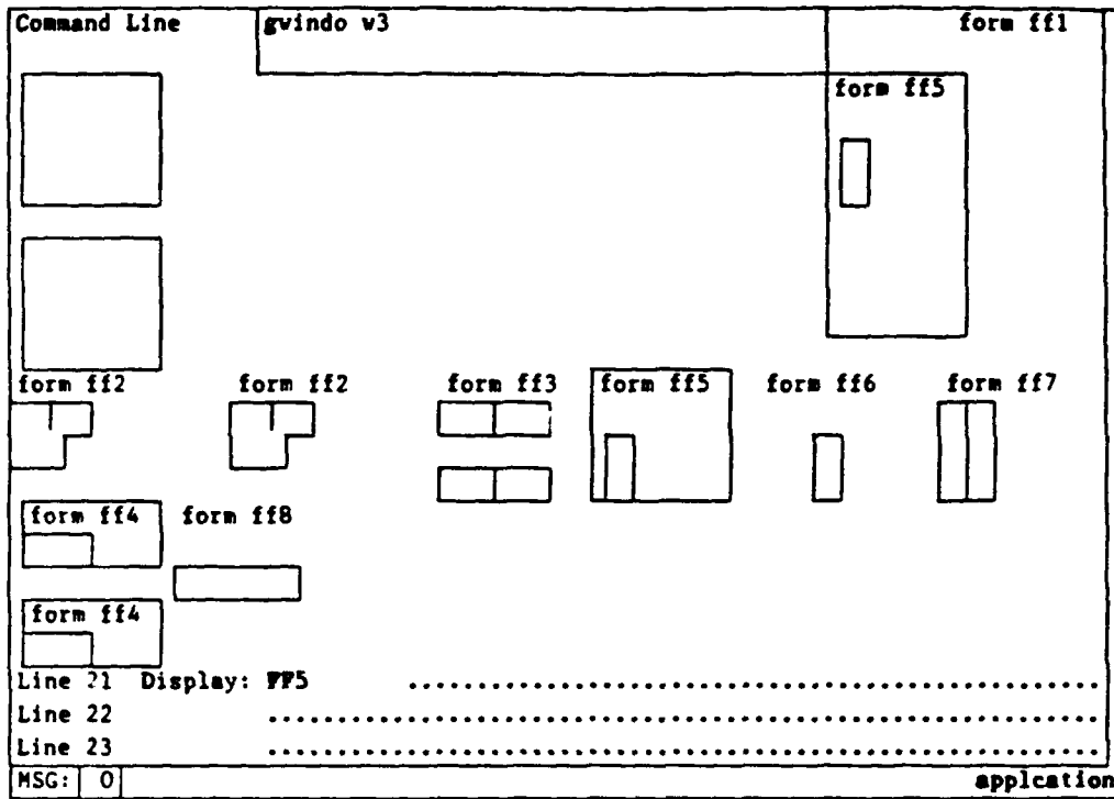
Figure 5-12a Test GWINDO
