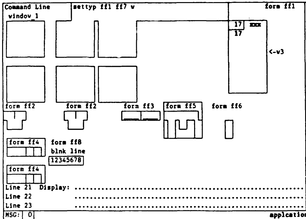
Figure 5-88b Case 3 Result
