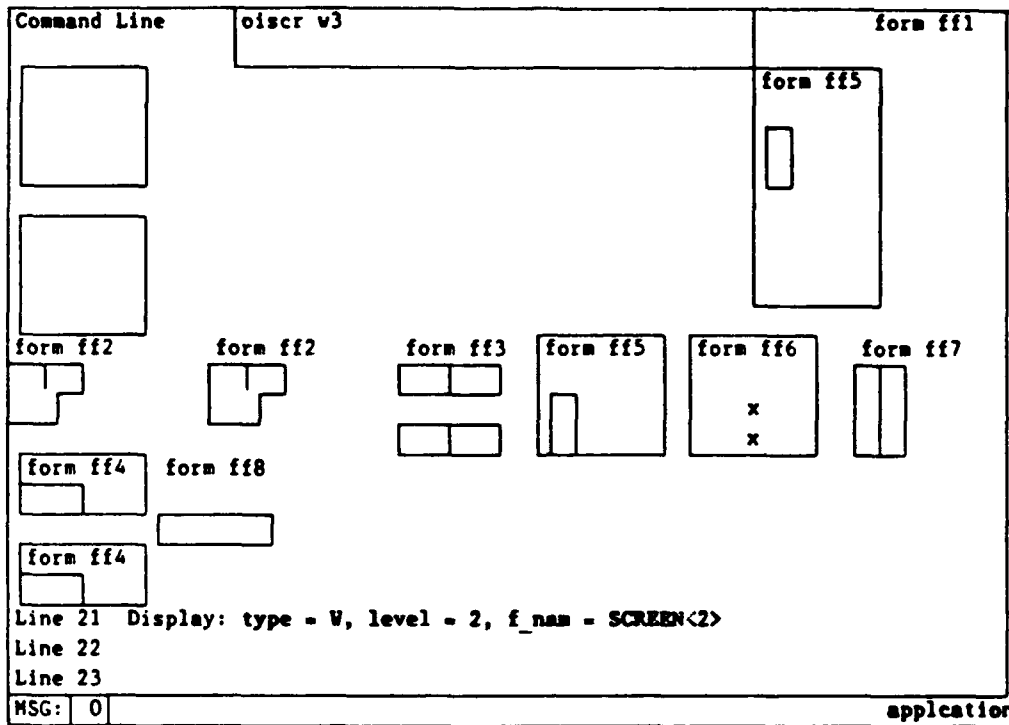
Figure 5-31b Test Screen
