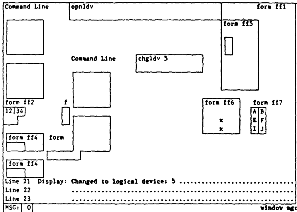
Figure 5-43b Location Result
