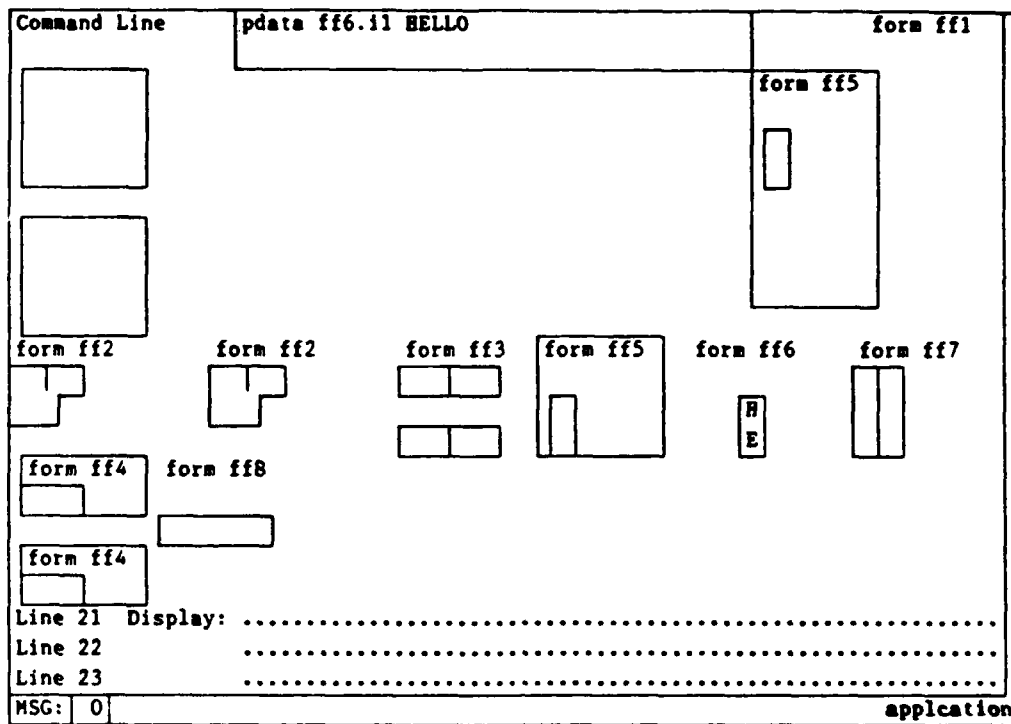
Figure 5-16b PDATA Result
