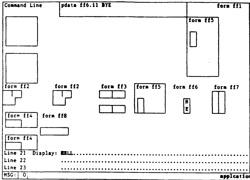
Figure 5-18a PDATA 'BYE'
