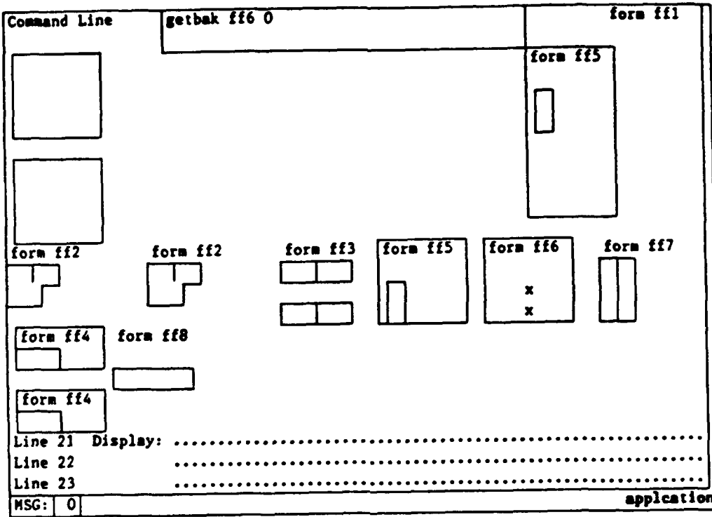
Figure 5-26a Test GETBAK
