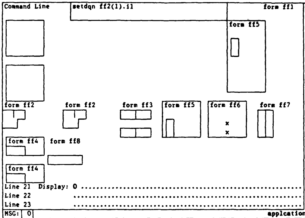
Figure 5-32a Test SETDQN
