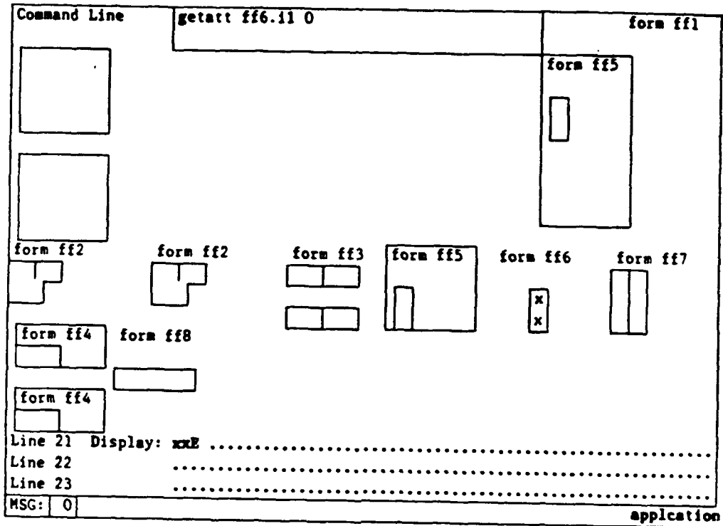
Figure 5-22a Test GETATT
