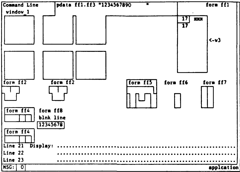
Figure 5-84c Test Verification
