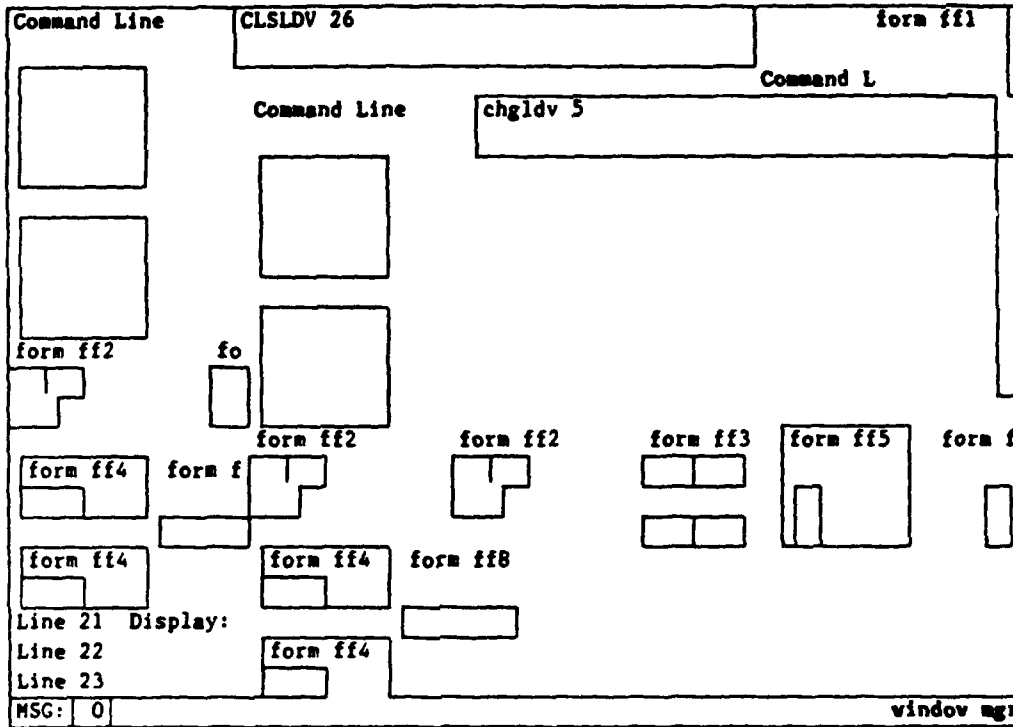
Figure 5-54a Test CLSLDV
