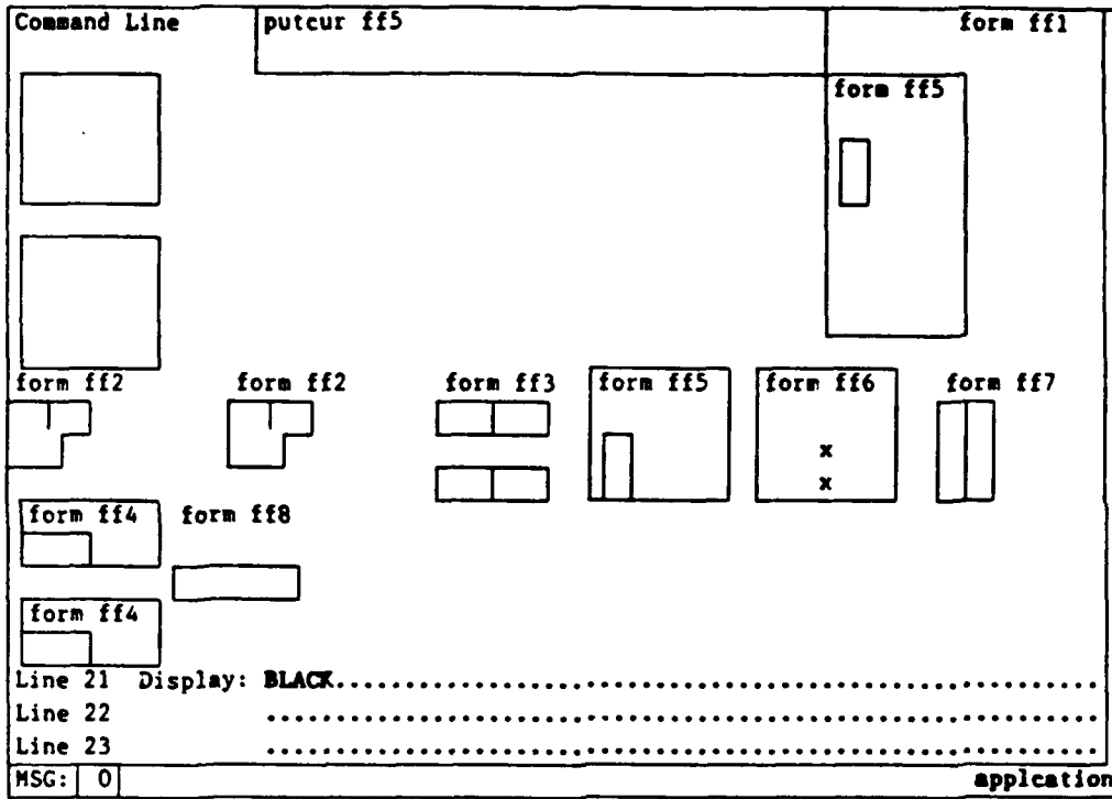
Figure 5-29a Test PUTCUR
