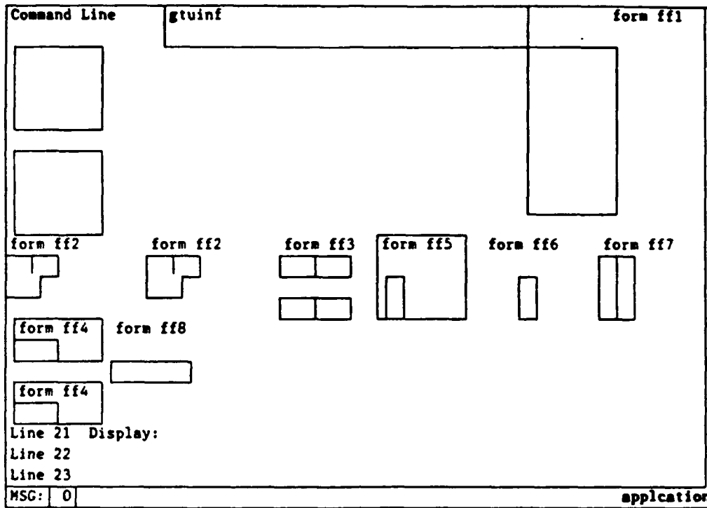
Figure 5-3a Test GTUINF
