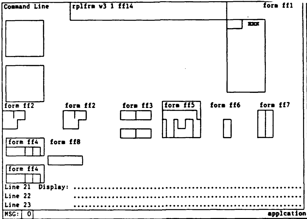
Figure 5-69b RPLFRM Result
