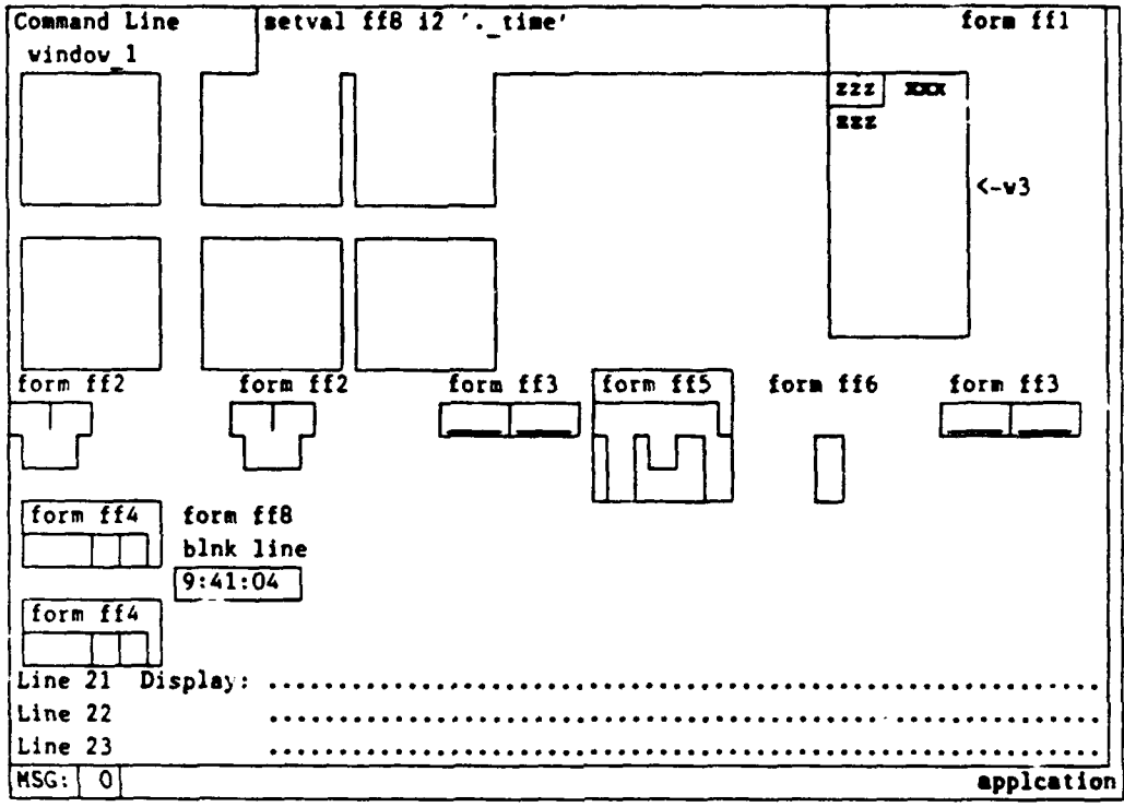
Figure 5-90b Case 2 Result
