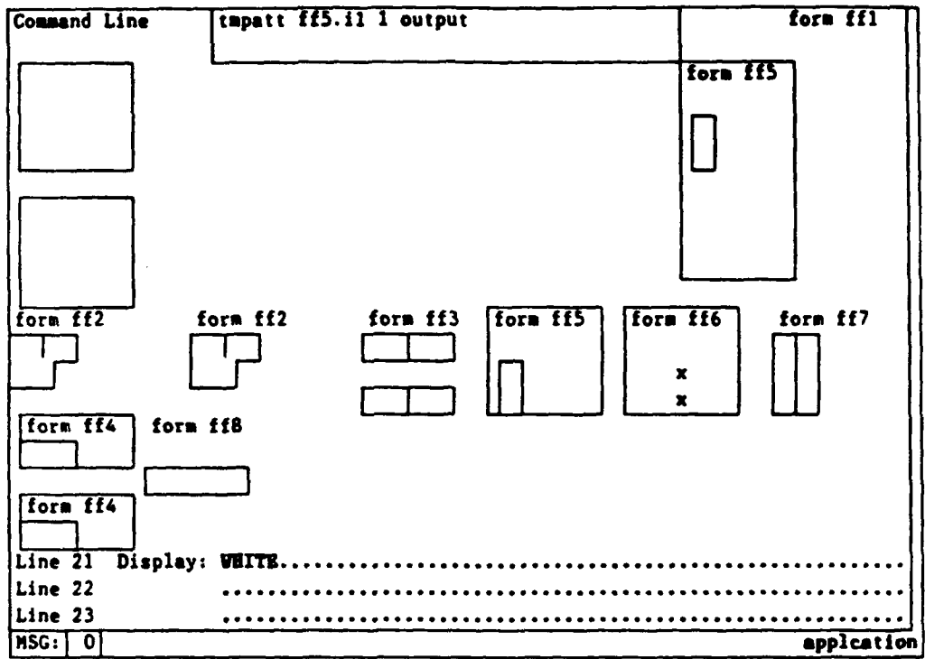
Figure 5-27a Change Attribute
