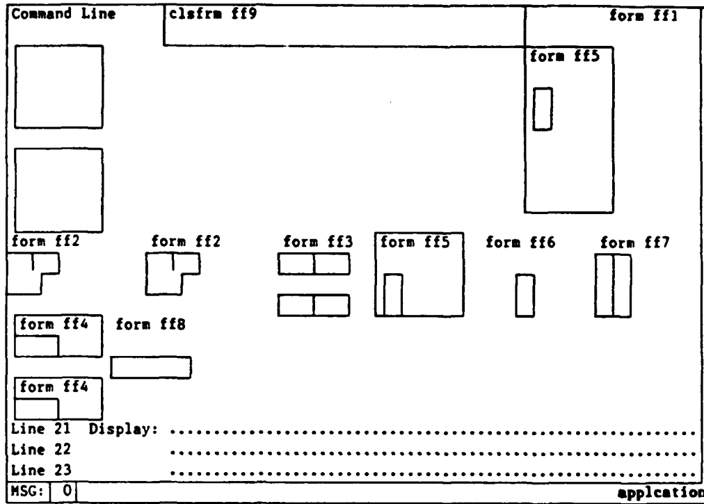
Figure 5-15a Test CLSFRM
