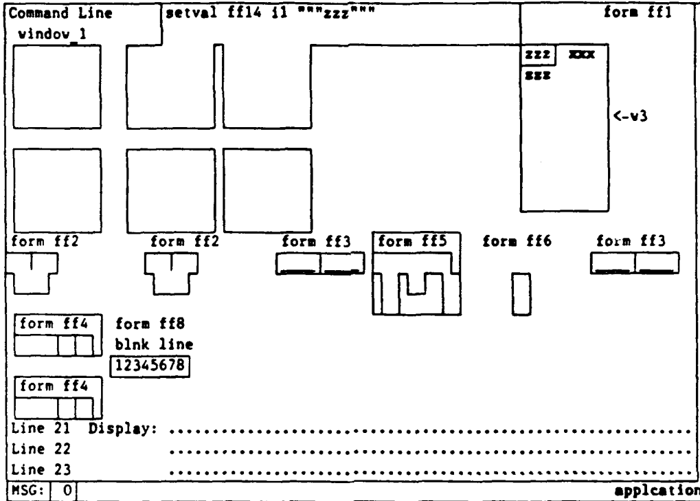
Figure 5-89b Case 1 Result
