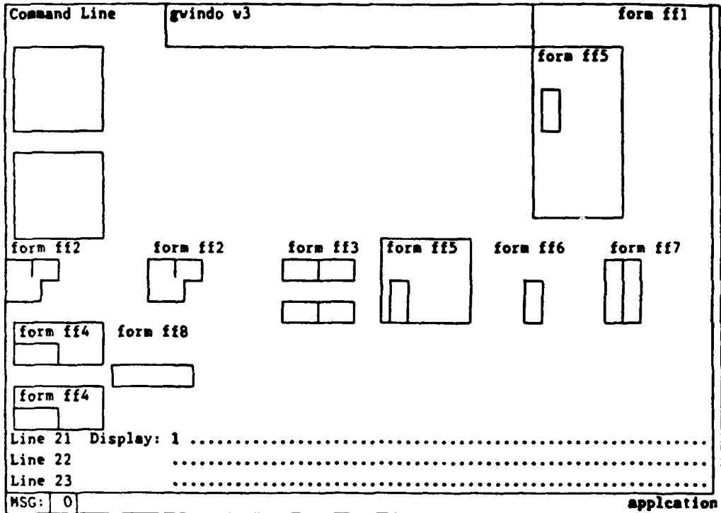
Figure 5-12b GWINDO Result
