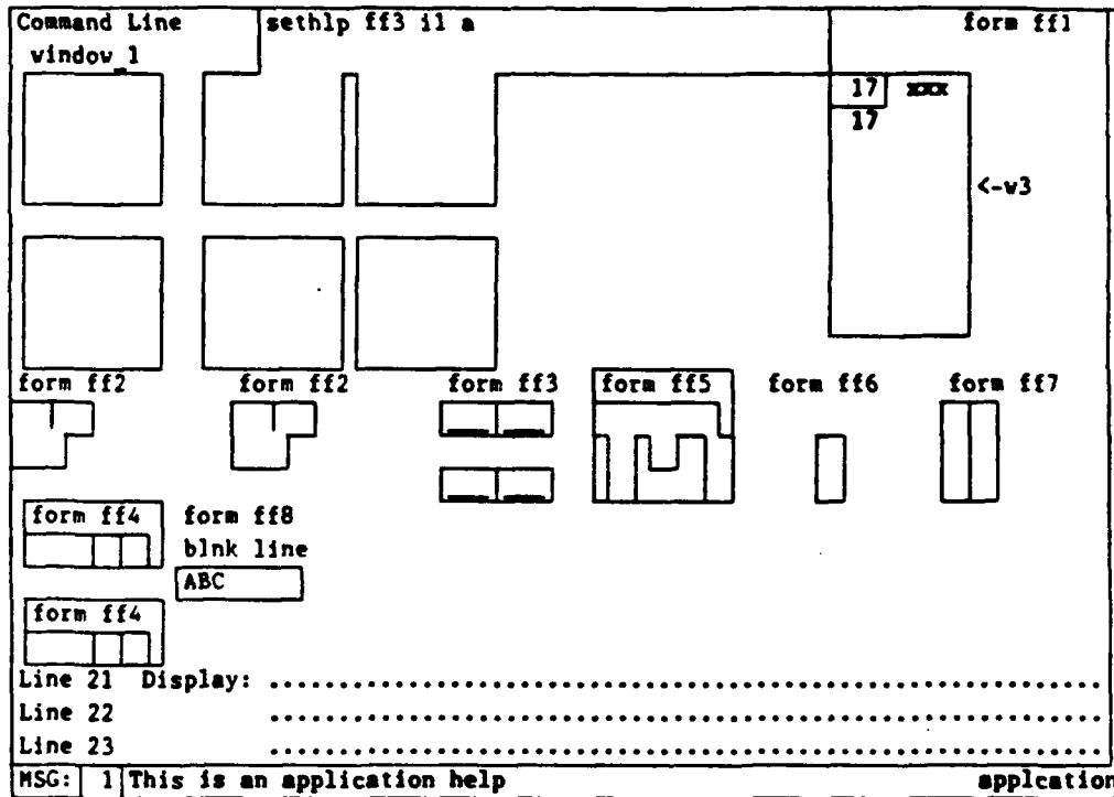
Figure 5-80b Case 1 Result
