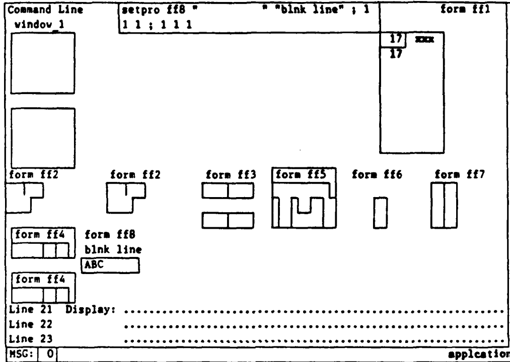
Figure 5-77d Case 2 Result
