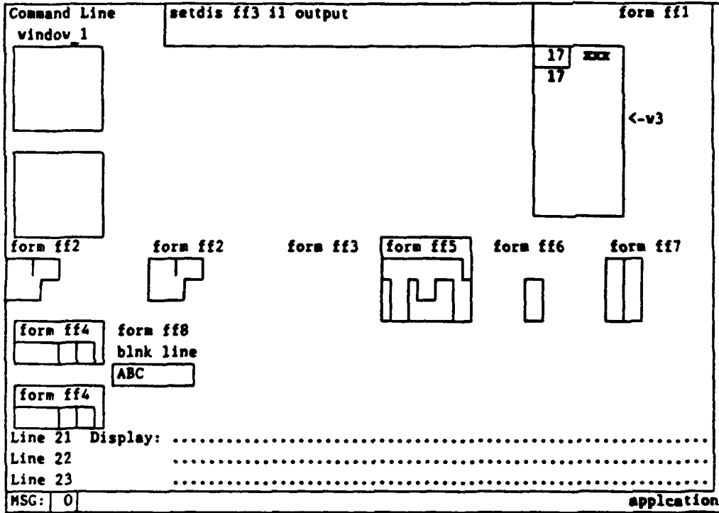
Figure 5-79b Case 1 Result
