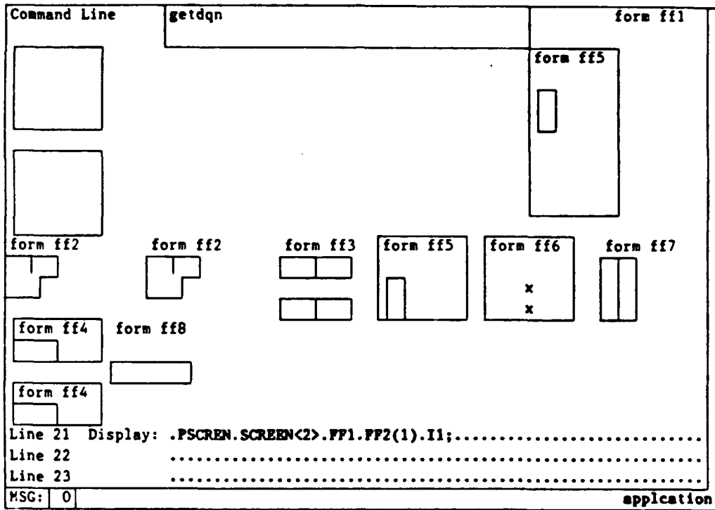
Figure 5-32c GETDQN Result
