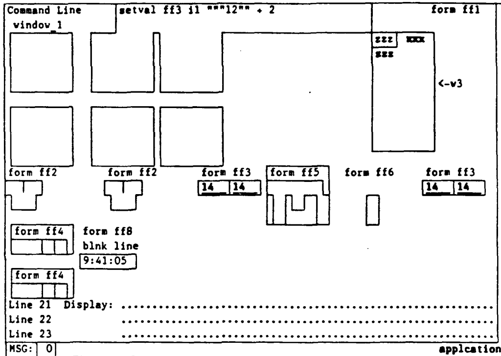
Figure 5-91b Case 3 Result
