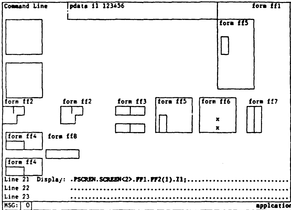
Figure 5-32d Enter Data
