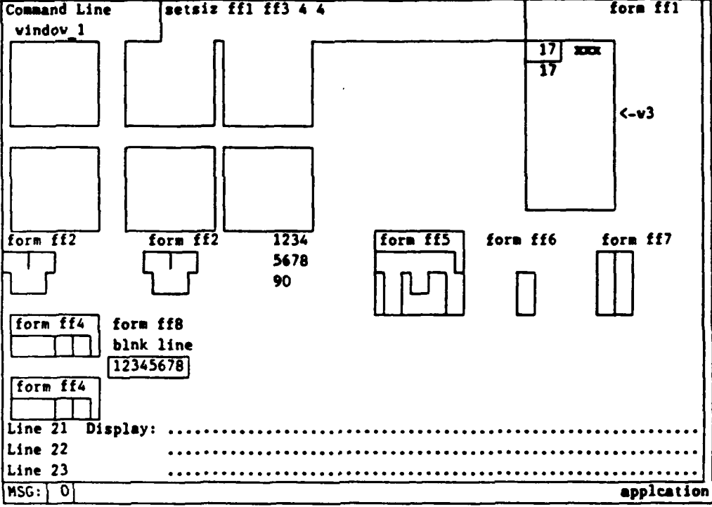
Figure 5-85b Case 1 Result
