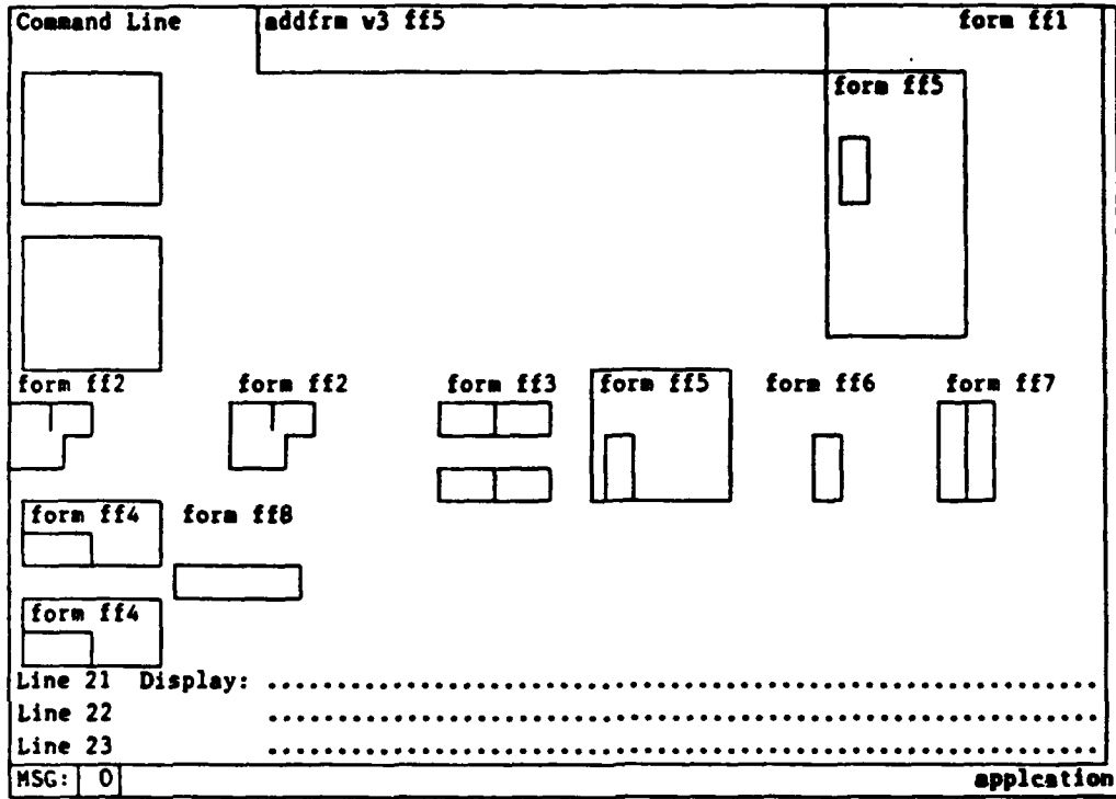
Figure 5-7x New Screen
