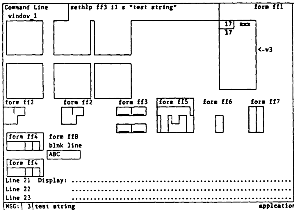
Figure 5-80d Case 2 Result
