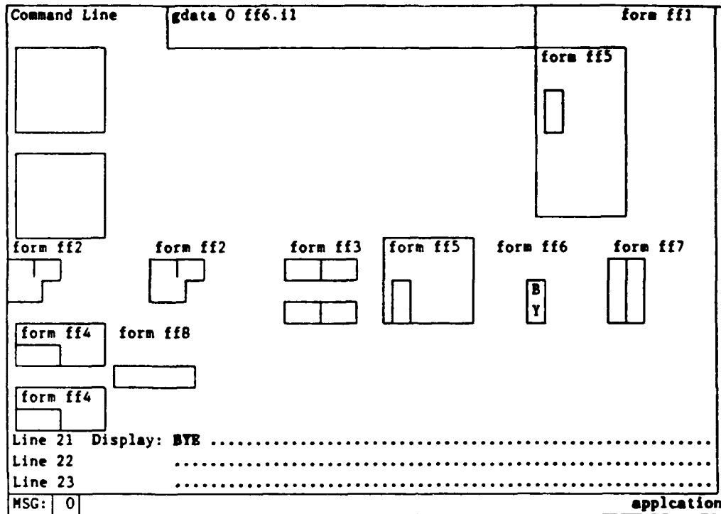
Figure 5-19b GDATA Result
