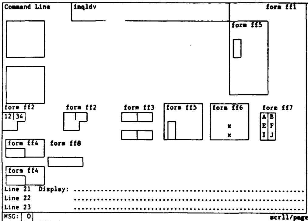
Figure 5-35a Test INQLDV
