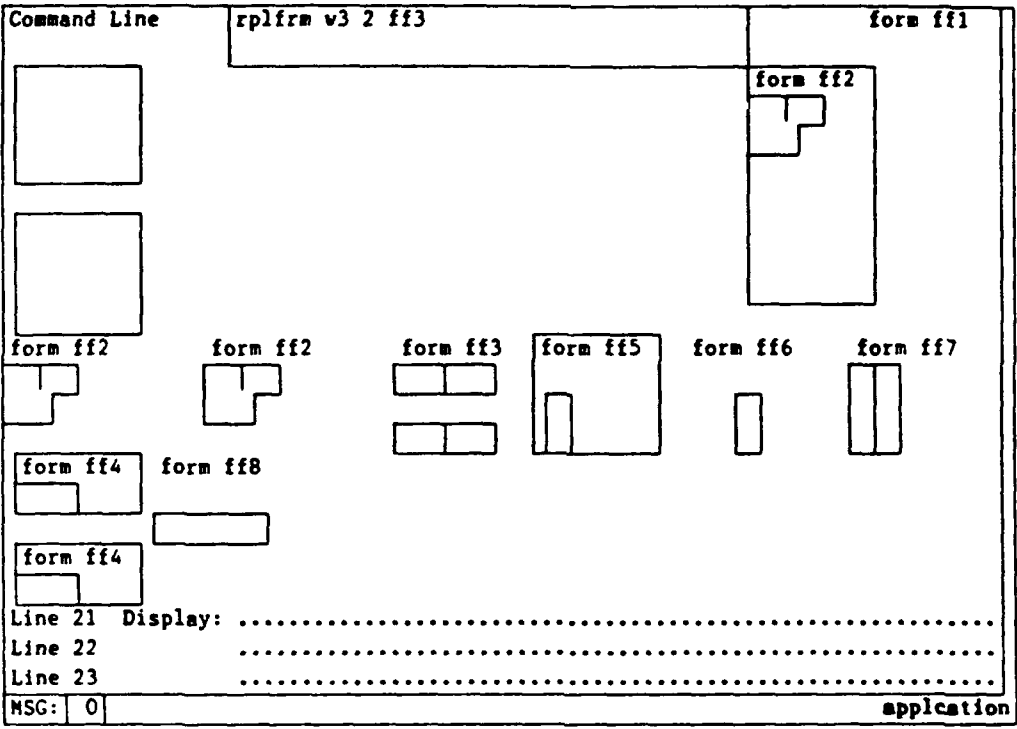
Figure 5-9a Test RPLFRM
