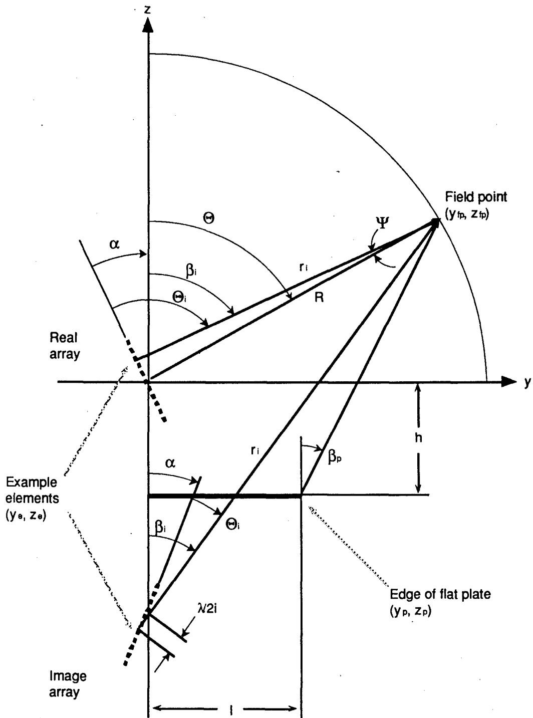
Figure C-4. Computer simulation geometry.
