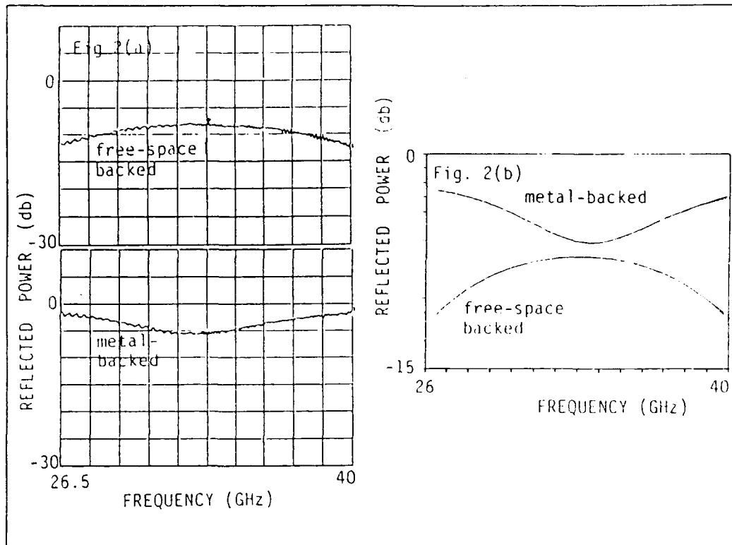
Figure 2. (a) The measured reflectance, open and short circuit, from a poly-pyrrole-treated, 5000 ohms/square DC resistance, polyester resin composite at \theta_i = 16^\circ , (b) the best fit to the measured data assuming \epsilon' = 2.7 and \sigma = 0.004 .
