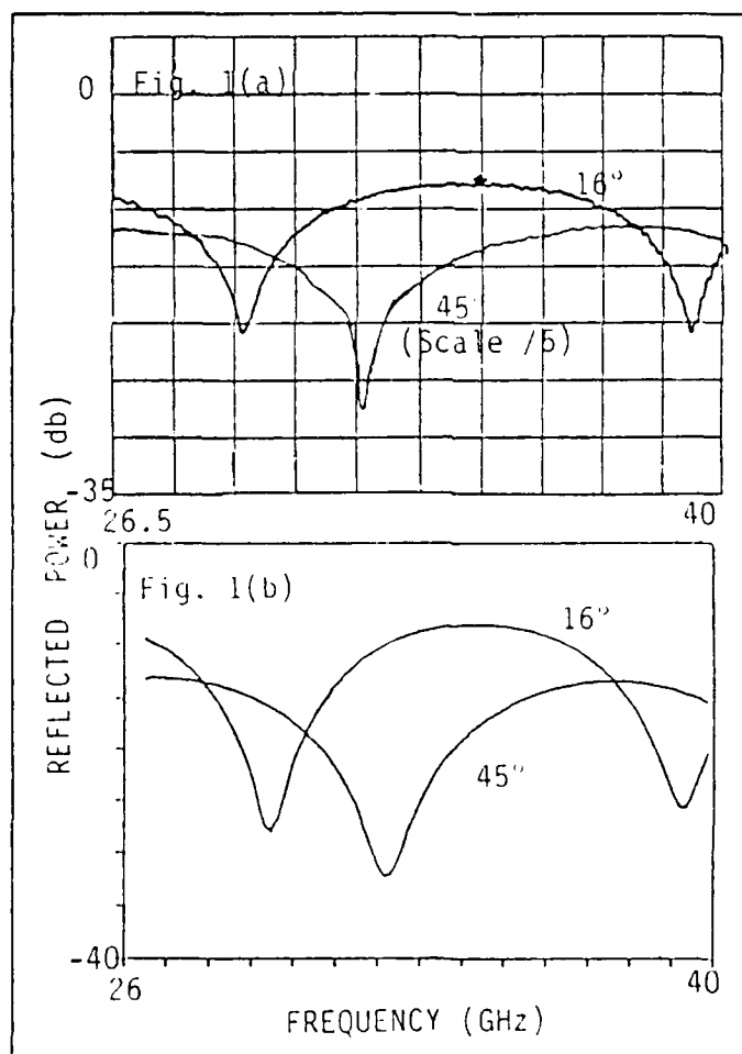
Figure 1. (a) The measured reflectance from untreated polyester/polyester composite from 26.5 GHz to 40 GHz, (b) the best fit to the above data using \epsilon' = 2.65 and \epsilon'' = 0.05 .
