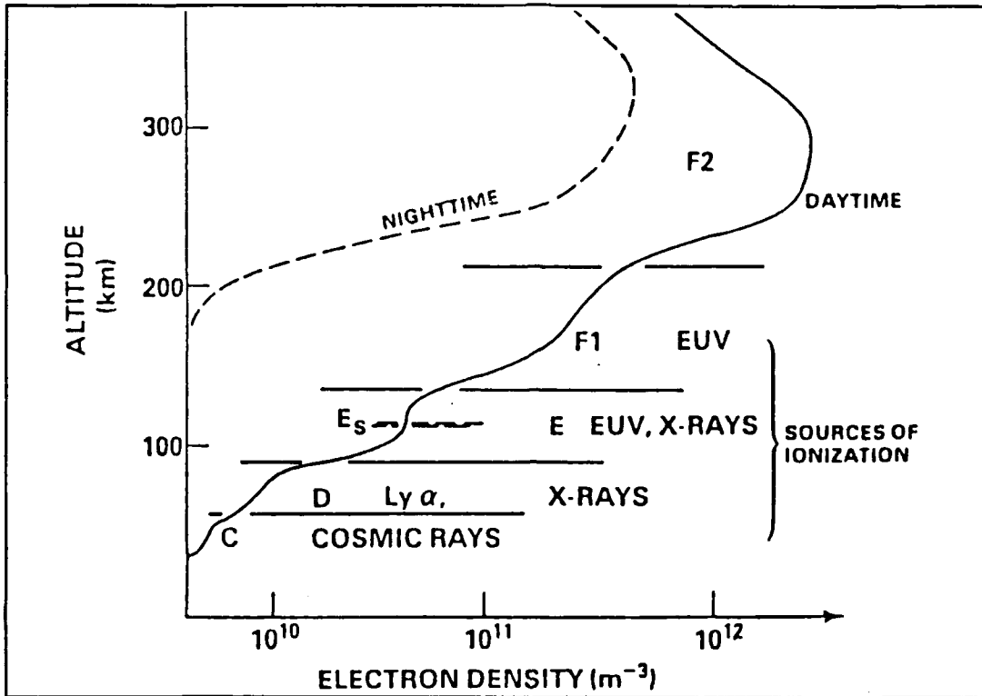
Figure 14. Ionospheric Layers
