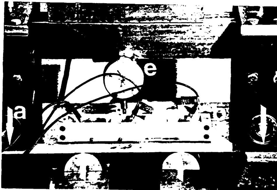
B. Above, Details of plate loading and ultrasonic velocity measurement module.
