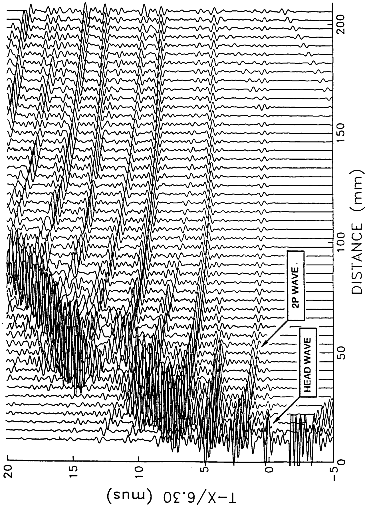
Figure 3. Seismogram style plot for Al-6061-T651 plate waves in a 0.050" thick plate.
