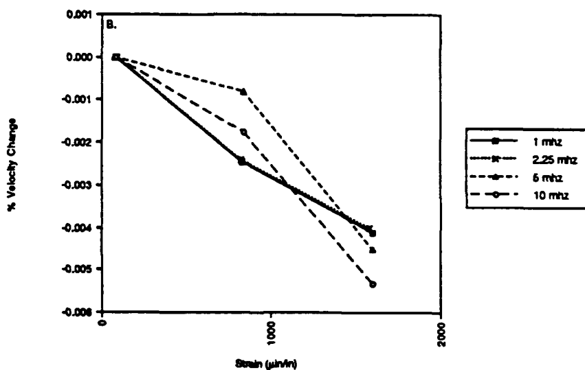
4340 - Tension Test
