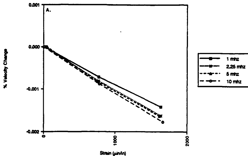
Al-6061-T651 - Tension Test
