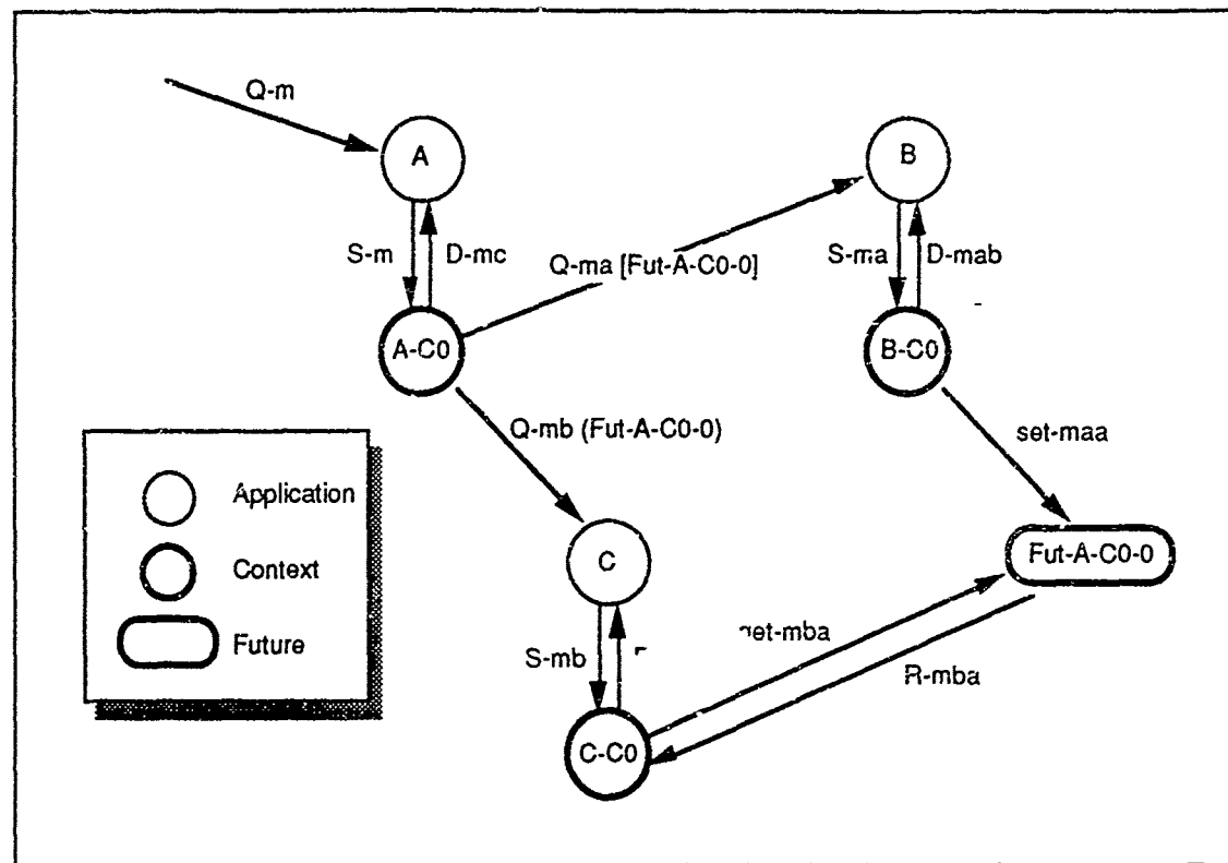
Figure 4. Method Execution
