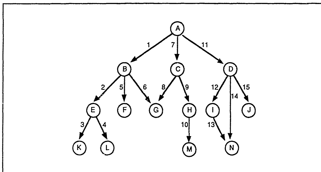
Figure 1. Serial Execution
