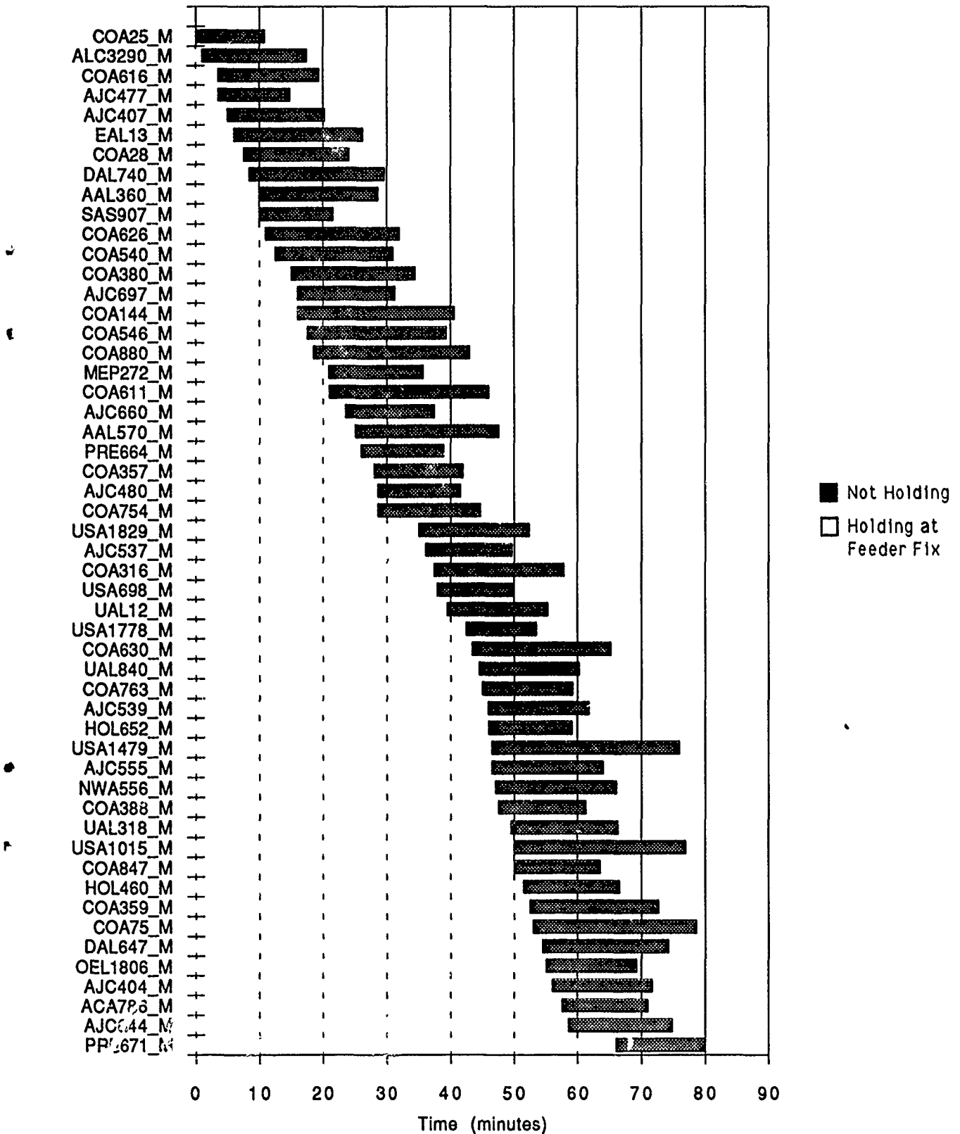
Figure D-31b. Arrival Aircraft Holding and In-flight Time Lines
