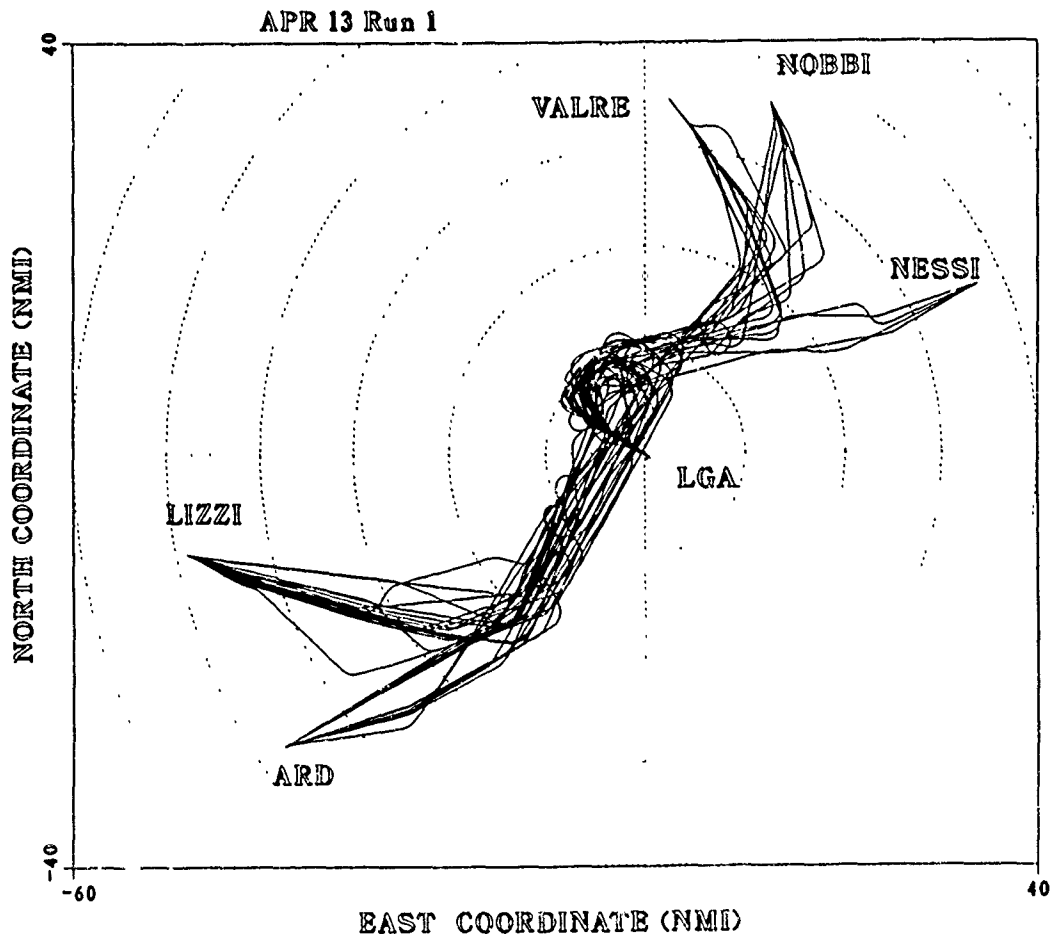
Figure D-4a. Summary Data & Arrival Aircraft Flight Tracks for No.4 D-8
