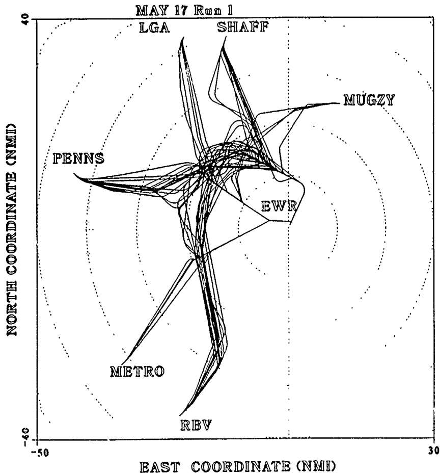
Figure D-30a. Summary Data & Arrival Aircraft Flight Tracks for No.30 D - 60
