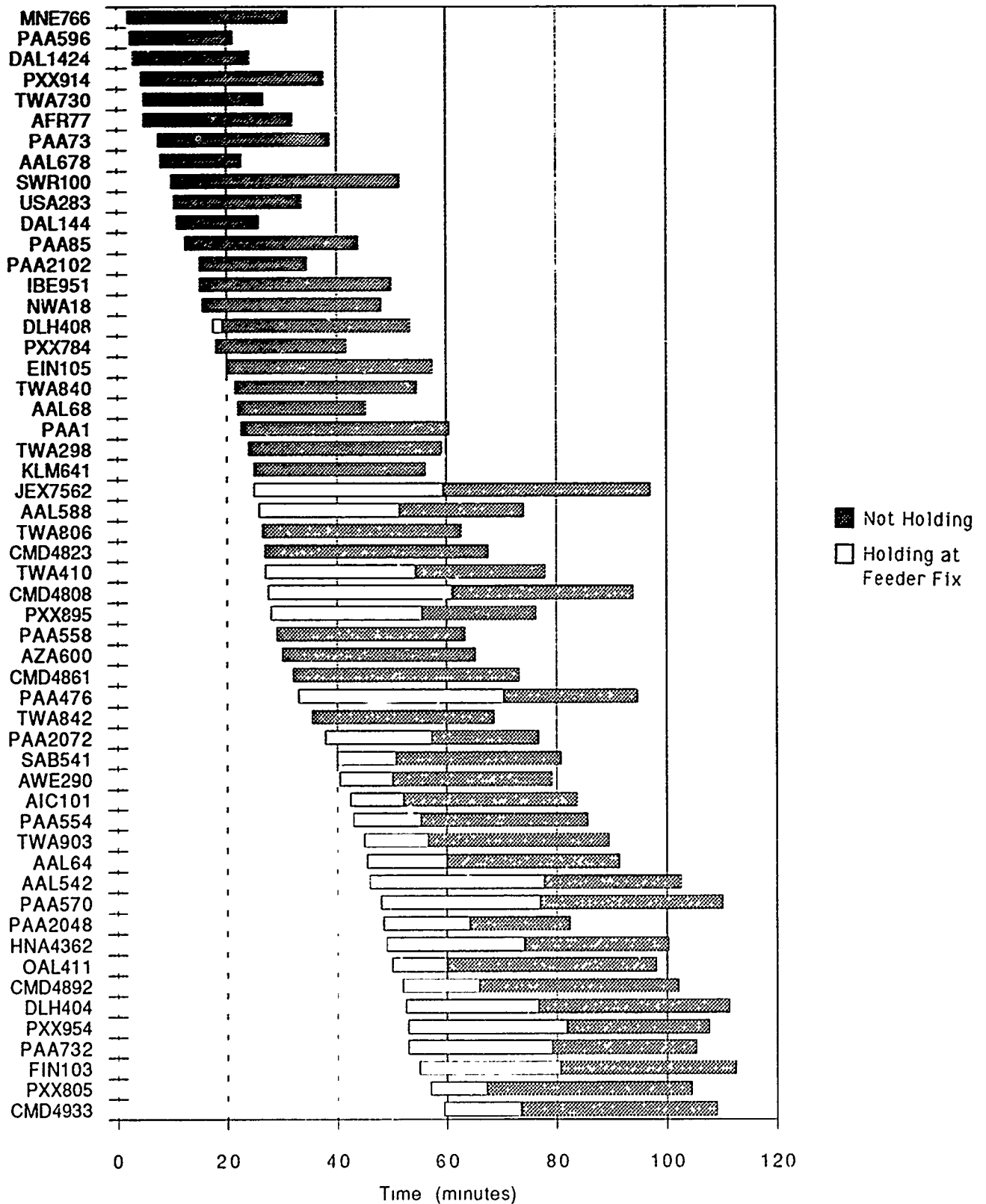
Figure D-12b. Arrival Aircraft Holding and In-flight Time Lines
