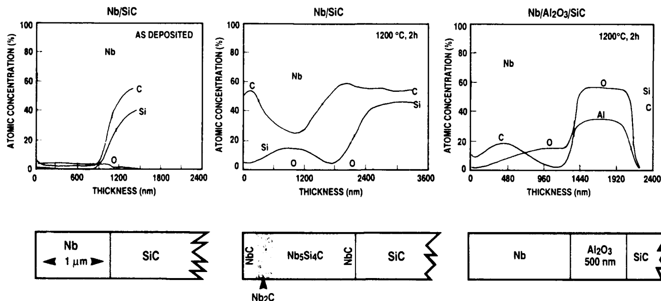
Figure 1. Diffusion barriers in high-temperature metal matrix composites.
