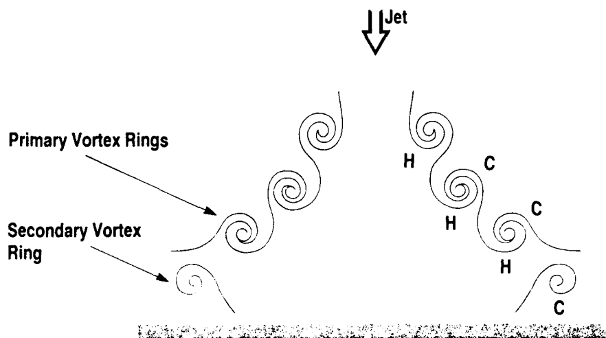
Figure 2. Total temperature separation in an impinging jet.
