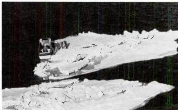
Figure 4-6 Ice floes.
