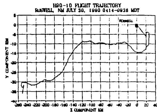
Figure 12. Flight H90-10 was launched from Roswell, NM at 0414 MDT. Note the strong backing in the trajectory at -120 kilometers.
