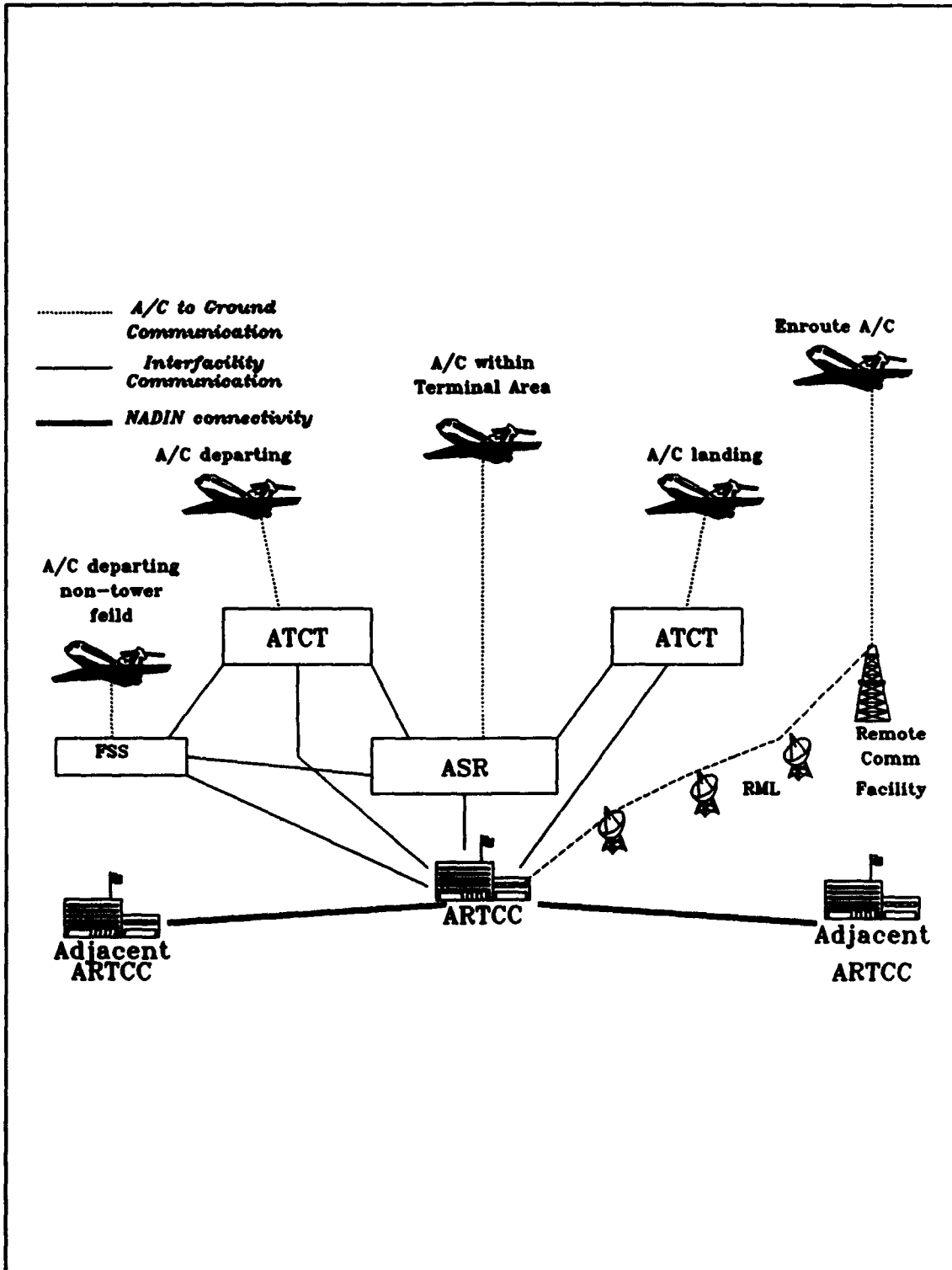
Figure 2 NAS COMMUNICATION CONNECTIVITY
