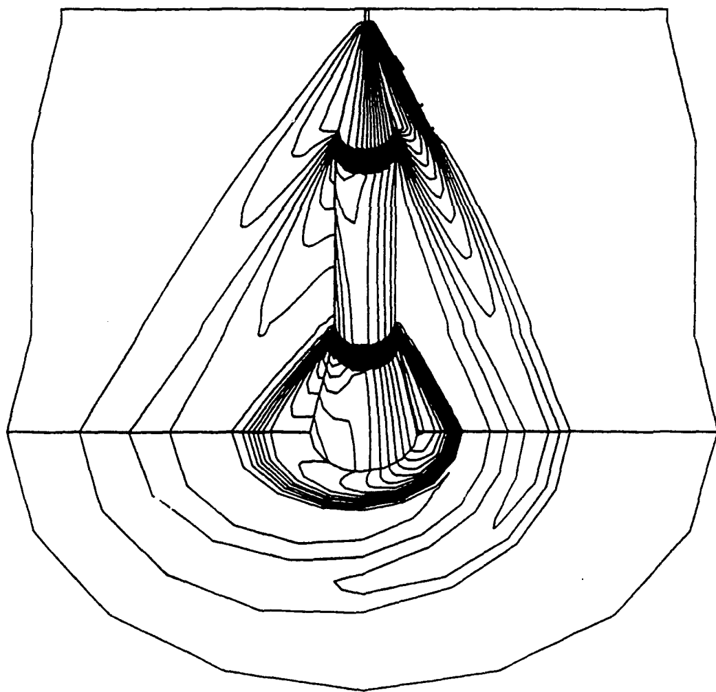
Figure 3a. Cone-Cylinder-10° Flare, M_\infty = 3, \alpha = 5^\circ, (38 \times 41 \times 9) : Three dimensional view of C_p contours.
