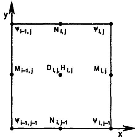
Figure 3. Positions of variables in the finite-difference grid of the lake circulation model. (After Schwab et al. 1981.)
