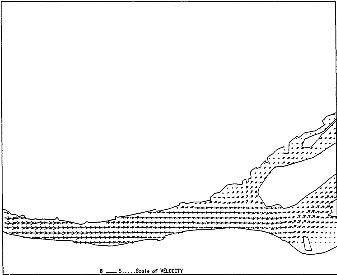
d. Third section. Figure D2 (cont'd).
