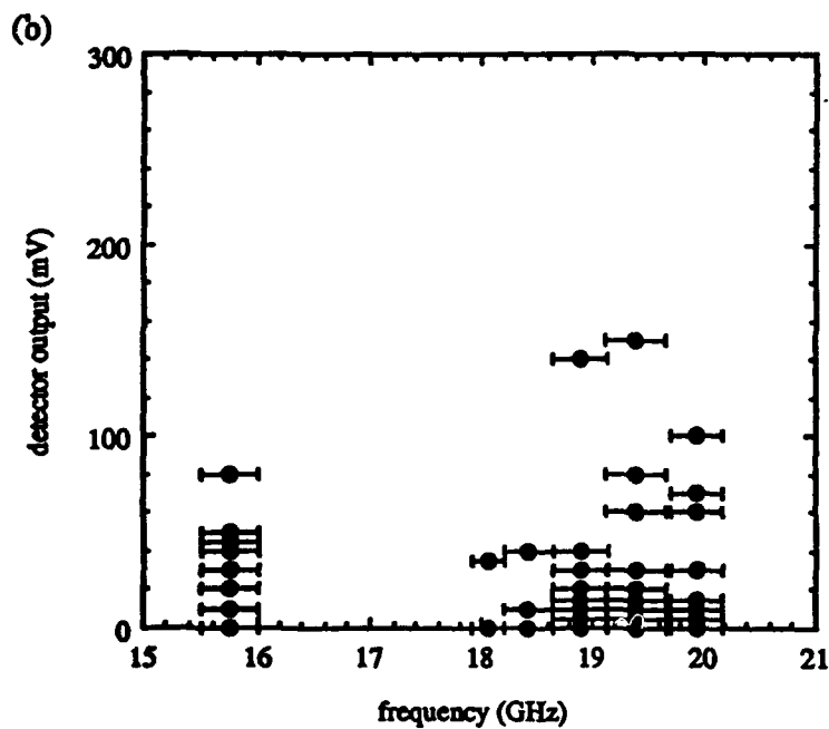
Figure 8. Data of frequency measurements for the case of (a) Bragg resonator BRFO and (b) small diameter ( r_w = 1.64 cm) smooth tube without Bragg reflectors.
