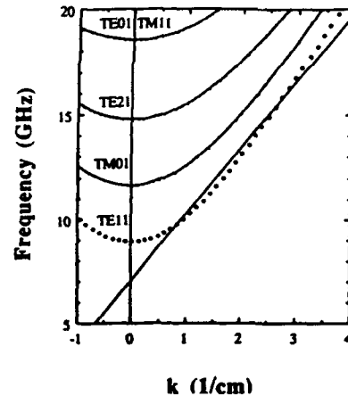
Fig. 1. Uncoupled dispersion relations of electron-beam cyclotron wave and cavity-waveguide modes for experiments; parameters are: B_0 = 4.34 kG, V_e = 370 kV, and \alpha = v_{\perp}/v_{\parallel} = 0.72 .
