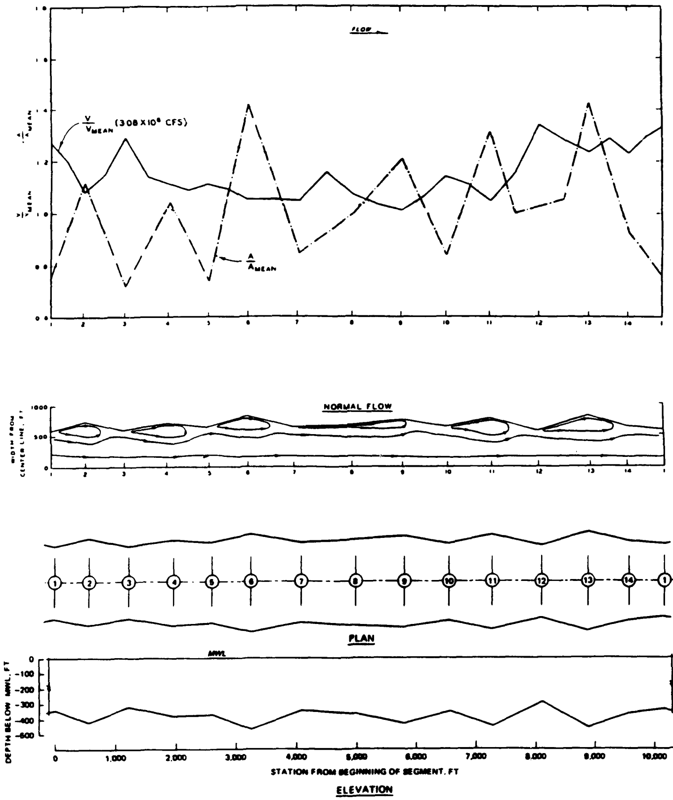
Figure 3. Flow in a highly irregular channel
