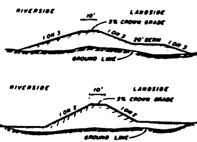
TYPICAL LEVEE SECTIONS
