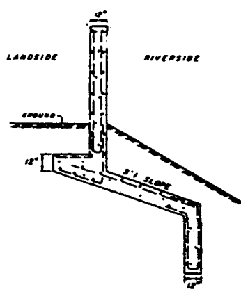
TYPICAL FLOOD WALL SECTION
