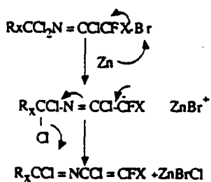
Scheme 3.
