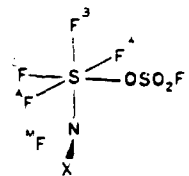
Figure 1. Generalized structure of one enantiomer of the addition products derived from F_4S=NF ( X = \text{Cl, Br, OSO}_2\text{F} ).
