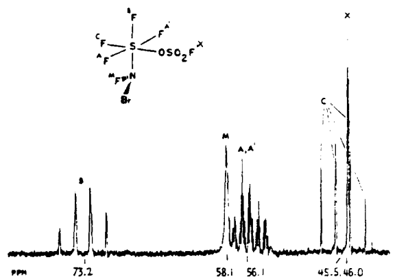
Figure 3. ^{19}\text{F} NMR (94.1 MHz) spectrum of cis - \text{SF}_4(\text{OSO}_2\text{F})\text{NBrF} at -51^\circ\text{C} and 5000-Hz sweep width.
