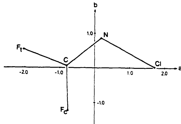
FIG. 1. The coordinates of \text{CF}_2 = {}^{14}\text{N}^{35}\text{Cl} in its principal inertial axis system. The structure is the r_2 structure with r(\text{N}-\text{Cl}) = 1.745 \text{ \AA} .
