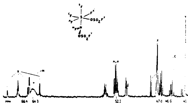
Figure 4. ^{19}\text{F} NMR (94.1 MHz) spectrum of cis - \text{SF}_4(\text{OSO}_2\text{F})\text{NF}(\text{OSO}_2\text{F}) at 30^\circ\text{C} and 2500-Hz sweep width.
