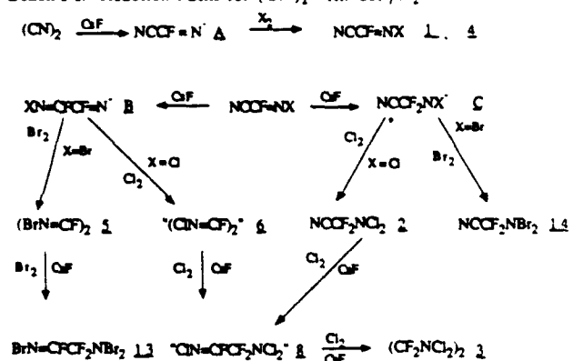
Scheme 1. Reaction Paths for (\text{CN})_2 with \text{CsF}/\text{X}_2
