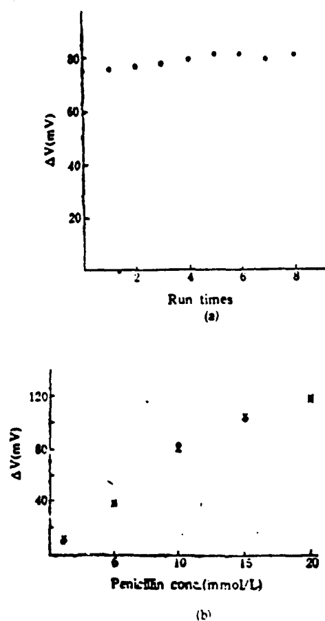
Fig.6 Reproductivity of response of penicillin-ENFET to penicillin
