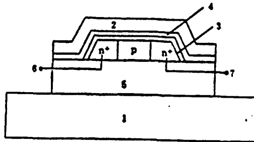
Fig. 2 Cross section diagram of the chip of penicillin-ENFET probe
