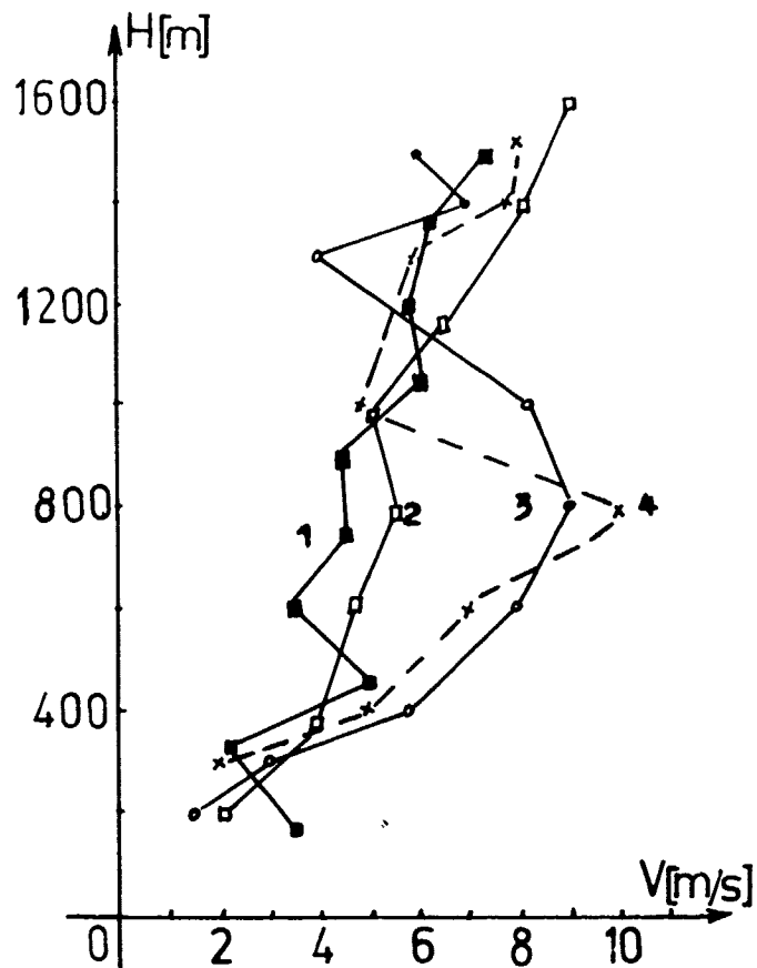
FIG.3 A comparison of lidar (2,3) and pilot balloon (1), radar-tracked pilot balloon (4) wind measurements.
