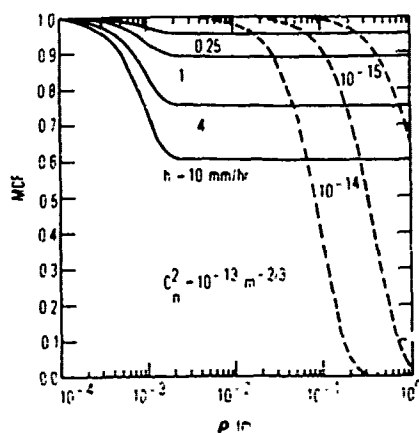
Fig. 2: The mutual coherence function at 10.6 \mu m for a path of 1200 m and various rain rates h (solid curves). Dashed curves: Clear air turbulence, different values of the index structure constant C_n .
