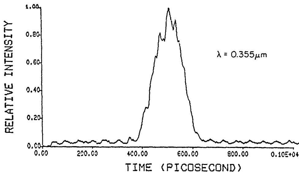
Figure 2. Average waveform of 50 pulses reflected from the tilted CCR array target described in Figure 1. The structure within the average pulse is due to the range spread of the target and corresponds to reflections from individual CCR's within the array.
