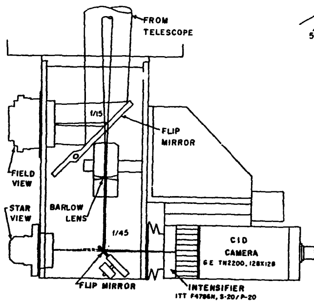
Figure 3. Seeing monitor camera optical layout.
