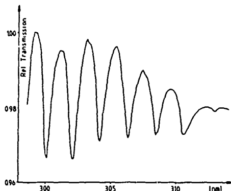
Fig.5. Doas monitoring of ambient \text{SO}_2 over a 600 m urban pathlength (MV: 22 ppb [10]).
