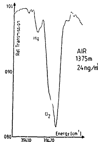
Fig.6. Doas recordings of Hg in air [11].
