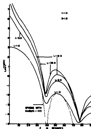
Fig. 2. The natural logarithm of the form factor averaged over all orientations of a fiber is plotted versus the scattering angle for fixed fiber diameter D and for various fiber lengths L .
