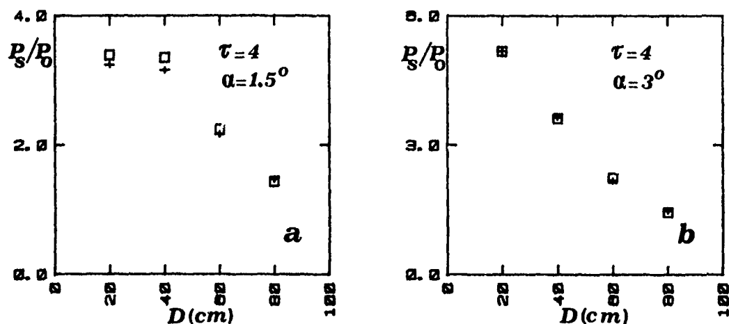
Fig. 2 - Ratio P_s/P_0 plotted versus D . Crosses: measured ratios. Squares: calculated ratios. Spheres with average radius 7.85 \mu\text{m} . a: \alpha = 1.5^\circ , b: \alpha = 3^\circ .
