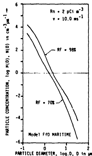
Fig.3: Dynamic of the FFO-MARITIME Aerosol Model size distribution with increasing relative humidity
