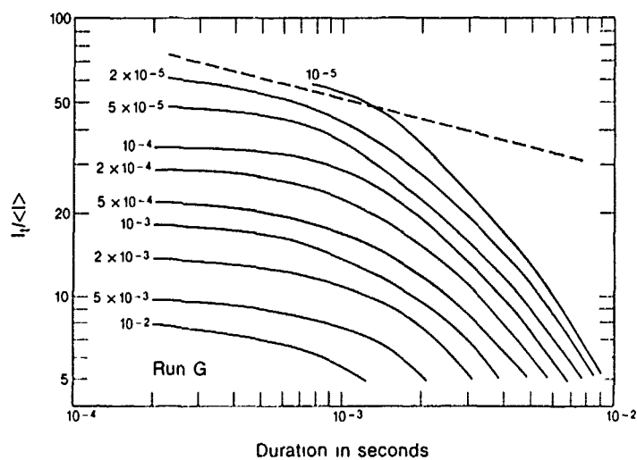
Figure 2. Contours of the joint probability distribution of \tau > \tau_e and I > I_e . The dashed line has the -1/4 slope of the exposure limit.
