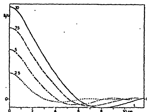
Figure 1 : Theoretical spatial covariance of stellar shadow patterns in arbitrary scale, assuming a thin turbulent layer at the altitude indicated in km on each curve (2.5, 5, 7.5 and 10 km). The integral \int \Delta h \cdot C_N^2(h) over the layer thickness is assumed to be the same in each case
