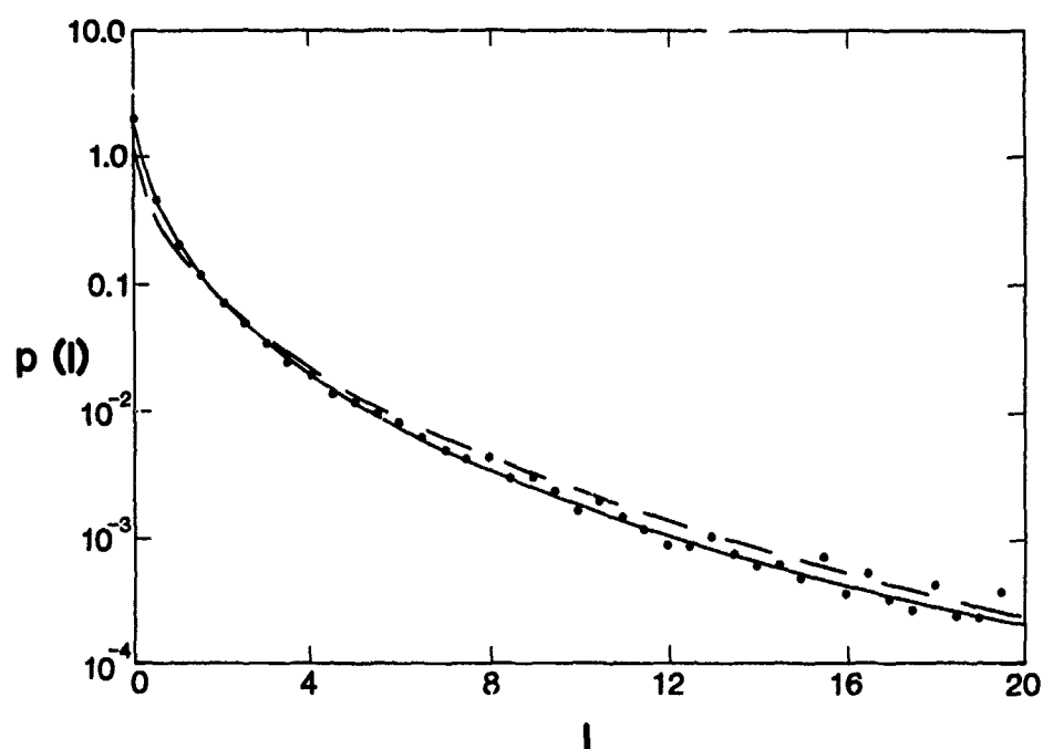
Figure 1. Plot of probability density function vs. intensity for K (dashed line) and lognormal-exponential (solid line) models along with experimental values (points).
