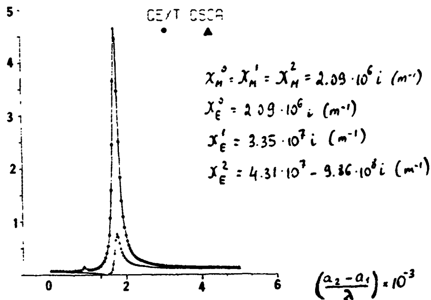
Fig. 1. The extinction and scattering efficiencies as a function of the coated layer relative depth.
