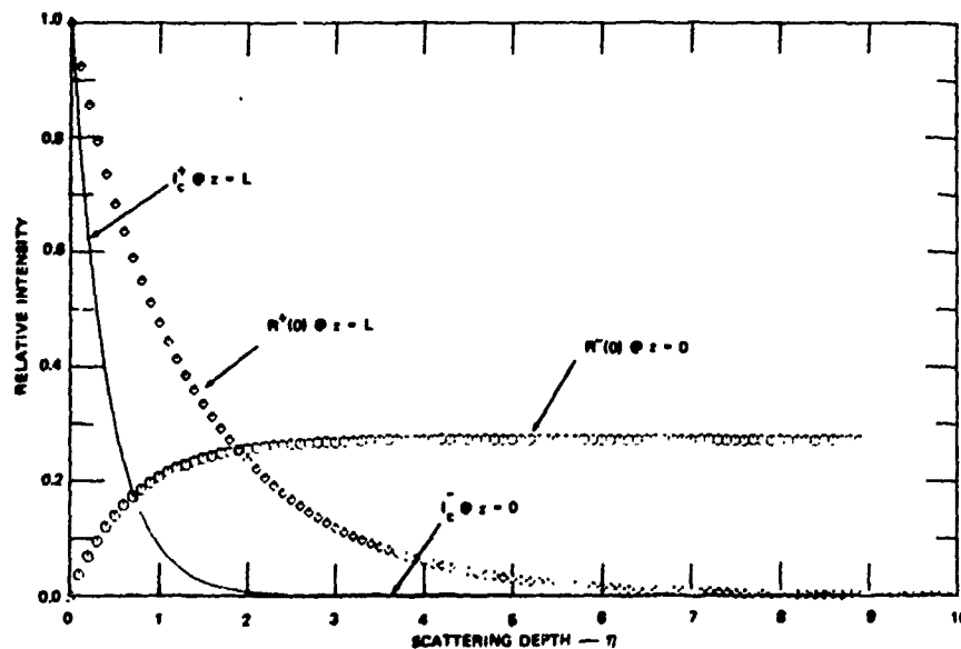
FIGURE 4 SAME PLOT AS FIGURE 3, BUT FOR ABSORBING SPHERES ( \epsilon = 4.0 - i0.01 )
