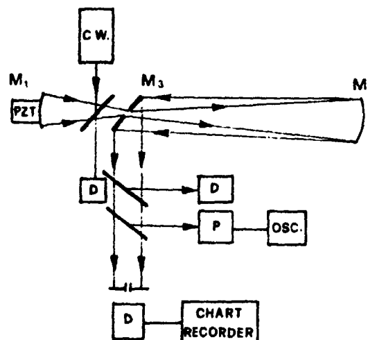
Fig. 2 - The CO 2 SFUR resonator: M 1 , M 2 , M 3 are mirrors; D = pyroelectric detector; P = photon drag detector; C.W. = CO 2 injection laser; PZT = piezo-transducer.
