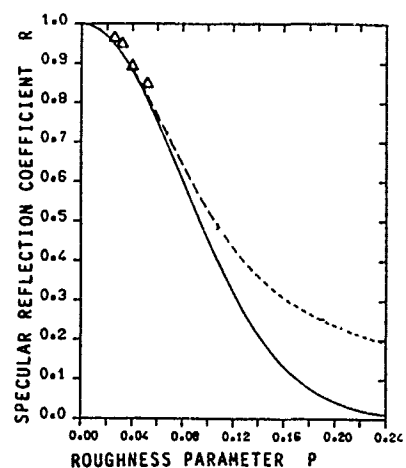
Fig. 3.3: Dependence of the Specular Scattering Coefficient on the Roughness Parameter
