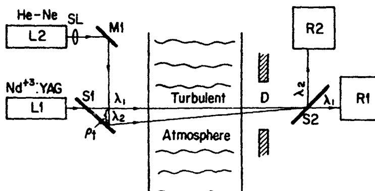
Fig. 1 - Experimental setup. L1, L2, lasers; SL - beam forming lens; M1, plane mirror; S1, S2 dichroic beam splitters; D, variable circular aperture; R1, R2 receivers.
