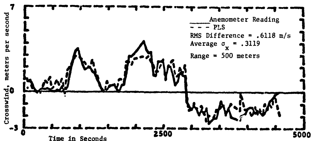
Figure 1. Wind measurement, pulsed laser system.
