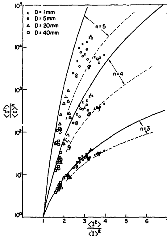
FIG. 2. Measured values of the aperture averaged normalized third, fourth, and fifth moments are compared with the values predicted by the various model distributions, having the same normalized second moments as the experimental data. The continuous lines indicate the moments expected from log-normally distributed intensity fluctuations and apply to all values of normalized second moment. The dashed lines indicate moments expected from K-distributed fluctuations and apply to values of the normalized second moment greater than 2.
