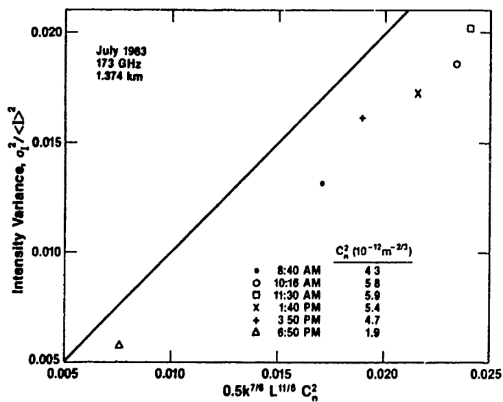
Figure 6.—The normalized variance of intensity versus its inertial-range formula. The straight line shows theoretical calculations.
