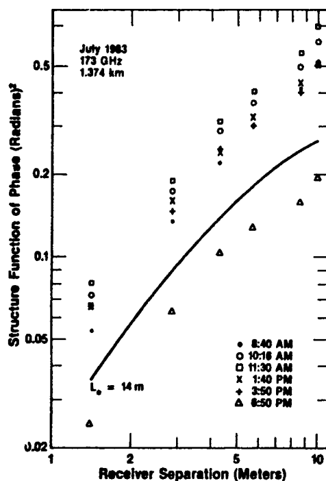
Figure 4.—The structure function of phase. The solid line represents a theoretical prediction for the 6:50 p.m. data
