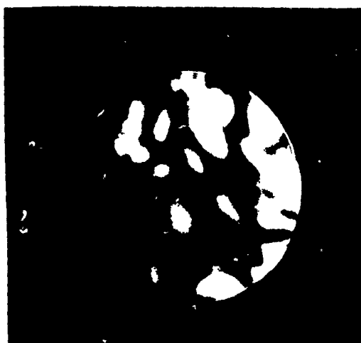
Figure 1. Intensity-scintillation pattern of a 0.63- \mu m spherical wave 1012 m from its source. The pattern is 50 mm in diameter, the exposure is 1/2000 s with winds less than 1 m/s, and C_n^2 = 3 \times 10^{-13} .
