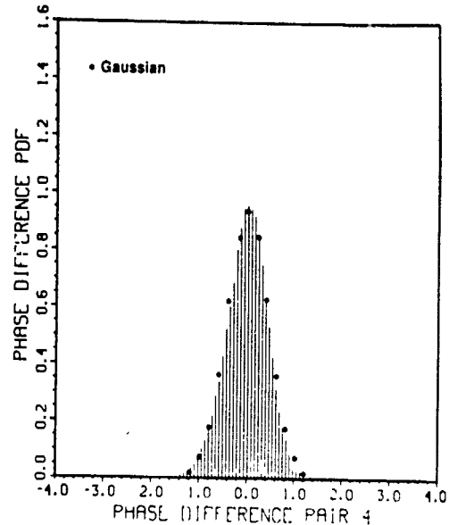
Figure 3.--Probability distribution of phase difference in radians
