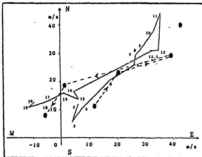
Figure 2 : Hodograph of Nimes : full-line ; the small numbers along the full-line represent the altitude scale.
