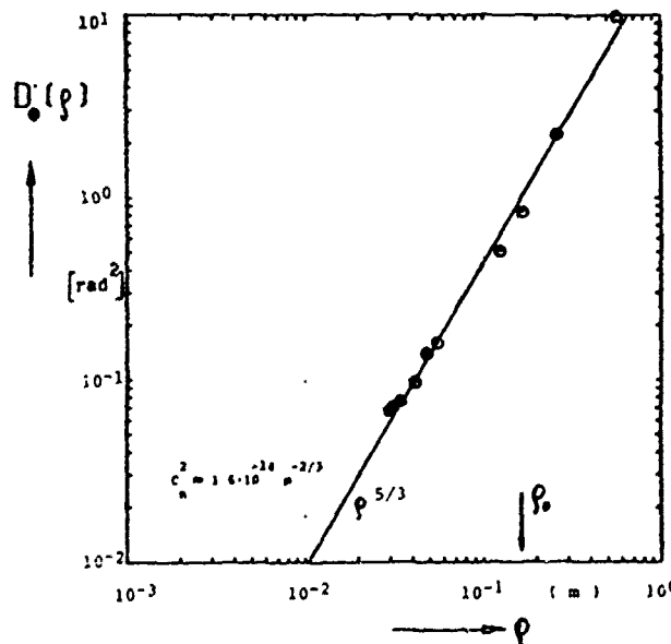
Fig. 1: Phase difference fluctuations between two points of separation \rho due to turbulence.
