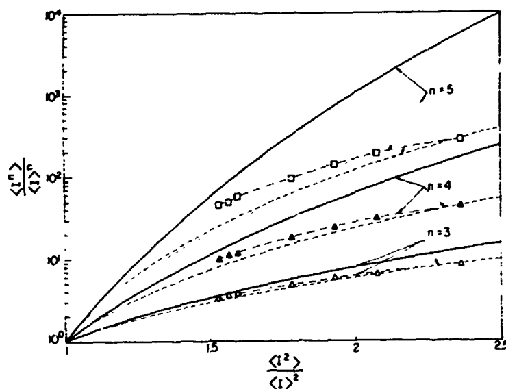
Fig. 1: Computed values of the aperture averaged normalized moments \langle I^n \rangle / \langle I \rangle^n for n=3-5 are compared with the values expected from various model distributions, having the same second moments \langle I^2 \rangle / \langle I \rangle^2 . The continuous lines indicate the moments obtained from log-normally distributed intensity fluctuations. The dashes lines indicate moments from \Gamma -distributed intensity fluctuations. Data were computed for \sigma_1^2 = 20
