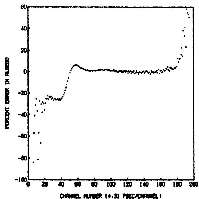
Fig. 2. Estimated percent errors in f_0 versus time for B(t) calculated from 7 azimuthal angles.
