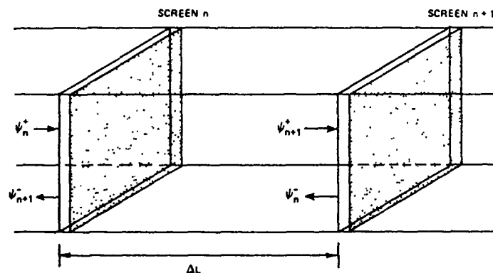
FIGURE 1 SPECTRAL DOMAIN ITERATION FOR INCREMENTAL SLAB
