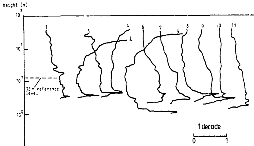
Figure 1. Examples of extinction profiles (see text).
