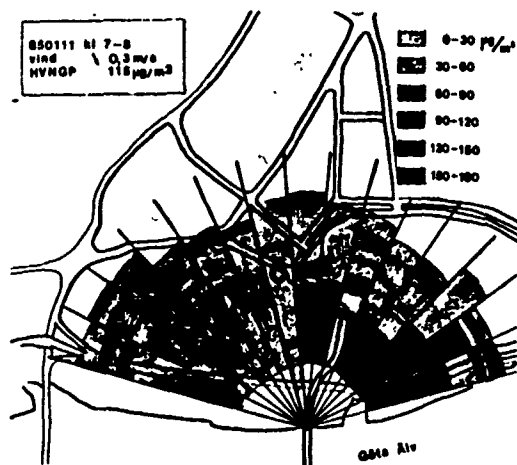
Fig. 1. Charting of \text{NO}_2 distribution by the dial technique [4].
