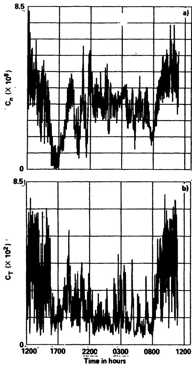
Figure 2. Comparison of optical (a) and acoustic (b) turbulence measured at the same location.
