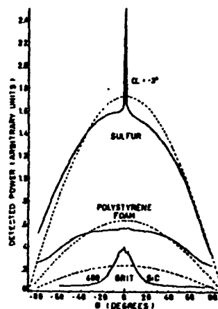
Fig. 5: Backscattered power as a function of target aspect angle \theta . Detector viewing angle \alpha = 3^\circ . For each curve the dashed line is least-squares best fit to a cosine ^5 .
