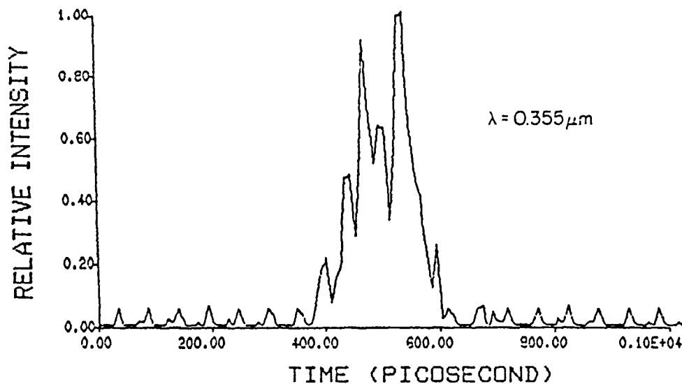
Figure 1. Typical waveform of a 30 ps FWHM Nd:YAG laser pulse that was reflected from a tilted CCR array target. The wavelength was 0.355 \mu\text{m} and target range was 389 m. The target consisted of 4 CCR's spaced 4 cm apart and tilted so that the range separation between adjacent CCR's was 4 mm. The structure within the pulse is due to speckle noise.
