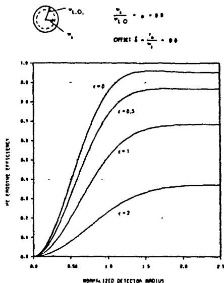
Fig. 4: Heterodyne efficiency as a function of normalized detector radius, the signal spot size w_s being slightly smaller than the L.O. ( w_{L.O.} ), for various levels of angle of arrival fluctuations \epsilon , \epsilon = 2 corresponding to strong turbulence and a path of several km.
