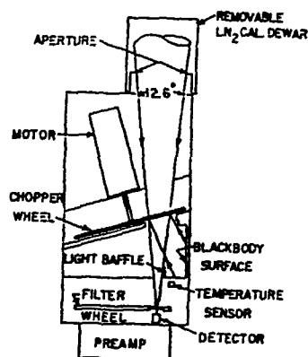
Figure 6. Infrared sky monitor.
