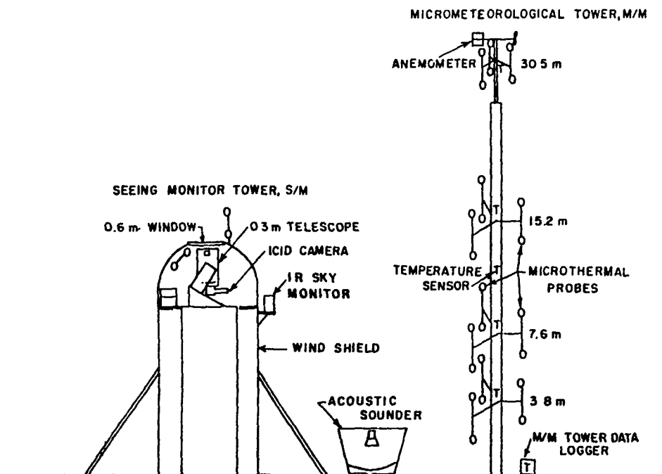
Figure 1. Site survey equipment arrangement.
