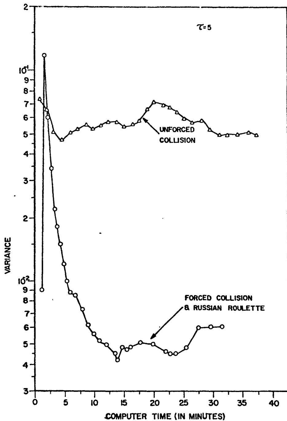
Fig. 1 - Variance in time dispersion vs computer time
