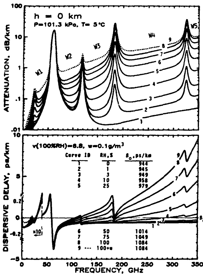
Figure 1. Specific attenuation ( \alpha ) and dispersive delay ( \beta ) for 9 (see ID) humidity cases of sea level air as predicted by the MPM program for a frequency range, f=1 to 350 GHz [1].
