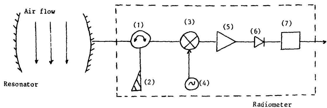
Figure 1 : Experimental set-up
