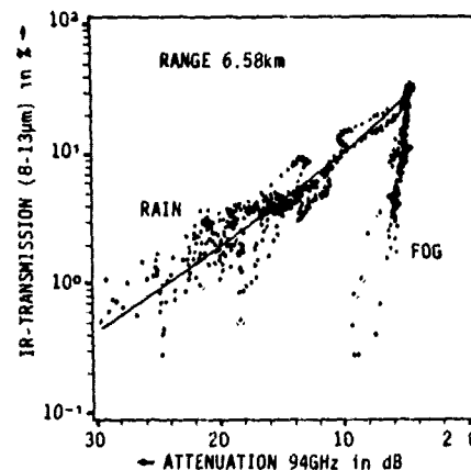
Fig.1: Correlation of IR-transmission and mmW attenuation for a range of 6.58km
