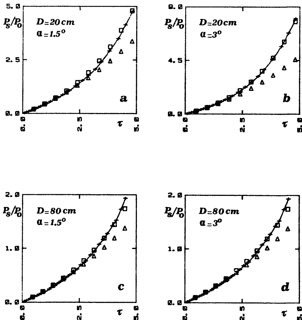
Fig. 1 - Comparison between calculated (squares) and measured (crosses connected by a continuous line) ratios P_s/P_0 between the received scattered power and the direct beam attenuated power. The ratios are plotted versus the optical depth \tau . The triangular marks indicate the summed contributions of the first two orders of scattering.
