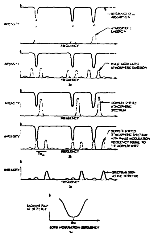
Figure 3. The principle of operation of the EOPM in measuring winds is shown.
