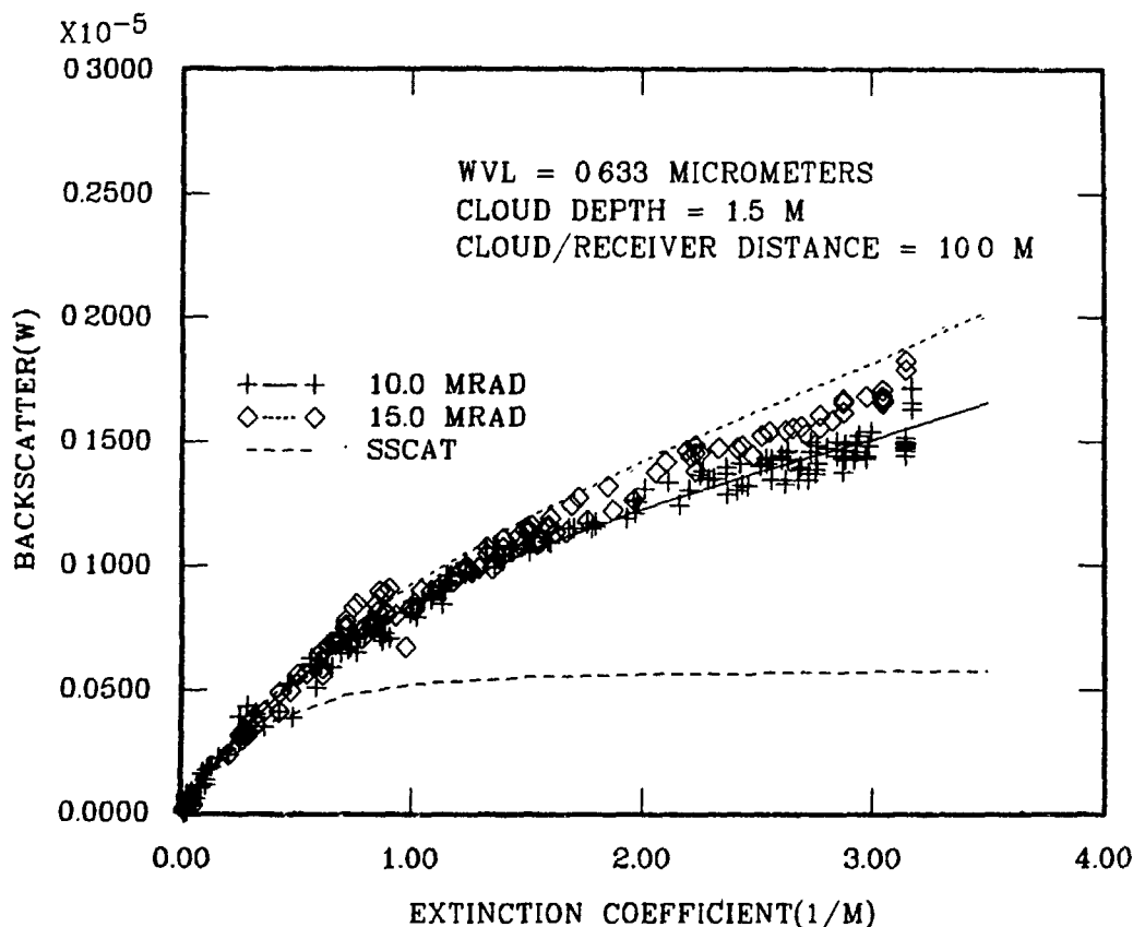
Fig. 2 - Measured and calculated backscattered power from laboratory-generated water droplet clouds as a function of cloud extinction coefficient. Curves are calculations and symbols, measurements. SSCAT is single-scattering solution.
