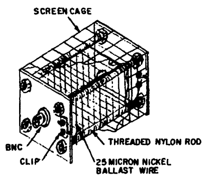
Figure 7. Microthermal probe construction
