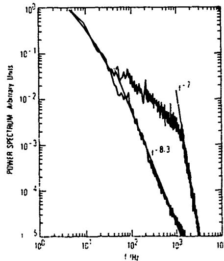
Fig. 3: Experimentally obtained phase-difference power spectrum measured during drizzle/light-rain conditions (upper trace) and a few minutes after the rain stopped (lower trace).
