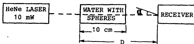
Fig. 3 - Scheme of the measurements. The container with the suspension of latex spheres in water is placed at different distances ( D ) from the receiver. \alpha : semiaperture of the receiver's F.O.V.
