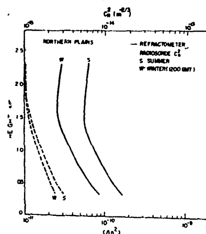
Fig.1 Height profiles of variance ( \langle \Delta n^2 \rangle ) of refractive index fluctuations measured with the refractometer for summer and winter conditions (solid curves). The corresponding profiles from radiosonde are marked dotted.
