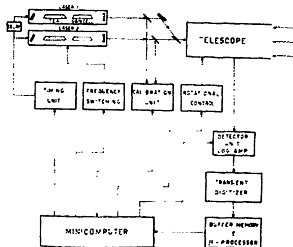
Fig. 1 - Layout of the LIDAR/DIAL facility
