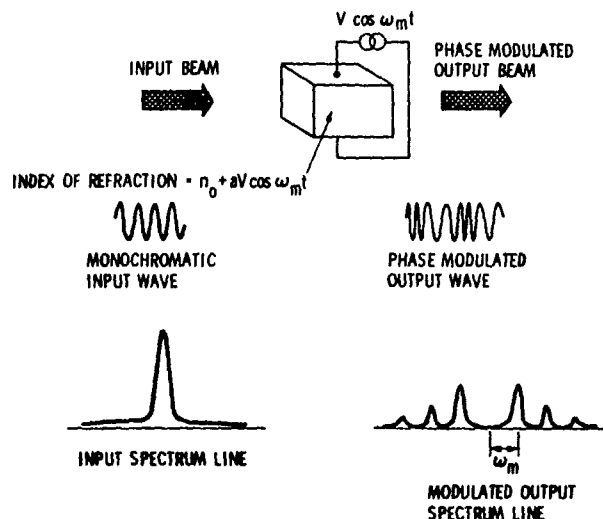
Figure 1. Electrooptic phase modulation is illustrated showing the effect of phase modulation upon a spectral line.
