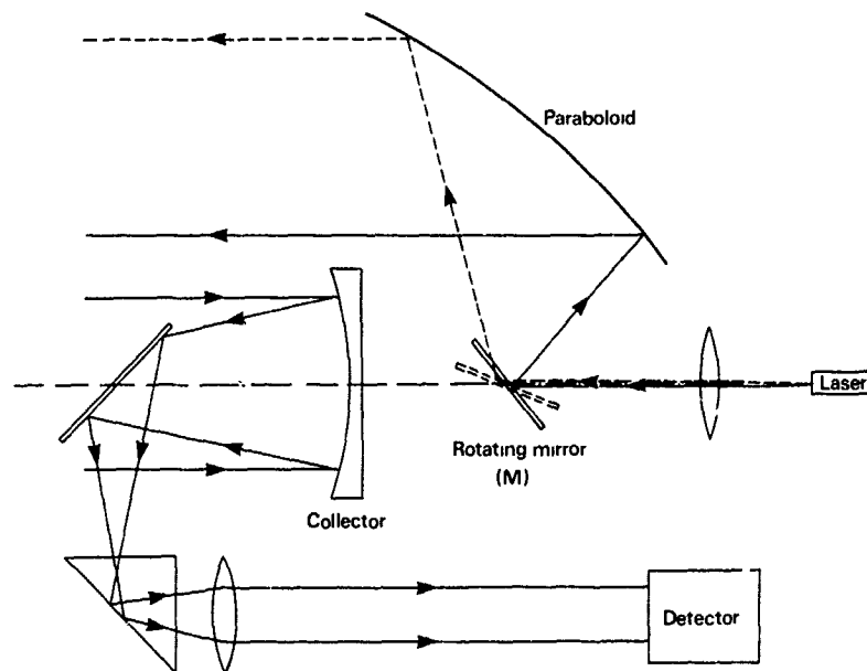
Fig. 1. Schematic diagram of proposed transmitter/receiver geometry.
