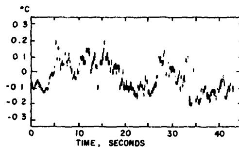
Figure 8. Typical digitized microthermal record.
