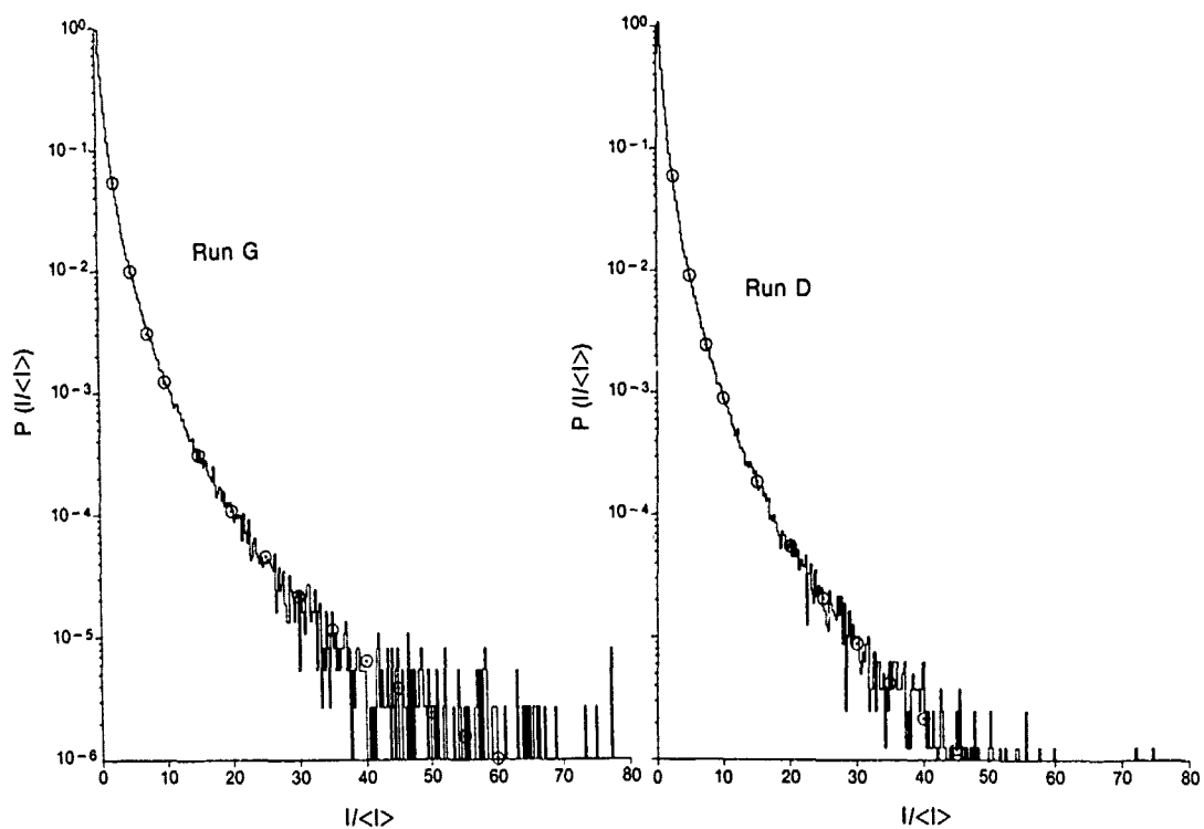
Figure 1. Probability density of irradiance normalized by the mean irradiance.
