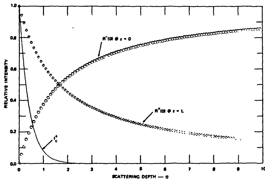
FIGURE 3 PLOT OF THE COHERENT INTENSITY, I_c^+ , AND THE INTENSITY OF THE TOTAL WAVE FIELD, R^+(0) , MEASURED AT THE EXIT PLANE OF A SLAB OF LOSSLESS SPHERES ( ka = 10 ), TOGETHER WITH TOTAL BACKSCATTERED INTENSITY AT THE ENTRY PLANE OF THE SLAB R^-(0) . (The depth parameter is defined as \eta = \pi a^2 DL , where a is the sphere radius, D is its density, and L is the layer thickness.)
