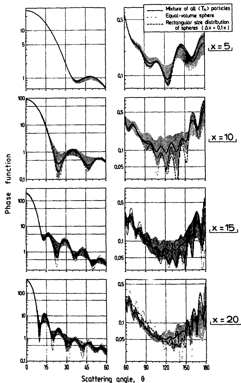
FIG. 3 Phase function in the near-forward scattering regime (left column) and in the side- and back-scattering regime (right column) versus scattering angle, \theta , for the mixture of all randomly-oriented Chebyshev particles, \langle T_n \rangle , and for equal-volume-sphere size parameters x = 5, 10, 15, 20 . Un-size-averaged and \Delta x = 0.1x size-averaged spherical phase functions are also shown for comparison. The shaded areas -- that are bounded by the lower and upper envelopes of the phase functions for all individual \langle T_n \rangle particles -- represent the range of variation of the nonspherical phase function.
