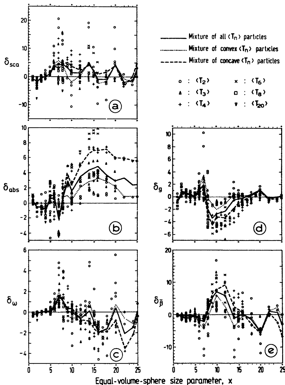
FIG. 2 Percent differences \delta_{sca} , \delta_{abs} , \delta_{\omega} , \delta_g , and \delta_{\beta} , between nonspherical and size-averaged (over \Delta x = 0.1x ) spherical Q_{sca} , Q_{abs} , \omega , g , and \beta , respectively, versus equal-volume-sphere size parameter, x . All randomly-oriented Chebyshev particles \langle T_n \rangle considered in this study are represented, as well as the three indicated different 'mixtures' of them.
