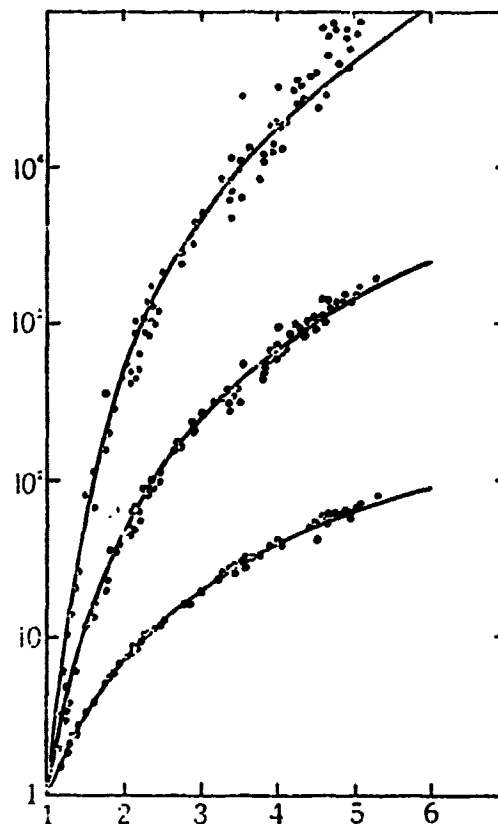
Fig. 1 Comparison of experimental data with I-K distribution for the special case \alpha=1/2 .
