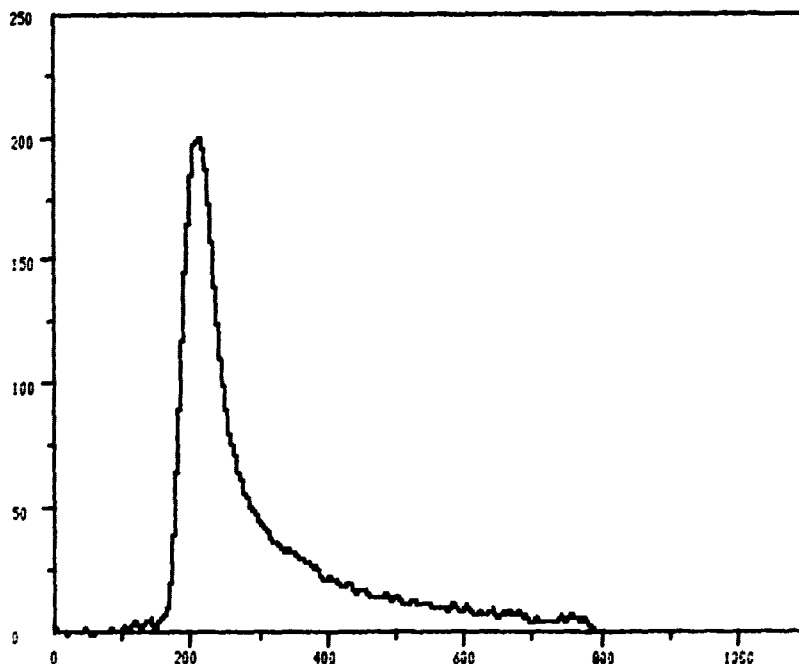
Fig. 1. Normalized backscattered radiance versus time in psec at outgoing polar and azimuthal angles of 20^\circ and 180^\circ and ingoing angles of 52^\circ and 0^\circ , respectively.
