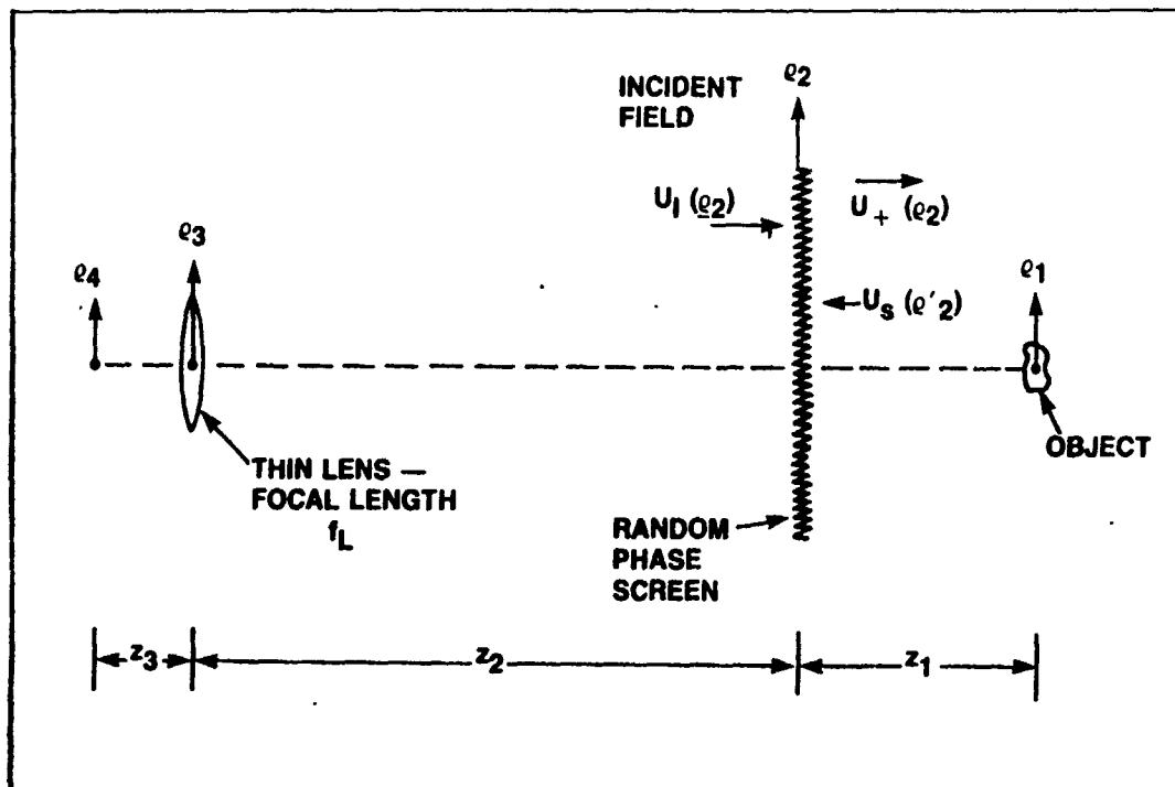
Figure 1: Imaging of an Object Behind a Phase Screen
