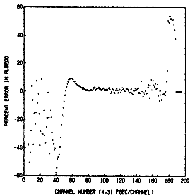
Fig. 3 Estimated percent errors in f_0 versus time for B(t) calculated from single azimuthal angle of 180^\circ , shown in Fig. 1.
