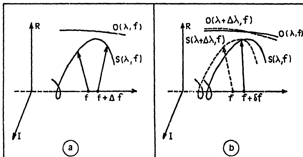
Figure. Schematic representation of complex functions O(\lambda, f) , O(\lambda+\Delta\lambda, f) , S(\lambda, f) and S(\lambda+\Delta\lambda, f) which appear in equations (5) and (7) of Knox Thompson (a) and dichromatic (b) techniques. Curves are drawn for one-dimensional signals and a region of the Fourier plane limited to a spatial frequency difference which corresponds to about one speckle. R = real part. I = imaginary part. Knox Thompson technique assumes small phase differences in S(\lambda, f) for \Delta f small with regard to r_0/\lambda . Dichromatic technique assumes a similarity relation between S(\lambda, f) and S(\lambda+\Delta\lambda, f) so that S(\lambda, f+\delta f) \sim S(\lambda+\Delta\lambda, f) with \delta f = f\Delta\lambda/\lambda . It is also assumed that O(\lambda+\Delta\lambda, f) \sim O(\lambda, f) .
