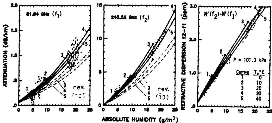
Figure 2. Specific attenuation \alpha and refractive dispersion \Delta N = N'(f_2) - N'(f_1) for air at temperatures ranging from 0° to 40°C measured in Tokyo, Japan over a line-of-sight path ( L = 0.81 km): rectangles, data clusters [2]; lines, MPM; circles, RH = 100%.
