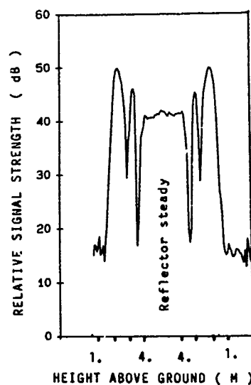
Fig. 3.2: Interference Pattern during Up-Down Sequence of Reflector. Field without Snow
