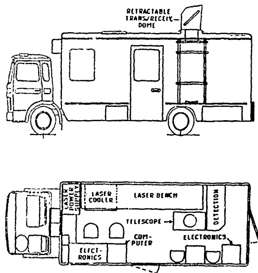
Fig.3. Mobile laboratory for atmospheric remote sensing [6]
