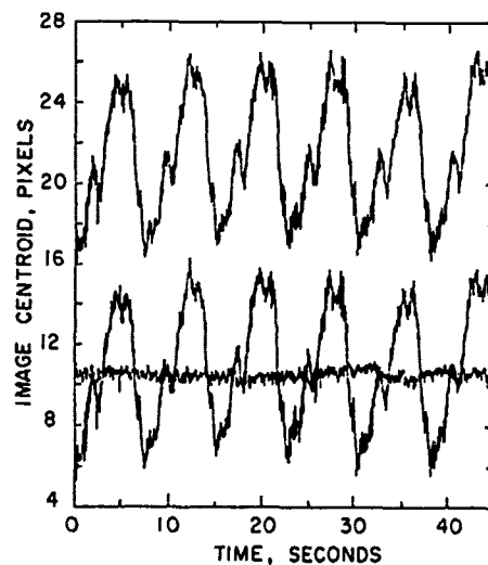
Figure 10. Seeing monitor image centroid motion for two separated images together with their difference motion.
