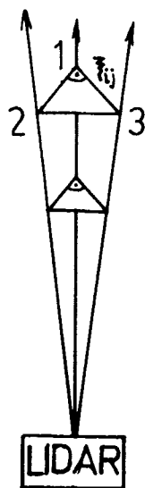
FIG.1 The geometry used for lidar wind measurements.
