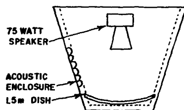
Figure 5. Acoustic sounder
