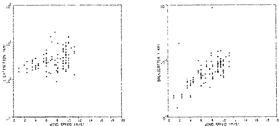
Figure 2. Windspeed dependence of lidar-derived extinction and backscatter coefficients ( 70\% < \text{RH} < 80\% ).
