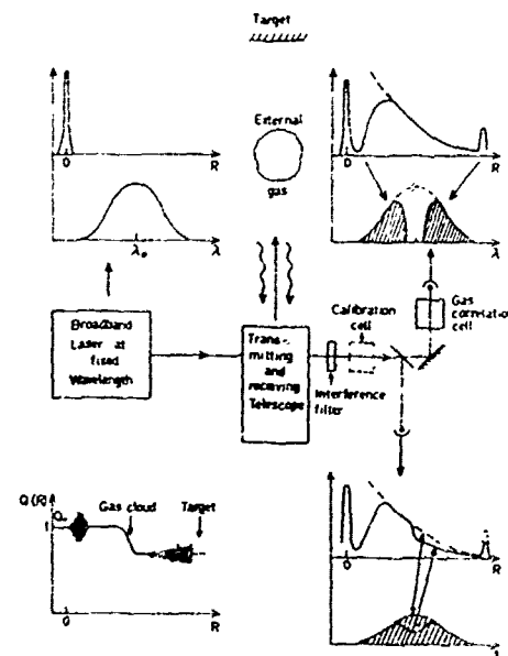
Fig.4. The principle of gas correlation lidar [7].
