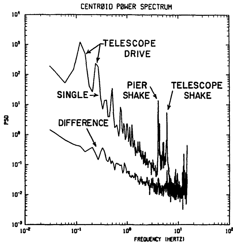
Figure 9. Seeing monitor image motion power spectral density vs. frequency for a single image and the difference motion. Telescope drive periodic errors and resonances in the pier and telescope excited by wind shake are also noted.
