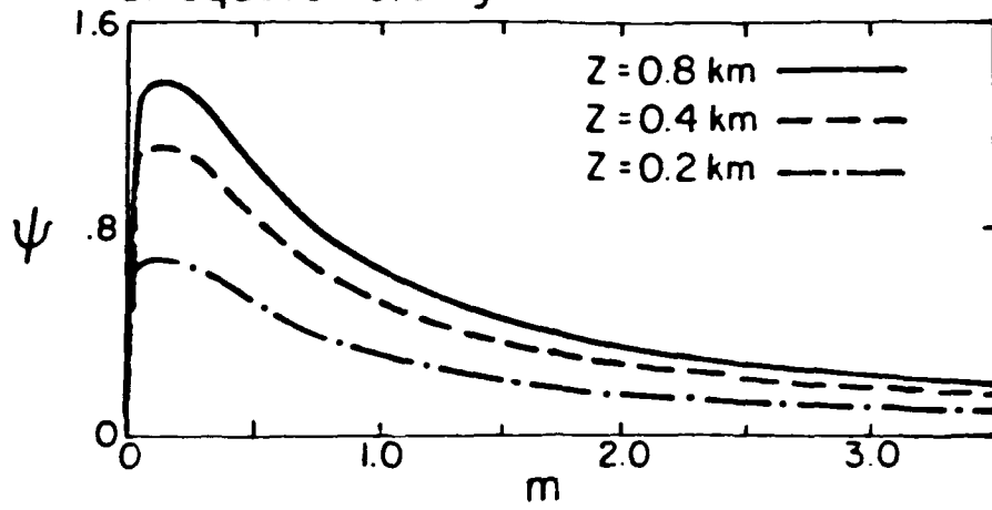
d. square forcing
