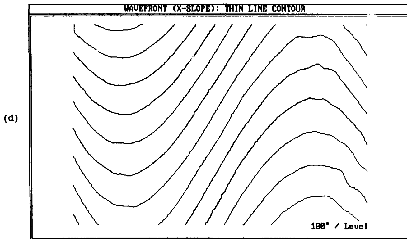
Figure 12: (c, d). Contour maps of wavefront slope {X-shear, off focus, large misalignment (negative)}
