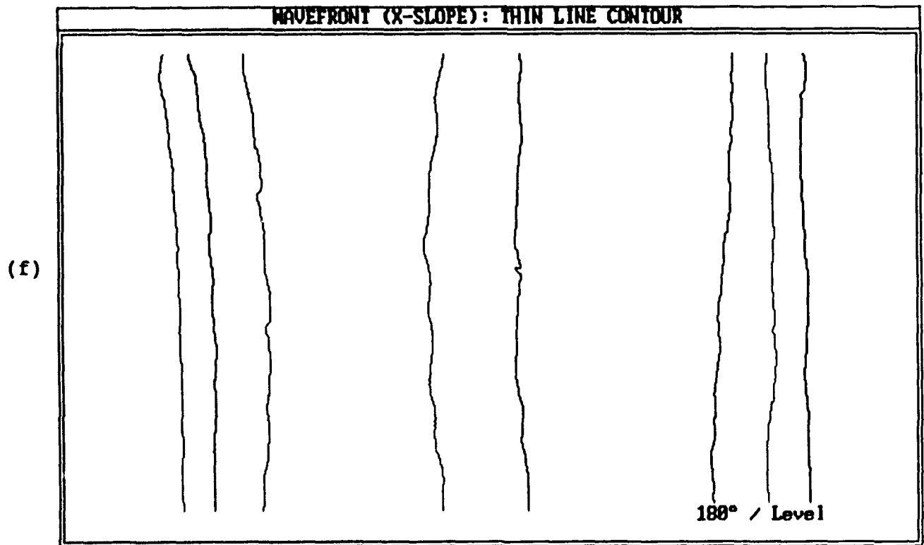
Figure 12: (e, f). Contour maps of wavefront slope, tilt removed {X-shear, off focus, large misalignment (negative)}
