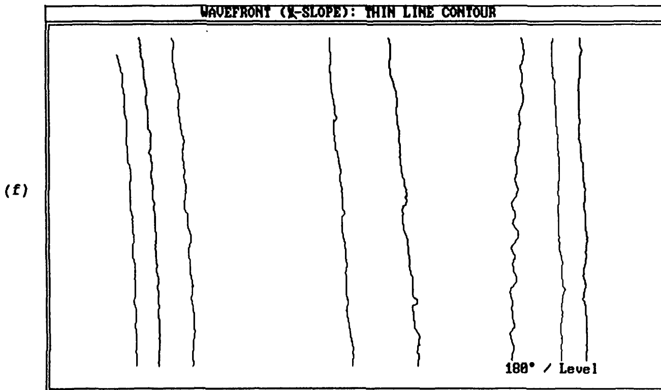
Figure 10: (e, f). Contour maps of wavefront slope, tilt removed {X-shear, off focus, large misalignment (positive)}
