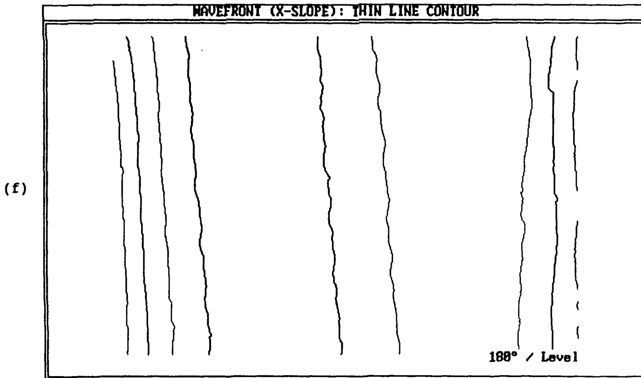
Figure 7: (e, f). Contour maps of wavefront slope, tilt removed {X-shear, in focus, large misalignment (negative)}
