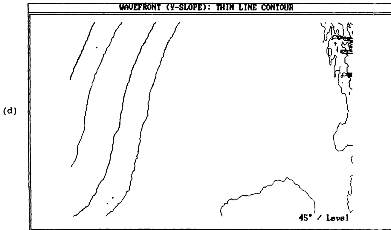
Figure 13: (c, d). Contour maps of wavefront slope (Y-shear, in focus, aligned)
