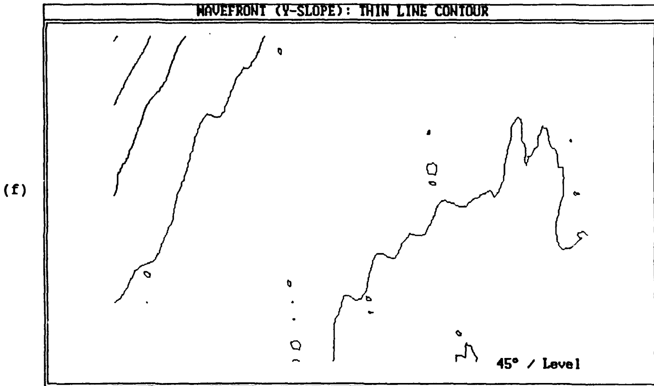
Figure 15: (e, f). Contour maps of wavefront slope, tilt removed (Y-shear, in focus, medium misalignment)
