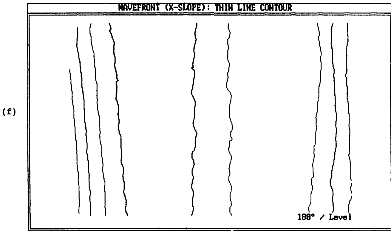
Figure 4: (e, f). Contour maps of wavefront slope, tilt removed {X-shear, in focus, large misalignment (positive)}
