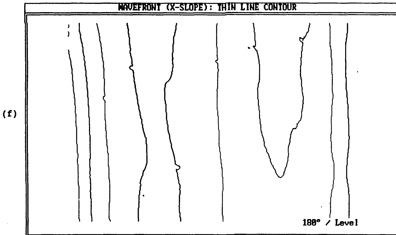
Figure 2: (e, f). Contour maps of wavefront slope, tilt removed (X-shear, in focus, small misalignment (positive))
