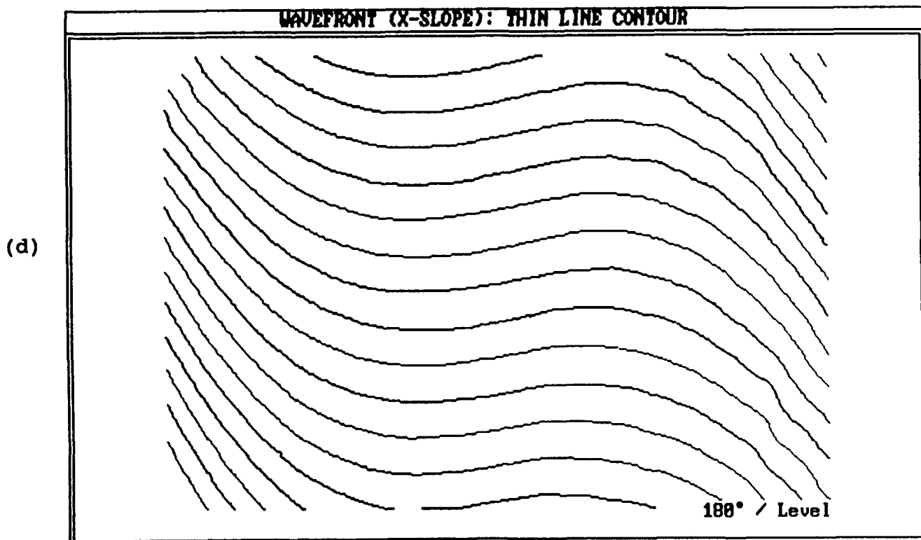
Figure 4: (c, d). Contour maps of wavefront slope {X-shear, in focus, large misalignment (positive)}
