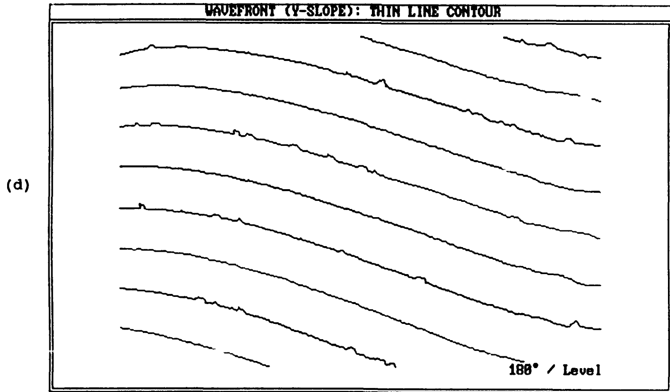
Figure 20: (c, d). Contour maps of wavefront slope {Y-shear, off focus, small misalignment (negative)}
