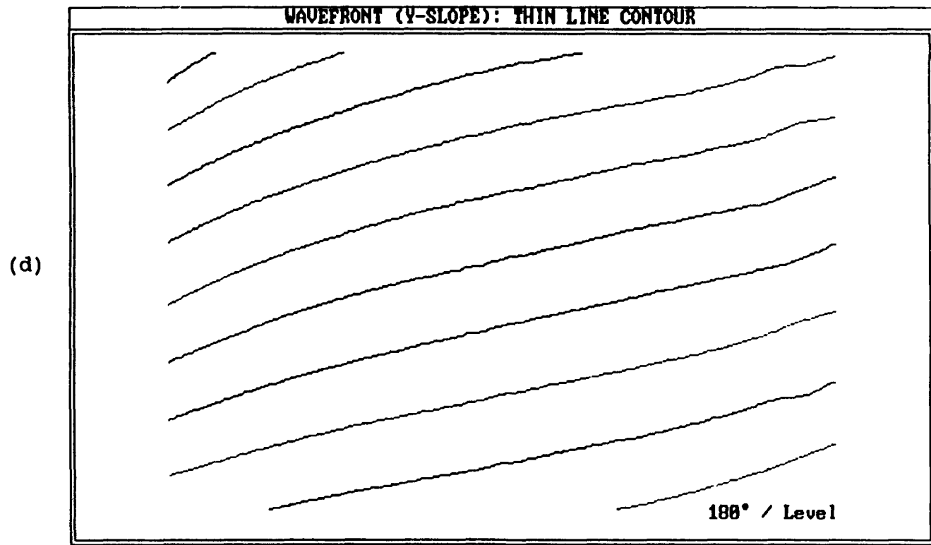
Figure 18: (c, d). Contour maps of wavefront slope {Y-shear, off focus, small misalignment (positive)}
