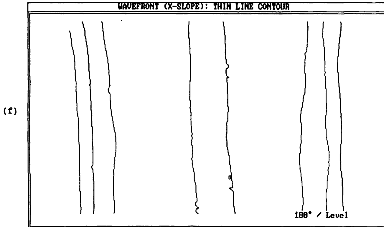
Figure 9: (e, f). Contour maps of wavefront slope, tilt removed {X-shear, off focus, small misalignment (positive)}
