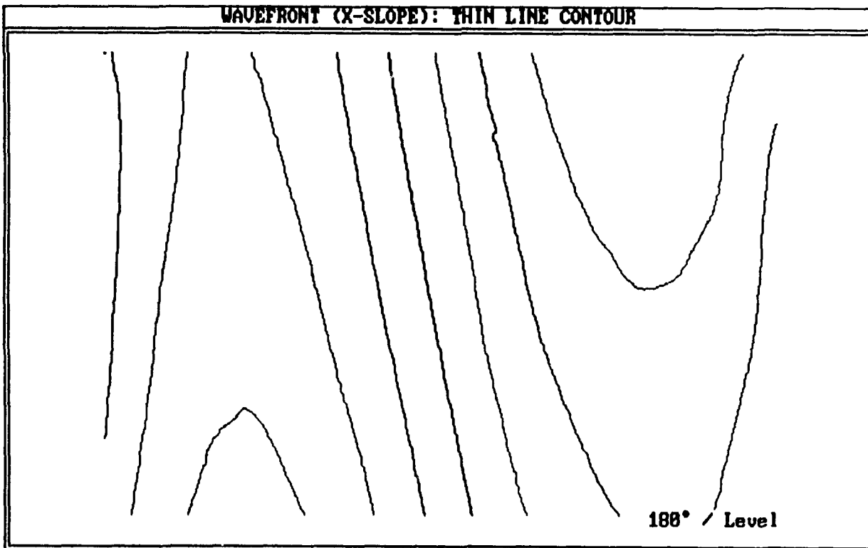
Figure 9: (c, d). Contour maps of wavefront slope {X-shear, off focus, small misalignment (positive)}
