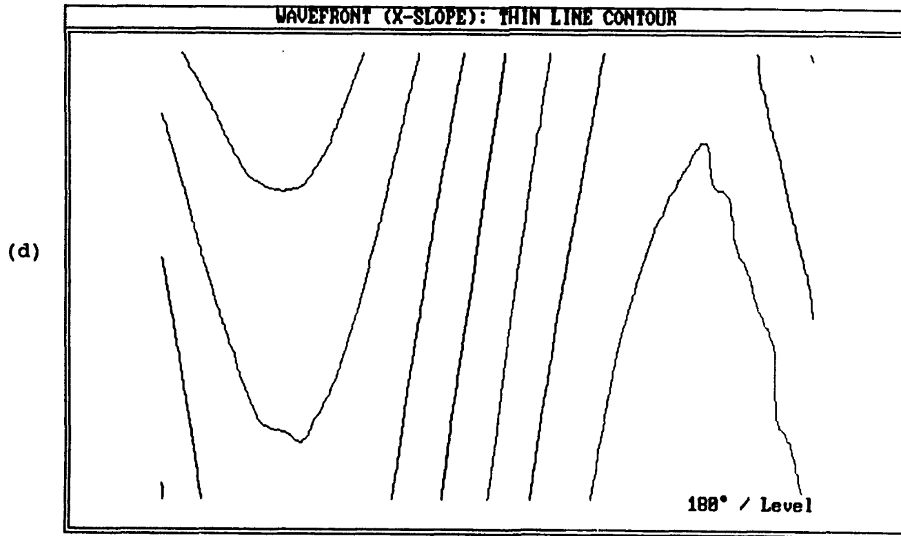
Figure 11: (c, d). Contour maps of wavefront slope {X-shear, off focus, small misalignment (negative)}
