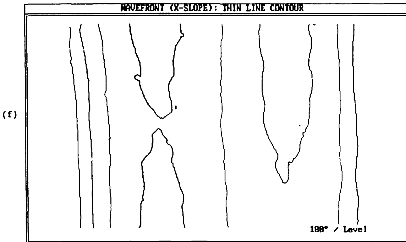
Figure 3: (e, f). Contour maps of wavefront slope, tilt removed {X-shear, in focus, medium misalignment (positive)}
