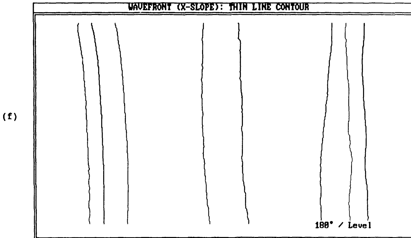
Figure 8: (e, f). Contour maps of wavefront slope, tilt removed (X-shear, off focus, aligned)
