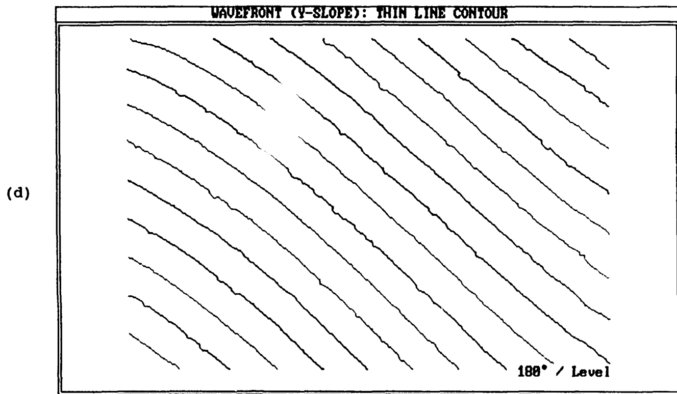
Figure 21: (c, d). Contour maps of wavefront slope {Y-shear, off focus, large misalignment (negative)}
