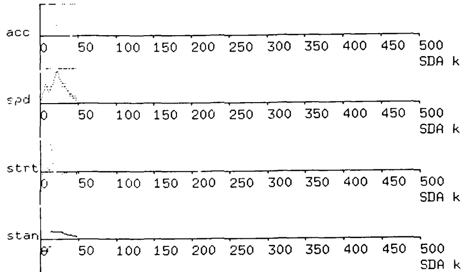
Figure 58: Command signals generated: acc - wheel acceleration, spd - rear wheel speed, strt - steering angle rate, stan - steering angle
