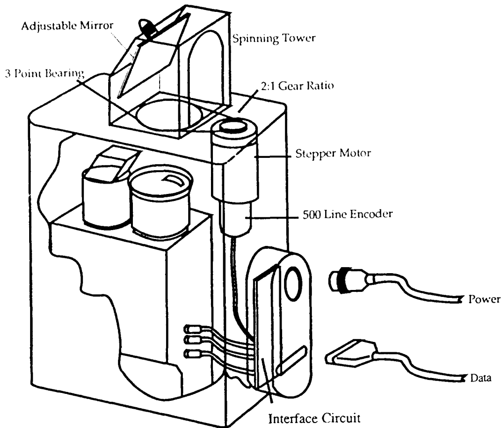
Figure 68: Scanner enclosure
