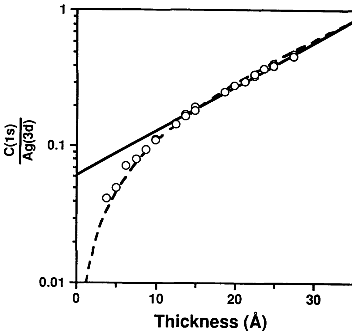
Figure 2. Relation between XPS intensities of C(1s) and Ag(3d), and thicknesses for n -alkanethiolate monolayers on silver. Values of C(1s)/Ag(3d) are a function of instrumental parameters; trends are important here. The dashed line displays the theoretical relation given in eq 8 using K = 1.75 . The thicknesses of the hydrocarbon layer of the monolayers were estimated using eq 9. The solid line represents a linear least-squares fit to the data presented in the figure ( R^2 = 0.994 ) for monolayers prepared from C_nH_{2n+1}SH ( n = 11 - 22 ).
