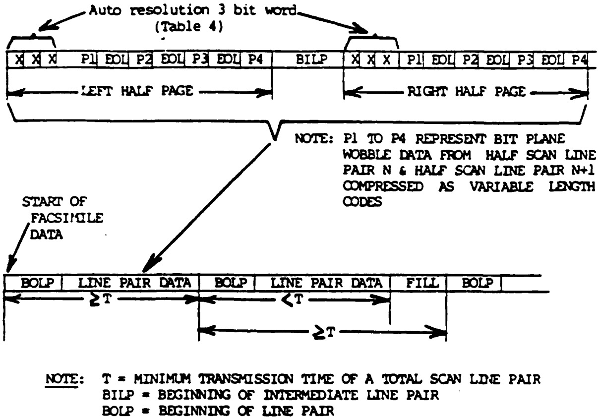
Figure 1. Example for an encoded scan line pair of 16 grey shades starting at the beginning of a page
