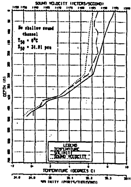
Figure 40. Characteristic profiles representing typical summer oceanographic conditions found on the central Iceland/Faeroes Ridge in water 400 to 500 m deep: (a) with small amounts of Arctic water close to seabed. (b) with filament/eddy Arctic water close to seabed.
