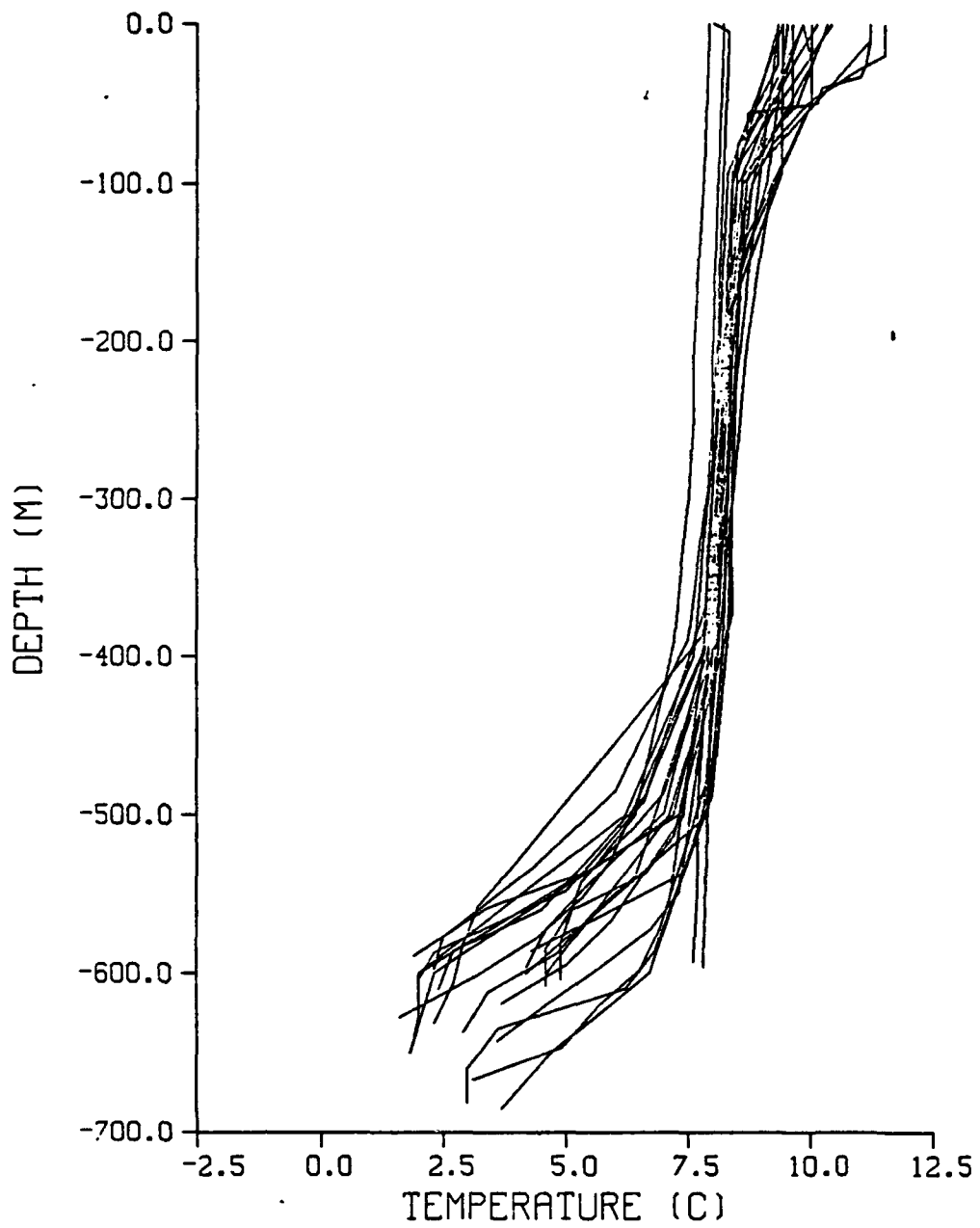
Figure 26. Temperature-depth plot for summer data collected between 10° and 12°W on the south-western side of the Iceland/Faeroes Ridge with water depths between 600 and 700 m.
