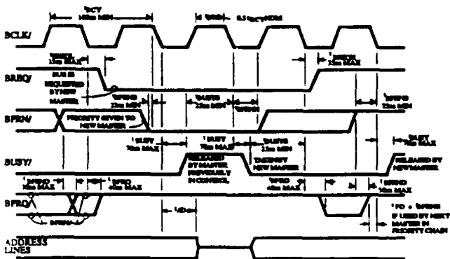
Figure 2. A timing diagram from the specification of the Intel Multibus [1]. Constraints specify separation times between events (i.e., changes in logic level on signal wires).
