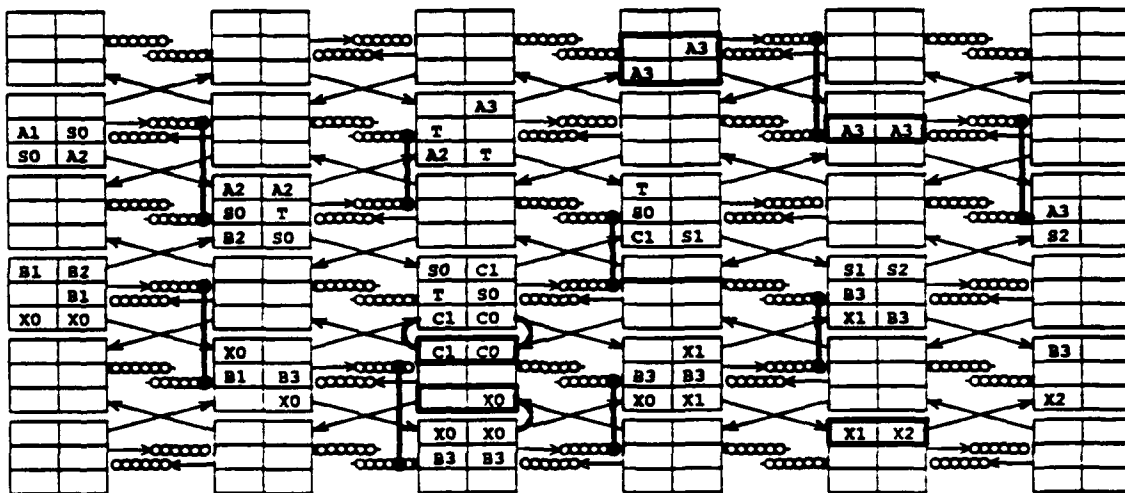
Figure 10 Layout for the Lyon bit-serial multiplier cell.
