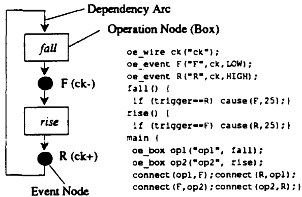
Figure 4. Graphical and textual versions of a simple single phase clock in the OEgraph representation (from a behavioral perspective). The clock has a cycle time of 50 time units with a 50% duty-cycle.
