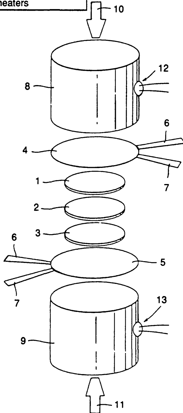
Fig 8 Simplified diagram of the single cell tester
