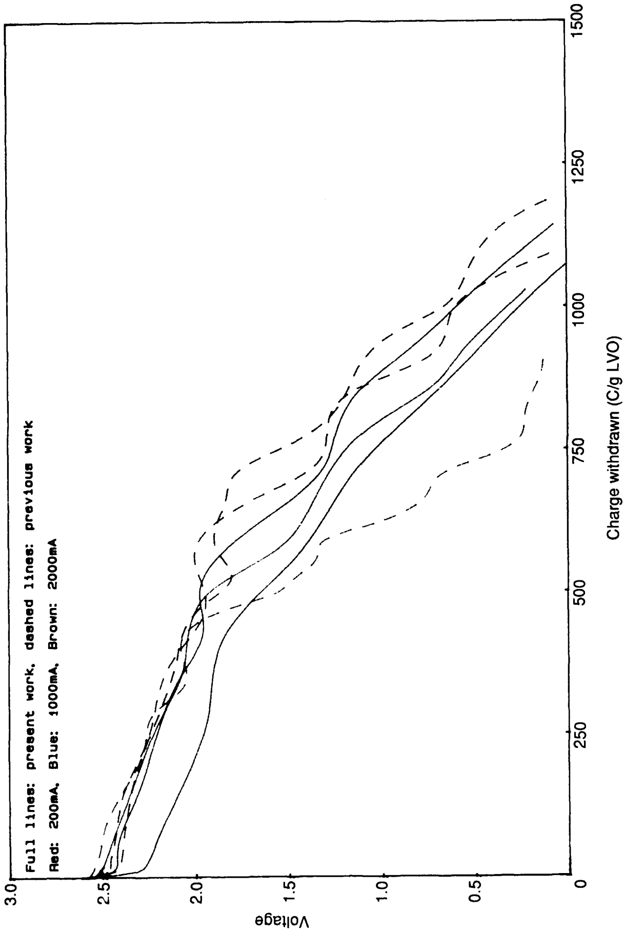
Fig 21 LVO 580C
