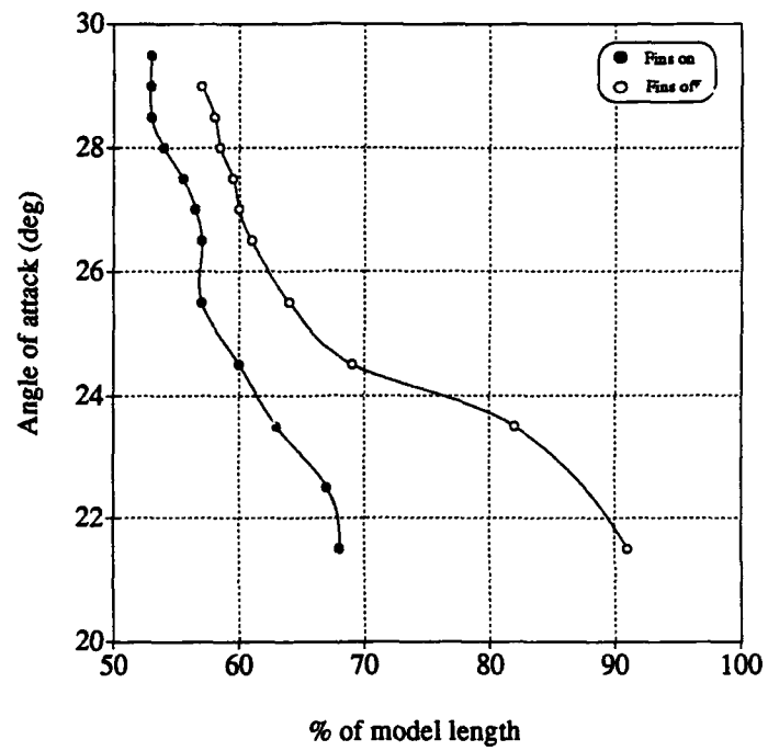
Figure 6. Location of vortex burst position
