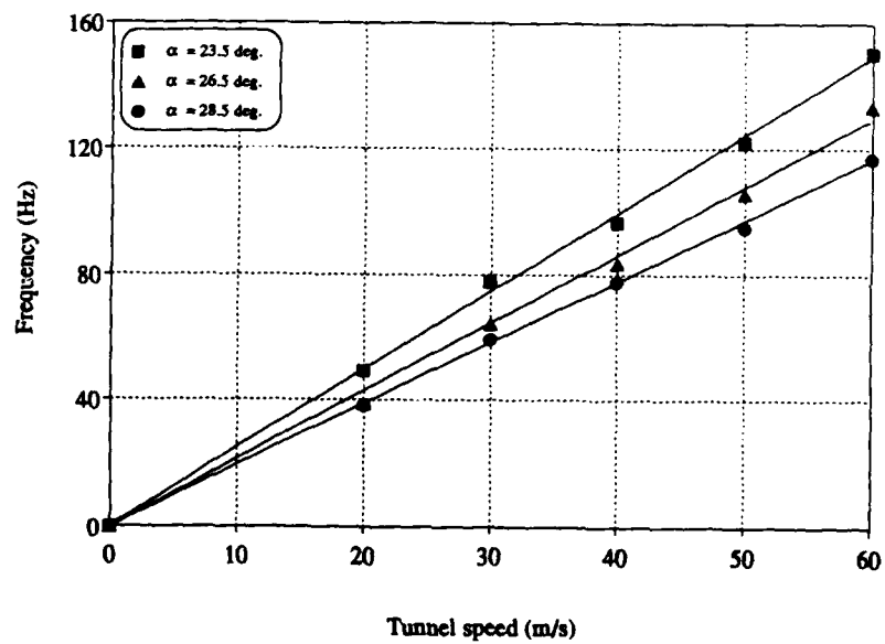
Figure 12. Variation of vortex burst frequency with tunnel speed - fins off
