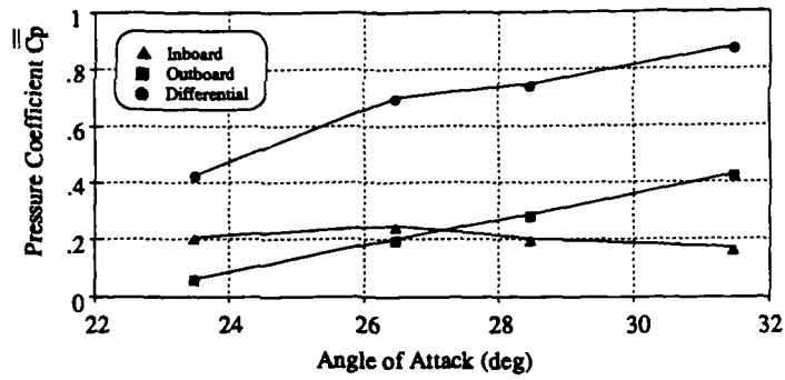
Figure 20. Pressure coefficient variation on port fin; 10 % chord, 30 % span, tunnel speed 50 m/sec
