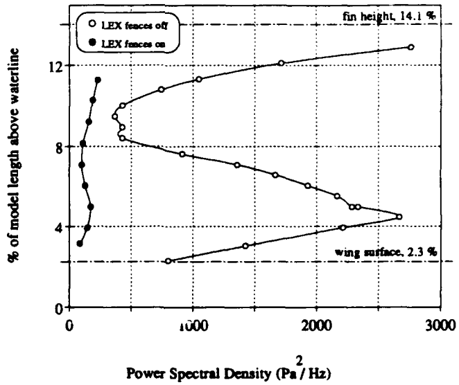
Figure 14. Power Spectral Density of pressure probe measurements through vortex burst; Traverse parallel to model normal axis. \alpha = 26.5 deg, V = 50 m/s
