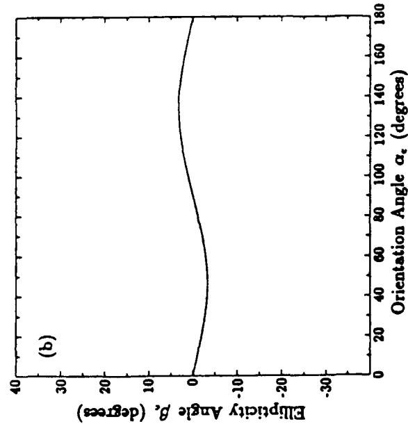
Figure 1.4.11 For the three-layer configuration: (a) Copolarized signature normalized to \sigma_{AA} , (b) Signature distortion track.
