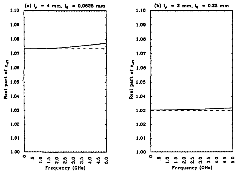
Figure 3. Real part of \epsilon_{eff} as a function of frequency. (a) l_\rho = 4 mm and l_z = 0.0625 mm, (b) l_\rho = 2 mm and l_z = 0.25 mm, (c) l_\rho = 1 mm and l_z = 1 mm, (d) l_\rho = 0.5 mm and l_z = 4 mm, and (e) l_\rho = 0.25 mm and l_z = 16 mm. The dashed line corresponds to discrete scatterer theory. The solid curve corresponds to strong fluctuation theory.
