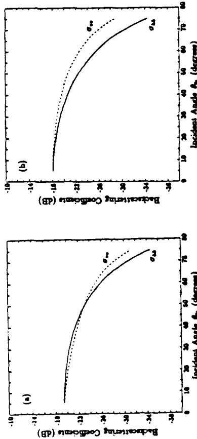
Figure 1.4.2 Conventional backscattering coefficients: (a) untilted anisotropic random medium, (b) isotropic random medium.
