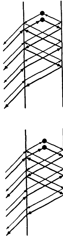
b Opposite directions
