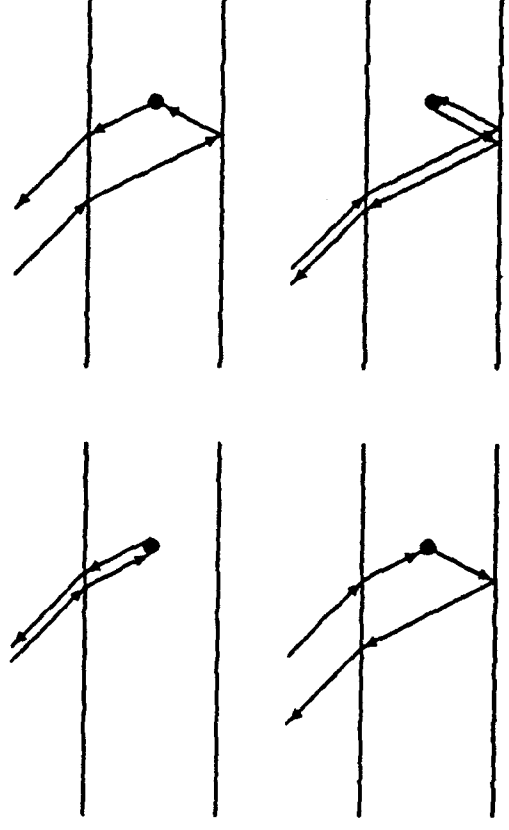
Figure 1.3.4 Wave scattering processes.
