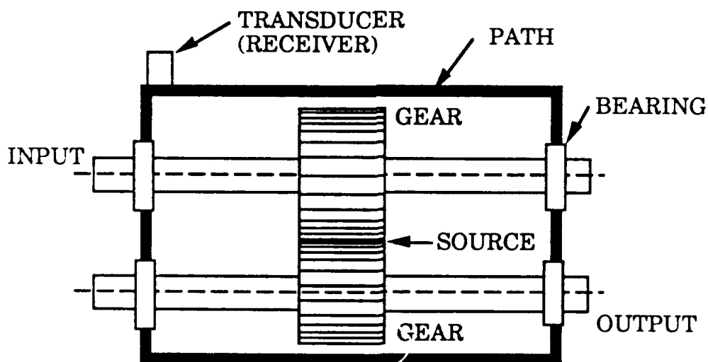
Figure IV-3. Source-path-receiver Model.
