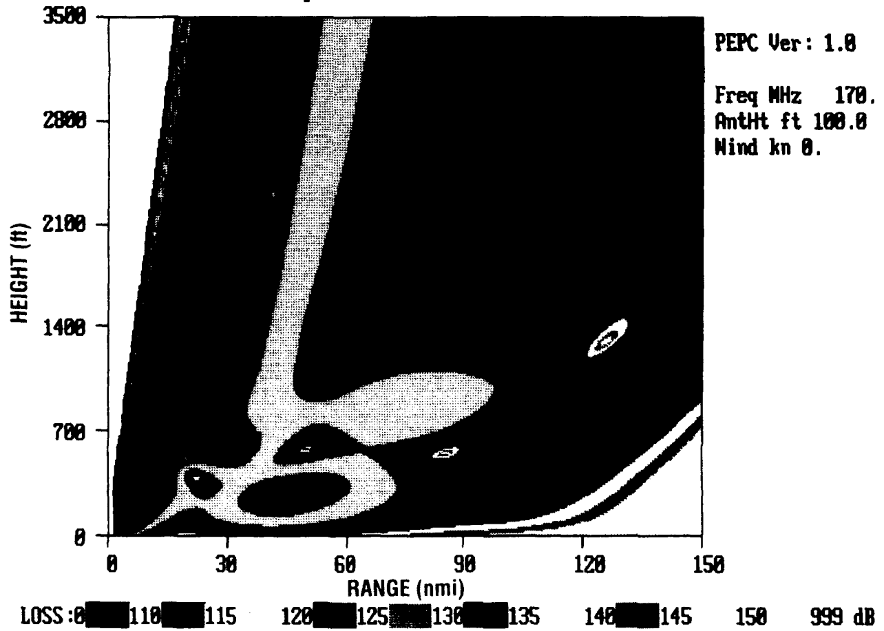
Figure 26. Coverage diagram for environment of 12 March 1948 at 170 MHz.
