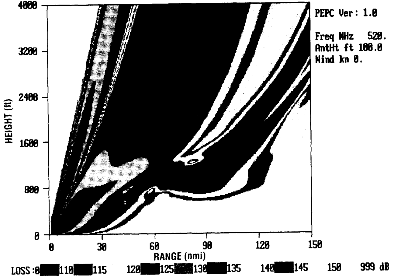
Figure 57. Coverage diagram for environment of 13 November 1947 at 520 MHz.
