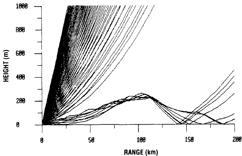
Figure 11. Range-dependent ray trace with trapping layer (represented by shaded area) varying with range. Antenna height is 25 m.
