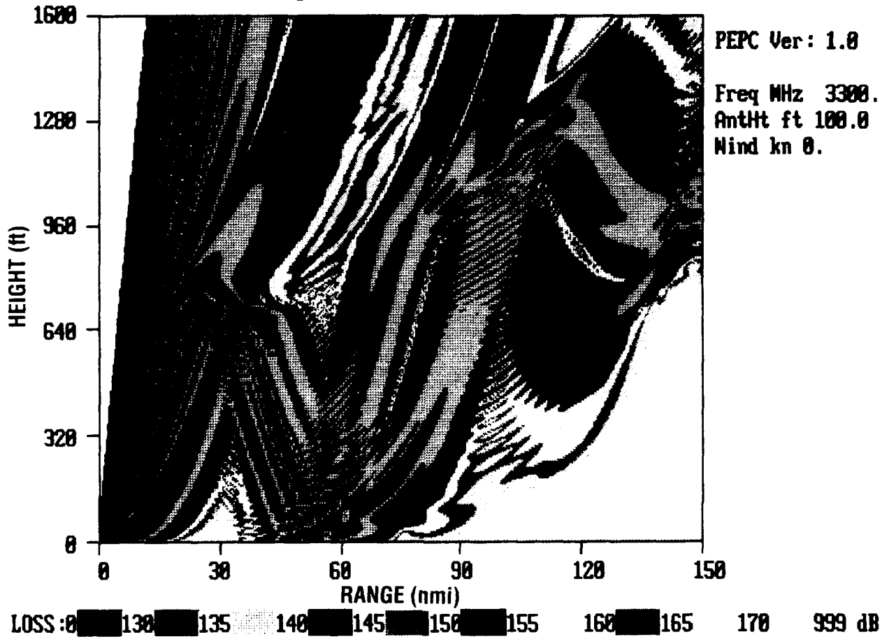
Figure 28. Coverage diagram for environment of 12 March 1948 at 3300 MHz.
