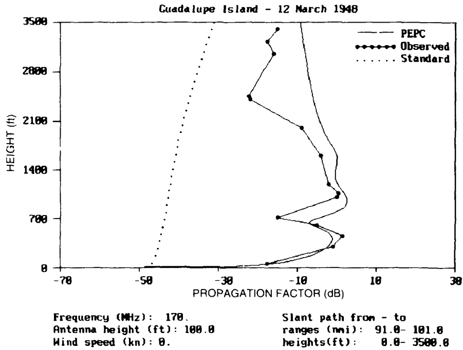
Figure 18. Comparisons between PEPC and measured radio data at 170 MHz for 12 March 1948, along slant path from 91 to 101 nmi.
