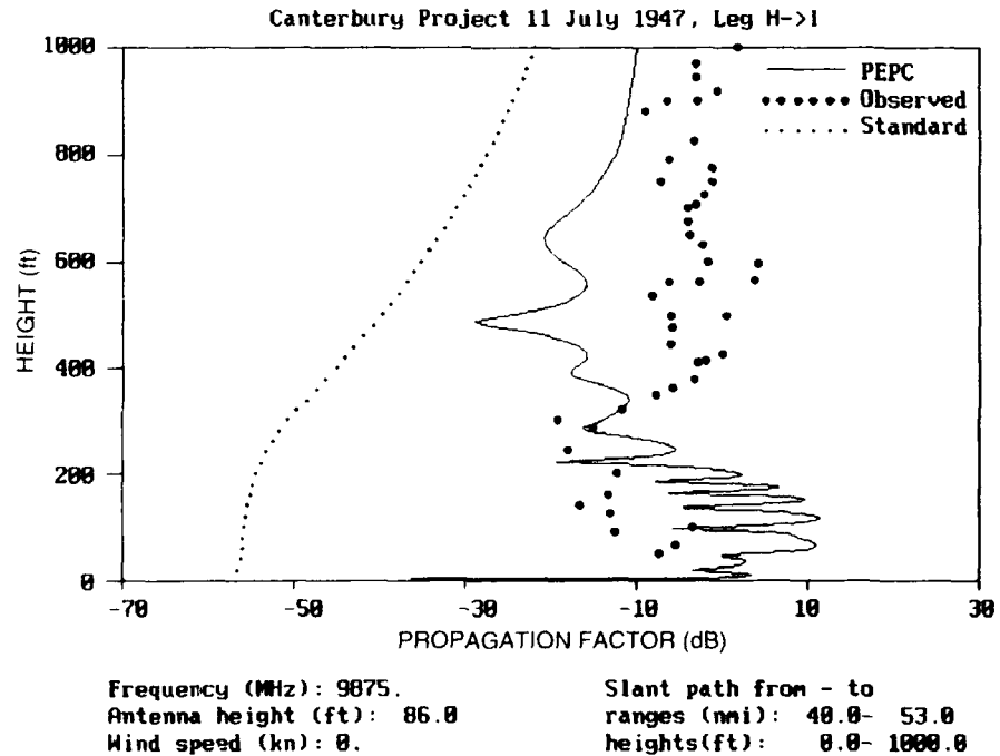
Figure 70. Comparisons between PEPC and measured radio data for flight path labeled HI from Canterbury Project data record of 11 July 1947, for antenna height at 86 feet.
