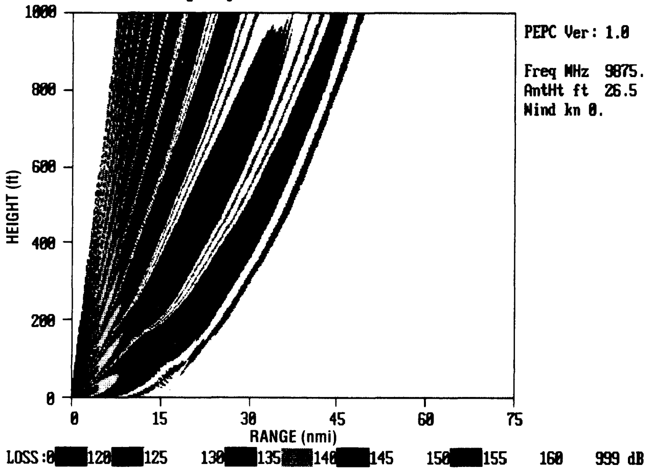
Figure 65. Cover diagram for frequency and environment from figure 62.
