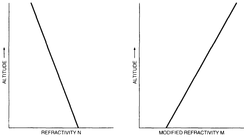
Figure 1. Refractivity N and modified refractivity M versus altitude for a standard atmosphere.
