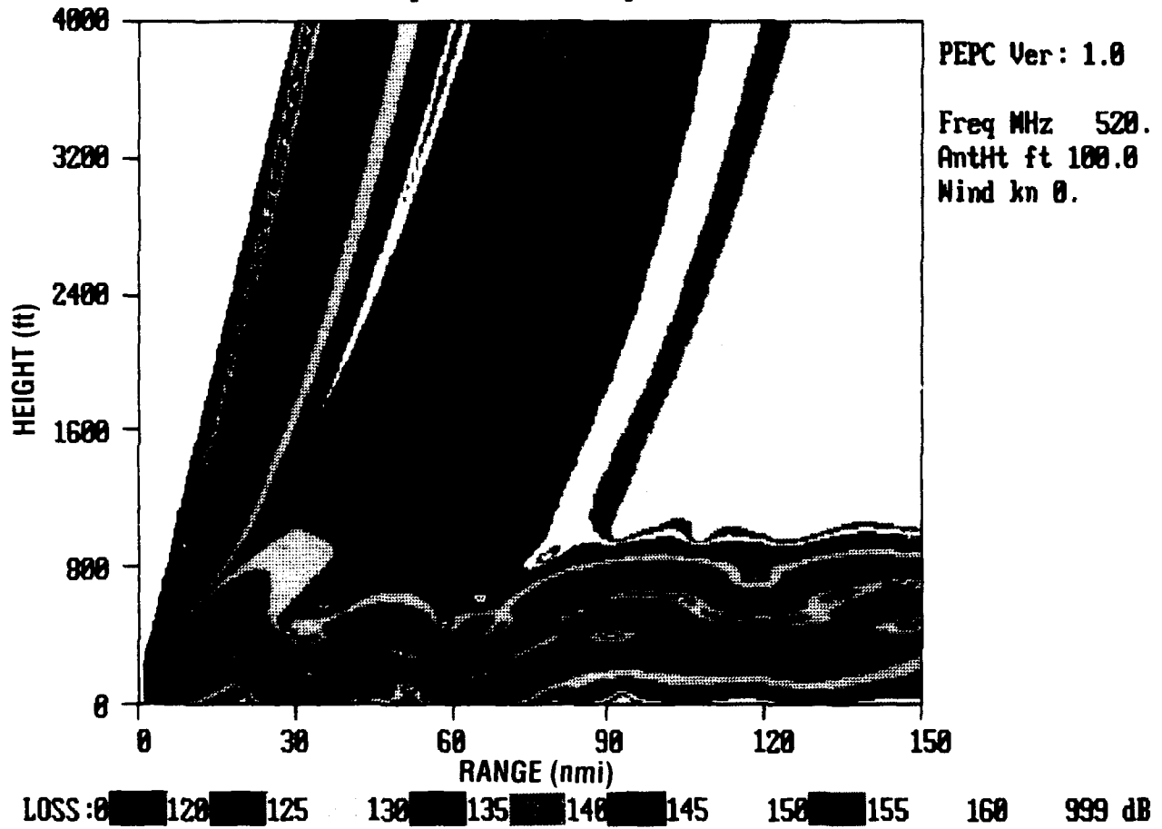
Figure 45. Coverage diagram for environment of 8 April 1948 at 520 MHz.
