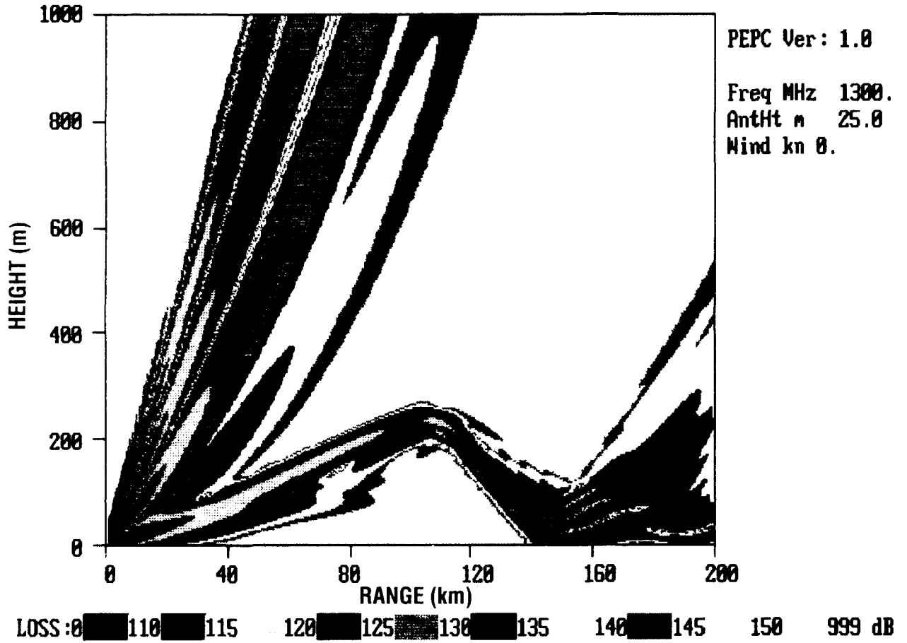
Figure 12. Coverage diagram for environment of figure 11.
