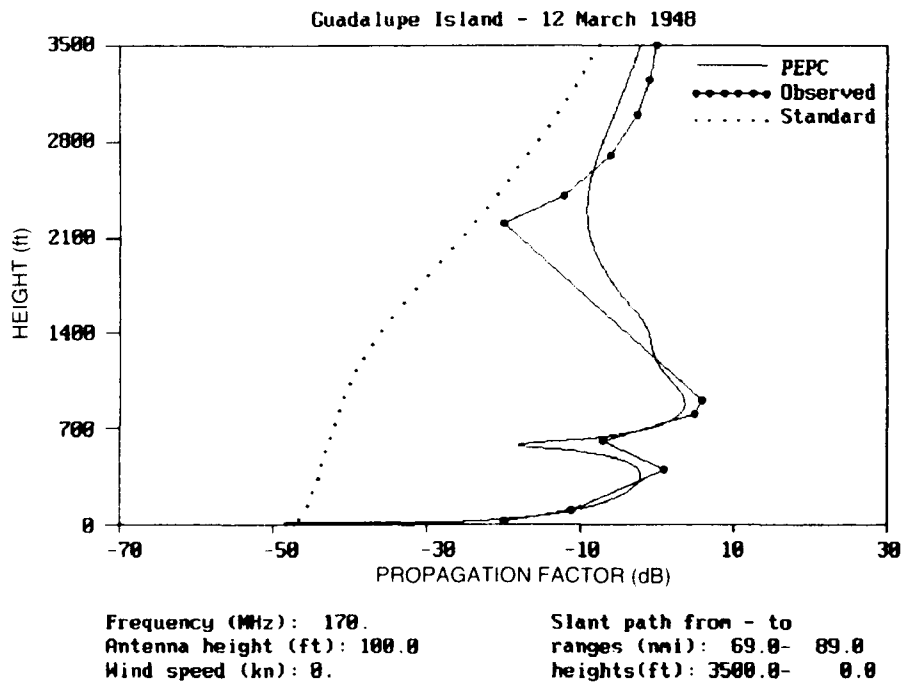
Figure 17. Comparisons between PEPC and measured radio data at 170 MHz for 12 March 1948, along slant path from 69 to 89 nmi.
