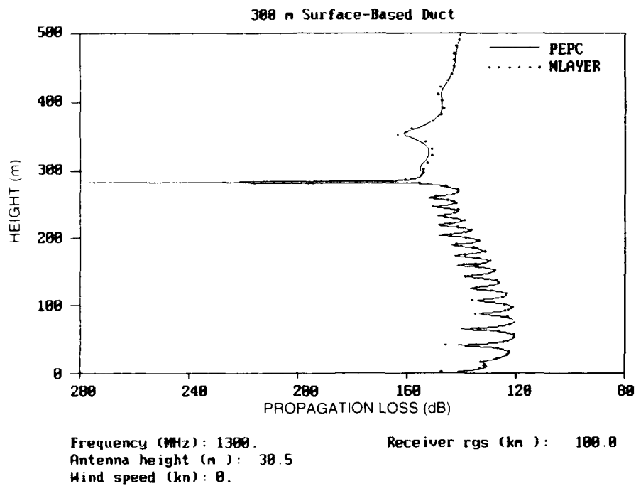
Figure 6. Height-gain plot comparison of PEPC and MAYER for 300-m surface-based duct.
