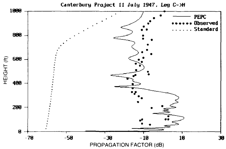
Figure 67. Comparisons between PEPC and measured radio data for flight path labeled GH from Canterbury Project data record of 11 July 1947, for antenna height at 26.5 feet.
