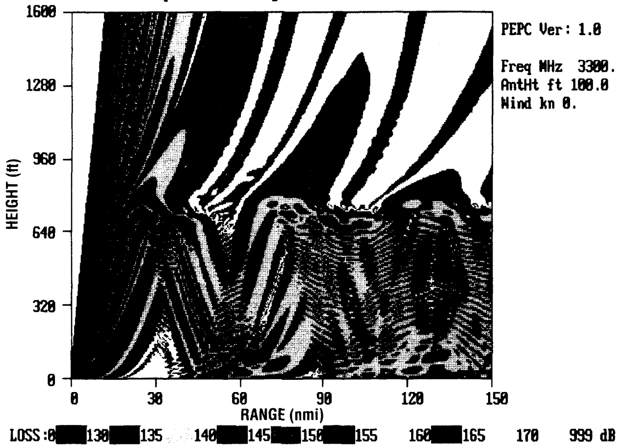
Figure 29. Coverage diagram using homogeneous profile measured at 39 nmi taken from the 12 March 1948 data record.
