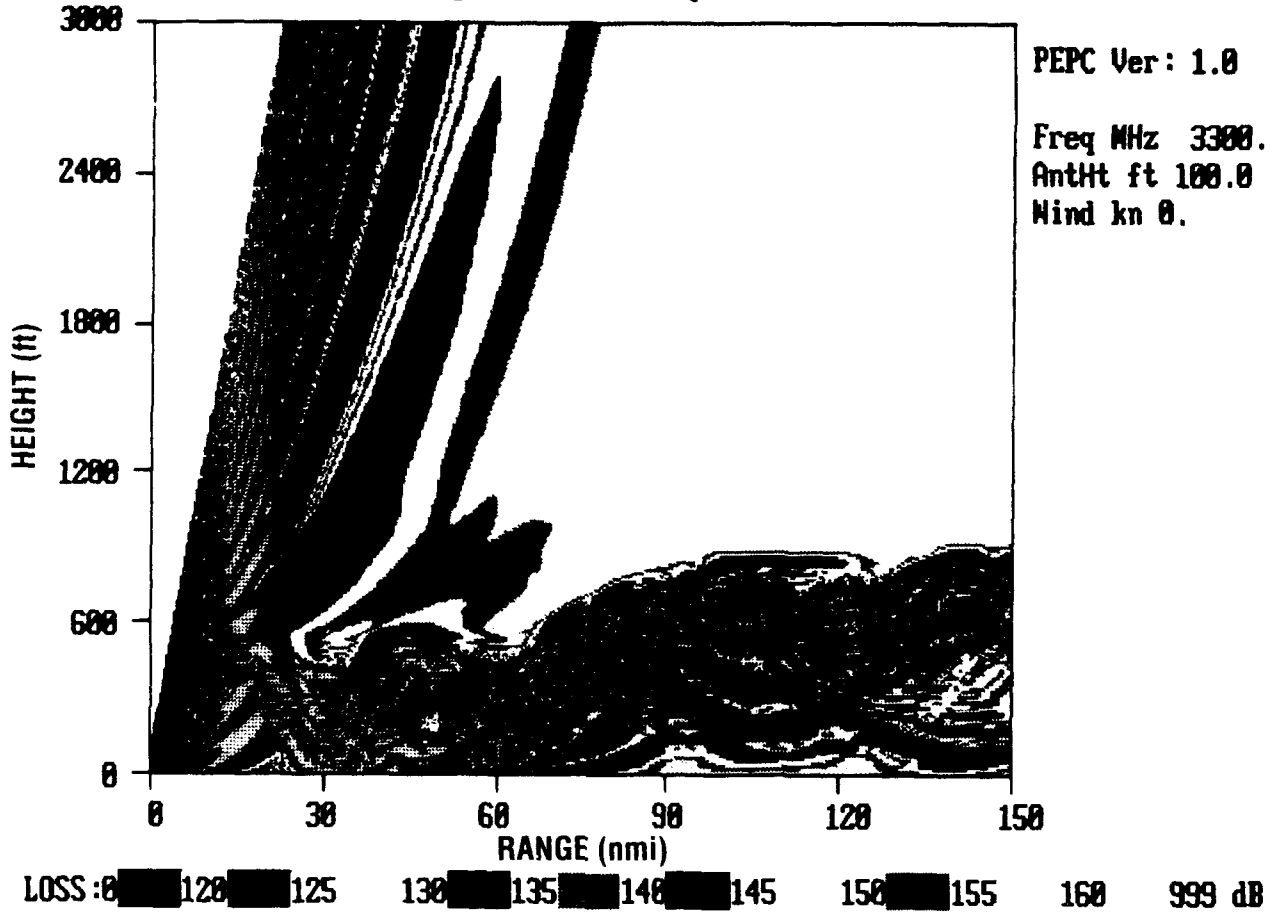
Figure 46. Coverage diagram for environment of 8 April 1948 at 3300 MHz.
