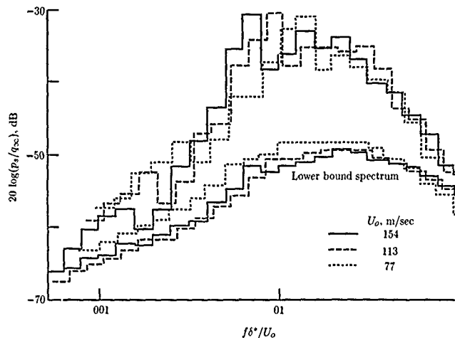
Figure 11. Measured surface pressure spectra p_s at two spanwise stations near the trailing edge of an HFB 320 flap in cruise configuration. q_\infty is free-stream dynamic pressure. (From ref. 54.)
