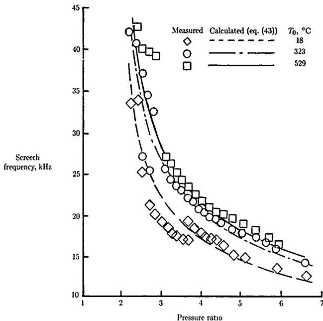
Figure 33. Dependence of screech tone frequency on jet pressure ratio at different total temperatures T_0 for convergent nozzle. (Based on ref. 98.)
