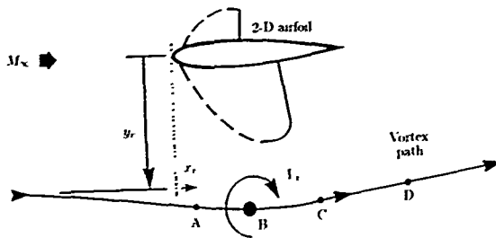
Figure 61. Two-dimensional approximation of BVI problem. (Based on ref. 70.)
