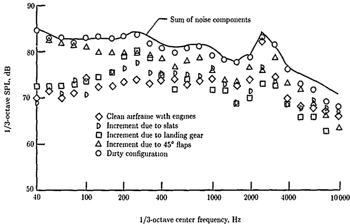
Figure 14. Comparison of sum of measured noise components with measured total noise for VC10 at approach (ref. 10). (From ref. 27.)
