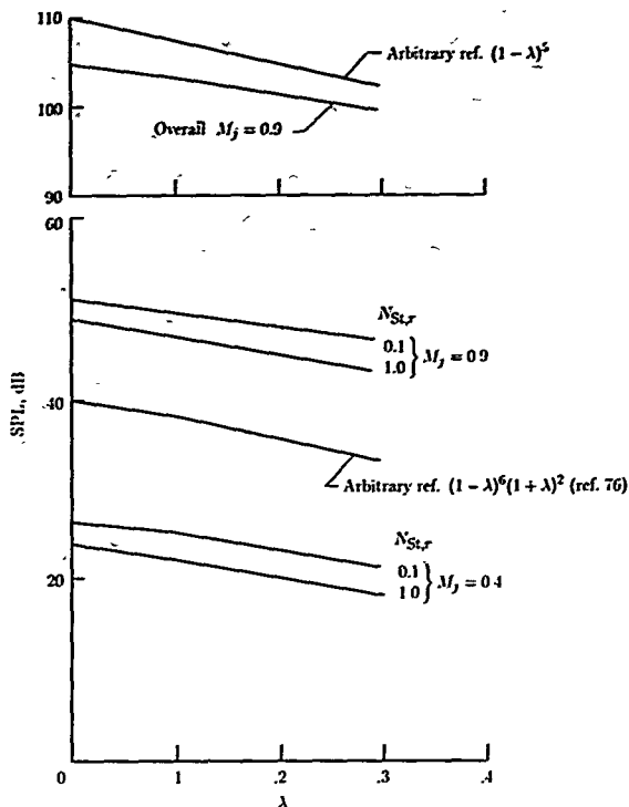
Figure 26. Variation in SPL due to flight effects.
