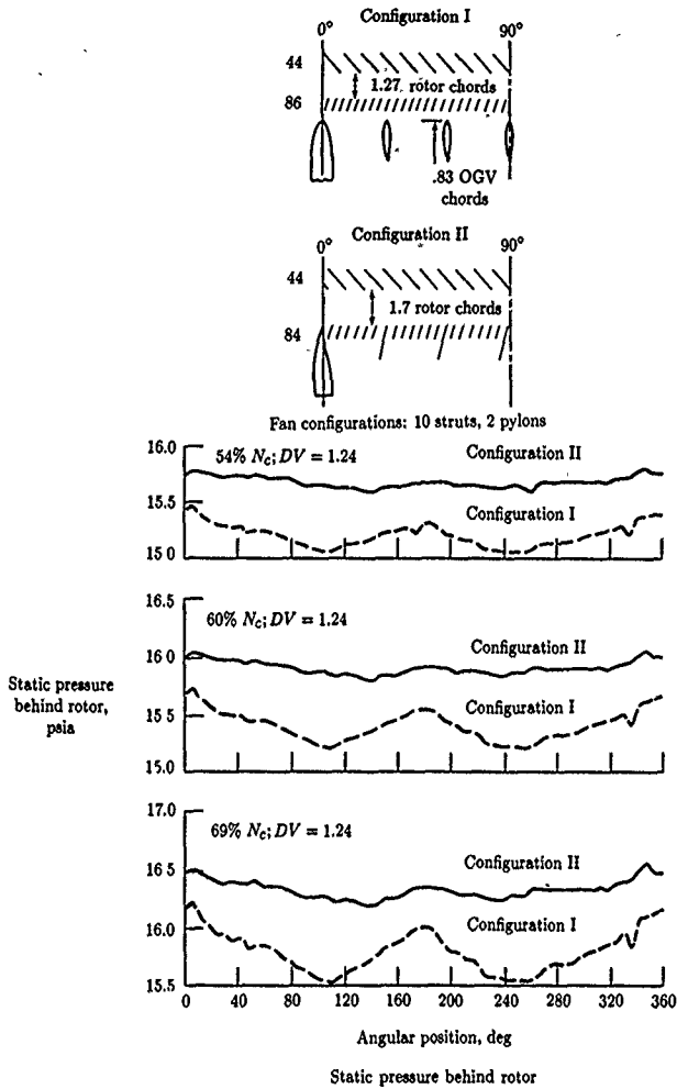
Figure 35. Rotor exit static-pressure distortions for integral vane-strut frame and separate vane-strut frame. (From ref. 56.)
