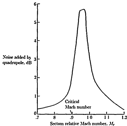
Figure 19. Increase of blade thickness sound pressure level caused by including quadrupole noise. (From ref. 23.)
