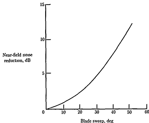
Figure 40. Noise reduction due to blade sweep calculated using frequency-domain method. M_x = 0.8 ; tip speed, 800 ft/sec; 8-bladed propfan; BPF harmonic.
