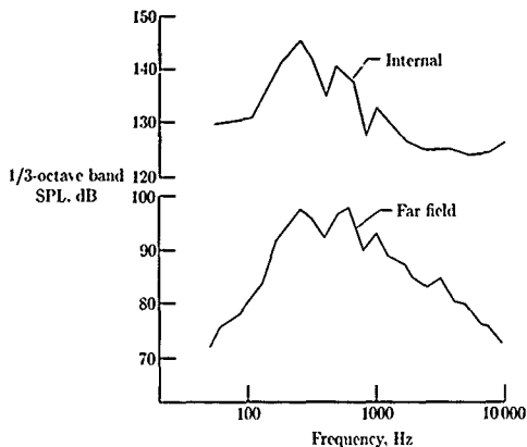
Figure 5. One-third-octave band sound pressure levels measured in a can-type combustor and in its far field. (From ref. 12 Copyright AIAA. Reprinted with permission.)
