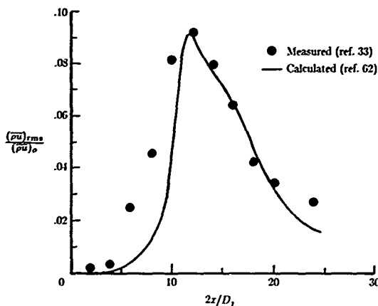
Figure 24. Measured and calculated axial distributions of centerline mass-velocity fluctuation of Mach 2.1 jet excited at N_{St} = 0.4 .
