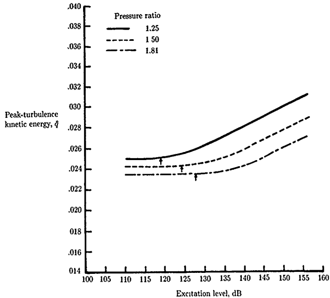
Figure 40. Effect of excitation level and Mach number on peak turbulent kinetic energy for cold jet. Arrows indicate measured threshold levels (ref. 11). N_{St} = 0.5 ; plane wave mode. (From ref. 48.)
