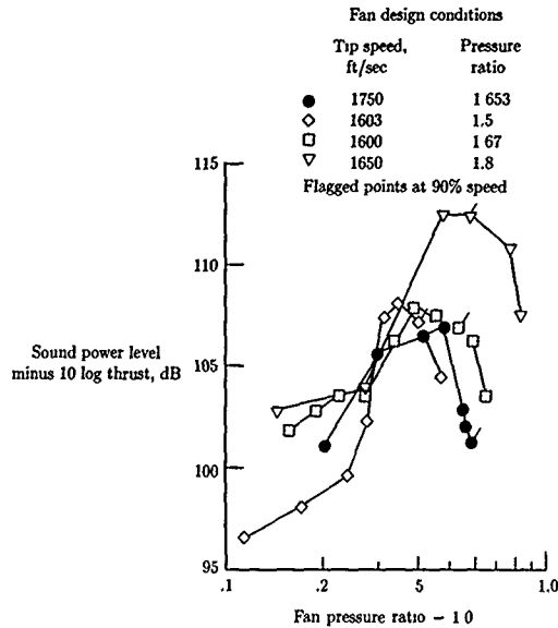
Figure 26. Inlet noise characteristics of high-tip-speed fans. (Based on ref. 86.)
