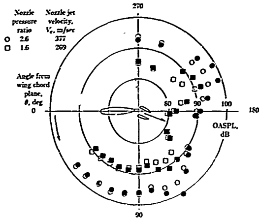
Figure 5. OASPL directivity for augmentor wing at takeoff flap deflection ( 20^\circ ) and zero forward speed. Open symbols denote acoustic treatment; solid symbols denote hard walls. (From ref. 8.)
