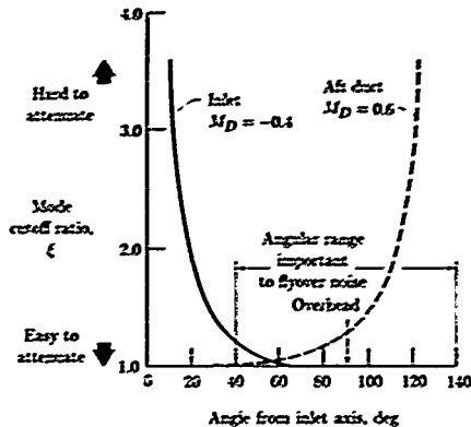
Figure 10. Location of peak sound pressure of single modes. Modes identified by cutoff ratio.
