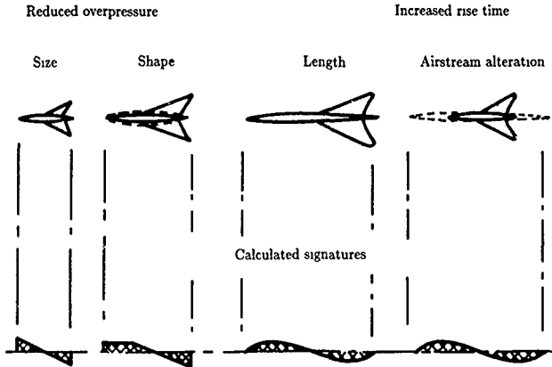
Figure 22. Sonic boom minimization concepts.
