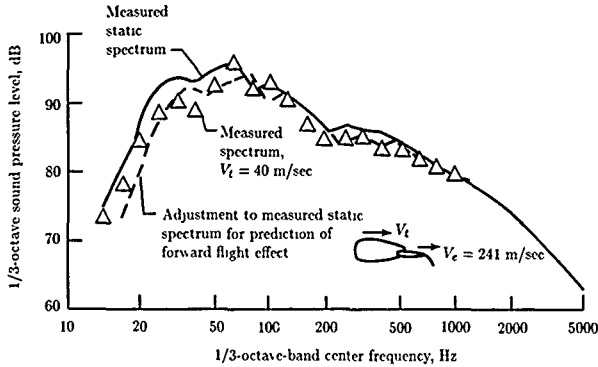
Figure 17. Predicted and measured effect of wind tunnel velocity on 1/3-octave-band spectrum for nominal half-scale USB model at takeoff flap deflection.
