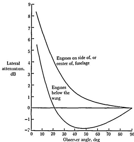
Figure 24. Typical variation of lateral attenuation with observer angle. (From ref. 54)
