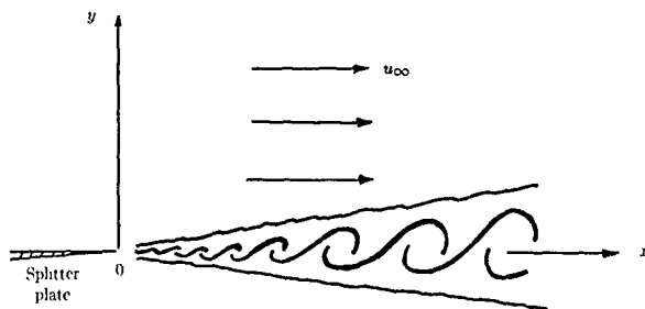
Figure 1. Large turbulence structures in high Reynolds number two-dimensional mixing layer.
