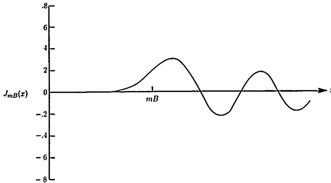
Figure 14. General behavior of Bessel function with order not equal to zero
