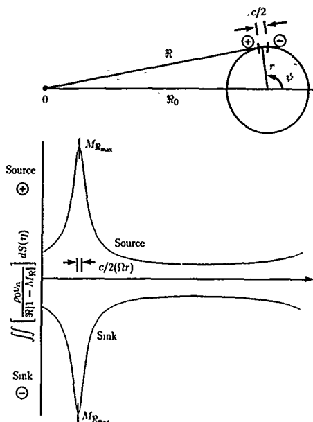
Figure 9. Doppler amplification of simple sources. (From ref. 5.)
