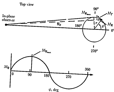
Figure 8. Doppler amplification geometry. R_0/r = 20 ; M_T = 0.8 . (From ref. 5.)
