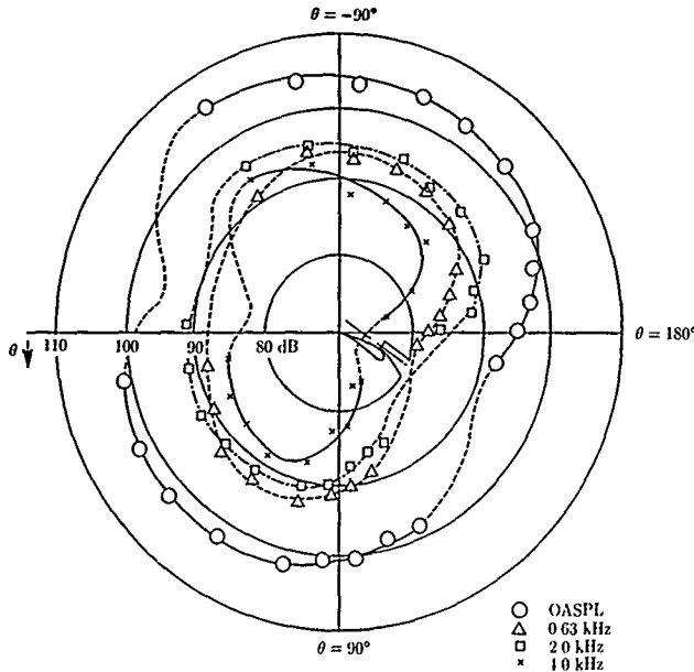
Figure 12. Directivity of isolated blown-flap noise. (From ref. 95.)
