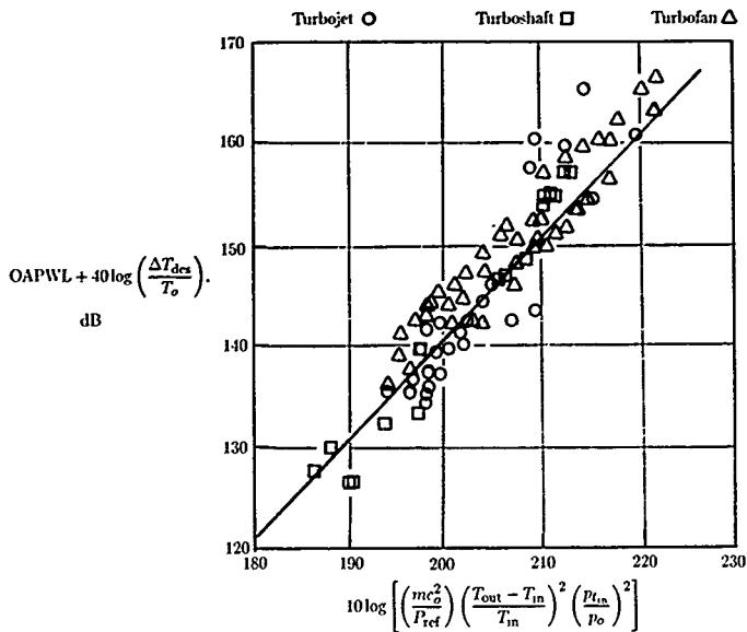
Figure 9. Comparison of the core noise overall sound power level correlation represented by equation (3) with experimental data (From ref. 31. Copyright AIAA. Reprinted with permission.)
