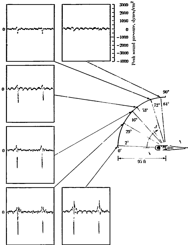
Figure 34. Lateral acoustic directivity for UH-1H in level flight at 115 knots IAS. \alpha = 7^\circ . (From ref. 5.)
