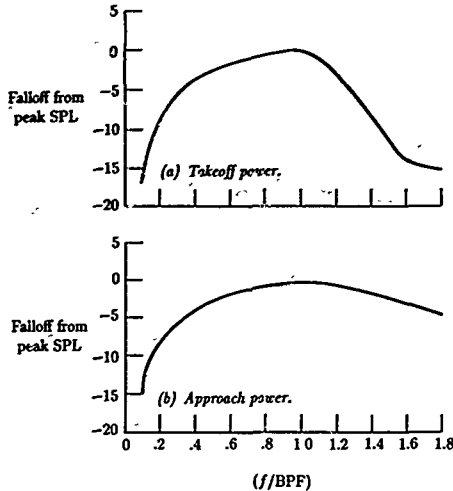
Figure 32. Correlation functions for mean turbine broadband noise spectrum. 120^\circ from inlet; 1/3 -octave band levels. (Based on ref. 90.)
