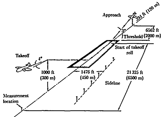
Figure 38. Noise certification measurement locations. (From ref. 72.)
