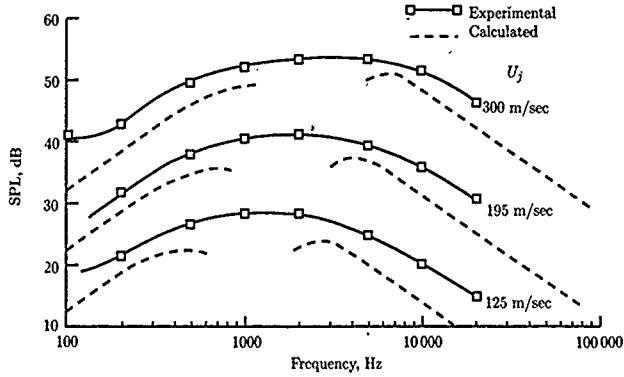
Figure 22. Calculated and experimental (ref. 76) jet noise spectra at \theta = 90^\circ and y_1/D_j = 120 ( D_j = 25 mm).
