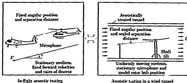
Figure 40. Equivalence between model- and full-scale acoustic testing. (From ref. 31.)
