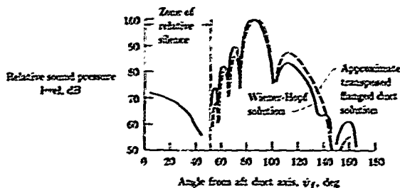
Figure 9. Approximate and exact single-mode aft directivity patterns. (8,4) mode; M_D = 0.6 ; M_{\infty} = 0 ; \eta = 7.11 . (From ref. 32.)
