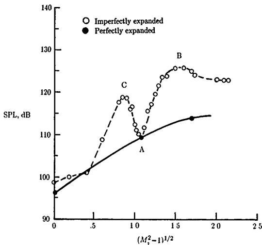
Figure 11. Overall sound pressure level at 150° angle to jet axis. M_d = 1.5 . (Based on ref. 80.)
