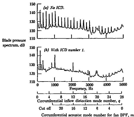
Figure 14. Narrow-band blade pressure spectra. Pressure side transducer 1.9 cm from tip; JT15D engine; fan speed, 10 500 rpm. (From ref. 38.)
