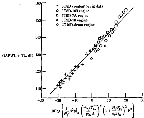
Figure 12. Comparison of core noise overall sound power level correlation represented by equation (4) with experimental data. (From ref. 32. Copyright AIAA. Reprinted with permission.)
