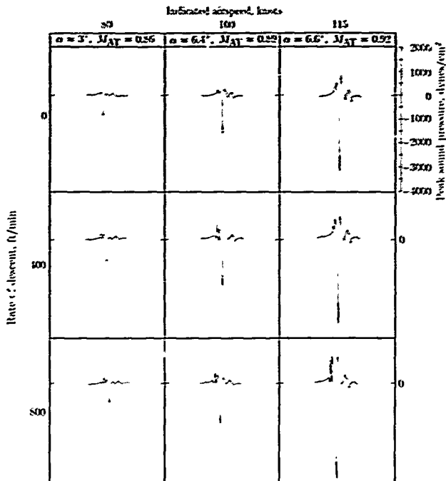
Figure 32. Averaged acoustic signature of UH-1H impulsive noise for 1/2 revolution versus forward airspeed and rate of descent. (From ref. 5.)
