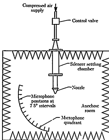
Figure 27. Anechoic jet noise facility. (From ref. 76.)
