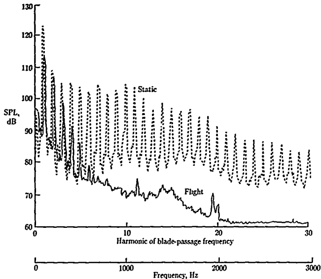
Figure 26. Effect of forward flight on propeller noise. (From ref. 59.)
