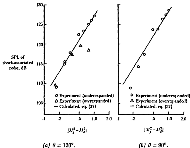
Figure 30. Broadband shock-associated noise SPL scaling. M_d = 1.67 . T_r/T_\infty = 2.0 . (From ref. 81.)
