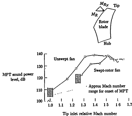
Figure 25. Effect of rotor leading-edge sweep on multiple pure tone generation. (Based on ref. 85.)
