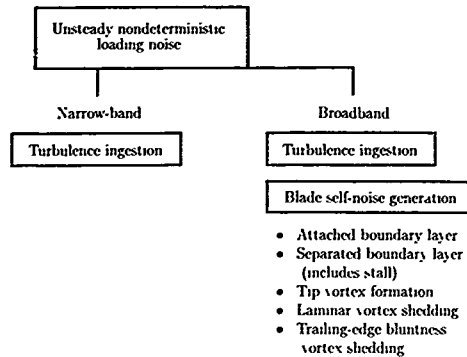
Figure 24. Categorization of helicopter rotor broadband noise. (Based on ref. 19.)
