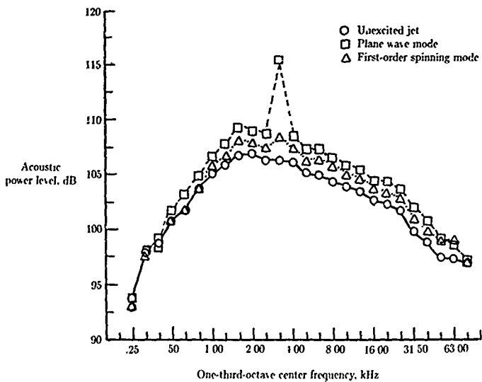
Figure 37. Spectra showing noise amplification by tone excitation. M_j = 0.78 ; u_j = 250 m/sec; N_{St} = 0.63 ; Excitation level = 136 dB. (From ref. 151.)
