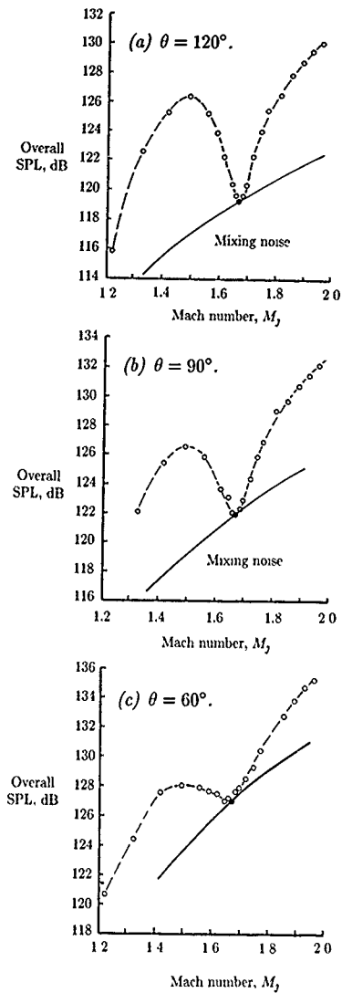
Figure 12. Shock-associated and turbulent mixing noise components for convergent-divergent nozzle operated with T_j/T_0 = 1.0 . (Based on ref. 81.)
