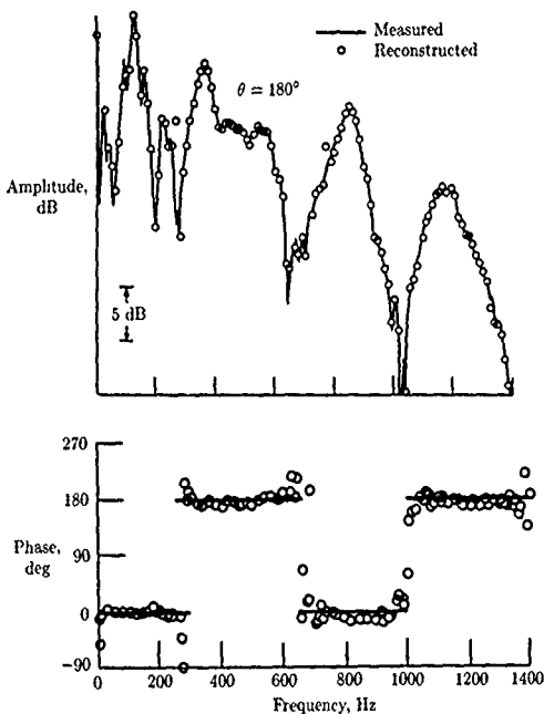
Figure 18. Measured and reconstructed cross-spectra between two waveguide probes in an annular gas turbine combustor. (From ref. 36.)
