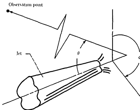
Figure 3 Coordinates for observation point.
