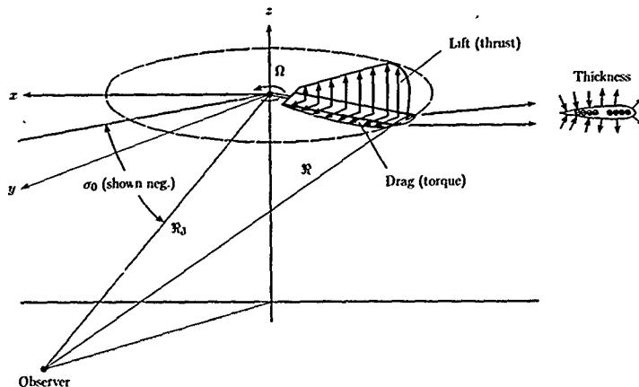
Figure 4. Geometry of simple hovering rotor.
