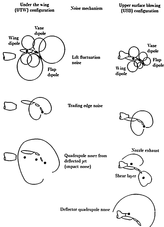
Figure 8. Sketch of directivity patterns for different assumed mechanisms of externally blown flap noise. (From ref. 18.)
