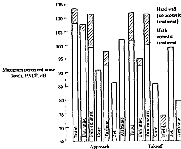
Figure 2. Component flyover noise levels for advanced turbofan. (From ref. 1.)
