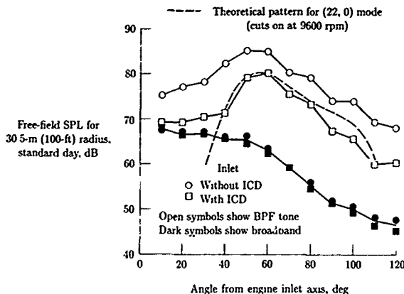
Figure 15. Directivity pattern indicating presence of 22-lobed acoustic mode due to rotor-strut interaction. JT15D fan; fan speed, 10 500 rpm. (Based on ref. 30.)
