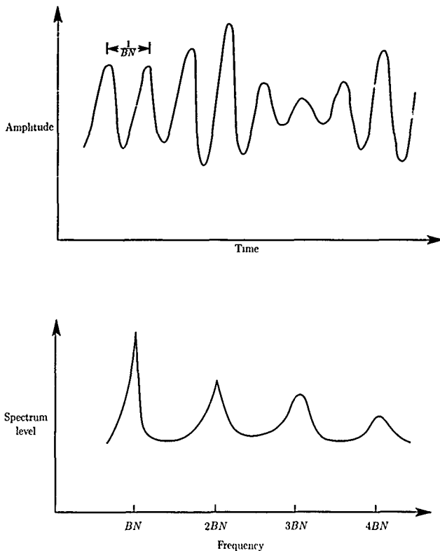
Figure 6. Characteristics of propeller narrow-band random noise.
