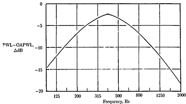
Figure 10. Universal gas turbine combustion noise spectral shape. (From ref. 31. Copyright AIAA. Reprinted with permission.)
