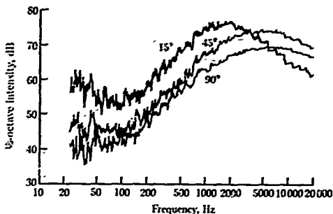
Figure 24. Jet noise spectra at \theta = 15^\circ , 45^\circ , and 90^\circ . U_j = 195 m/sec. (From ref. 76.)
