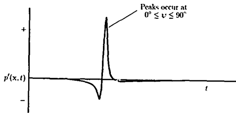
Figure 21. Acoustic pressure signature of advancing BVI.
