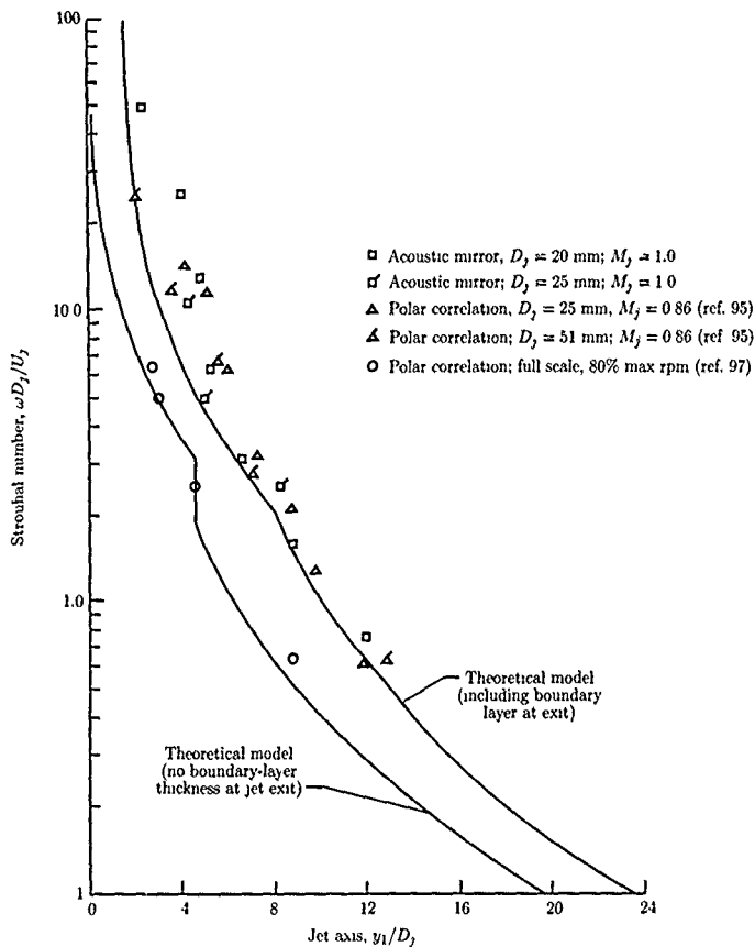
Figure 29. Calculated and measured peak source strength locations.
