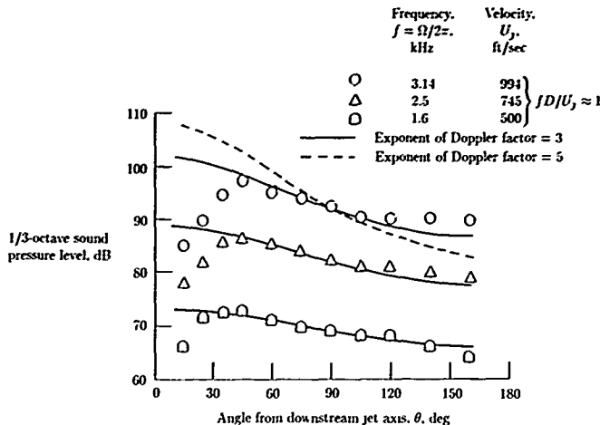
Figure 7. Experimental 1/3-octave directivity data of Olsen and Friedman (ref. 51) plotted at constant source frequency \Omega , where \Omega/2\pi is equal to peak frequency of spectrum at 90^\circ from jet axis.
