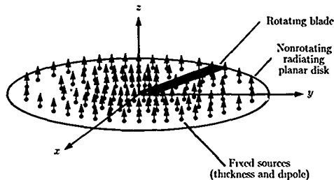
Figure 5. Fixed-space representation of classical thickness and loading acoustic sources.
