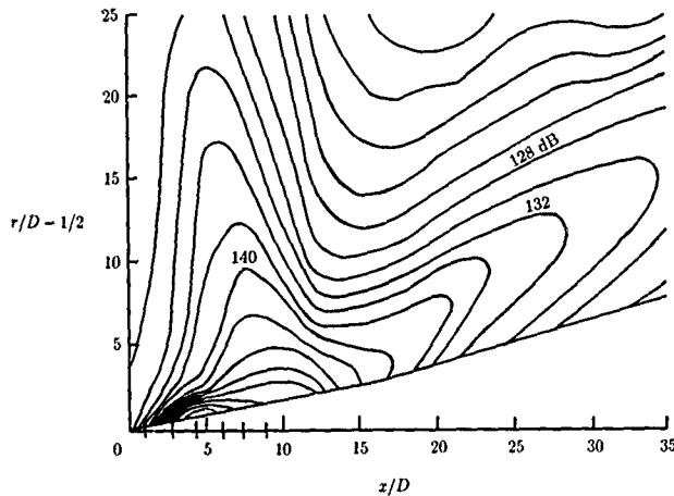
Figure 10. Near-field 1/3-octave-band sound-pressure-level contours of Mach 1.50 supersonic jet at 20-kHz center frequency. M_j = 1.67 . (From ref. 74.)
