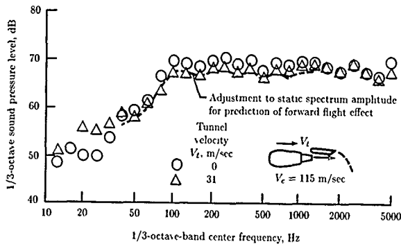
Figure 16. Predicted and measured effect of wind tunnel velocity on 1/3-octave-band spectrum for nominal half-scale UTW model at approach flap deflection.
