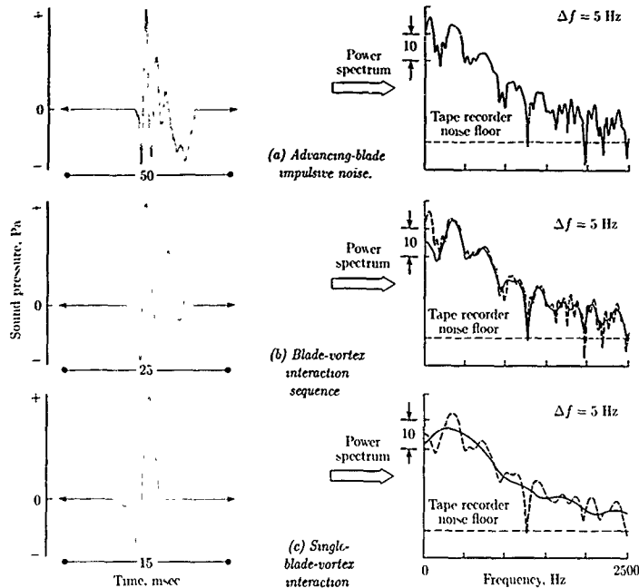
Figure 37. Time windowing of impulsive noise. (From ref. 26.)
