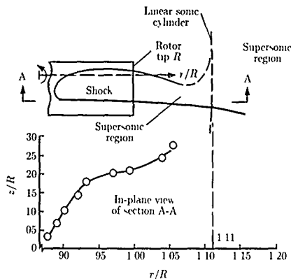
Figure 52. Top and aft views of shock boundaries of rotor and development of delocalization phenomenon at M_T = 0.90 . (From ref. 41.)
