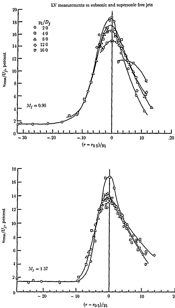
Figure 12. Variation of u_{rms}/U_j across jet at different distances from jet exit at jet Mach numbers of 0.90 and 1.37. (From ref. 71.)
