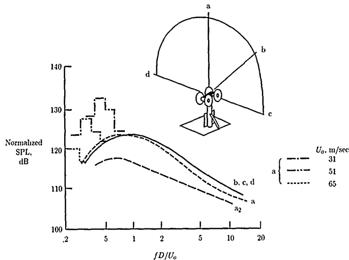
Figure 10. Normalized main gear model spectra at four measurement points. a_2 is spectrum of simplified two-wheel model at point a. Reference flight speed, 100 m/sec. (From ref. 77.)
