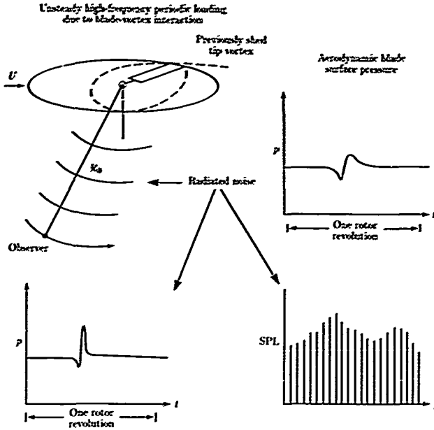
Figure 14. Contribution of high-frequency airloads (impulsive events) to helicopter rotor noise.
