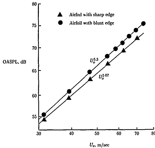
Figure 4. Overall sound pressure level of trailing-edge noise as a function of free-stream velocity U_0 . \alpha = 90^\circ (flyover plane); \Theta = 90^\circ . (From ref. 56.)
