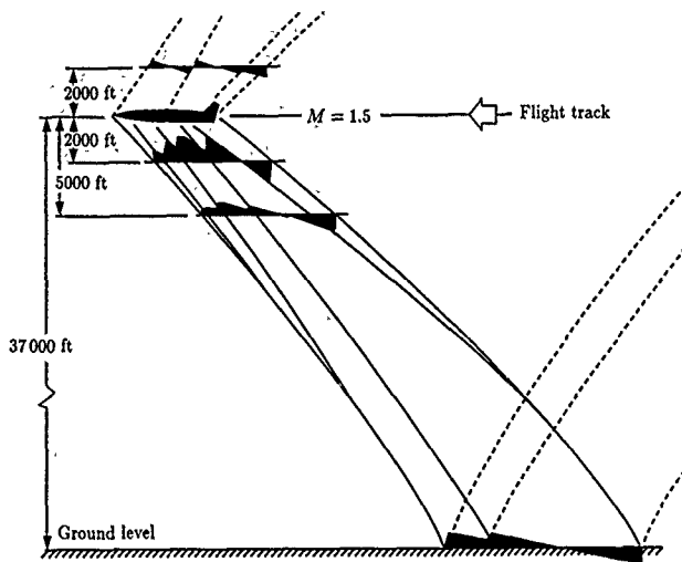
Figure 2. Measured signatures above and below XB-70 aircraft.
