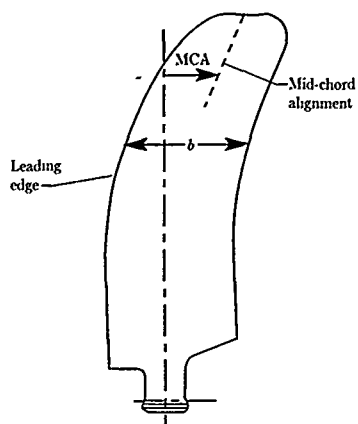
Figure 11. Blade planform defining chord b and mid-chord alignment (sweep).
