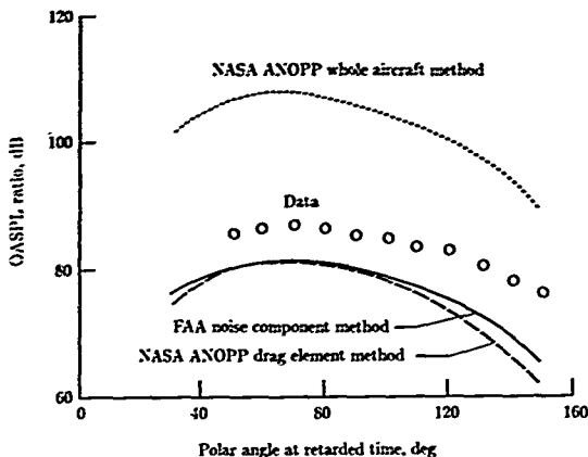
Figure 20. Comparison of measured and predicted OASPL directivity for Convair F-106B. (From ref. 27.)
