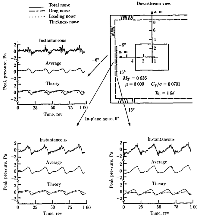
Figure 44. Measurements and predictions of isolated hover noise of model rotor.
