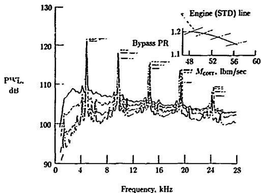
Figure 16. Variation of broadband levels with fan operating point. JT15D fan in anechoic chamber; \Delta f = 80 Hz; fan speed, 10 500 rpm.
