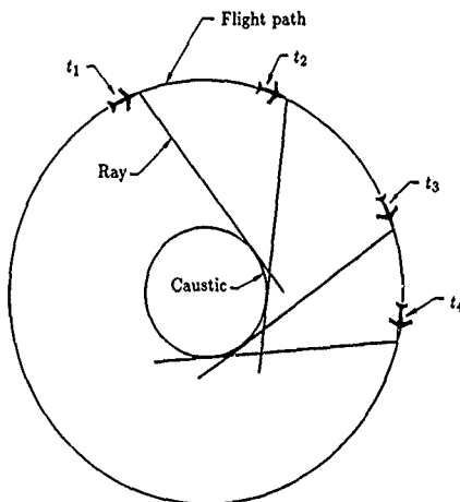
Figure 12. Focusing due to sonic cutoff and in-plane steady turn.
