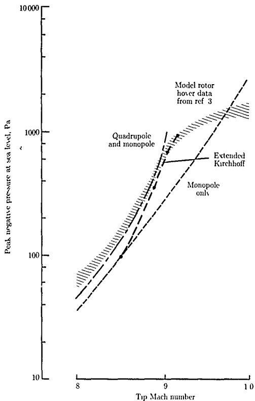
Figure 56. Theoretical and experimental pressures for rotor in hover. R_0/R = 3.0 . (Based on ref. 5)
