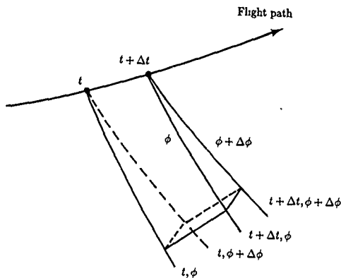
Figure 9. Ray tube outlined by four corner rays \Delta t and \Delta\phi apart.
