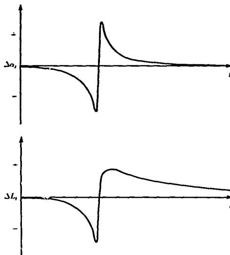
Figure 19. Changes in angle of attack \alpha_i and section lift L_i due to two-dimensional BVI. (From ref. 18.)
