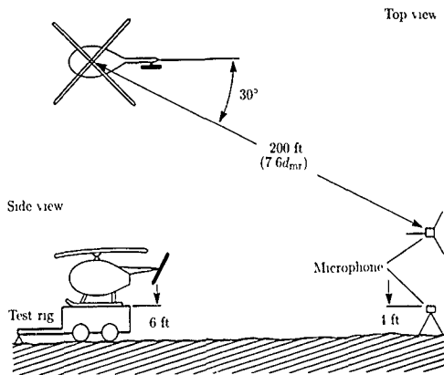
Figure 26 Microphone height and location relative to OH-6A test helicopter mounted on special test rig. (From ref 24.)
