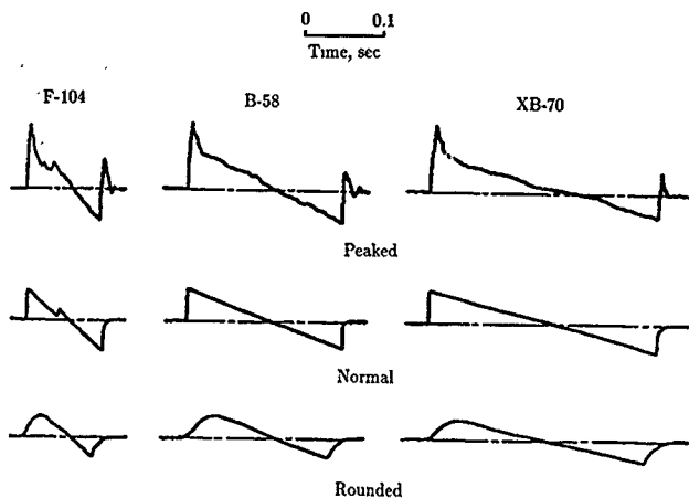
Figure 5. Variation of measured sonic boom waveforms at ground level for small, medium, and large aircraft in steady, level flight.
