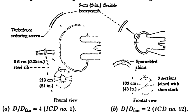
Figure 12. Inflow control devices for flight fan noise simulation. (From ref. 40.)
