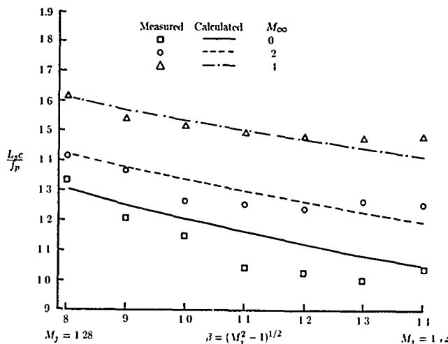
Figure 31. Effects of forward flight on peak frequency of broadband shock-associated noise. \psi = 90^\circ . (Based on ref. 103.)
