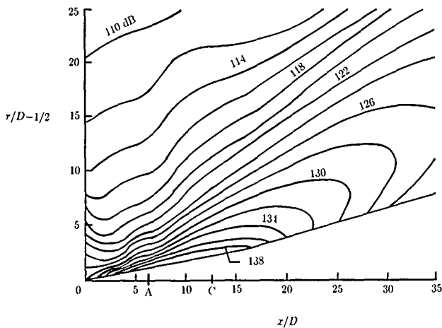
Figure 8. Near-field 1/3-octave-band sound-pressure-level contours of Mach 1.50 supersonic jet at 10-kHz center frequency. (From ref. 74.)
