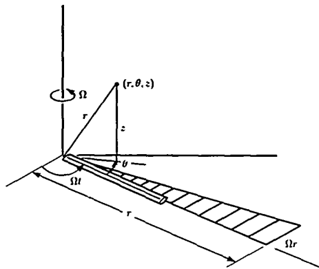
Figure 49. Cylindrical coordinate system of hovering rotor. (From ref. 5.)
