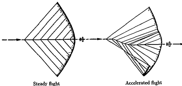
Figure 19. Shock wave ground-intersection patterns for aircraft in steady and accelerated flight at constant altitude. (From ref. 57.)
