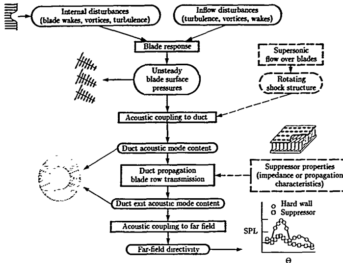
Figure 4. Turbomachinery noise-generation processes.
