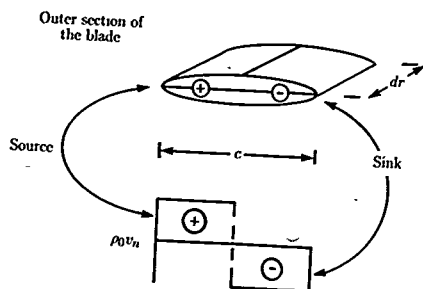
Figure 7. Simple source and sink representation of blade thickness noise. (From ref. 5.)
