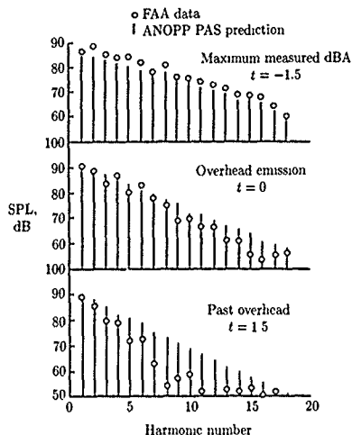
Figure 32. Measured and predicted noise spectra at three time periods for standard takeoff of Piper Lance airplane. (From ref. 67.)
