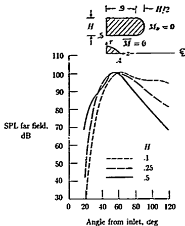
Figure 8. Effect of inlet lip thickness on single-mode directivity. M_D = 0 ; 3150 Hz; (13,0) mode; theory normalized to 100 dB at 60^\circ . (From ref. 31.)
