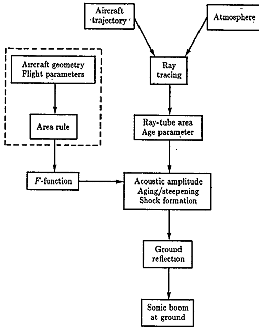
Figure 10. Logical flow of sonic boom calculation.
