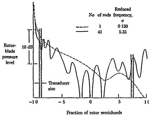
Figure 23. Calculated chordwise variation of fundamental component of rotor-blade pressure levels generated by wakes from upstream rods.
