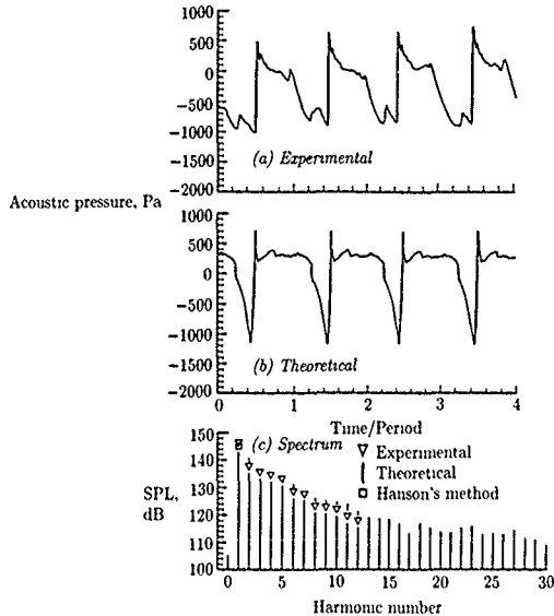
Figure 30. Measured and predicted acoustic pressure signatures and spectrum for boom microphone behind propeller disk. Boom reflection correction included. Period, 0.991 msec; BPF = 1009.2 Hz (From ref. 10)
