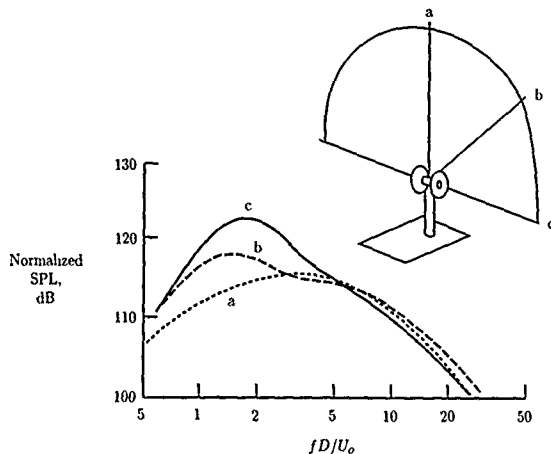
Figure 9. Normalized nose gear model spectra at three measurement points. Reference flight speed, 100 m/sec. (From ref. 77.)
