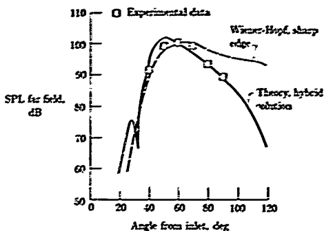
Figure 7. Theoretical and experimental single-mode inlet directivity. 3150 Hz; (13,0) mode; fan speed. 6750 rpm. (From ref. 31.)
