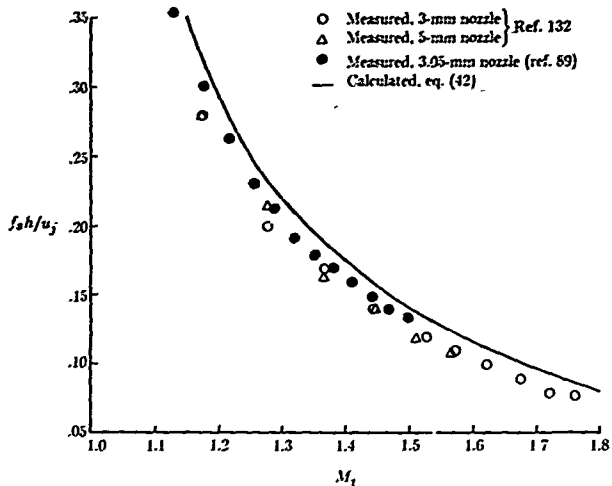
Figure 36. Measured and calculated screech tone frequencies of rectangular supersonic jets.
