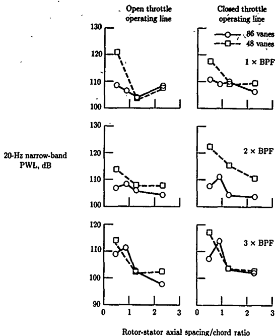
Figure 33. Tone PWL as function of spacing trends at subsonic tip speed (293 m/sec (960 ft/sec)) for single-stage fan. (From ref. 83.)
