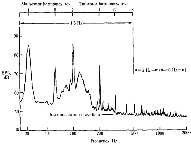
Figure 28. Narrow-band spectrum plot for complete OH-6A helicopter in simulated hover (From ref 24.)
