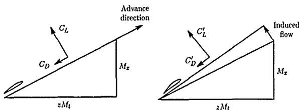
Figure 18. Reference axes for lift and drag definition.
