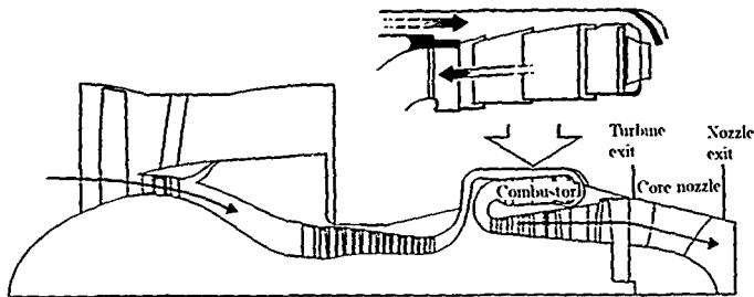
Figure 3. Cutaway view of turbofan engine showing the combustor, turbine exit, and core nozzle. (From ref. 5.)
