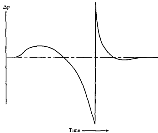
Figure 25. Character of transonic boom signature.
