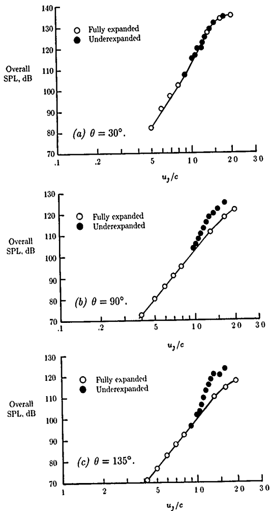
Figure 9. Overall sound pressure level of broadband shock-associated noise. T_j/T_0 = 1.0 . (From part II of ref. 76.)
