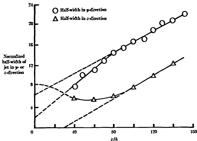
Figure 34. Growth of rectangular jet with downstream distance. Pressure ratio = 3.8; Aspect ratio = 16.7. (From ref. 132.)
