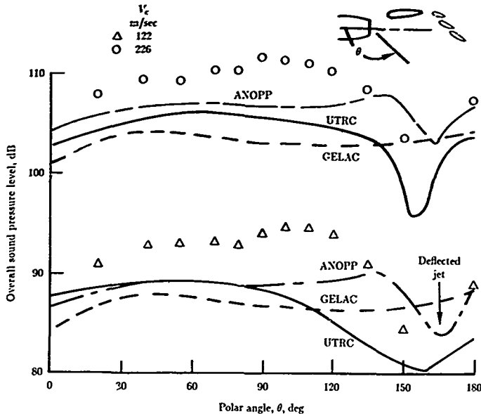
Figure 11. Predicted and measured OASPL directivity in flyover plane for three-flap UTW model at takeoff flap deflection. (From ref. 18.)
