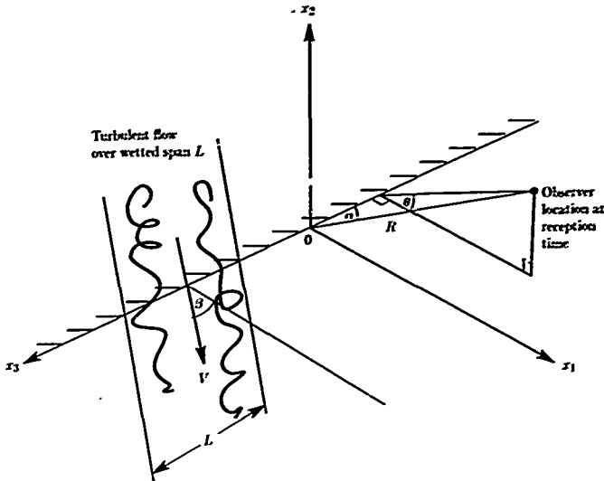
Figure 2. Turbulent flow over a wetted span L of a trailing edge. The observer has coordinates (R, \theta, \alpha) at reception time.
