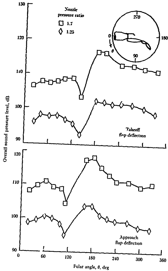
Figure 4. OASPL directivity in flyover plane for a small USB mode: with a D-shaped exhaust nozzle and jet deflector, at takeoff and approach flap deflections and zero flight speed.
