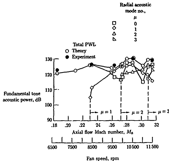
Figure 21. Relationship of speed and inlet fundamental tone acoustic power generated by 41 rod wakes interacting with JT15D fan. (From ref. 76.)
