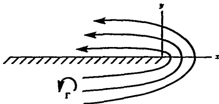
(a) Geometry of flow round side edge of a flap; lines give the streamlines of the main edge flow which are cut by a vortex \Gamma .
