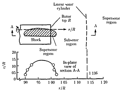
Figure 51. Top and aft views of shock boundaries of rotor at M_T = 0.88 (From ref. 41)
