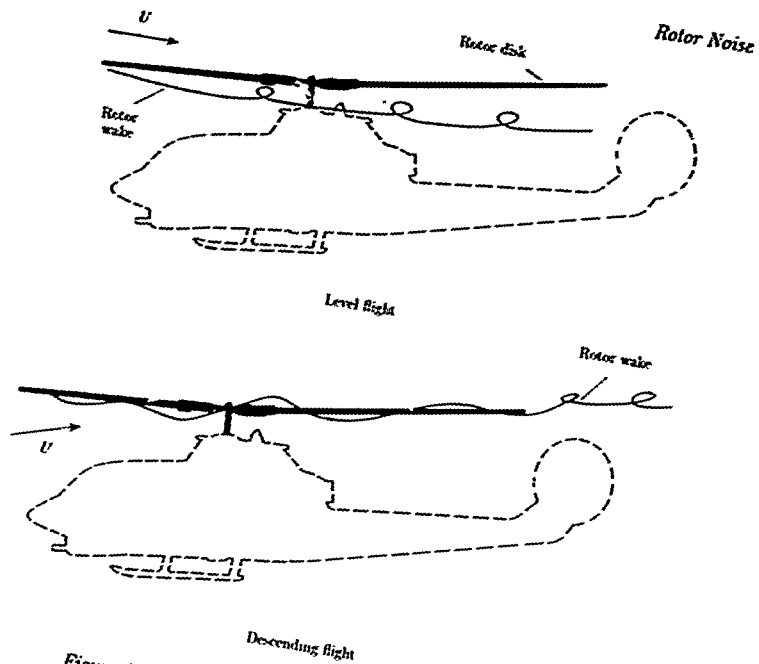
Figure 16. Flight-path effects on BVI noise. (From ref. 5.)
