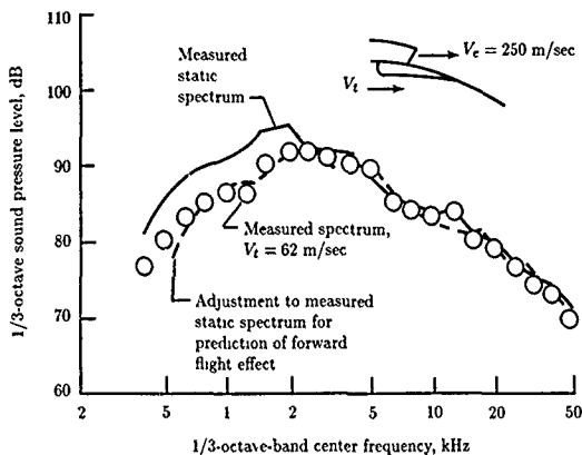
Figure 18. Predicted and measured effect of wind tunnel velocity on 1/3-octave-band spectrum for a USB configuration at takeoff flap deflection.
