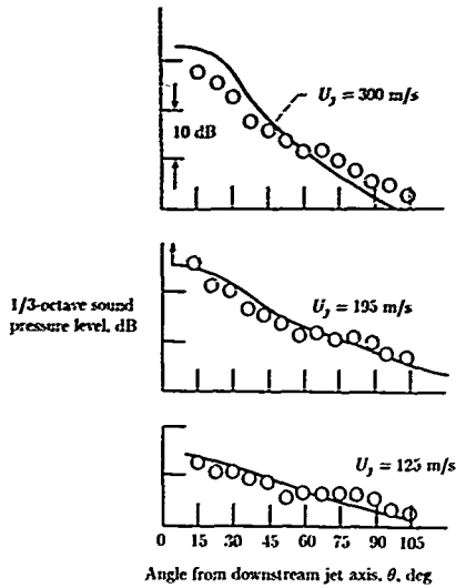
Figure 6. Comparisons of Mani's (ref. 44) analysis with the 1/3-octave directivity data of Lush (ref. 3) for source Strouhal number \Omega D/2\pi U_j = 0.03 .
