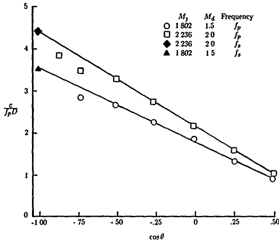
Figure 32. Screech tone frequency as limit of peak frequency of broadband shock-associated noise. (From ref. 73.)
