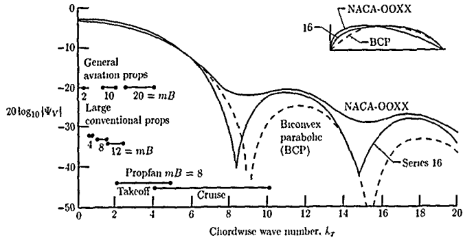
Figure 15. Reduction of thickness noise from blade element due to chordwise noncompactness. (From ref. 17.)
