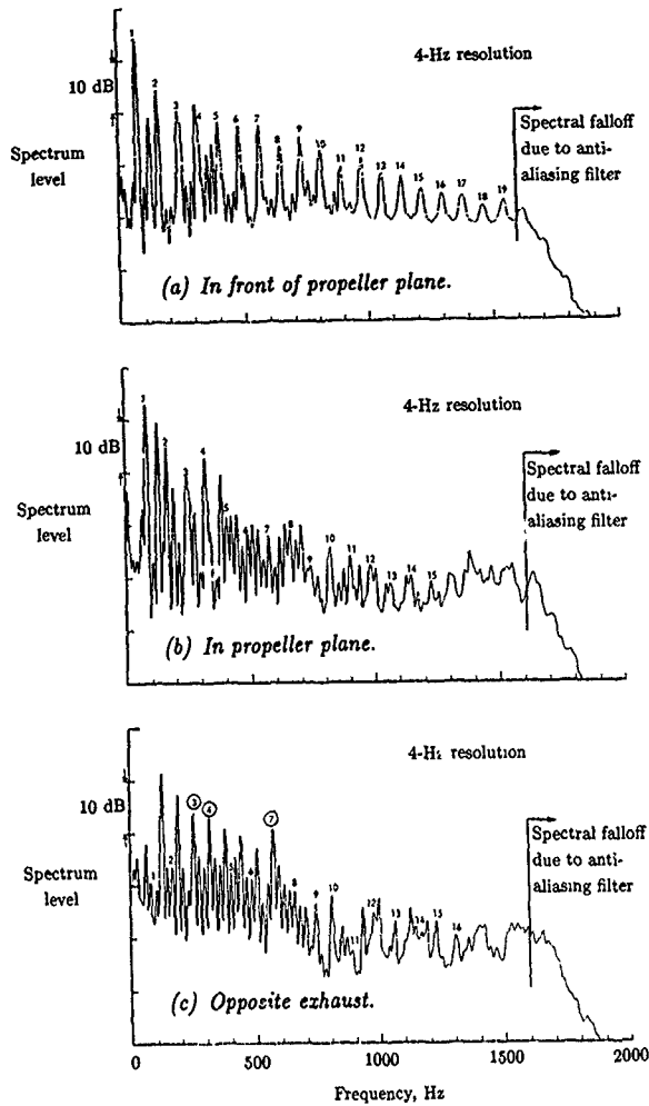
Figure 22. Sound pressure spectra showing propeller and exhaust noise on the fuselage of a reciprocating-engine powered airplane. Circled numbers indicate data heavily contaminated by exhaust tones. (From ref. 38.)
