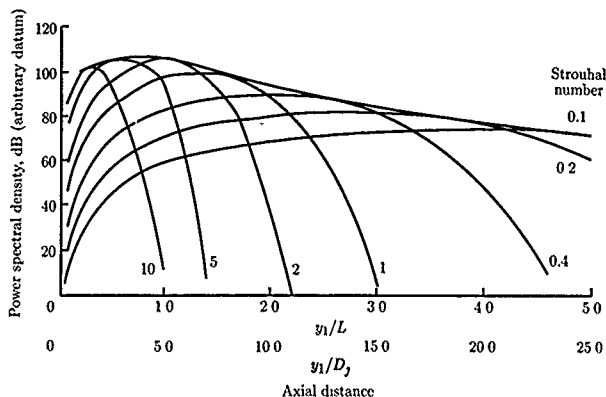
Figure 20. Jet noise effective source distribution at low Mach numbers for constant Strouhal number.
