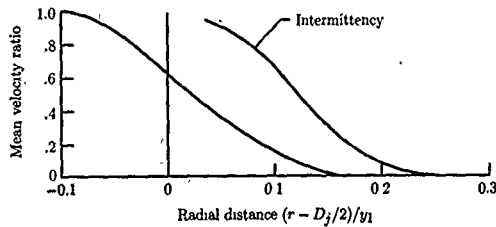
Figure 13. Variation of intermittency factor across mixing region of jet. (From ref. 31.)
