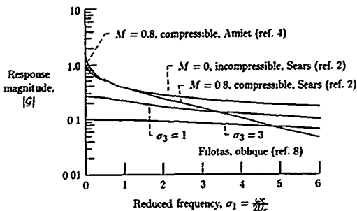
Figure 5. Airfoil gust response functions for single airfoil.
