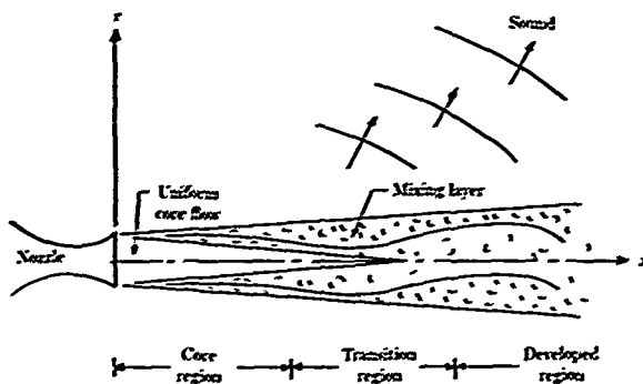
Figure 23. Instability waves and their sound field for axisymmetric jet.
