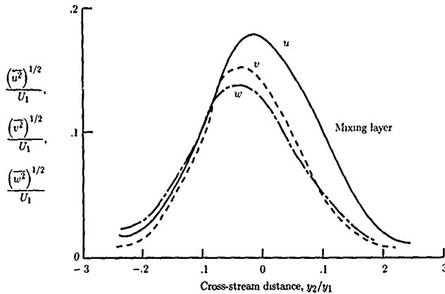
Figure 14. Variation of turbulence velocity components across mixing region of jet. (From ref. 31.)
