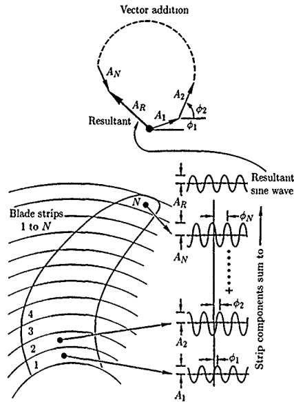
Figure 17. Conceptual benefit of blade sweep for reducing noise. (From ref. 17.)
