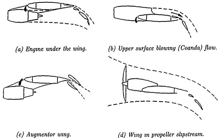
Figure 1. Types of propulsive lift STOL configurations. (Based on ref. 32.)
