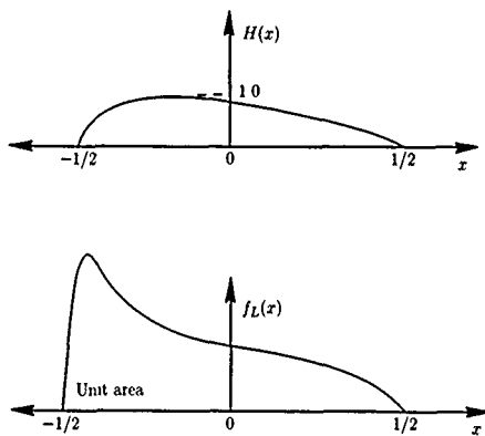
Figure 12. Shape functions for chordwise distributions of thickness and loading.
