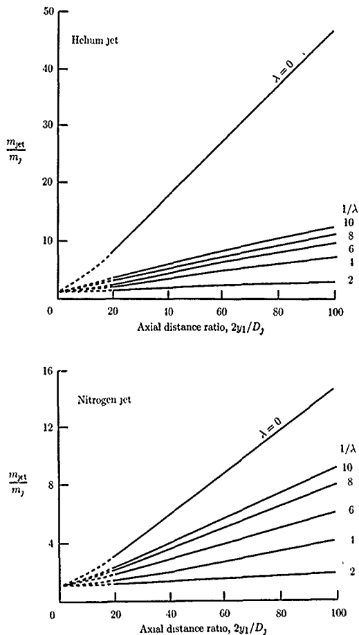
Figure 15. Ratio of mass flux in jet to exit mass flux. (From ref. 72.)
