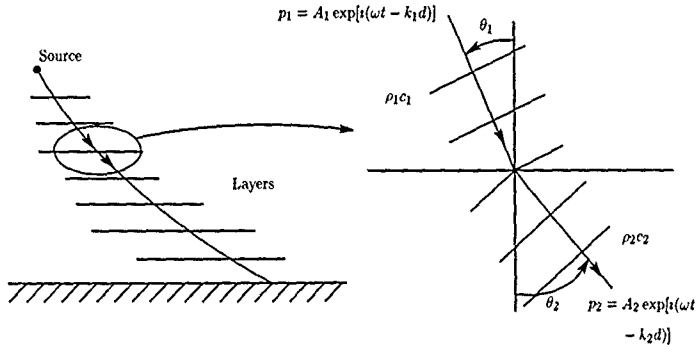
Figure 20. Refraction of acoustic wave.
