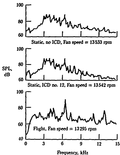
Figure 17. Supersonic tip speed noise spectra. JT15D engine; \Theta = 70^\circ . (From ref. 40.)
