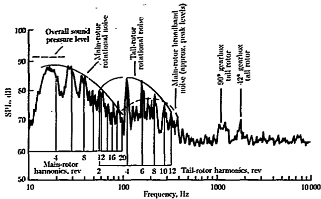
Figure 3. External noise spectrum of UH-1A. (Based on ref. 8.)
