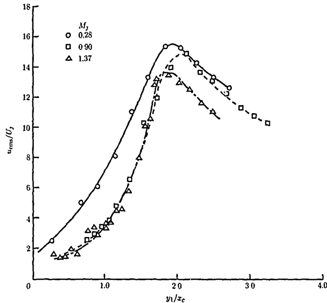
Figure 16. Variation of u_{rms}/U_j along centerline of jet at three Mach numbers. (From ref. 71.)
