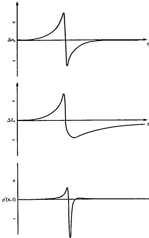
Figure 23. Angle-of-attack, lift, and acoustic pressure time histories of retreating BVI.
