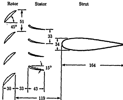
(a) Rotor-stator-strut cross section. All dimensions are in millimeters unless otherwise indicated.
