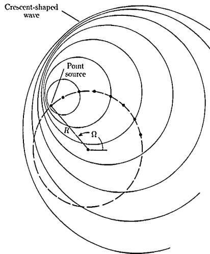
Figure 45. Linear wave amplification (Doppler effects) of rotating point source. M_T = 0.9 . (From ref. 5.)
