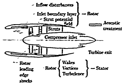
Figure 1. Schematic cross section of turbofan engine with turbomachinery noise-generating mechanisms.
