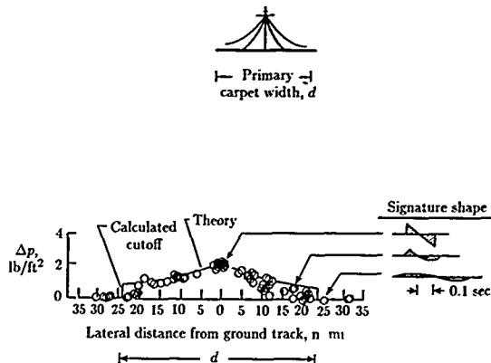
Figure 16. Sonic boom overpressures for XB-70 aircraft at an altitude of 60 000 ft as function of lateral distance. M \approx 2.0 .
