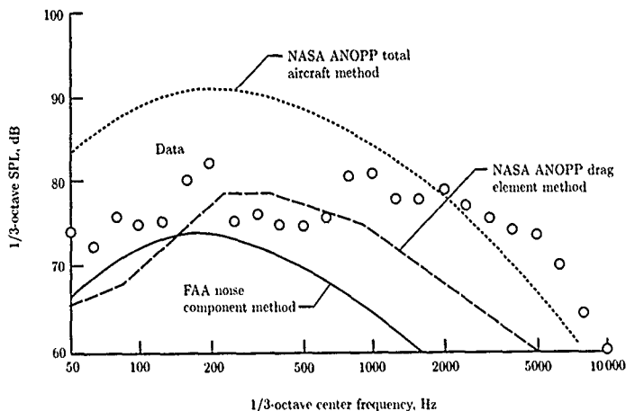
Figure 16. Comparison of measured and predicted flyover noise spectra for Boeing 747 in clean configuration at 253 knots. (From ref. 27.)
