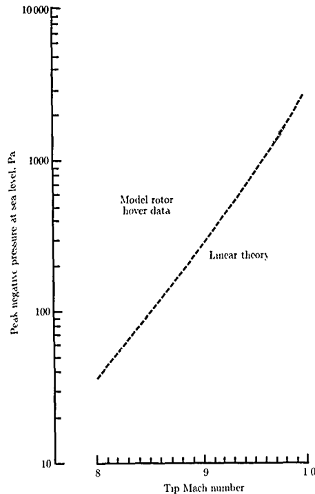
Figure 47. Theoretical and experimental peak pressures of rotor in hover. In-plane microphone; R_0/R = 3.0 . (From ref. 40.)
