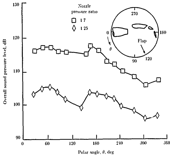
Figure 3. OASPL directivity in flyover plane for a small UTW model at approach flap deflection ( 60^\circ ) and zero flight speed.
