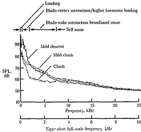
Figure 39. Typical overhead noise spectra of 2/5-scale BO-105 model rotor. (Based on ref. 21)
