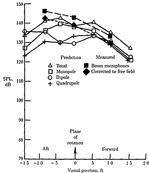
Figure 28. Measured and predicted BPF tone sideline directivity for SR-3 operating at design point condition. (From ref 66.)
