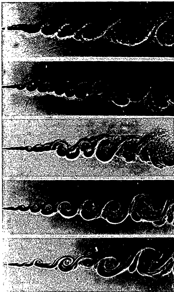
Figure 9. Flow visualization in mixing layer with density ratio of 7 at low Mach numbers. (From ref. 62.)
