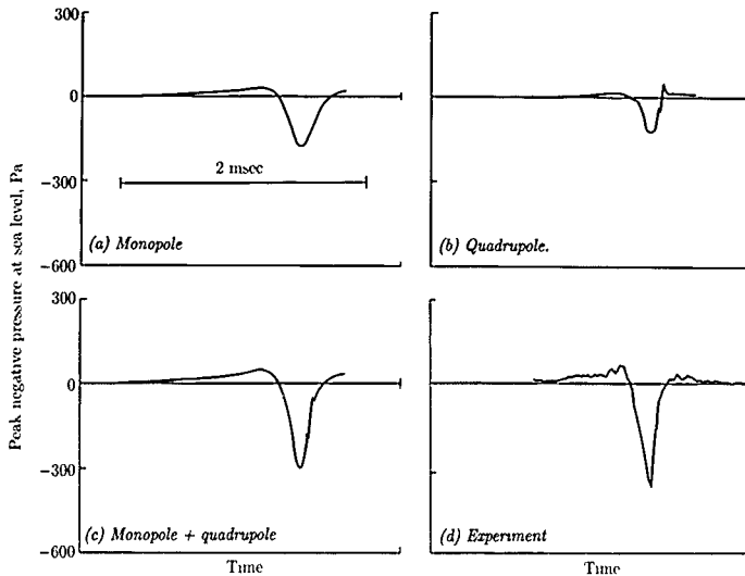
Figure 54. Theoretical and experimental time histories at M_T = 0.88 , R_0/R = 3.0 . (From ref 5.)
