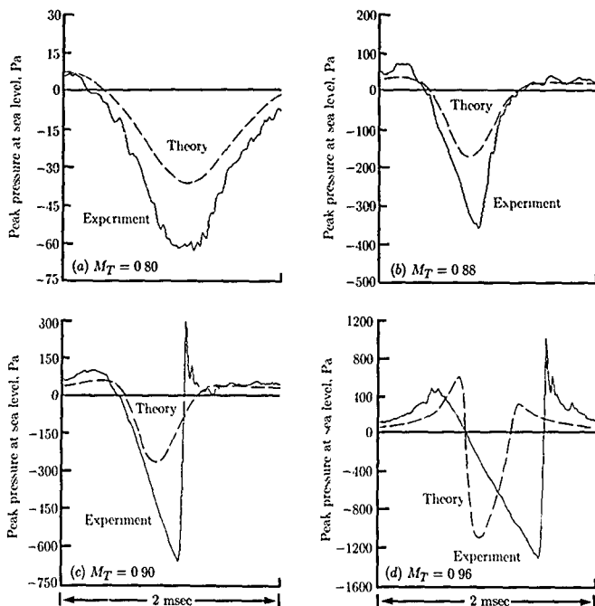
Figure 46. Theoretical and experimental pressure time histories for in-plane microphone. R_0/R = 3.0 . (From ref 40.)
