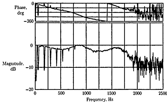
Figure 16. Magnitude and phase of transfer function of a typical 8-in. (20-cm) waveguide probe with 60-ft (18-m) coil.
