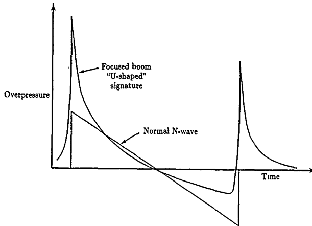
Figure 13. Focused and unfocused boom signatures.
