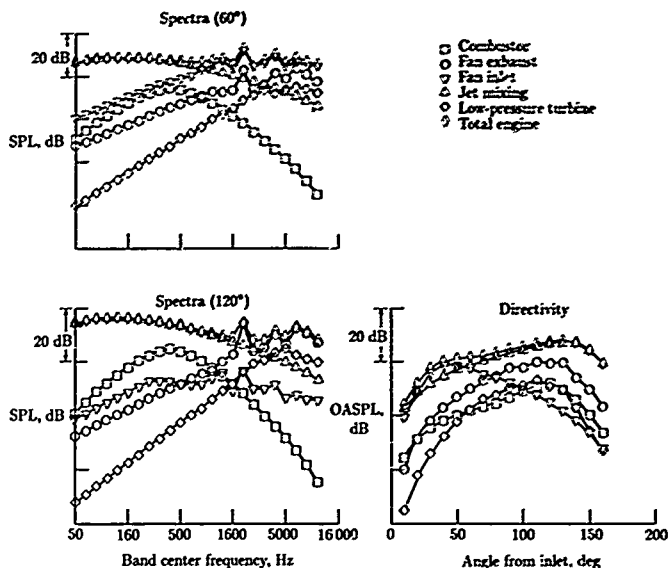
Figure 29. Typical turbofan engine component noise source contributions at takeoff power.
