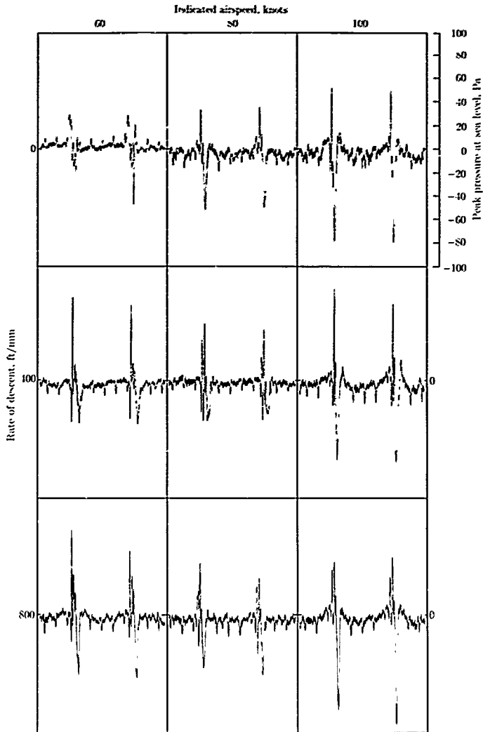
Figure 35. Unaveraged acoustic signatures of UH-1H as function of forward airspeed and rate of descent. (From ref. 5.)
