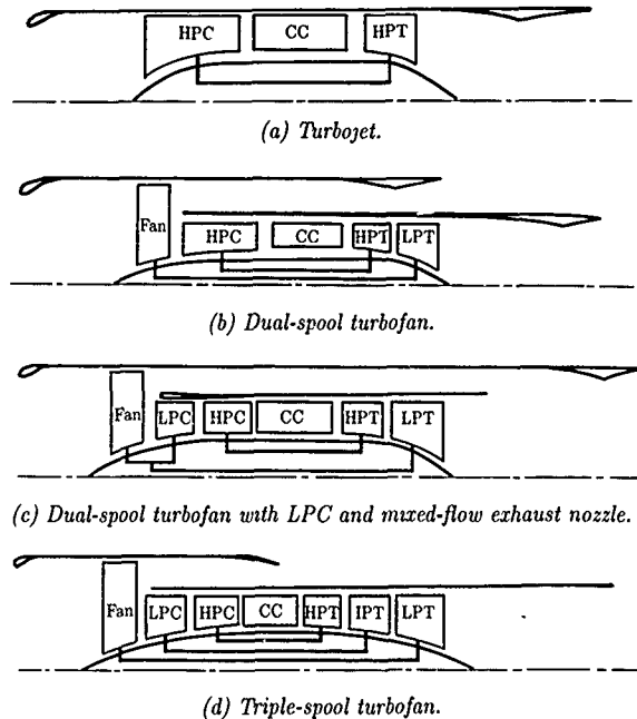
Figure 27. Typical turbojet-turbofan engine schematic arrangements.
