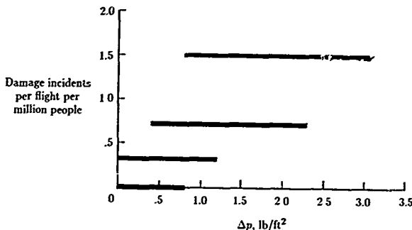
Figure 29. Sonic-boom-induced incidents for various overpressure ranges.
