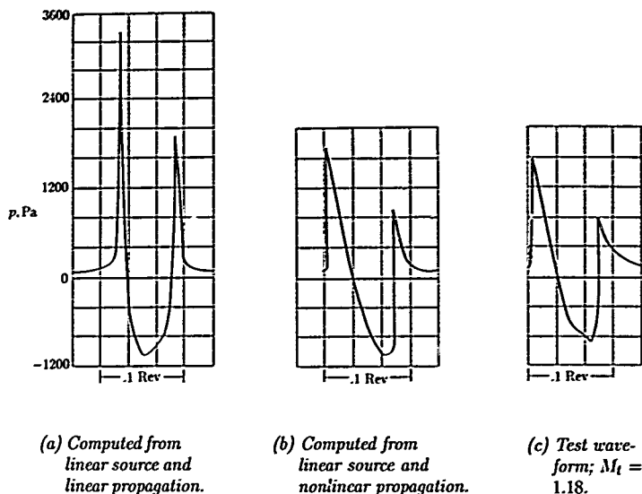
Figure 25. Nonlinear propagation effects computed from weak shock theory. (From ref. 56.)
