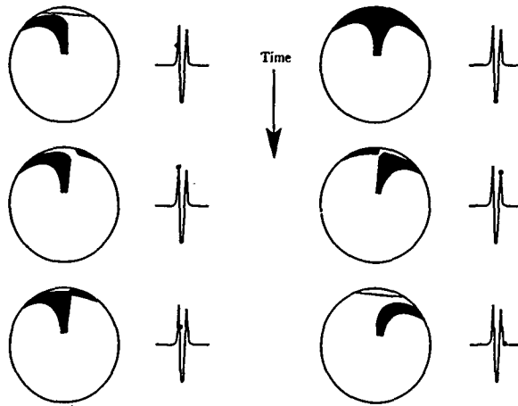
Figure 10. Evolution of acoustic planform with time at M_t = 1.1 . (From ref. 11.)
