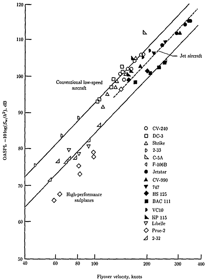
Figure 13. Airframe noise (maximum OASPL for clean configuration at flyover altitude h ) normalized for wing area S_w as suggested by trailing-edge noise theory. Solid lines correspond to the U_0^5 variation predicted by trailing-edge noise theory. (From ref. 27.)
