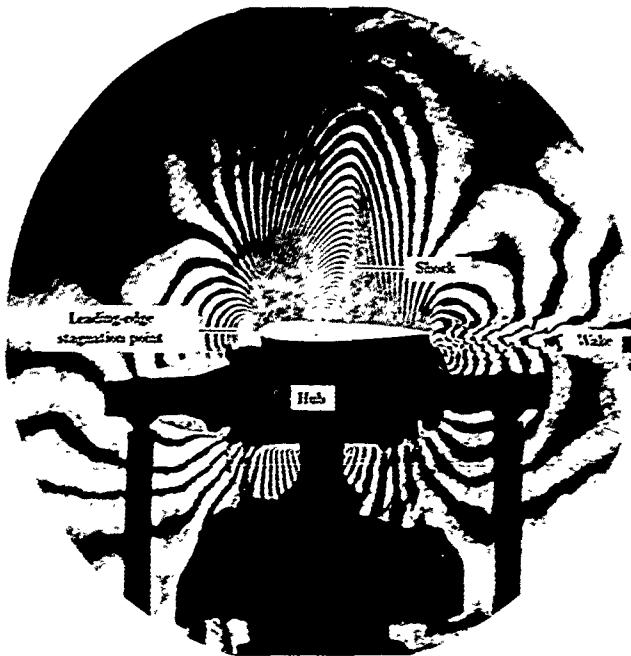
Figure 48. Interferogram recorded at \psi = 180^\circ (chordwise view). (From ref. 5.)
