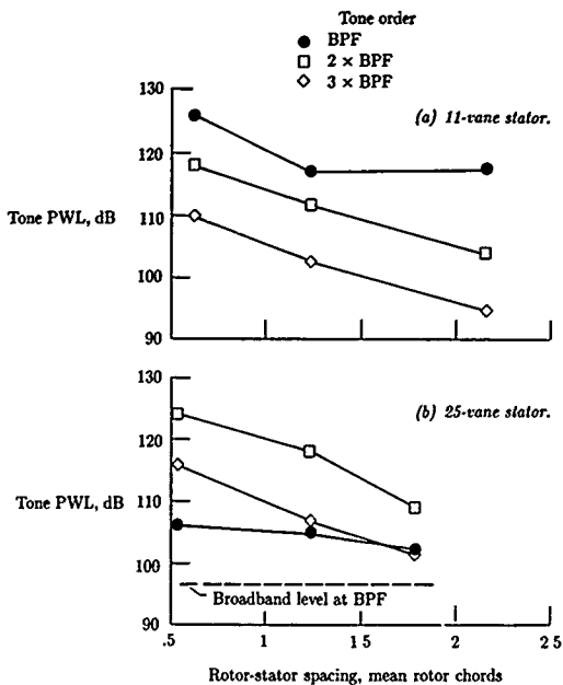
Figure 24. Variation of narrow-band tone harmonic power levels with rotor-stator spacing. 80 percent of design speed; 15 rotor blades; tunnel velocity, 41 m/sec (134.5 ft/sec). (From ref. 80.)
