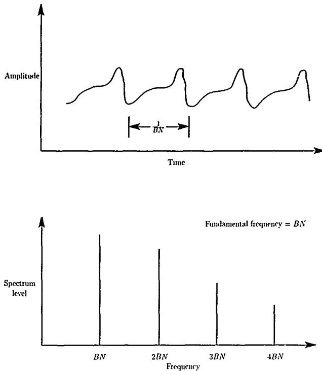
Figure 4. Characteristics of propeller rotational noise.
