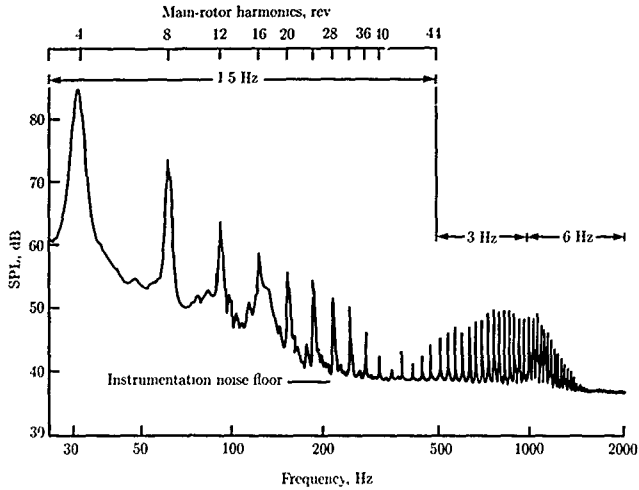
Figure 27. Narrow-band spectrum plot for OH-6A helicopter—main rotor only (4-bladed). (From ref. 24.)
