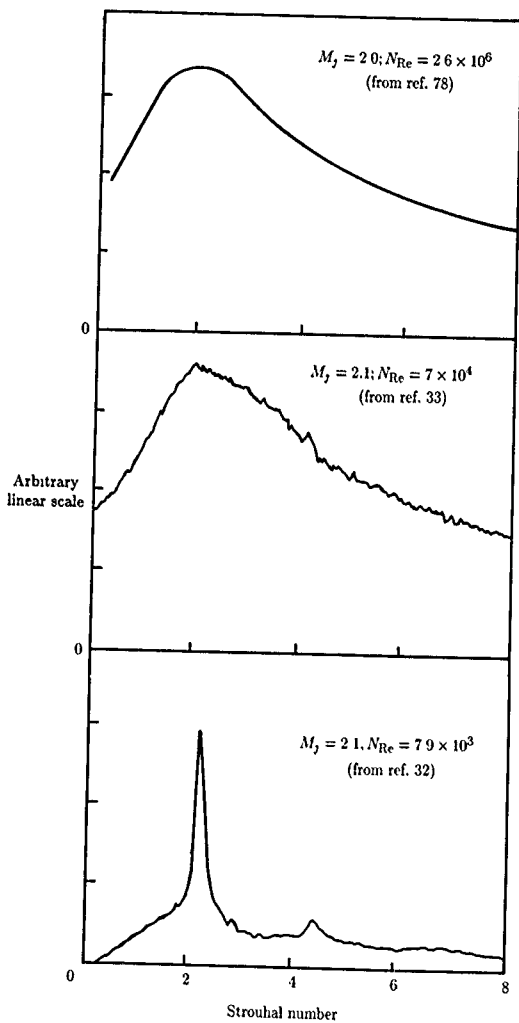
Figure 21. Acoustic spectra in direction of maximum noise radiation.
