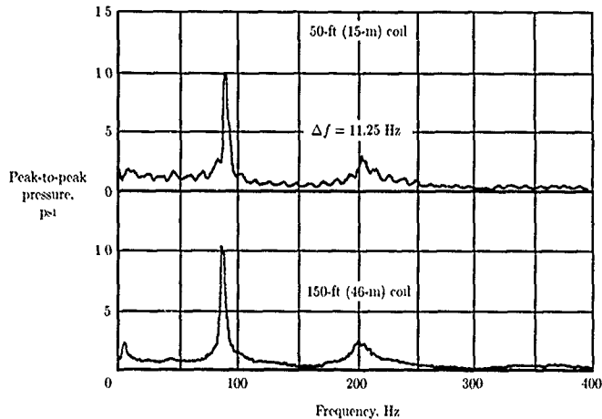
Figure 15. Comparison of pressure autospectra obtained simultaneously using two waveguide probes with different "infinite" coil lengths. 1 psi = 6.89 kPa.
