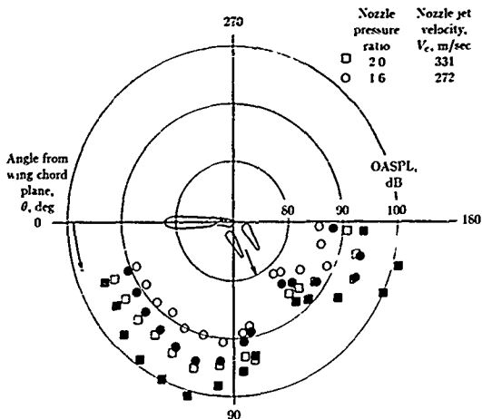
Figure 6. OASPL directivity for augmentor wing at approach flap deflection ( 65^\circ ) and zero forward speed. Open symbols denote acoustic treatment; solid symbols denote hard walls. (From ref. 8.)
