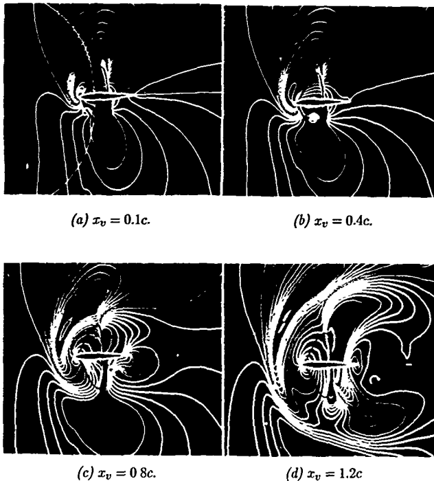
Figure 62. Pressure disturbance plots of NACA 0012 airfoil from computational Euler solution. M_\infty = 0.8 ; y_v = -0.26c , \Gamma_v = 0.2 . (From ref. 70)
