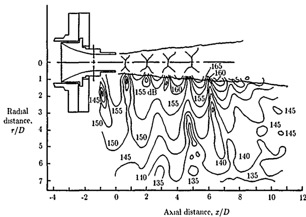
Figure 19. One-tenth-octave-band near-field SPL contours of screaming jet. f_s = 2 kHz; M_j = 1.67 ; helical screech mode. (From ref. 97.)
