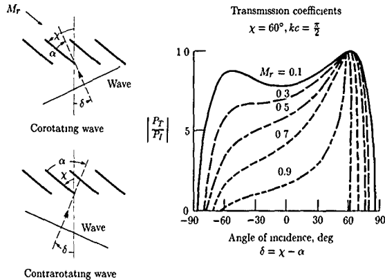
Figure 6. Blade row transmission. (Based on ref. 13.)
