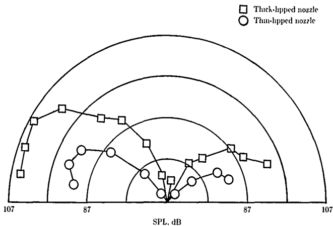
Figure 20. Comparison of far-field directivities of fundamental screech tones of two convergent nozzles at M_j = 1.49 (From ref. 92.)
