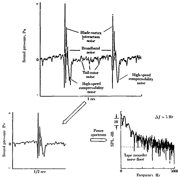
Figure 36. Time history and related power spectrum of UH-1H BVI impulsive noise. (From ref. 26.)
