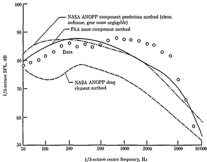
Figure 17. Comparison of measured and predicted flyover noise spectra for Boeing 747 with landing gear extended, at 222 knots. (From ref. 27.)
