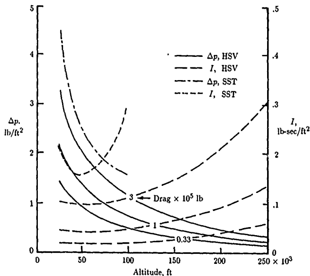
Figure 14. Overpressure and impulse as function of altitude for drag-dominated hypersonic vehicle. Conventional SST shown for comparison. (Based on ref. 52.)
