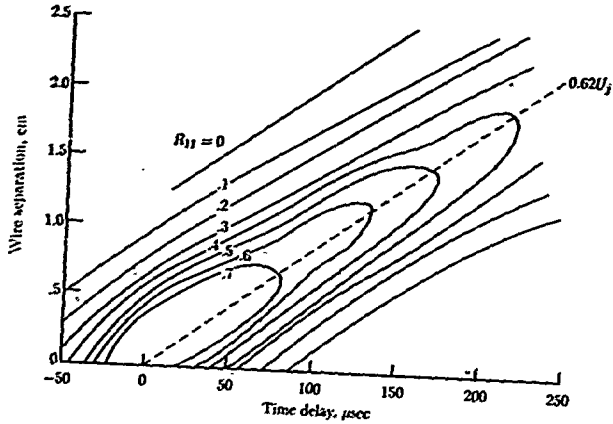
Figure 6. Isocorrelation curves of R_{11}(\xi, \tau) in 25-mm-diameter jet at M_j = 0.45 . y_1 = 1.5D_j ; \tau = 0.5D_j . (From ref. 29.)
