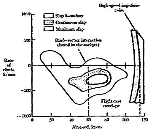
Figure 30. Impulsive-noise boundaries for UH-1H helicopter. (From ref. 5.)
