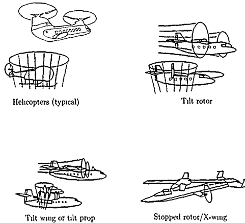
Figure 1. Current and promising rotorcraft configurations.
