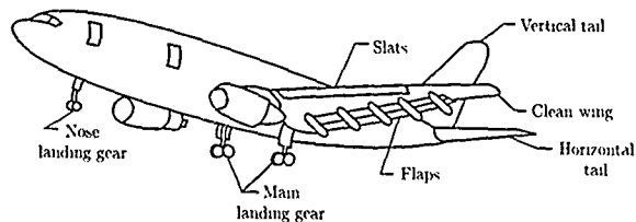
Figure 1. Sources of airframe noise. (From ref. 27.)
