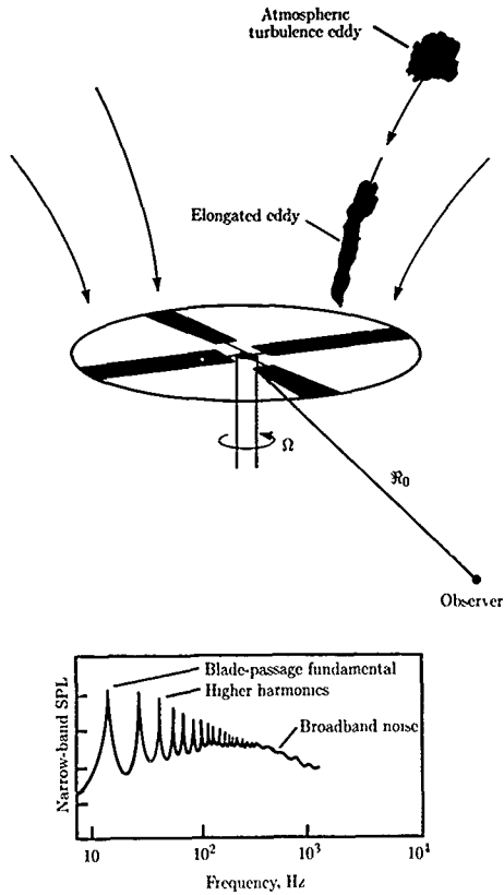
Figure 25. Origins of turbulence-ingestion noise.
