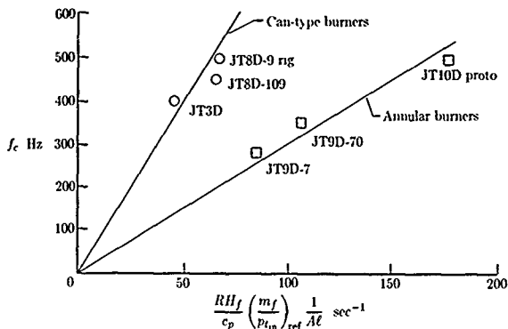
Figure 19. Comparison of core noise peak frequency correlation represented by equation (5) with experimental data. (From ref. 32. Copyright AIAA. Reprinted with permission.)
