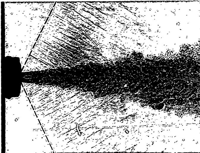
Figure 4. Directional acoustic radiation from supersonic jet generated by instability waves. Helium jet with reservoir pressure of 54.7 psia. (From ref. 22.)
