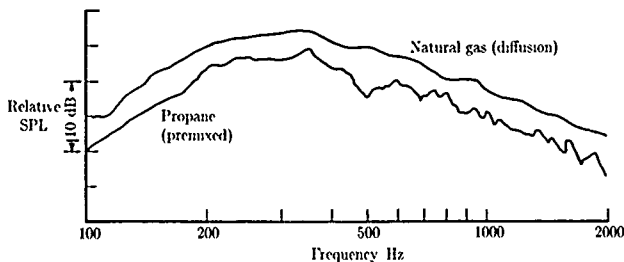
Figure 4. Typical sound pressure level spectra in the far field of open, turbulent, premixed and diffusion flames with gaseous hydrocarbon fuels. (From ref. 6. Copyright AIAA. Reprinted with permission)
