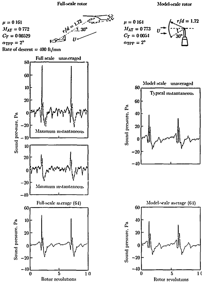
Figure 42. Unaveraged and averaged sound pressure time histories for one rotor revolution. (From ref. 27.)
