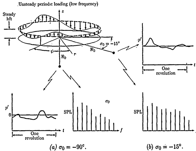
Figure 11. Relative contributions of low-frequency unsteady loading to helicopter rotor noise.
