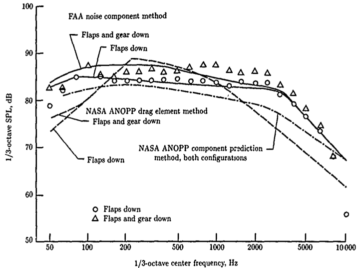
Figure 18. Comparison of measured and predicted flyover noise spectra for Boeing 747 with trailing-edge flaps and gear extended, at 204 knots. (From ref. 27.)
