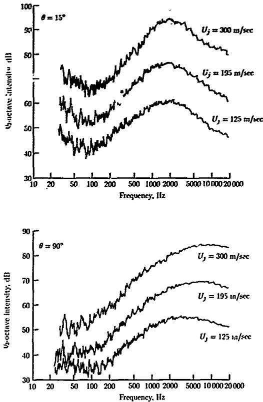
Figure 25. Jet noise spectra at \theta = 15^\circ and 90^\circ for various jet velocities. (From ref. 76).
