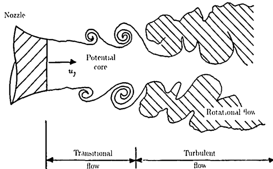
Figure 2 Schematic drawing of large turbulence structures in mixing layer of round jet at moderate Reynolds number (Based on ref. 6.)
