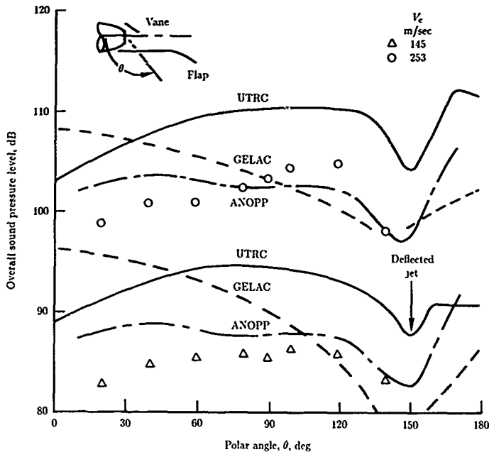
Figure 14. Predicted and measured OASPL directivity in flyover plane for USB model with circular nozzle and vane deflector at takeoff flap deflection. (From ref. 18.)
