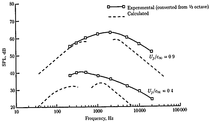
Figure 23. Calculated and experimental (ref. 77) jet noise spectra. D_j = 51 mm; \theta = 82.5^\circ ; y_1/D_j = 54 ; M_j/M_j = 0.05 .
