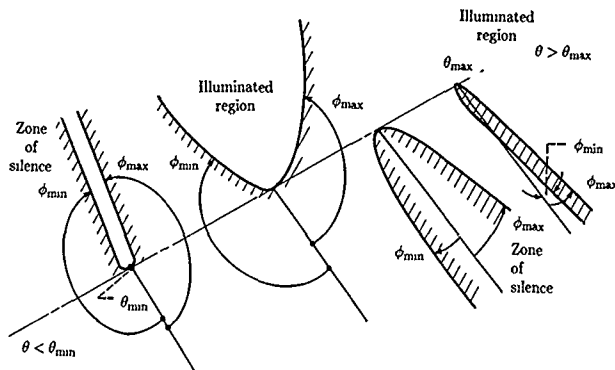
Figure 4. Asymmetric zone of silence.
