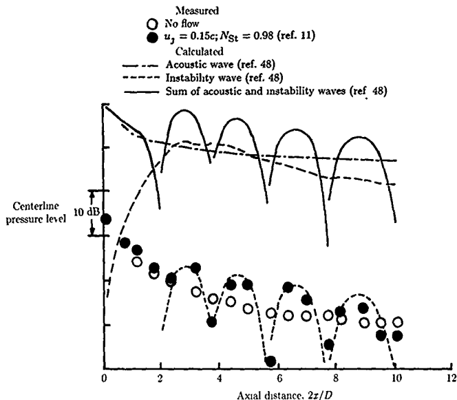
Figure 39. Prediction of centerline pressure fluctuation as sum of acoustic and instability waves and comparisons with experiments. (From ref. 48.)
