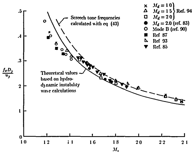
Figure 16. Strouhal number of dominant screech tone versus fully expanded jet Mach number for cold jets.
