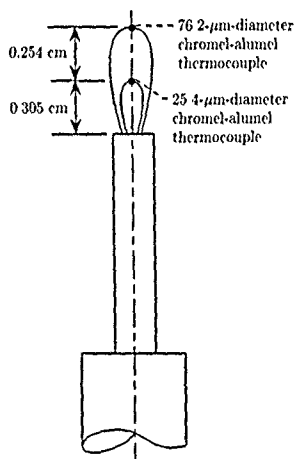
Figure 17. Two-wire thermocouple probe. (From ref. 34.)
