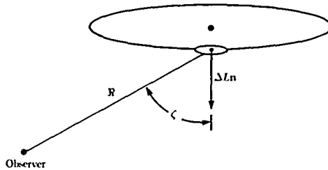
Figure 20. Geometry for far-field observer. (From ref. 5.)
