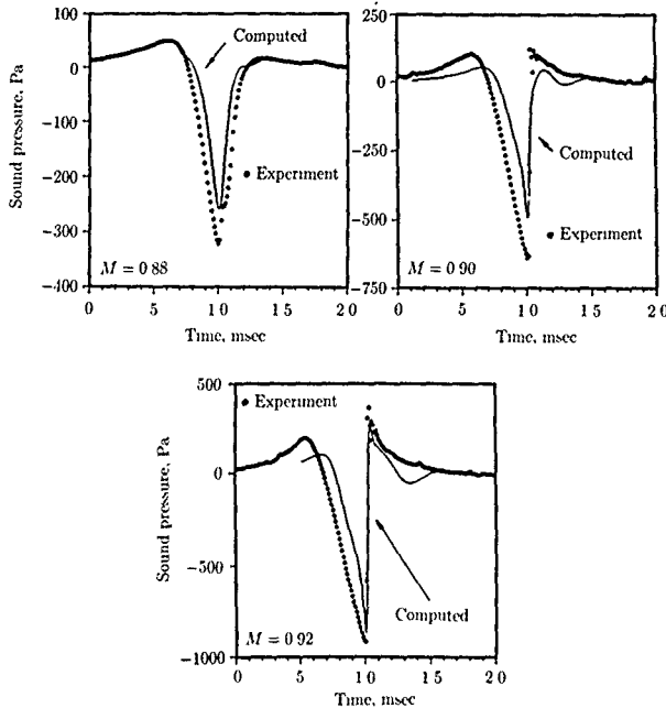
Figure 57. Predicted values from extended Kirchhoff computations and experimental values for M_T = 0.88, 0.90, and 0.92 .
