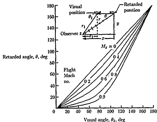
Figure 13. Relationship between retarded and visual angles. (From ref. 19.)
