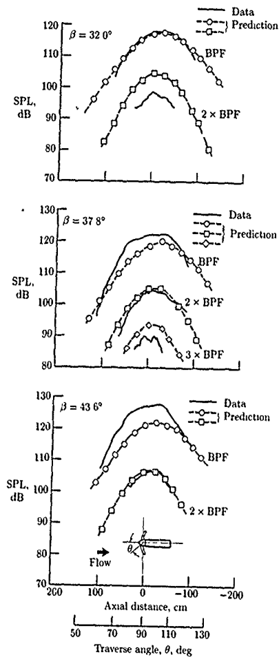
Figure 34. Measured and predicted values for SR-7A model. 1.68 m sideline; advance ratio, 0.886; M_x = 0.2 . (From ref. 69.)
