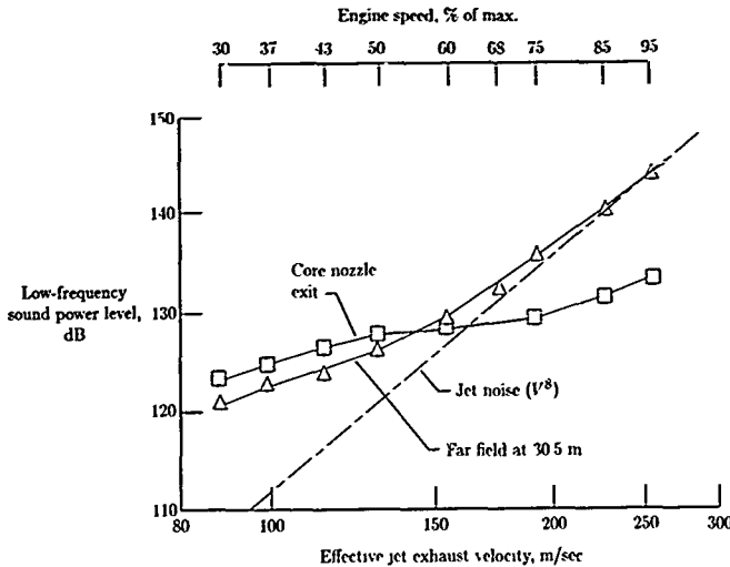
Figure 2. Low-frequency sound power in the far field and at the core nozzle exit of a turbofan engine as a function of effective jet velocity. (From ref. 4.)
