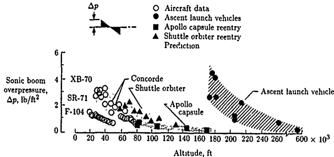
Figure 15. Measured and predicted on-track sonic boom overpressures in primary carpet area for several aircraft and spacecraft.
