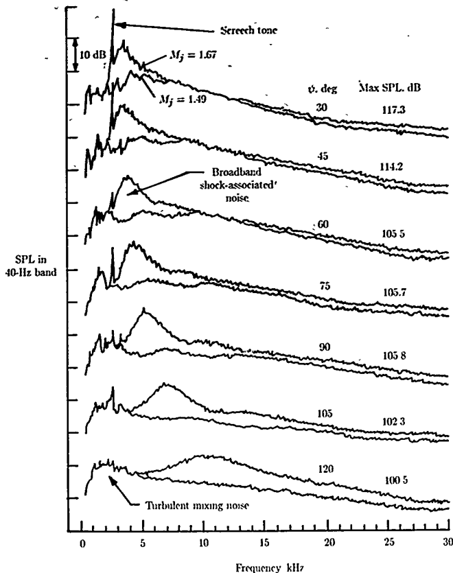
Figure 5. Narrow-band noise spectra of supersonic jet for fully expanded Mach numbers M_j of 1.49 and 1.67 and for jet inlet angles \psi of 30^\circ to 120^\circ . Nozzle design Mach number M_d = 1.5 . (Based on ref. 72.)
