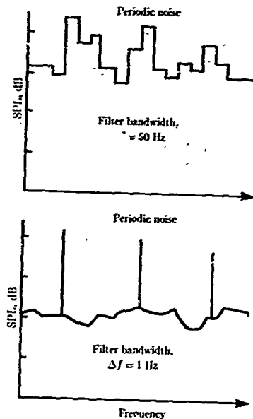
Figure 2. Effect of bandwidth reduction on spectra of rotorcraft noise.
