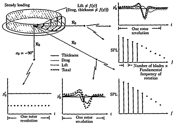
Figure 6. Relative contributions of steady loading and thickness effects to helicopter rotor noise.
