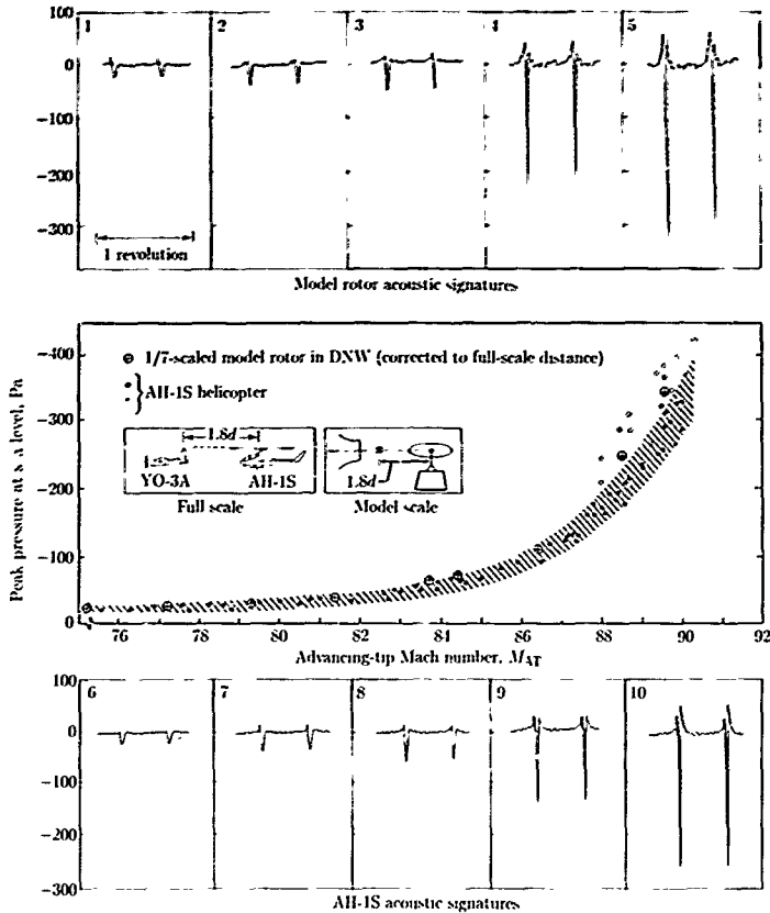
Figure 41. Model- and full-scale acoustic pressures for in-plane microphone 3.6 rotor radii ahead. (From ref. 5.)
