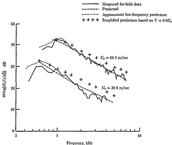
Figure 6. Measured far-field noise spectra and spectra predicted from measured surface pressure spectra. S(f) is power spectral density. \alpha = 90^\circ (flyover plane); \Theta = 90^\circ ; p_o = 20 \mu\text{Pa} . (From ref. 56.)
