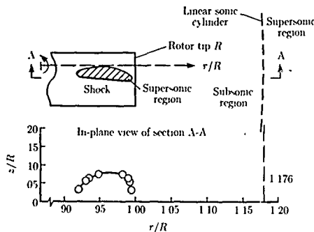
Figure 50. Top and aft views of shock boundaries of rotor at M_T = 0.85 . (From ref. 41.)
