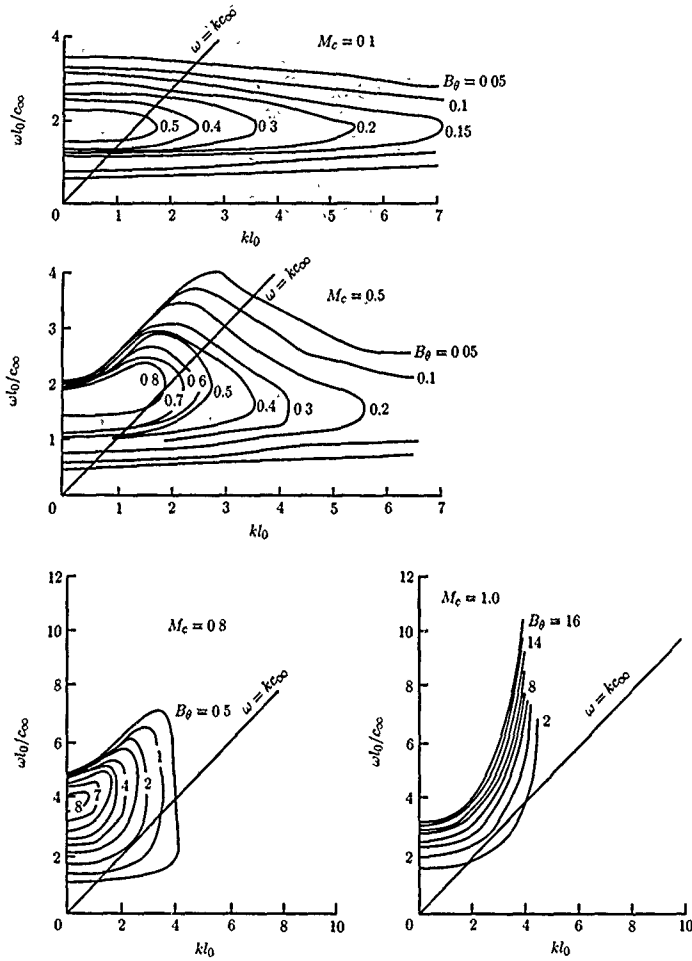
Figure 3. Isocorrelation curves of the Gaussian source function B_\theta for various values of convection Mach number.
