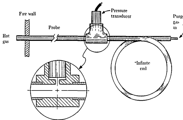
Figure 14. Waveguide pressure probe for use in hot gas path.
