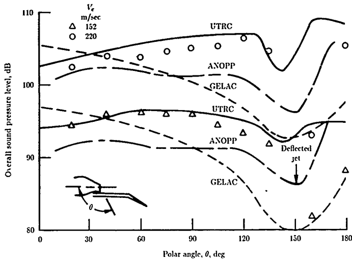
Figure 13. Predicted and measured OASPL directivity in flyover plane for QCSEE USB model at takeoff flap deflection. (From ref. 18.)
