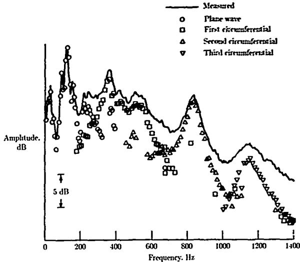
Figure 19. Measured pressure autospectrum and predicted contributions of individual modes in an annular gas turbine combustor. (From ref. 36.)
