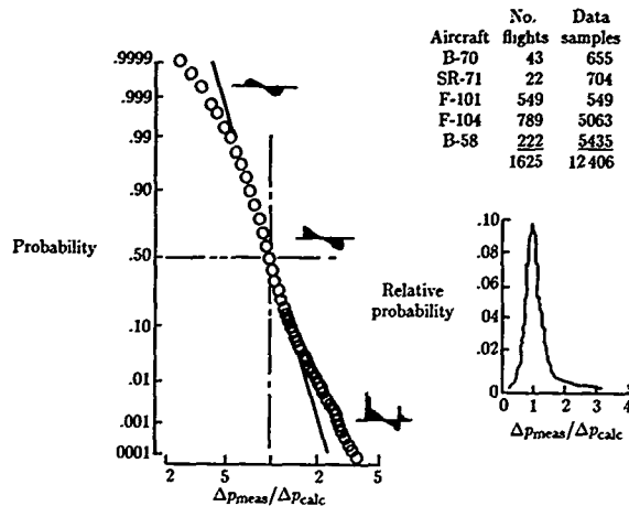
Figure 18. Statistical variation of sonic boom waveforms and overpressures resulting from atmosphere for steady, level supersonic flight.
