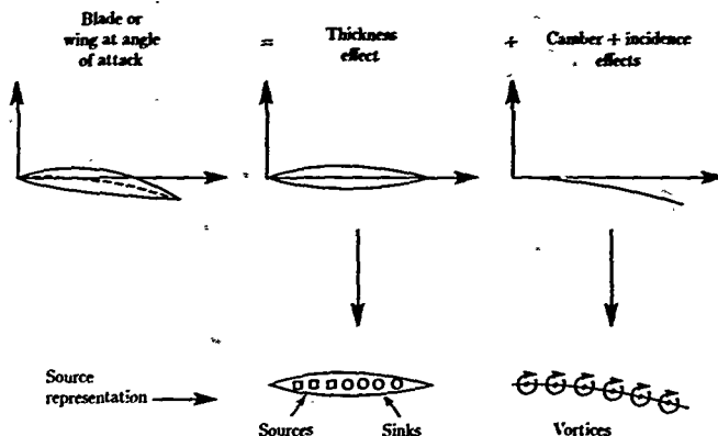
Figure 8. Decomposition of wing or blade section aerodynamics into thickness effect and camber and incidence effects. (Based on ref. 8.)
