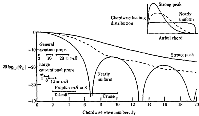
Figure 16. Reduction of loading noise from blade element due to chordwise noncompactness. (From ref. 17.)
