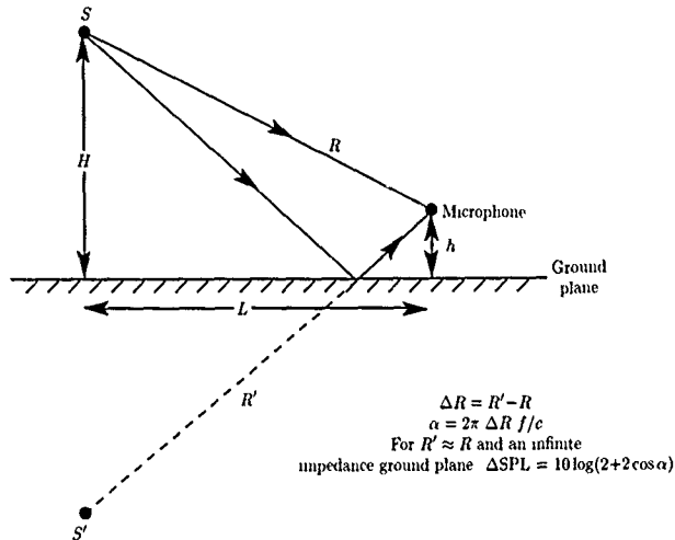
Figure 23. Ground reflection effects with image source.
