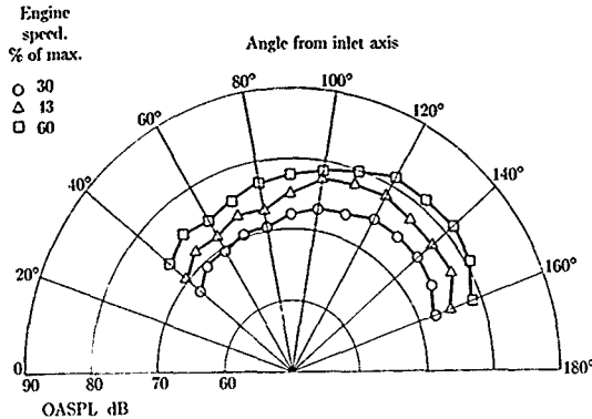
Figure 7. Combustion noise overall sound pressure level (OASPL) directivity patterns. (From ref. 13.)
