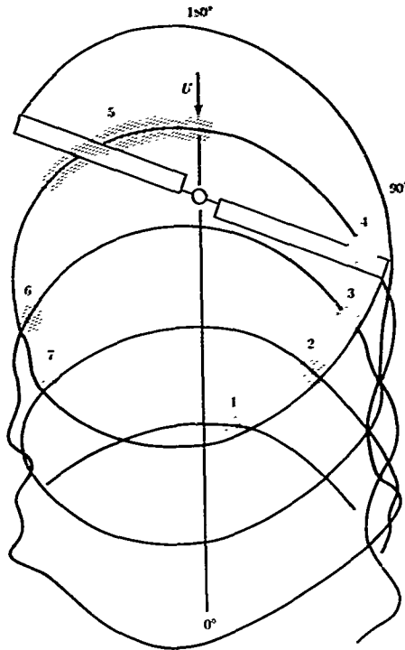
Figure 15. Blade-vortex intersections during partial-power descent. (From ref. 18.)
