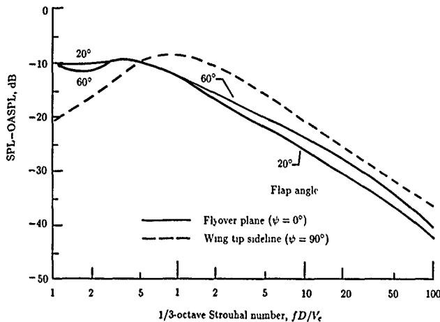
Figure 10. Normalized 1/3-octave-band spectra for USB configurations at all polar angles, used with the ANOPP noise prediction method (ref. 21).
