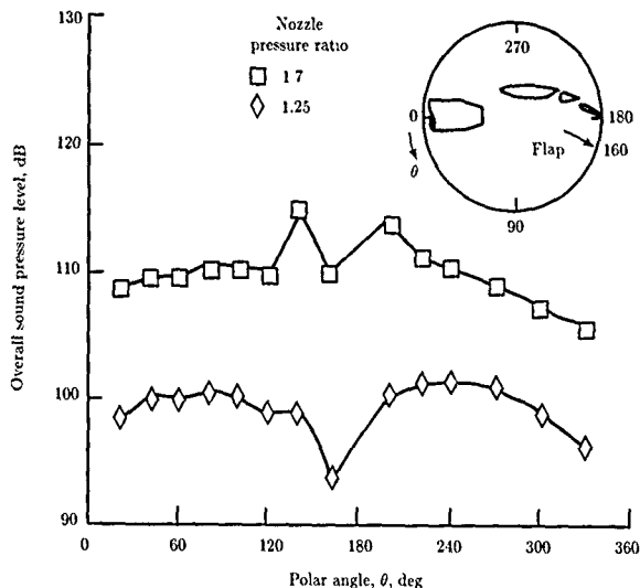
Figure 2. OASPL directivity in flyover plane for a small UTW model at takeoff flap deflection ( 20^\circ ) and zero flight speed.
