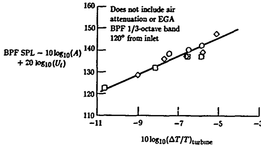
(b) Correlation for dominant tone SPL; based on turbine overall pressure ratio; 200-ft (61-m) sideline.
