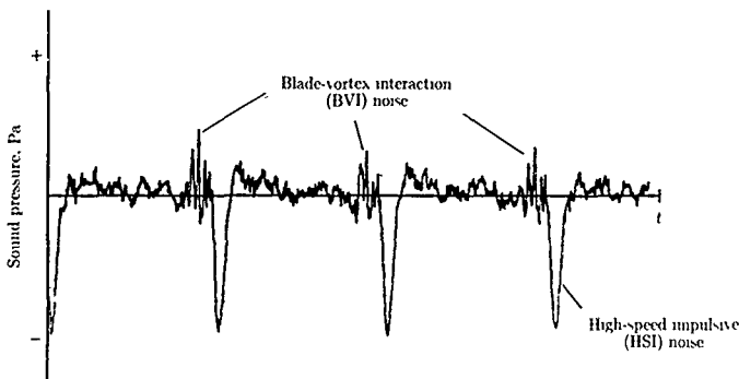
Figure 38. Acoustic signature of modern four-bladed helicopter. (Based on ref. 5.)
