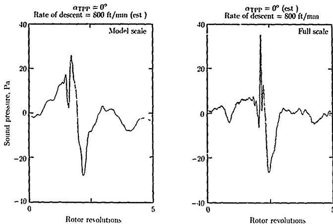
Figure 43. Model-scale and full-scale acoustic data for \mu = 0.270 . (From ref. 27.)
