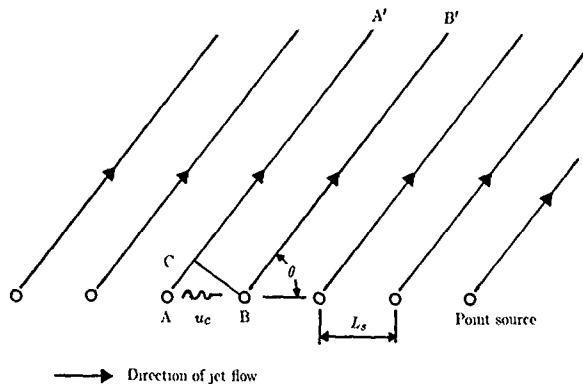
Figure 26. Schematic diagram of phased point-source array model.
