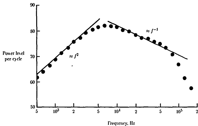
Figure 7. Noise power spectrum of M_j = 1.5 . (From ref. 74.)
