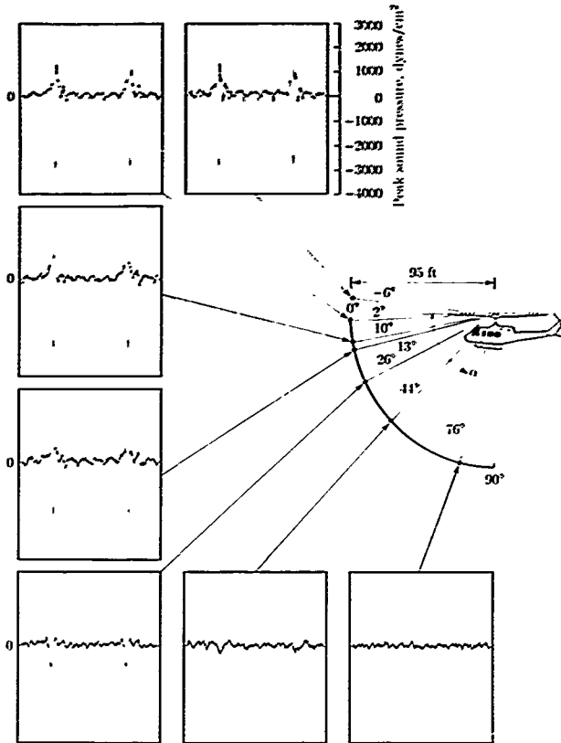
Figure 33. Longitudinal acoustic directivity for UH-1H in level flight at 115 knots IAS. \beta = 0^\circ . (From ref. 5.)
