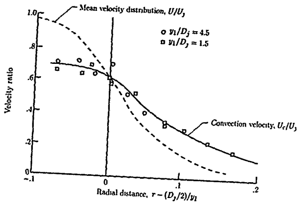
Figure 7. Variation of eddy convection speed across mixing region. (From ref. 29.)
