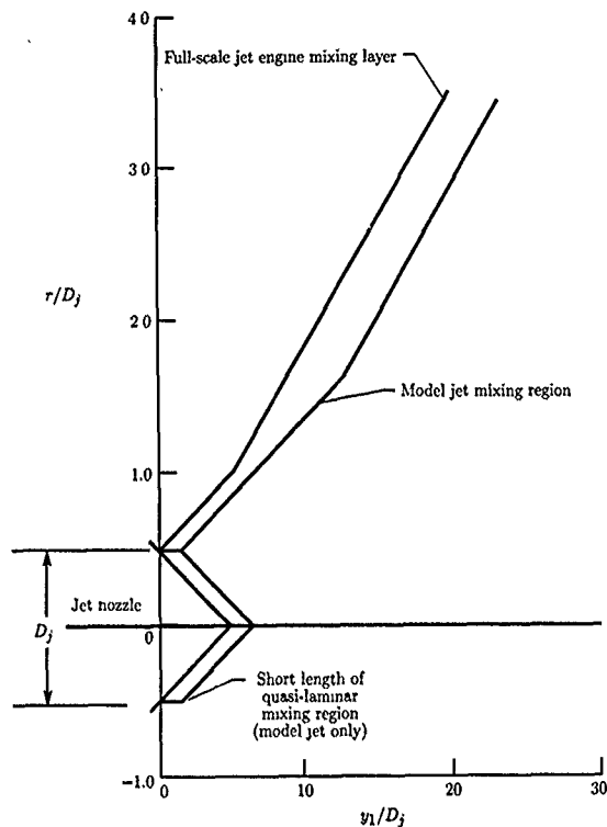
Figure 11. Diagram of composite mean width of mixing region.
