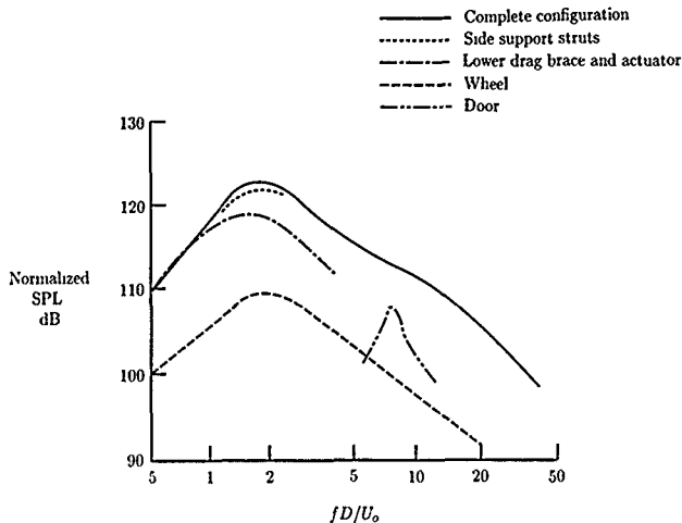
Figure 8. Normalized sideline spectra of nose gear model components. Reference flight speed, 100 m/sec. (From ref. 77.)
