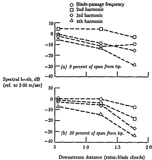
Figure 19. Mean wake harmonic levels from ensemble averaged spectra. Upwash component; 80 percent design speed; tunnel velocity, 41 m/sec (134.5 ft/sec). (From ref. 67.)
