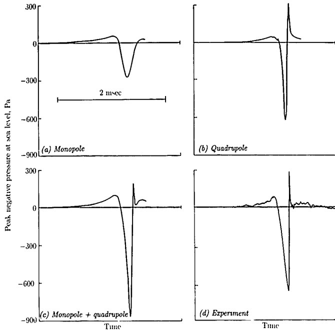
Figure 55. Theoretical and experimental time histories at M_T = 0.90 R_0/R = 3.0 (From ref. 5.)
