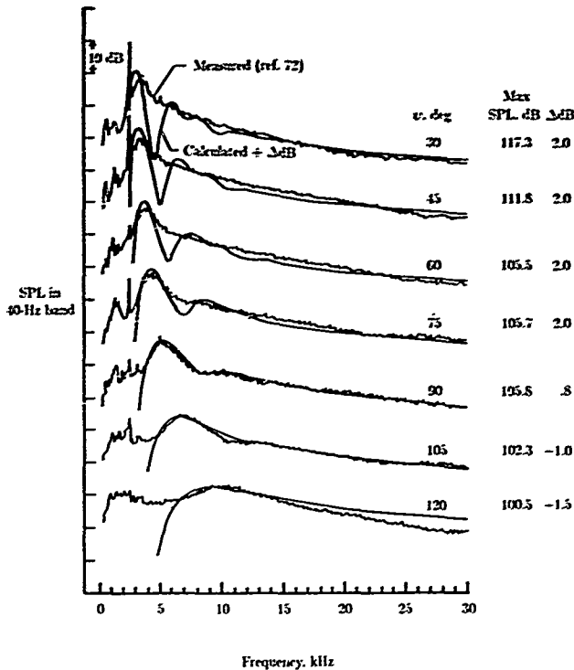
Figure 27. Far-field noise spectra. M_j = 1.67 ; M_d = 1.50 .
