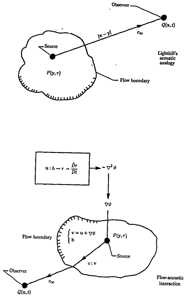
Figure 32. Differences between Lighthill's acoustic analogy theories of aerodynamic noise related to flow-acoustic interaction.
