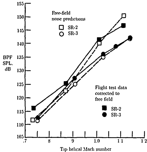
Figure 27 Measured and predicted sideline tone levels versus tip helical Mach number. Boom microphones, power coefficient, 1.9; advance ratio, 3.1. (From ref. 66.)
