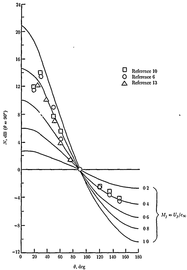
Figure 1. Directional distribution of jet noise as function of convection Mach number. U_j = 300 \text{ m/sec} ; M_c = 0.62M_j .
