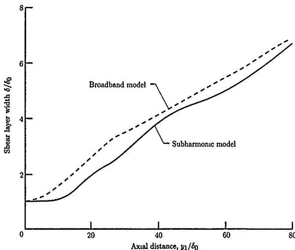
Figure 10. Calculated growth of shear layer at low speeds. (From ref. 61.)
