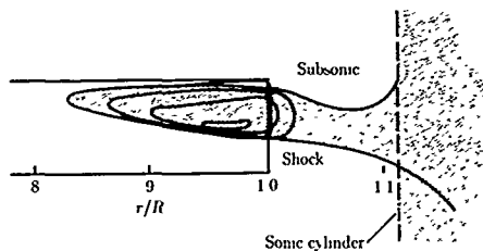
Figure 53. Tip flow field of hovering rotor. M_T = 0.90 . (From ref. 58.)
