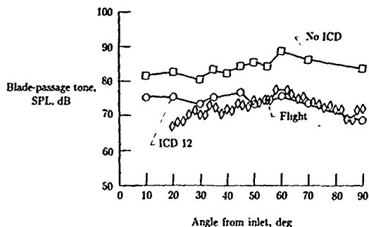
Figure 13. Effectiveness of inflow control for flight fan tone simulation. (From ref. 40.)
