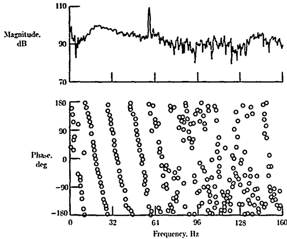
Figure 21. Pressure-temperature cross-spectrum at the exit of a can-type combustor. (From ref. 34.)
