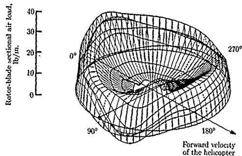
Figure 13. Air loads of rotor in forward flight. (From ref. 17.)
