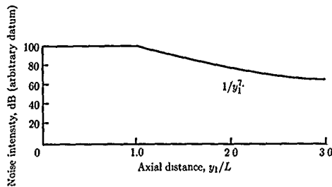
Figure 19. Jet noise effective source distribution at low Mach numbers for static jet.
