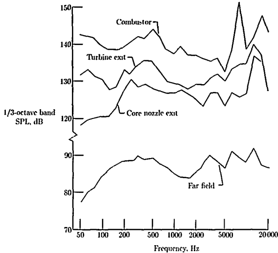
Figure 6. One-third-octave band sound pressure levels measured in the combustor, at the turbine exit, at the core nozzle exit, and in the far field of a turbofan engine having an annular combustor. (From ref. 4.)
