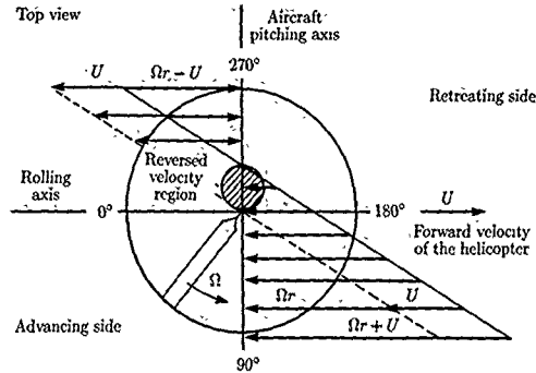
Figure 12. In-plane velocity asymmetry for rotor in nonaxial forward flight.
