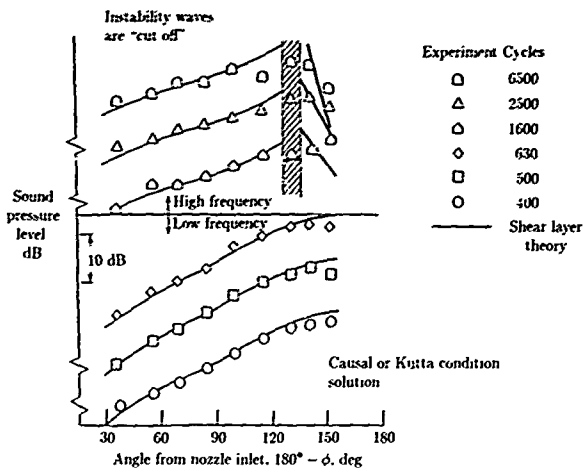
Figure 2. Comparison of causal or leading-edge Kutta condition solution with data of ref. 23 for U_j = 213 m/sec.
