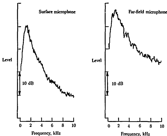
Figure 3. Comparison of spectral density functions for surface pressure fluctuations near a trailing edge and for far-field pressure fluctuations. (From ref. 42.)
