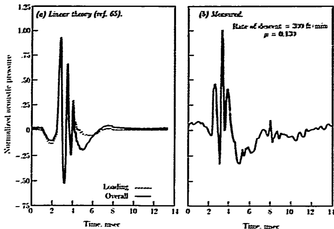
Figure 59. Blade-vortex interaction impulsive-noise time histories of AH-1 model rotor.
