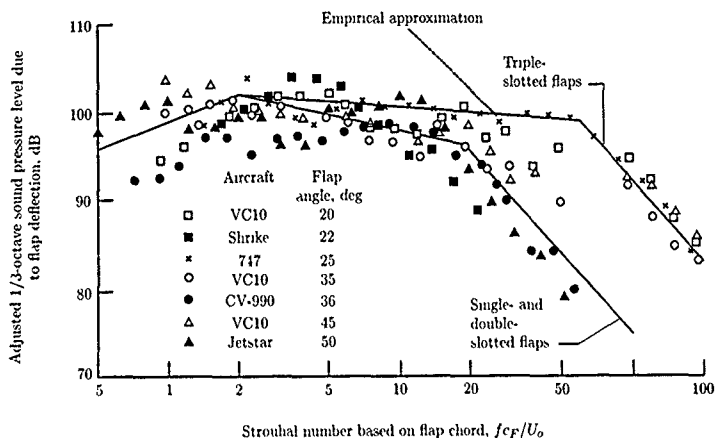
Figure 15. Measured normalized spectra of trailing-edge flap noise. (From ref. 27.)
