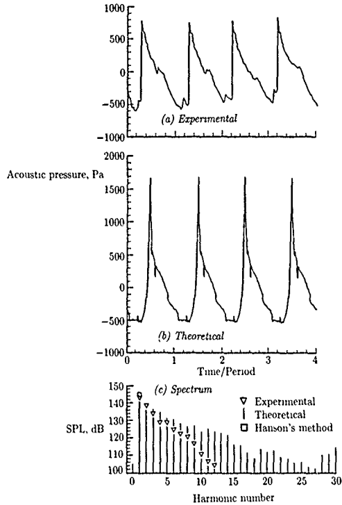
Figure 29. Measured and predicted acoustic pressure signatures and spectrum for boom microphone directly above propeller disk. Theoretical prediction corrected for boom reflection. Period, 0.991 msec; BPF = 1009.2 Hz. (From ref. 10.)
