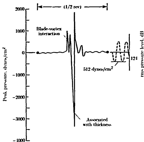
Figure 31. Composite illustration showing dominant UH-1H acoustic waveform features. (From ref. 5.)
