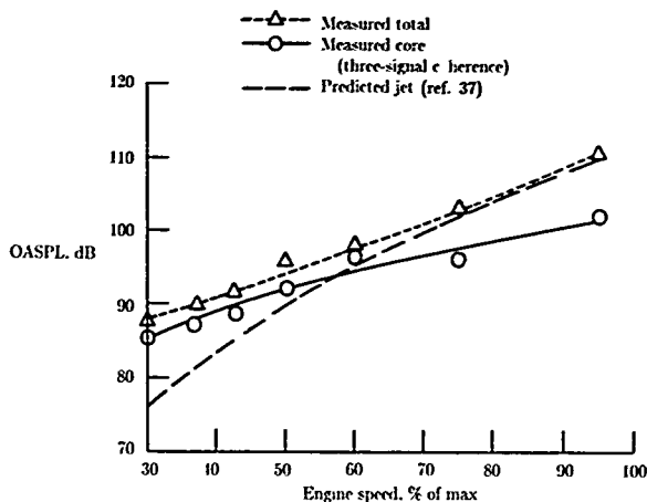
Figure 20. Engine core noise as a function of engine speed measured directly using the three-signal coherence technique. (From ref. 5.)
