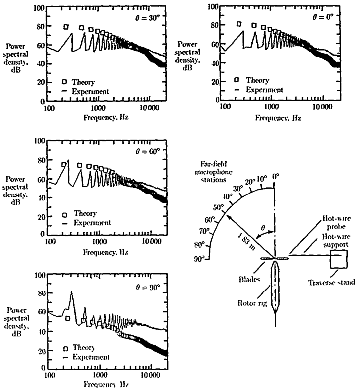
Figure 63. Predicted peak levels and measured spectra for hovering turbulence ingestion noise. (From ref. 74.)
