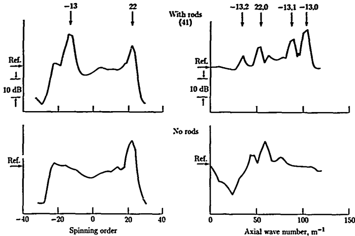
Figure 20. Inlet mode measurements on JT15D engine at 10 800 rpm. (Based on ref. 72.)
