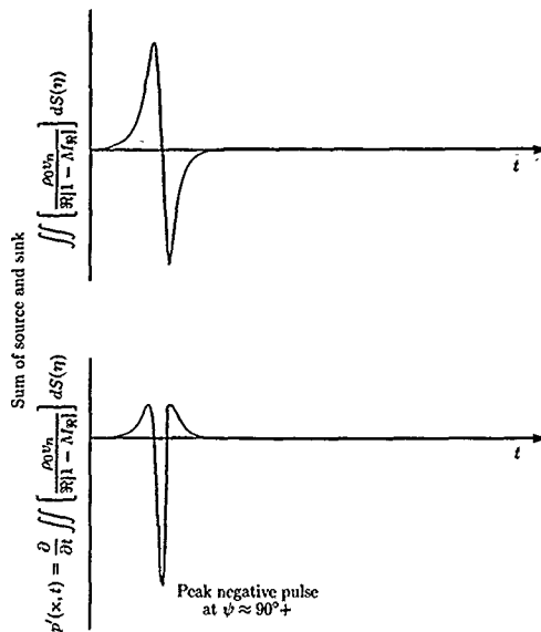
Figure 10. Simple source and sink far-field acoustic pressures. (From ref. 5.)
