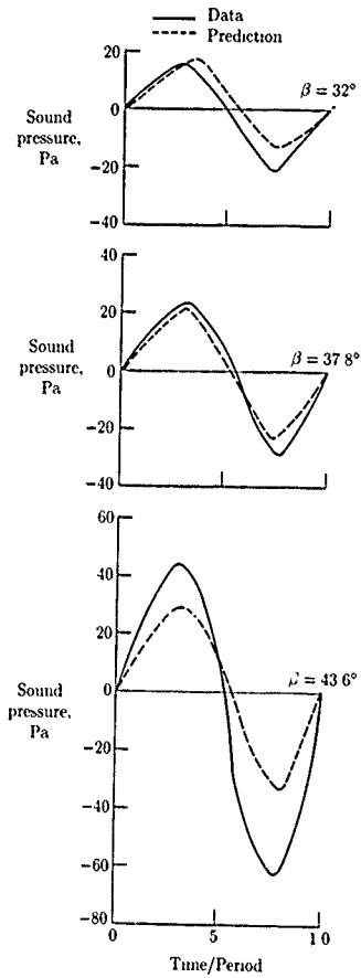
Figure 35. Waveforms in plane of propeller at three blade angles. Advance ratio, 0.886; M_x = 0.2 . (From ref. 69.)
