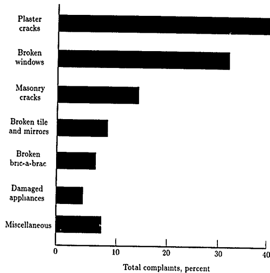
Figure 28. Sonic boom damage complaints. (From ref. 6.)
