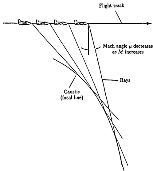
Figure 11. Sonic boom focusing due to acceleration.
