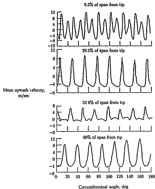
Figure 18. Rotor mean wake velocity profiles as a function of spanwise location. 1.23 rotor chords downstream; 80 percent design speed; tunnel velocity, 41 m/sec (134.5 ft/sec). (From ref. 67.)
