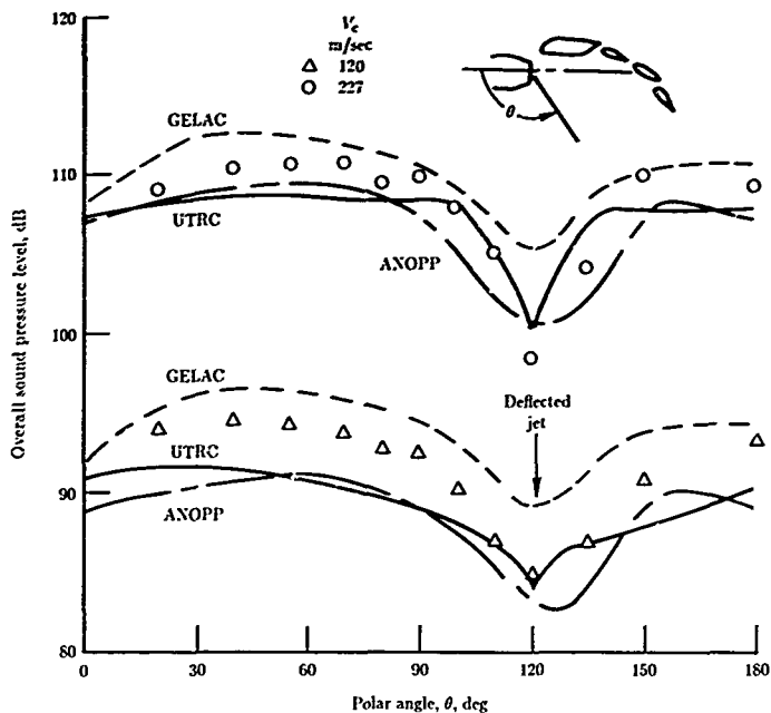
Figure 12. Predicted and measured OASPL directivity in flyover plane for three-flap UTW model at approach flap deflection. (From ref. 18.)
