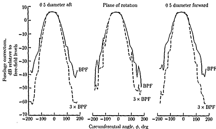
Figure 21. Calculated fuselage scattering effects at M_x = 0.8 . (From ref. 42.)
