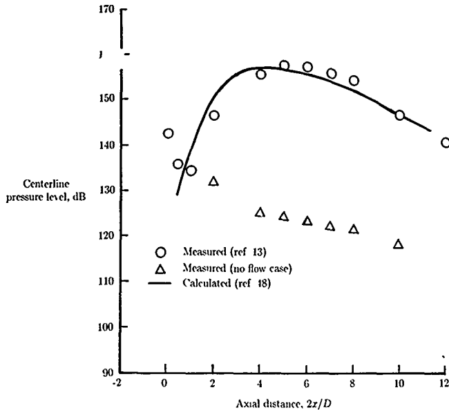
Figure 38. Calculated and measured instability wave amplitudes for cold jet. M_j = 0.575 ; Pressure ratio = 1.25; N_{St} = 0.5 ; Excitation level at nozzle exit = 141 dB; plane wave mode. (Based on ref. 48.)
