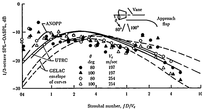
Figure 15. Predicted and measured normalized 1/3-octave-band spectra in flyover plane for USB model with circular nozzle and vane deflector. (From ref. 18.)
