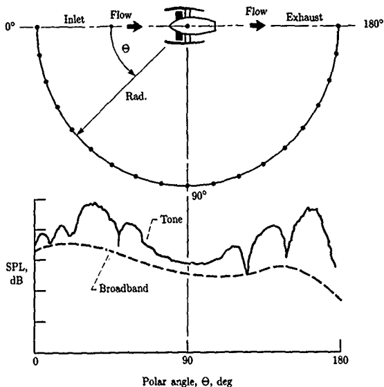
Figure 28. Typical turbomachinery sound pressure level polar directivity patterns.
