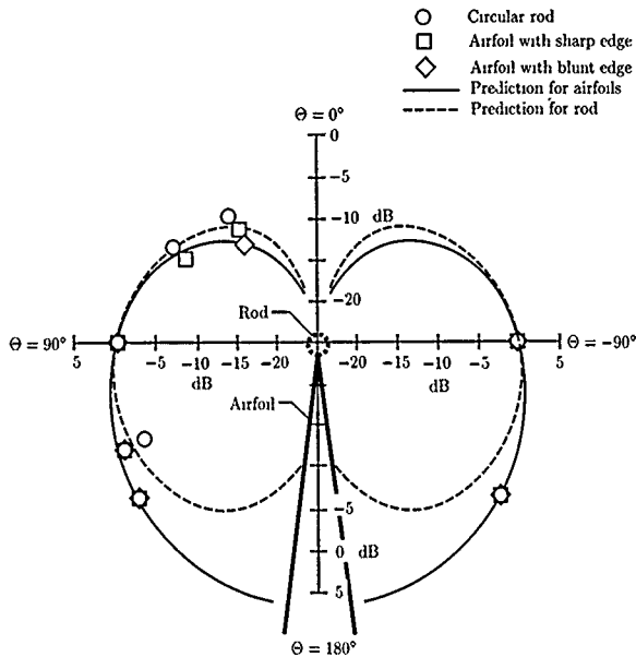
Figure 5. Directivity of trailing-edge noise OASPL in flyover plane as function of emission-time angle \Theta . Data corrected for wind-tunnel shear layer refraction. (From ref. 56.)
