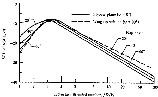
Figure 9. Normalized 1/3-octave-band spectra for UTW configurations at all polar angles, used with the ANOPP noise prediction method (ref. 21).
