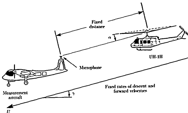
Figure 29. Technique for in-flight acoustic measurement. (From ref. 5.)
