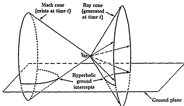
Figure 6. Mach and ray cones in supersonic flight.
