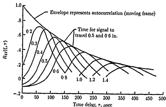
Figure 5. Cross correlation R_{11}(\xi, \tau) in 25-mm-diameter (1.0-in.) jet at M_j = 0.45 , y_1 = 1.5D_j ; r = 0.5D_j . (From ref. 29.)
