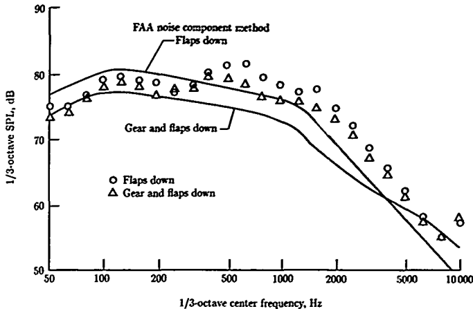
Figure 19. Comparison of measured and predicted flyover noise spectra for Convair CV-990, with trailing-edge flaps extended ( 36^\circ ) at 189 knots and flaps and gear extended at 160 knots. (From ref. 27.)
