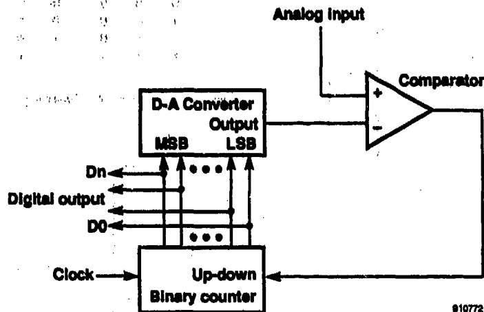
Figure 3-3. Tracking analog-to-digital converter.
