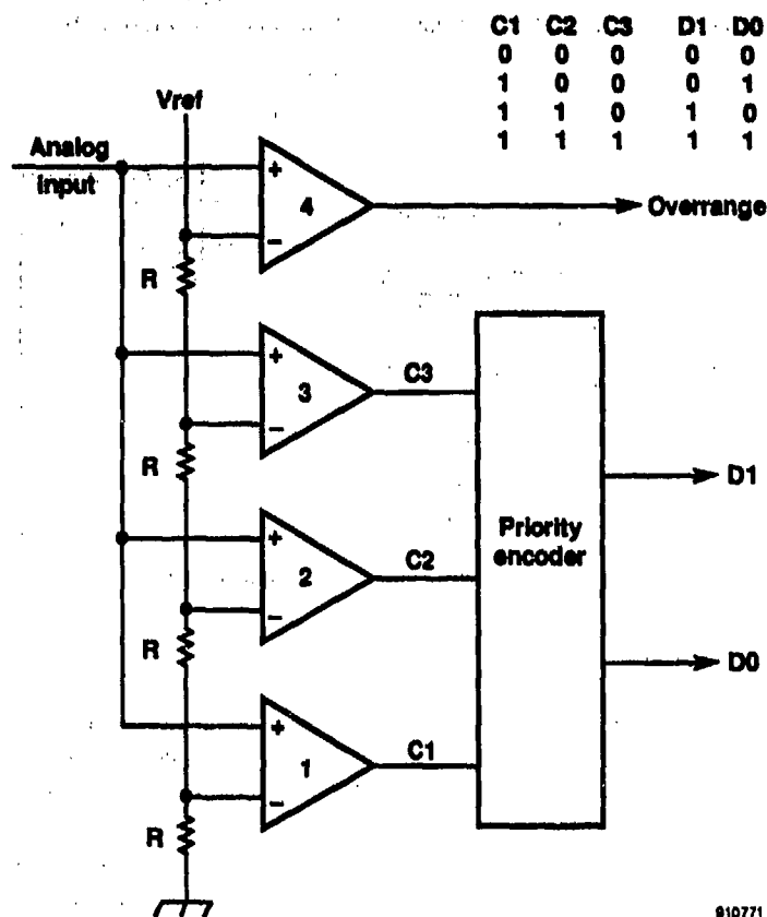
Figure 3-2. Simplified 2-bit flash converter.
