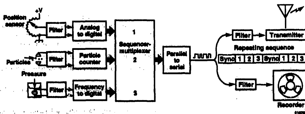
Figure 1-2. Simplified aircraft data acquisition system.
