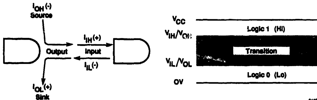
Figure 2-2. Logic circuit parameter-naming conventions.
