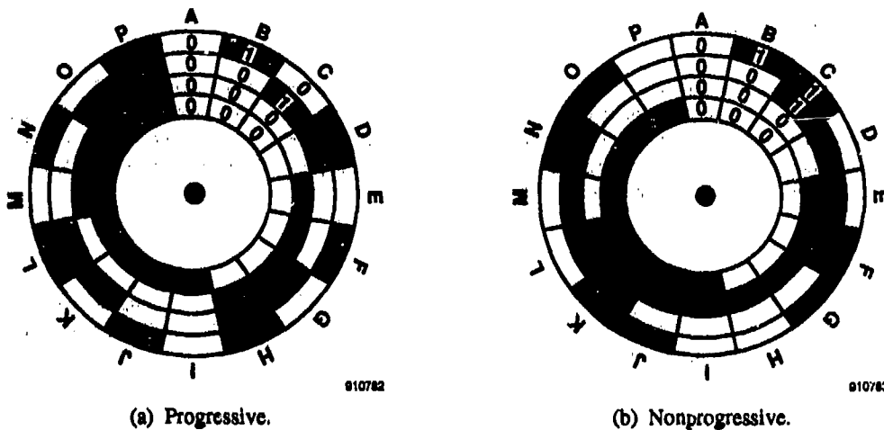
Figure 4-1. Encoded disks.
