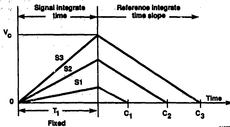
Figure 3-1. Dual slope integration analog-to-digital converter.
