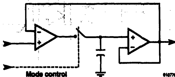
Figure 3-7. Sample and hold circuit.
