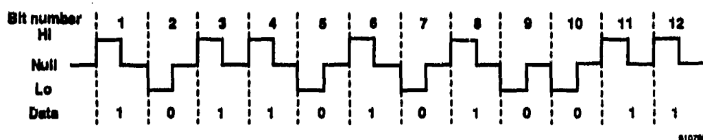
Figure 6-7. Bipolar RZ coding.
