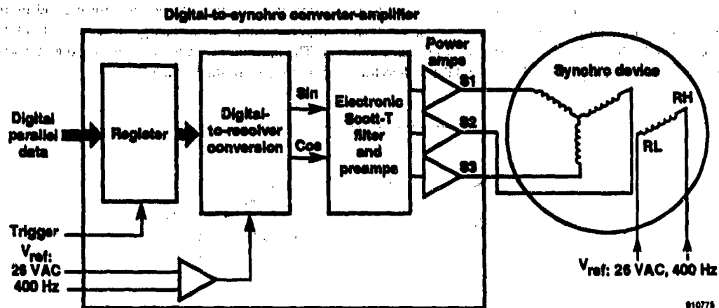
Figure 3-6. Typical digital-to-synchro system.
