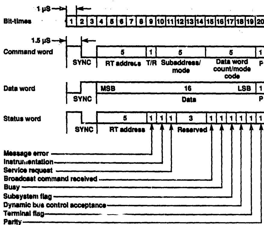
Figure 6-3. Word formats for MIL-STD-1553.
