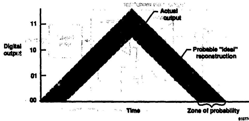
Figure 3-5. Digital-to-analog conversion.
