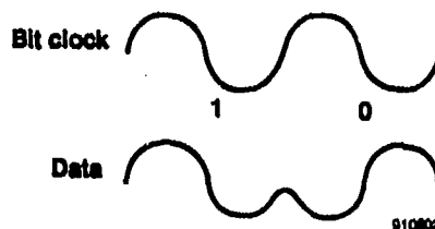
Figure 6-14. The H009 bus waveform.
