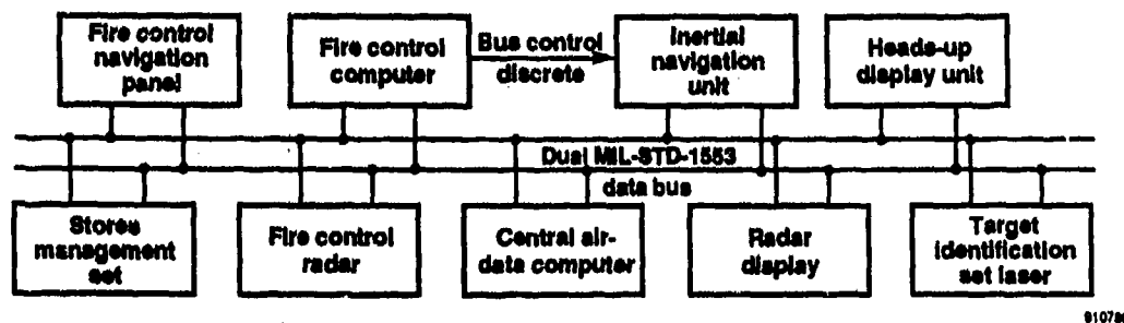
Figure 6-1. The F-16 avionics system architecture.
