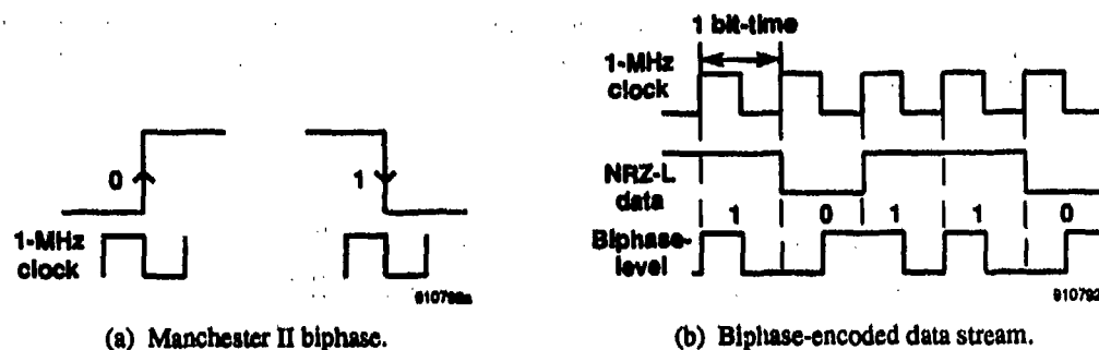
Figure 6-4. Data encoding for the Manchester II biphasic-level.
