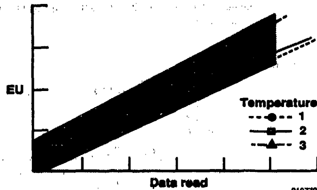
Figure 3-10. Temperature effects on a calibration.
