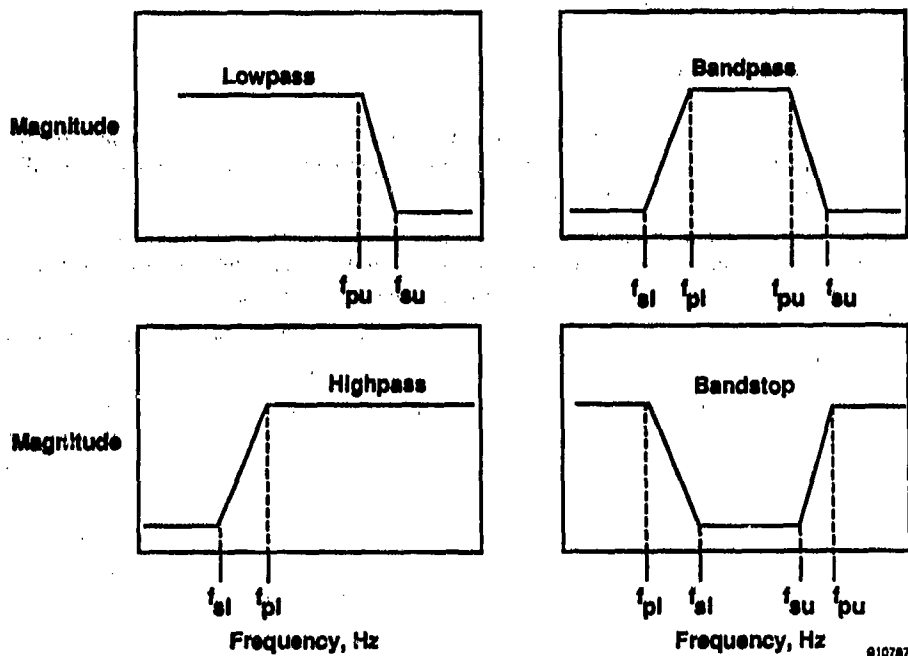
Figure 5-1. Time domain filters.
