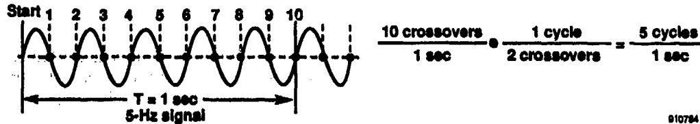
Figure 4-2. Zero-crossing count to determine frequency.
