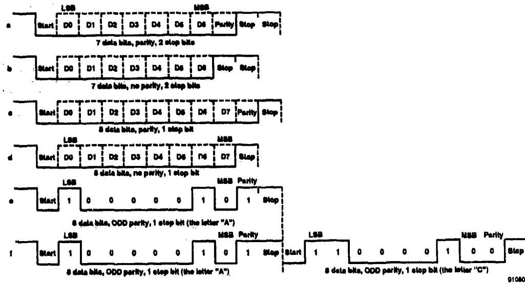
Figure 6-17. Examples of bit-sequential ASCII.
