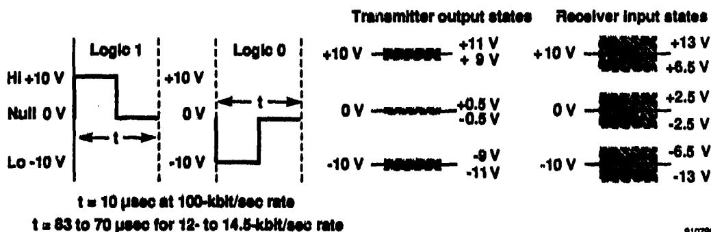
Figure 6-8. The ARINC 429 bit timing and signal levels.
