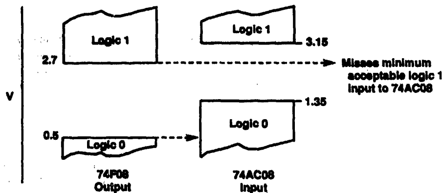
Figure 2-3. Logic family interfacing problem.
