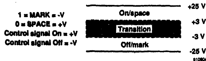
Figure 6-16. The RS-232-C voltage levels.
