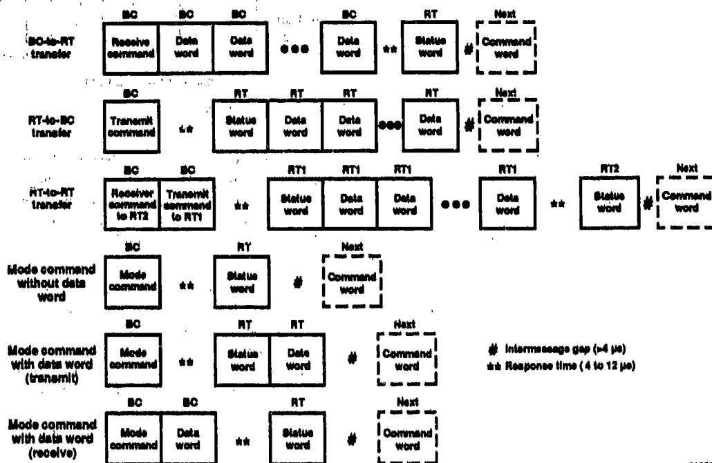
Figure 6-5. Bus message formats.
