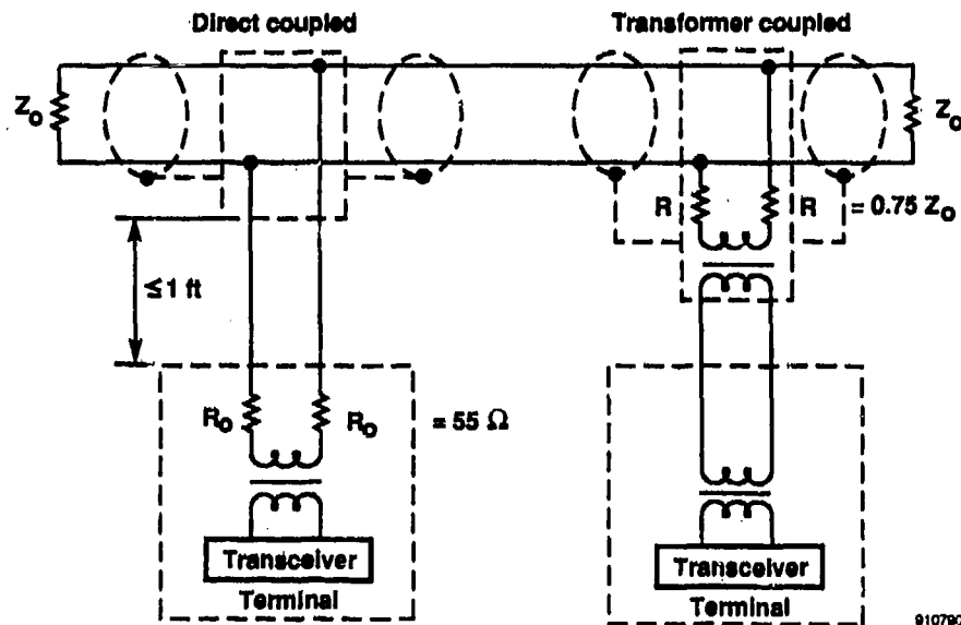
Figure 6-2. Connections to the MIL-STD-1553 data bus.
