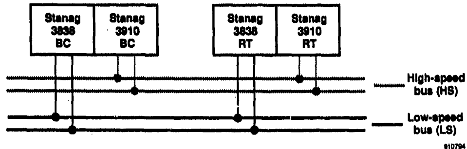
Figure 6-6. Hybrid high-speed/low-speed bus.
