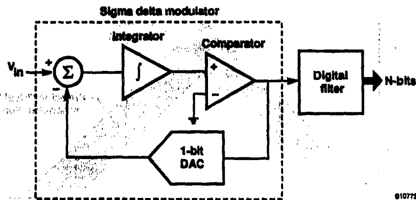
Figure 3-4. Sigma delta analog-to-digital converter.
